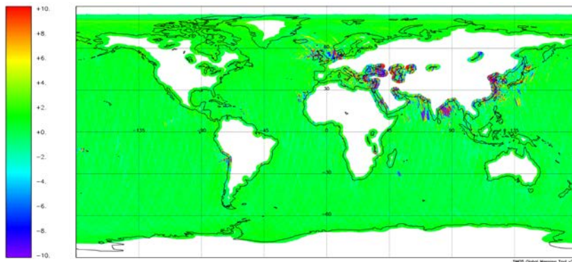
Weekly average of the 4 th Stokes parameter over the Ocean during the period 28 January – 4 February 2013. Areas affected by strong RFI show a 4 th Stokes parameter above 10K in absolute value.
