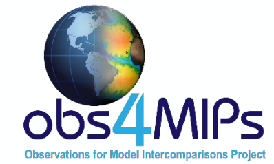
From: IPCC AR6, Chapter 3, Fig. 42
