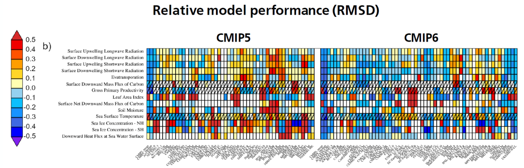
From: IPCC AR6, Chapter 3, Fig. 42
