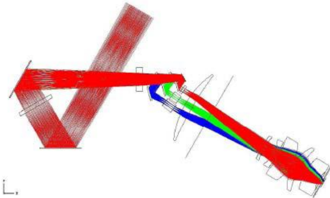
Figure 4.3: TIR Optical Design
