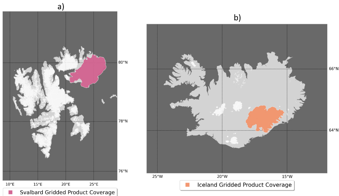
Figure 6: CryoTEMPO-EOLIS gridded product coverage for a) Svalbard and b) Iceland.
