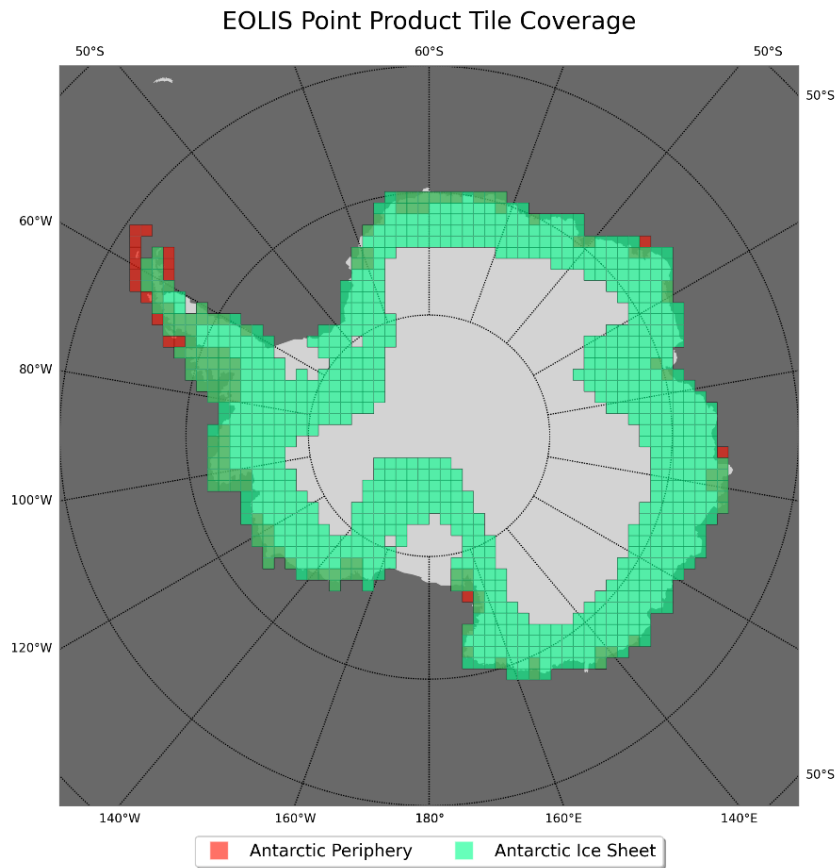
Figure 4: CryoTEMPO-EOLIS point product coverage for regions using the Southern Polar Stereographic projection system. Tiles are 100 x 100km.
