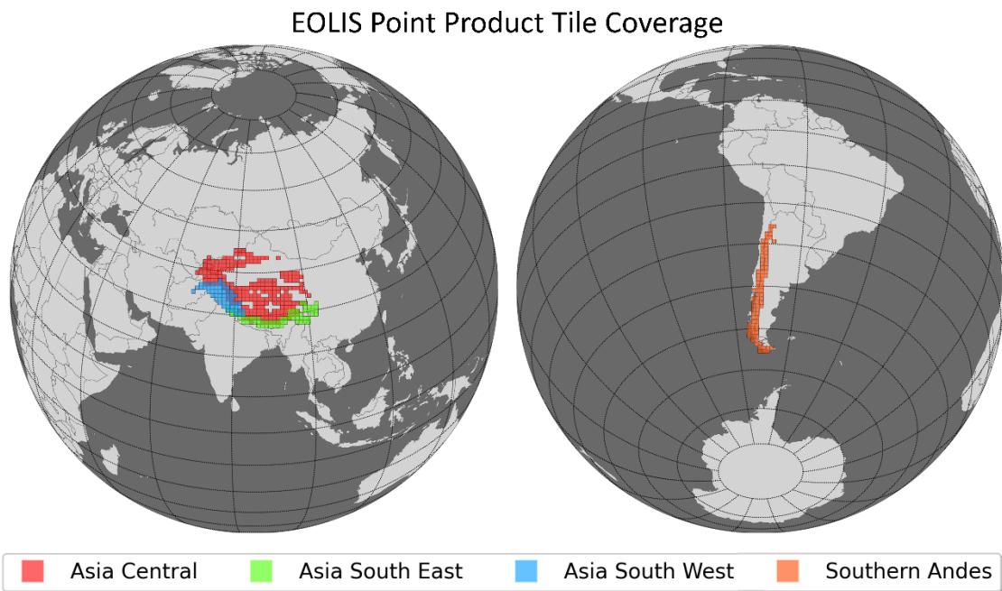
Figure 5: CryoTEMPO-EOLIS point product coverage for all regions using the WGS84 projection system. Tiles are 100 x 100 km.
