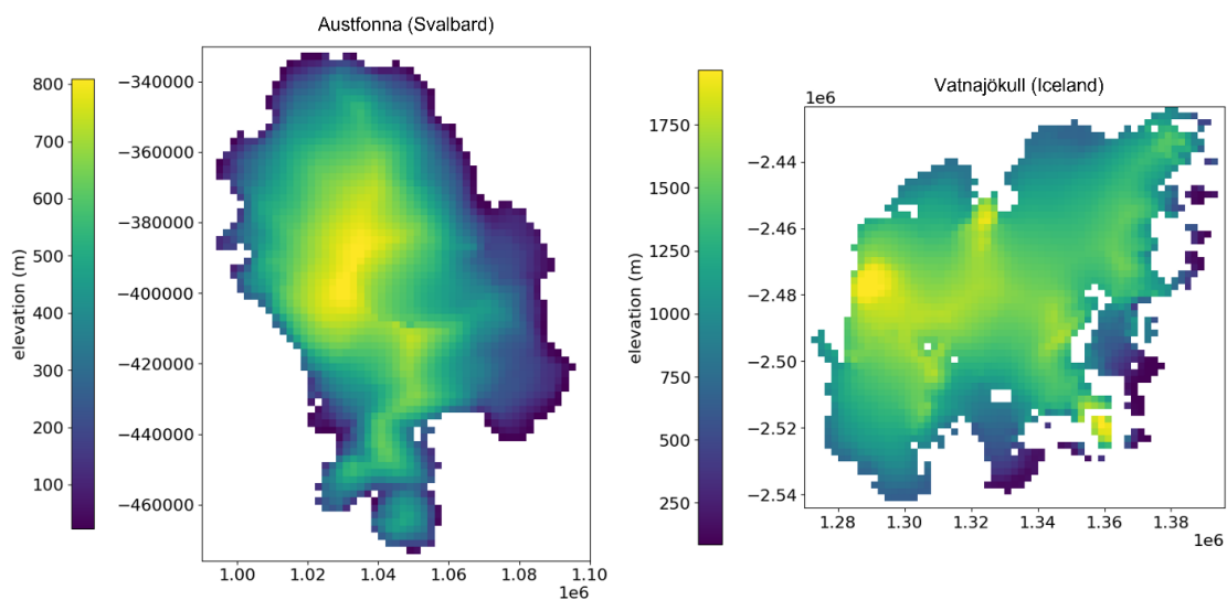
Figure 15: CryoTEMPO-EOLIS gridded products covering Austfonna (left) and Vatnajökull (right) for February 2019.
