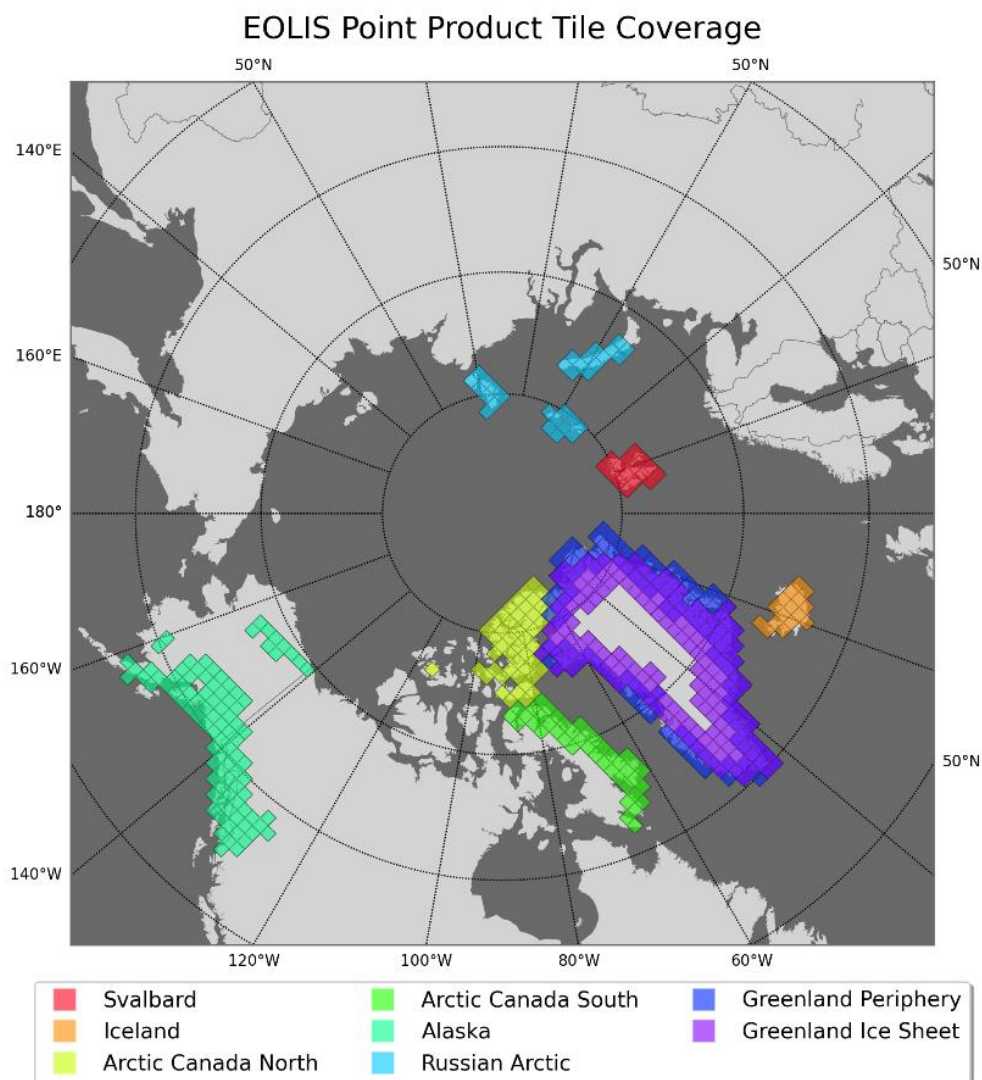
Figure 3: CryoTEMPO-EOLIS point product coverage for all regions using the Northern Polar Stereographic projection system. Tiles are 100 x 100 km.
