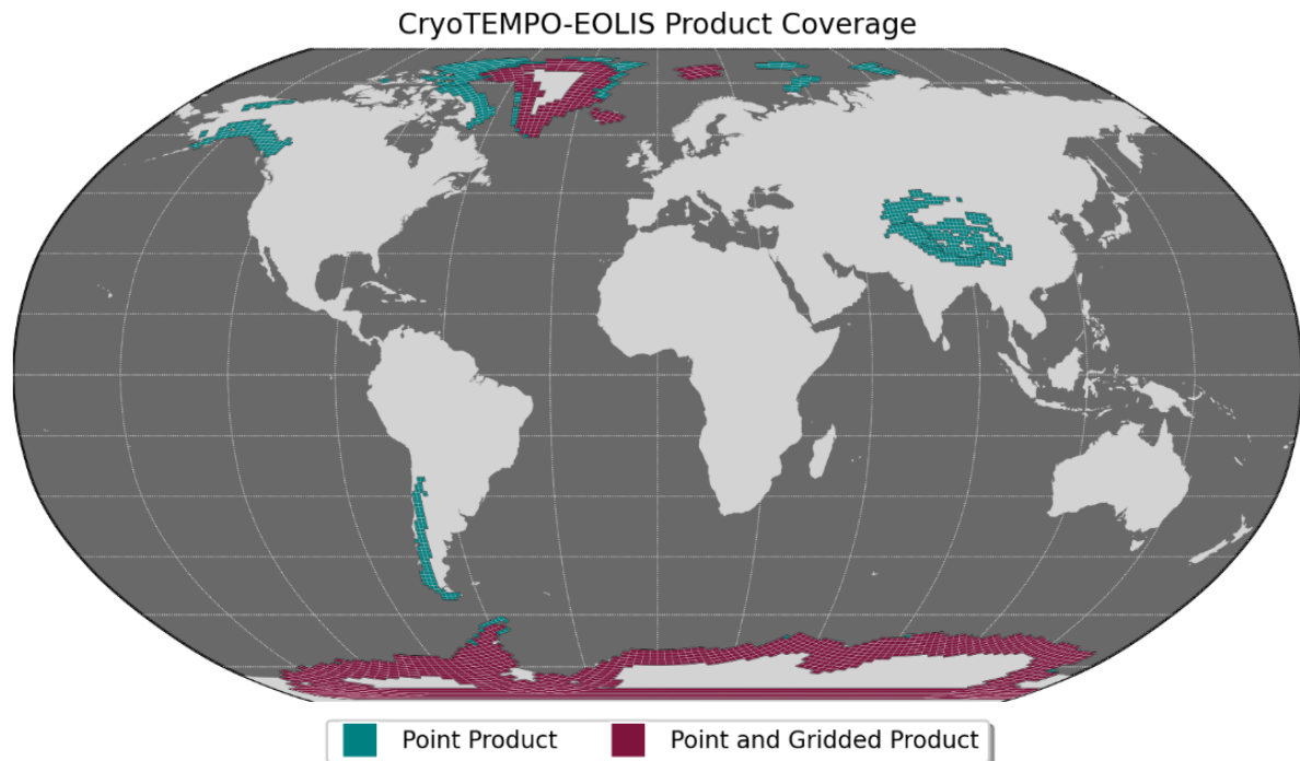
Figure 2: CryoTEMPO-EOLIS product coverage.
