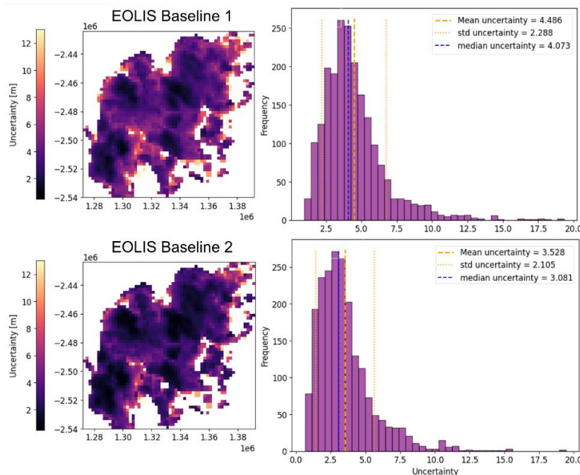
Figure 10: Reduction of uncertainties for the Vatnajökull ice cap between EOLIS Baseline 1 (top) and EOLIS Baseline 2 (bottom). The data shown is from the gridded product for February 2019. Left: uncertainty maps for the region, right: distributions of uncertainty values, with mean and median values indicated, as well as the standard deviation.
