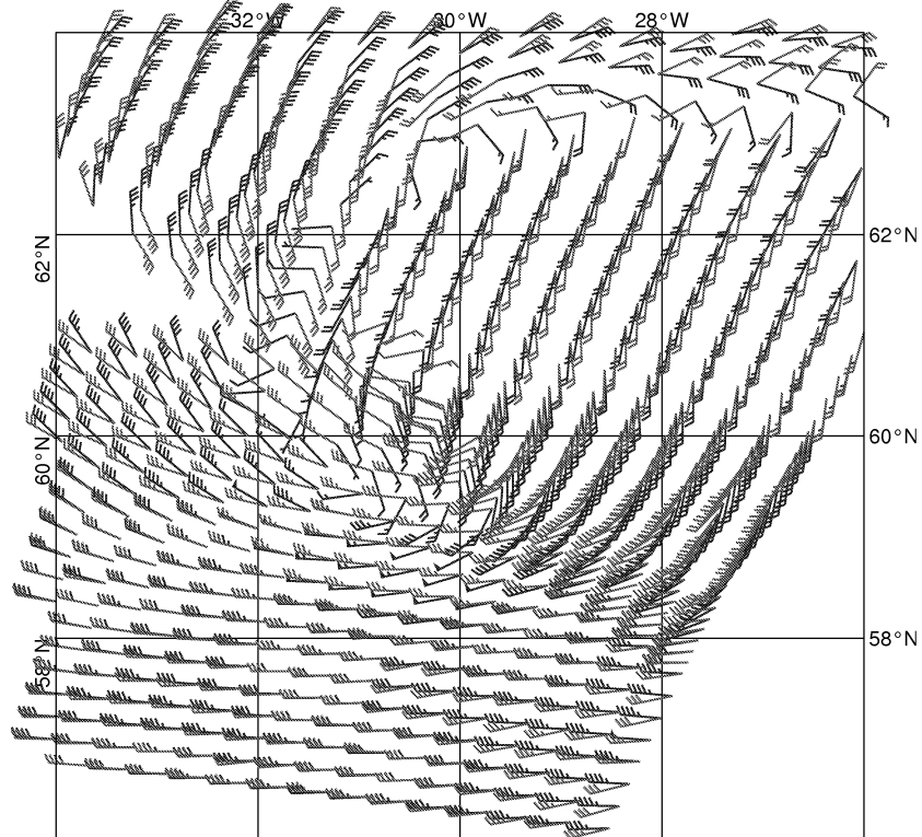
UWI winds (red) versus ECMWF FG winds (blue) North Atlantic 20110131 13:00 UTC
