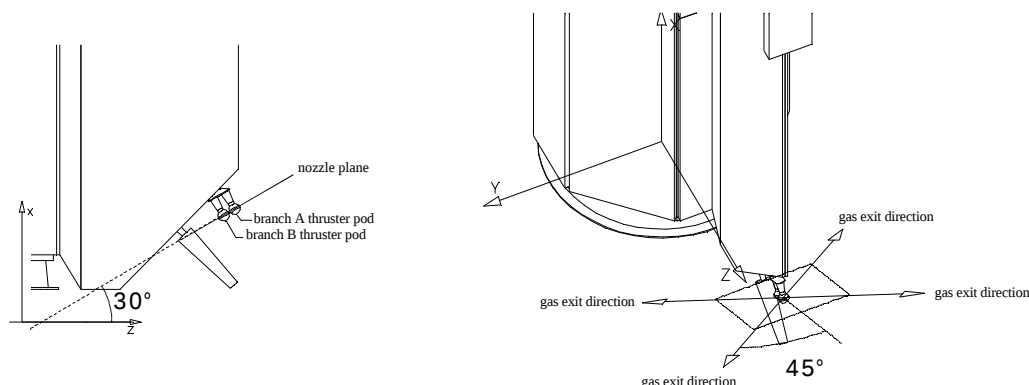
Figure 6.38. Micro-thruster accommodation.
