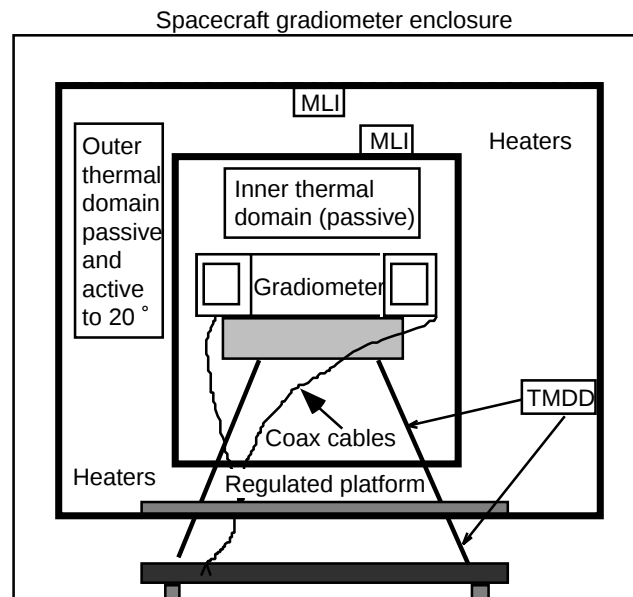
Figure 6.15. Gradiometer thermal concept.
