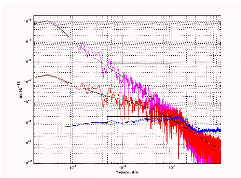
Figure 6.29. Residual attitude ( \text{rad Hz}^{-1/2} ), velocity ( \text{rad s}^{-1} \text{ Hz}^{-1/2} ), and acceleration ( \text{rad s}^{-2} \text{ Hz}^{-1/2} ), on the z-axis. The specified values within the gradiometer measurement bandwidth are indicated by black horizontal lines.
