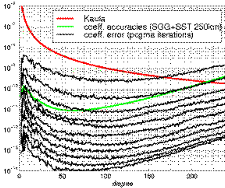
Figure 7.3. Result of a gravity field model recovery experiment complete to degree and order 250 based on a 48-day simulated data set of error-free SGG observations.
