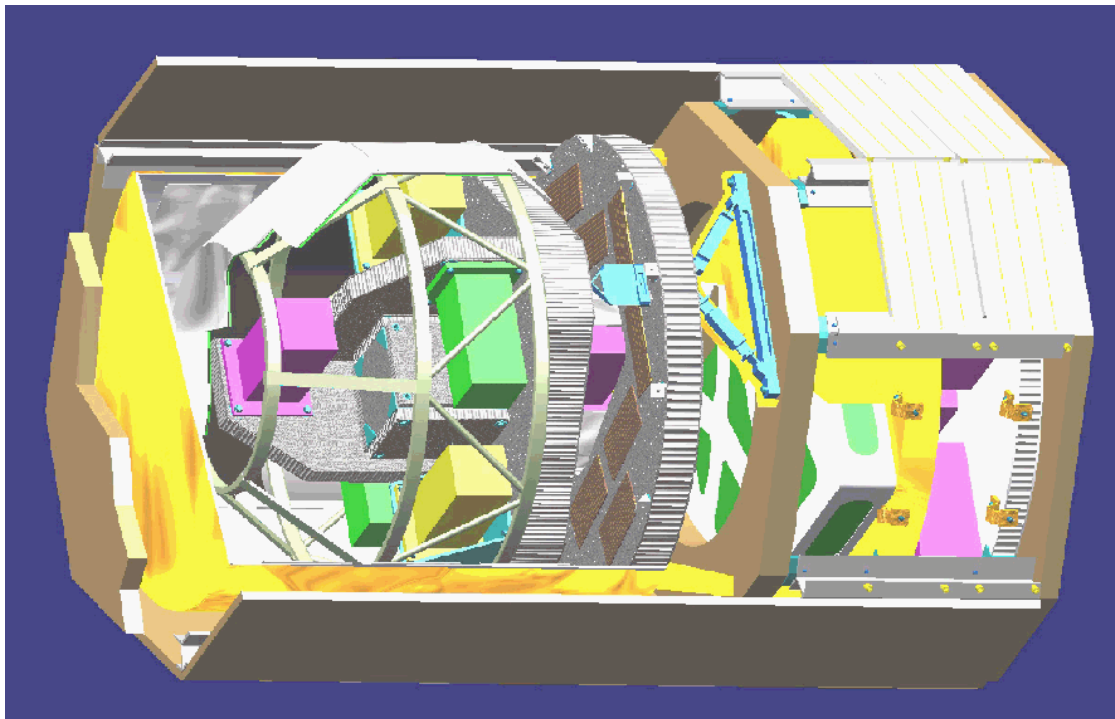
Figure 5.2. Gradiometer assembly.
