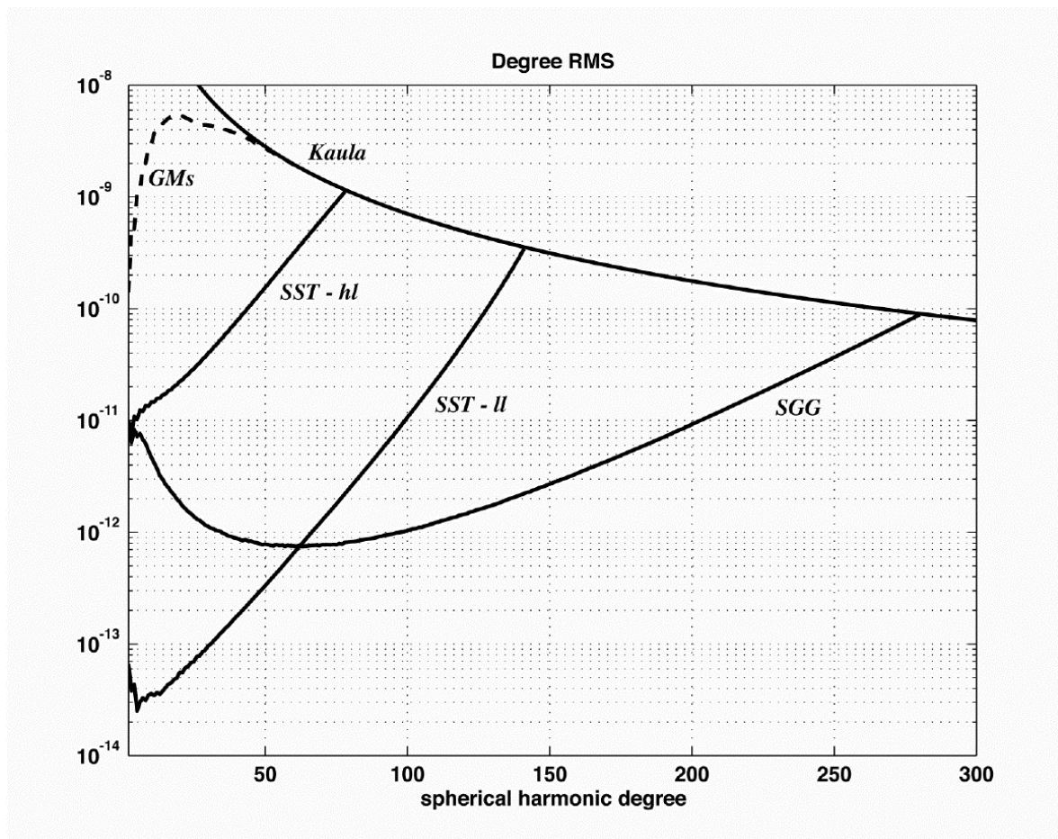
Figure 2.7. Representative error degree variance spectra (see Annex) of the gravity mission concepts SST-hl, SST-ll and satellite gradiometry in comparison with one of the best currently available satellite gravity models (GMs) and with the signal degree variances of the gravity field (Kaula). The high precision of SST-ll at long and medium length scales and the high-spatial-resolution of gradiometry are apparent here.
