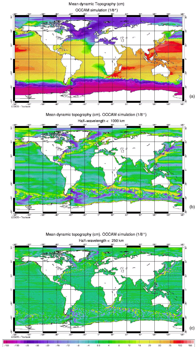
Figure 3.11. (a) Ocean topography over all spatial-scales obtained using the 1/8 -degree-resolution OCCAM global model; (b,c) the same topography but for spatial-scales shorter than 1000 and 250 km half-wavelength, respectively;
