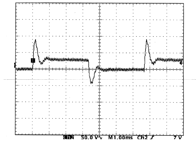
Figure 6.34. Quick step thrust change command. The vertical divisions are 50 V and the horizontal 1 ms.
