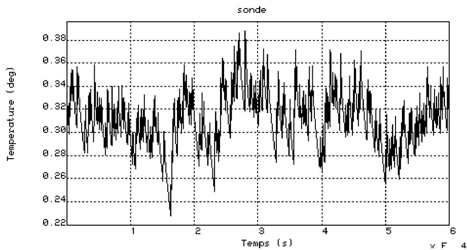
Figure 6.16. Temperature variations on the gradiometer along 60 000 sec.
