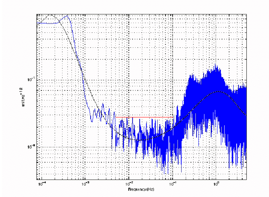
Figure 6.27. Residual acceleration along x as a function of frequency ( \text{ms}^{-2} \text{Hz}^{-1/2} ). The requirement within the gradiometer measurement bandwidth can be seen as a flat line in red.
