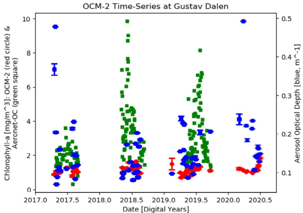
Figure 4-10. Time-series plot of the OCM-2 Chlorophyll-a (and Aerosol Optical Depth from the Level 2C files, and AERONET-OC estimated Chlorophyll-a for the Gustav Dalen Tower; data courtesy of AERONET website/Giuseppe Zibordi.
