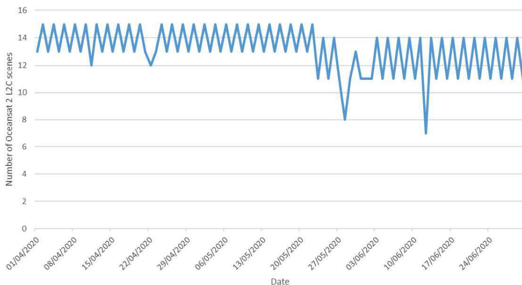
Figure 4-3: Plot showing the number of Oceansat 2 scenes per day.
