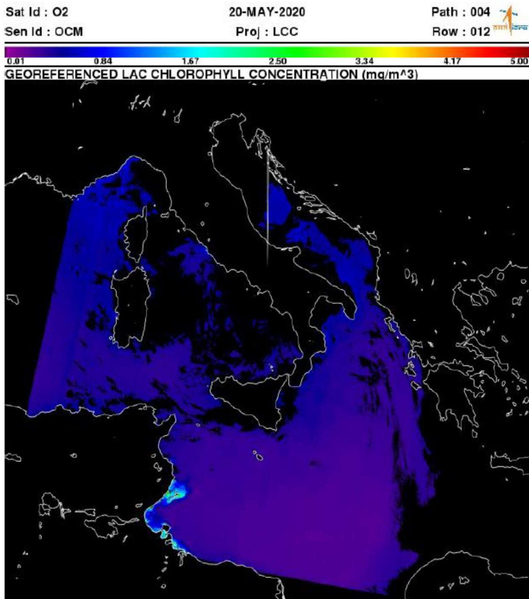
Figure 4-6. A sample of OCM-2 QLs for the 20 May 2020.
