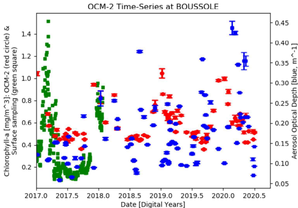
Figure 4-11. Time-series plot of the OCM-2 Chlorophyll-a and Aerosol Optical Depth from the Level 2C files, and surface sampling Chlorophyll-a for BOUSSOLE; data courtesy of BOUSSOLE website 2 .
