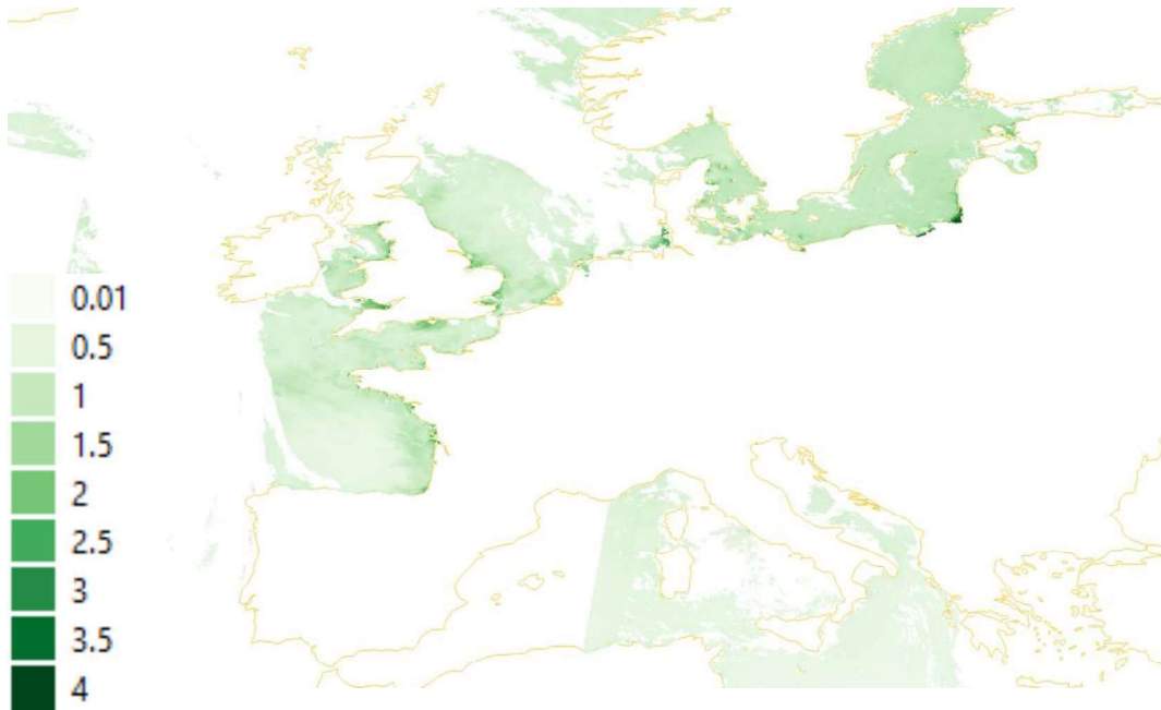
Figure 4-7. A snapshot from QGIS showing the daily Chlorophyll-a (mg/m 3 ) composite using data from 20 May 2020.
