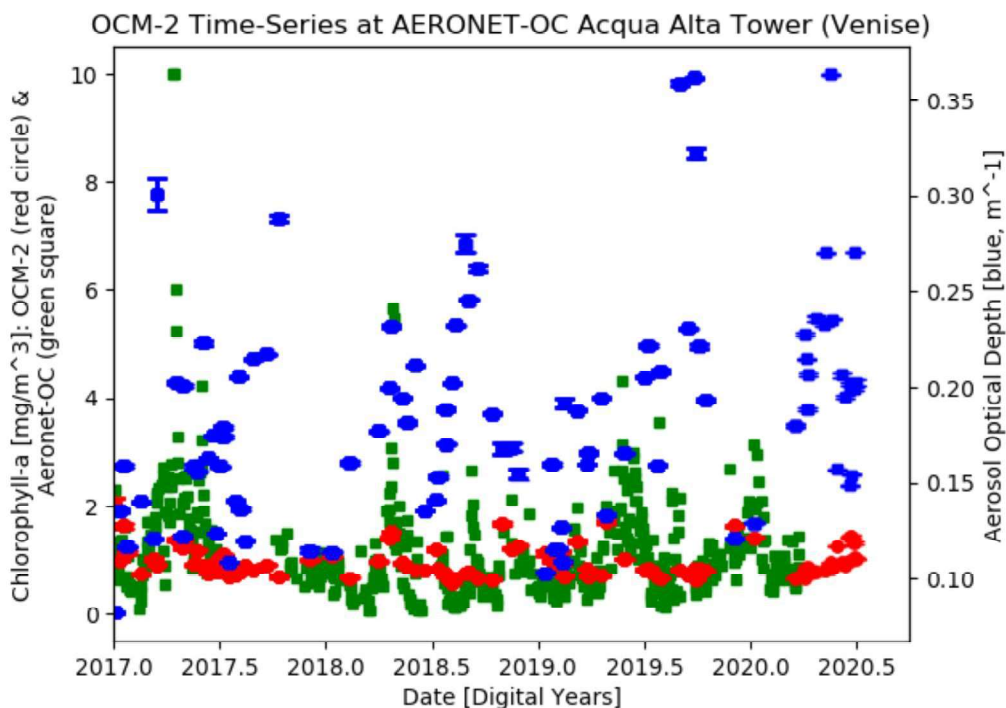
Figure 4-9. Time-series plot of the OCM-2 Chlorophyll-a (clo) and Aerosol Optical Depth (aod) products extracted from the Level 2C files, and AERONET-OC estimated Chlorophyll-a for the location of the AERONET-OC Acqua Alta Oceanographic Tower; data courtesy of AERONET website 1 /Giuseppe Zibordi.
