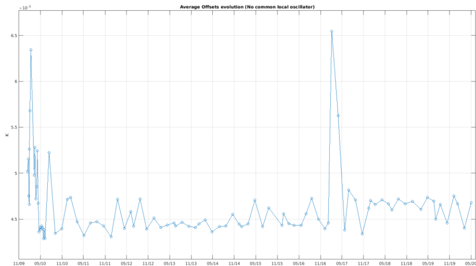
Figure 35 Evolution of the average of the Correlator offsets for the baselines which do not share local oscillator
