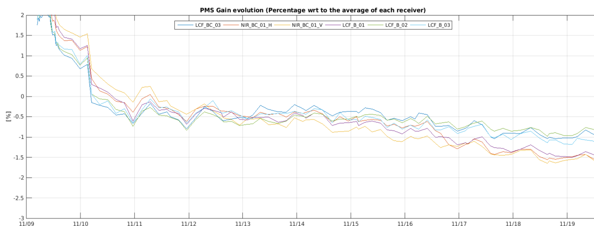
Figure 13 Evolution of the \Delta PMS Gain of the LICEFS in CMN H2
