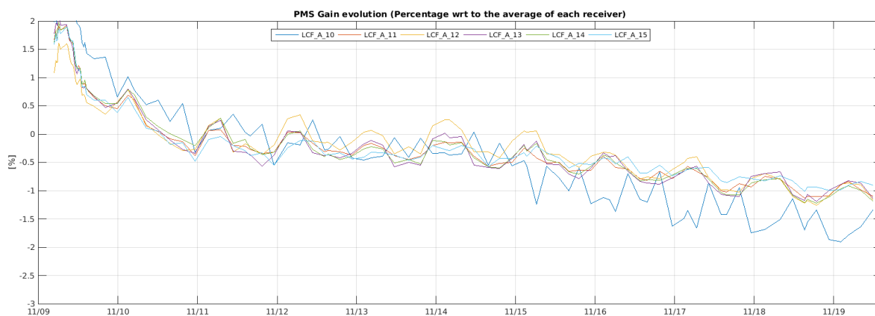
Figure 11 Evolution of the \Delta PMS Gain of the LICEFS in CMN A2
