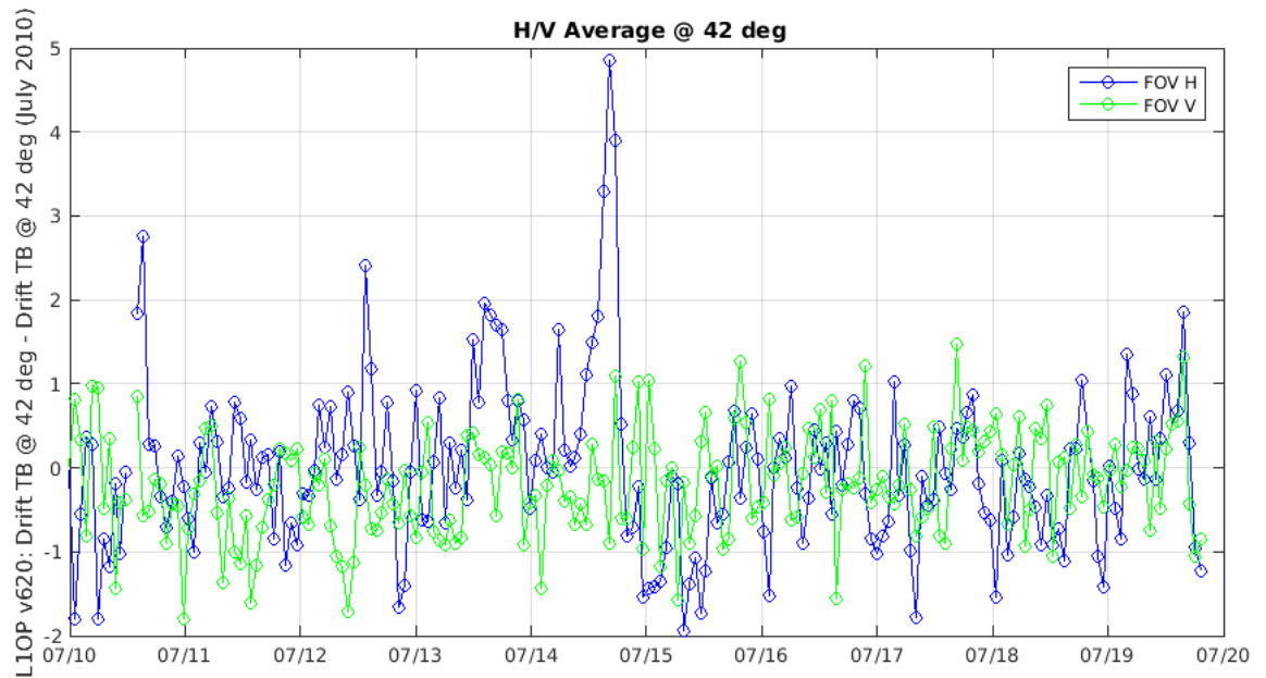
Figure 38: Dome-C H and V polarization trends in Extended Alias Free zone (incidence angle 42°)
