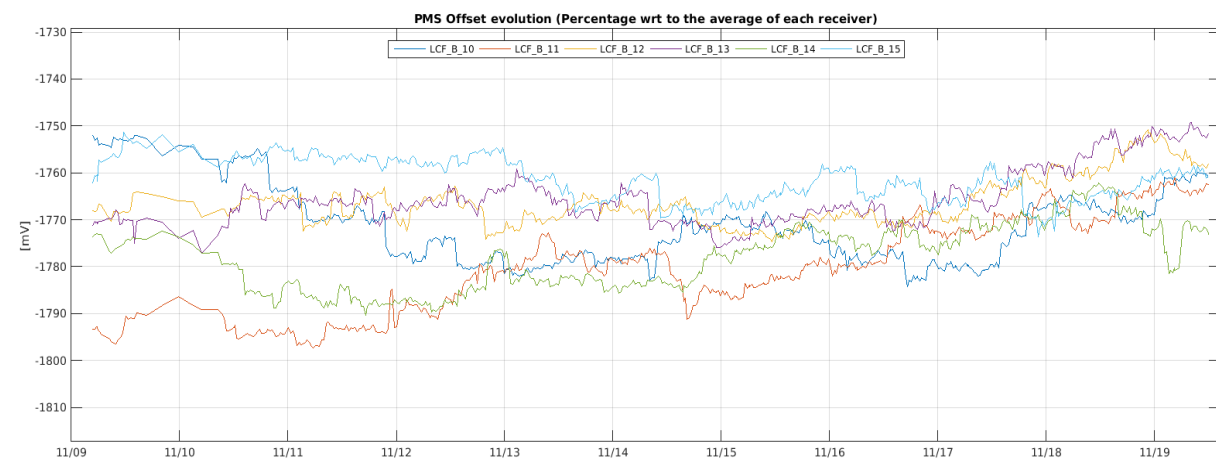
Figure 27 Evolution of the \Delta PMS Offset of the LICEFS in CMN B2
