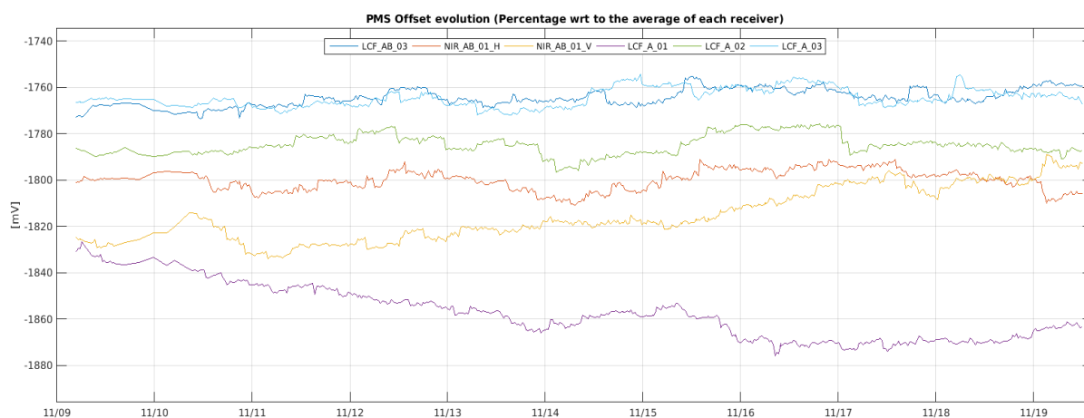
Figure 21 Evolution of the \Delta PMS Offset of the LICEFS in CMN H1
