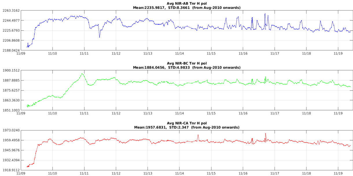
Figure 3 Tnr evolution of NIR AB (blue), NIR BC (green) and NIR CA (red) in the H-channel since the beginning of the mission.
