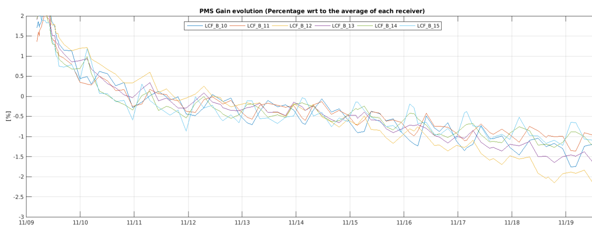
Figure 15 Evolution of the \Delta PMS Gain of the LICEFS in CMN B2
