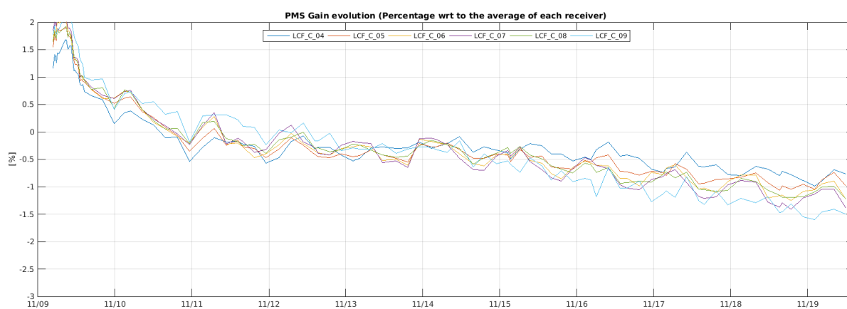
Figure 18 Evolution of the \Delta PMS Gain of the LICEFS in CMN C1
