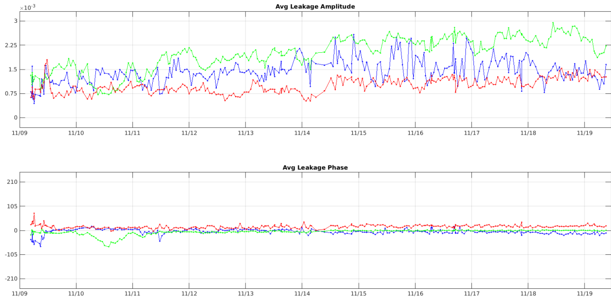
Figure 8 Leakage factor evolution in amplitude and phase of NIR AB (blue), NIR BC (green) and NIR CA (red) since the beginning of the mission
