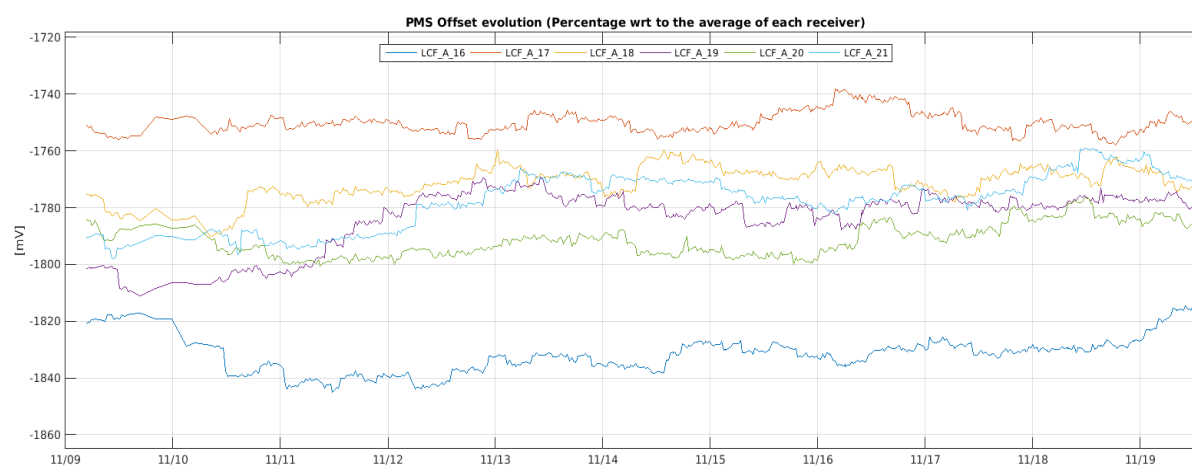
Figure 24 Evolution of the \Delta PMS Offset of the LICEFS in CMN A3
