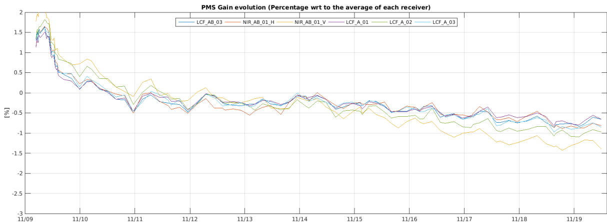
Figure 9 Evolution of the \Delta PMS Gain of the LICEFS in CMN H1
