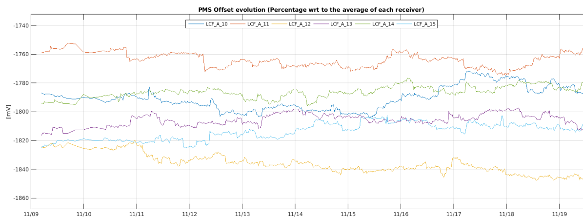
Figure 23 Evolution of the \Delta PMS Offset of the LICEFS in CMN A2
