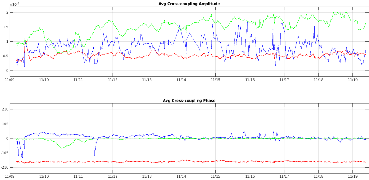
Figure 7 Cross-coupling evolution in amplitude and phase of NIR AB (blue), NIR BC (green) and NIR CA (red) since the beginning of the mission
