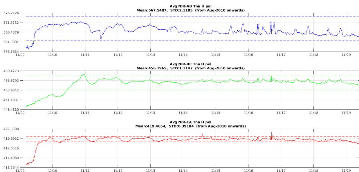
Figure 1 Tna evolution of NIR AB (blue), NIR BC (green) and NIR CA (red) in the H-channel since the beginning of the mission. Thresholds in dashed lines
