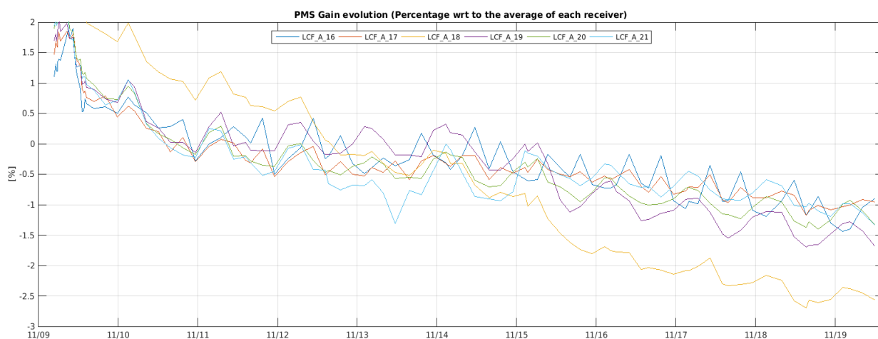
Figure 12 Evolution of the \Delta PMS Gain of the LICEFS in CMN A3
