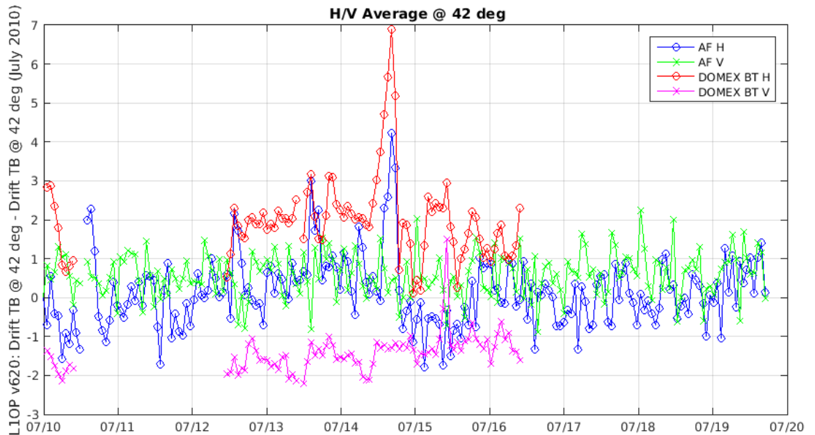
Figure 37: Dome-C H and V polarization trends in Alias Free zone (incidence angle 42°)
