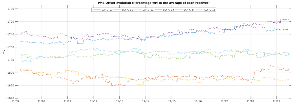
Figure 31 Evolution of the \Delta PMS Offset of the LICEFS in CMN C2
