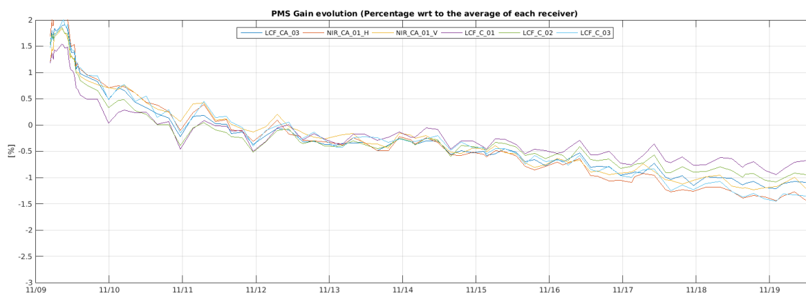
Figure 17 Evolution of the \Delta PMS Gain of the LICEFS in CMN H3
