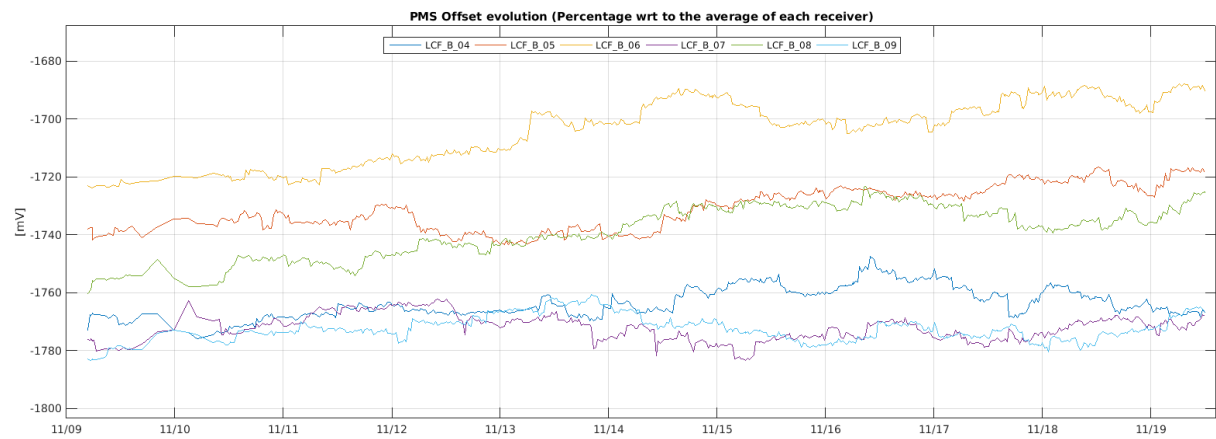
Figure 26 Evolution of the \Delta PMS Offset of the LICEFS in CMN B1
