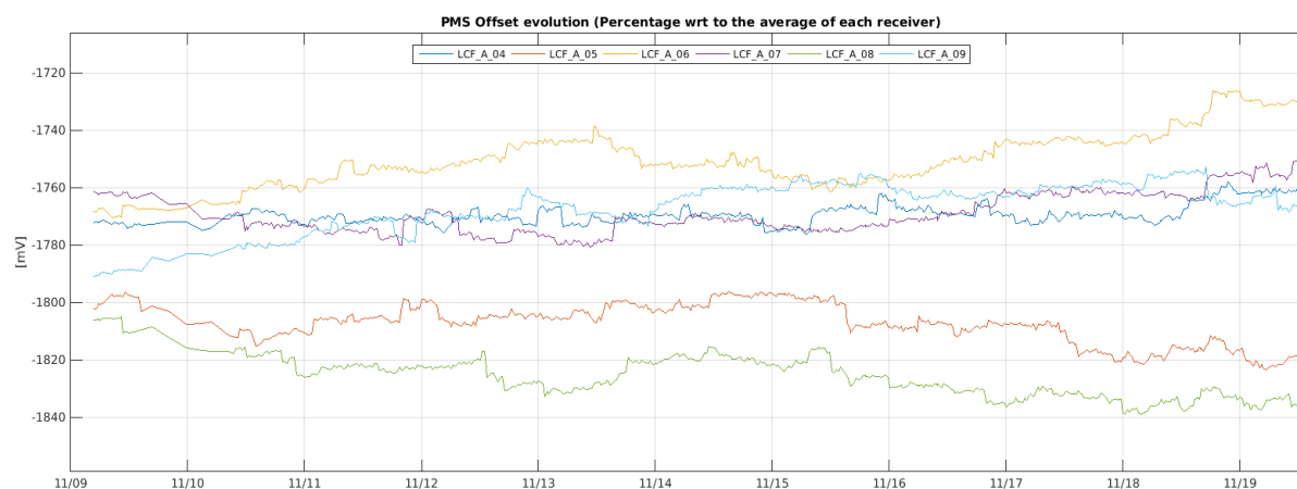
Figure 22 Evolution of the \Delta PMS Offset of the LICEFS in CMN A1
