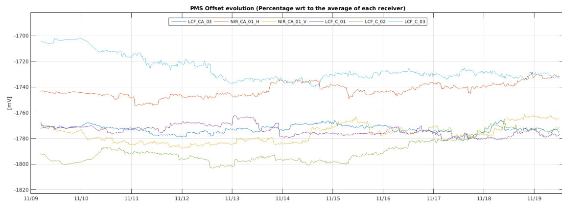
Figure 29 Evolution of the \Delta PMS Offset of the LICEFS in CMN H3
