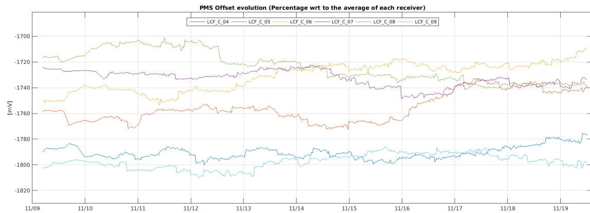
Figure 30 Evolution of the \Delta PMS Offset of the LICEFS in CMN C1
