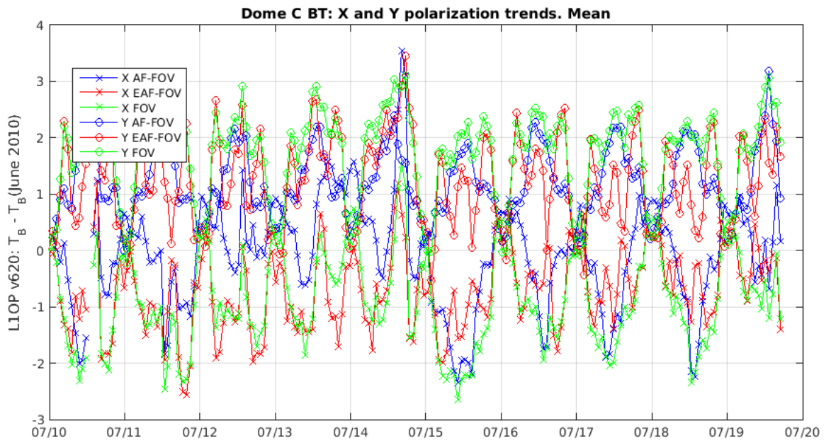
Figure 36: Dome-C X and Y polarization trends (all incidence angles)
