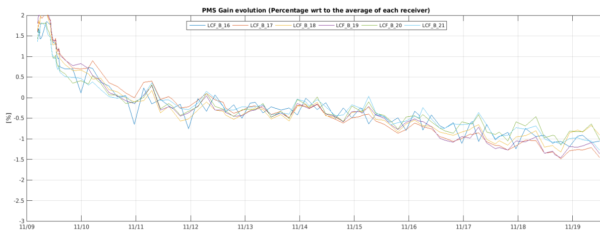
Figure 16 Evolution of the \Delta PMS Gain of the LICEFS in CMN B3
