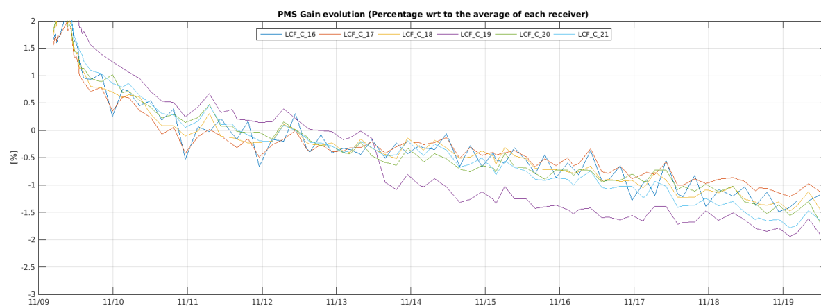
Figure 20 Evolution of the \Delta PMS Gain of the LICEFS in CMN C3
