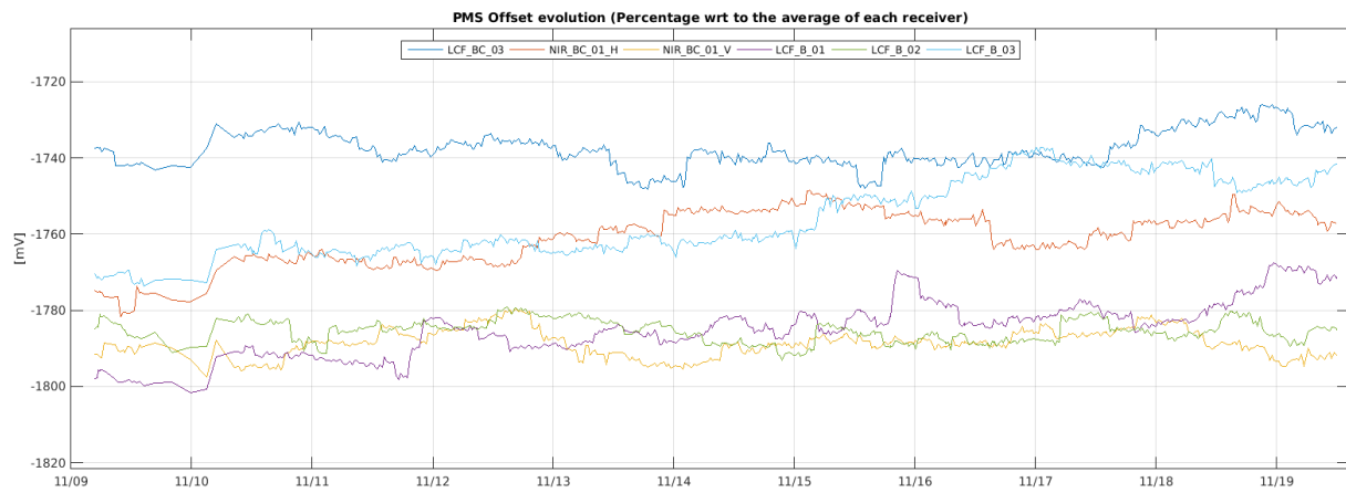
Figure 25 Evolution of the \Delta PMS Offset of the LICEFS in CMN H2
