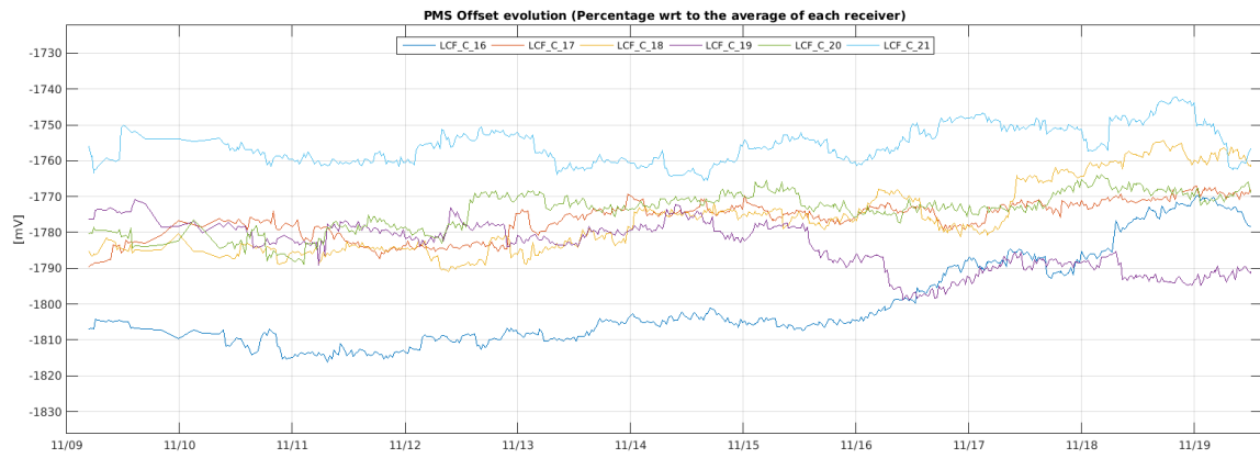
Figure 32 Evolution of the \Delta PMS Offset of the LICEFS in CMN C3
