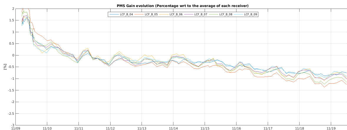
Figure 14 Evolution of the \Delta PMS Gain of the LICEFS in CMN B1
