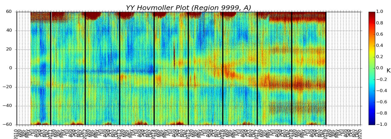
Figure 42: BT stability over the ocean, for YY polarization and Ascending passes.
