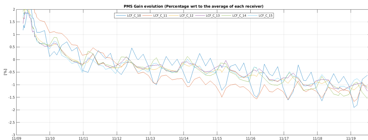
Figure 19 Evolution of the \Delta PMS Gain of the LICEFS in CMN C2
