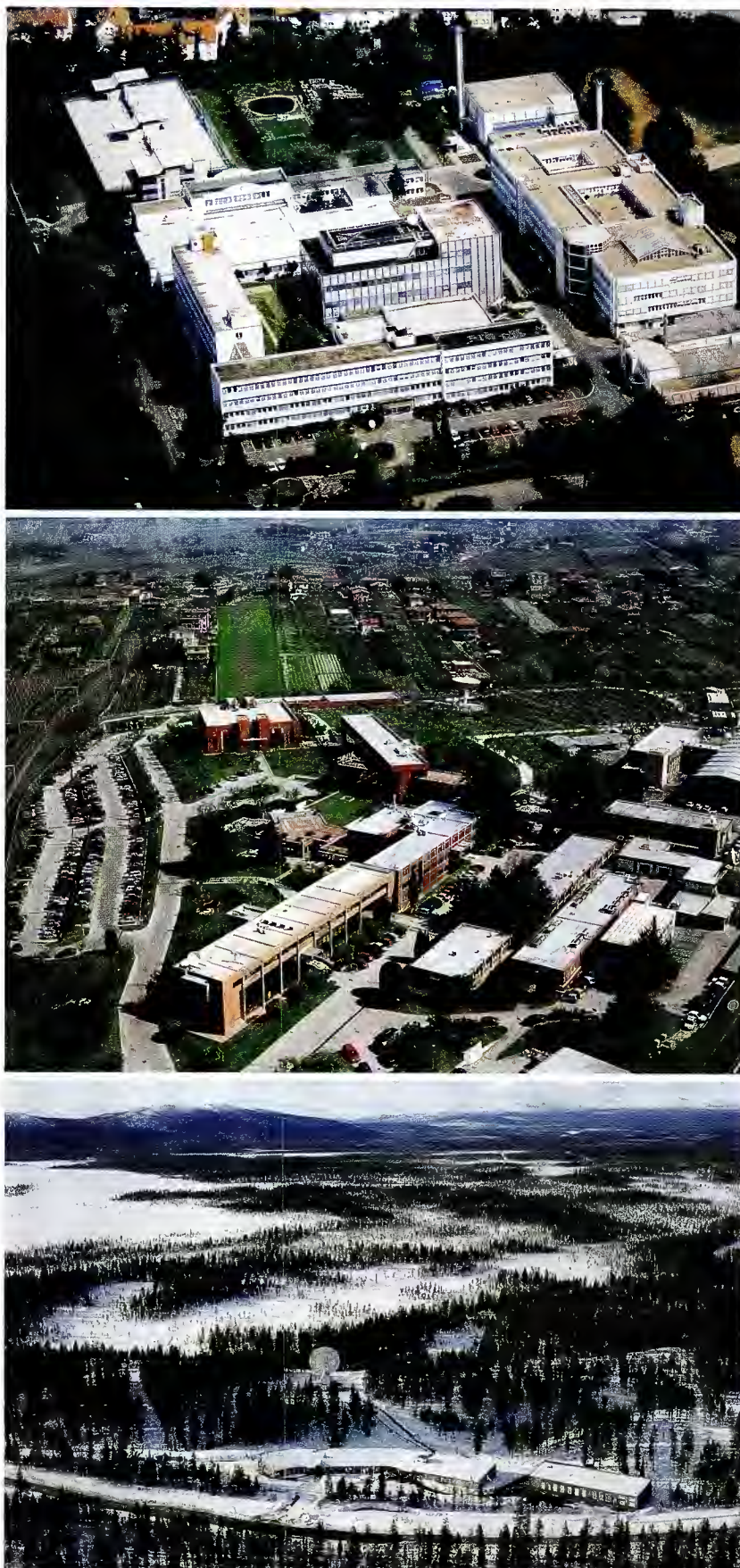
Fig. 2.7 The ESA centres hosting major ENVISAT ground segment facilities with ESOC/Darmstadt ( top ) and ESRIN/Frascati ( middle ). The bottom photograph shows ESA's S-band and X-band station at Kiruna-Salmijärvi (Photos: ESA, S. Corvaja).
