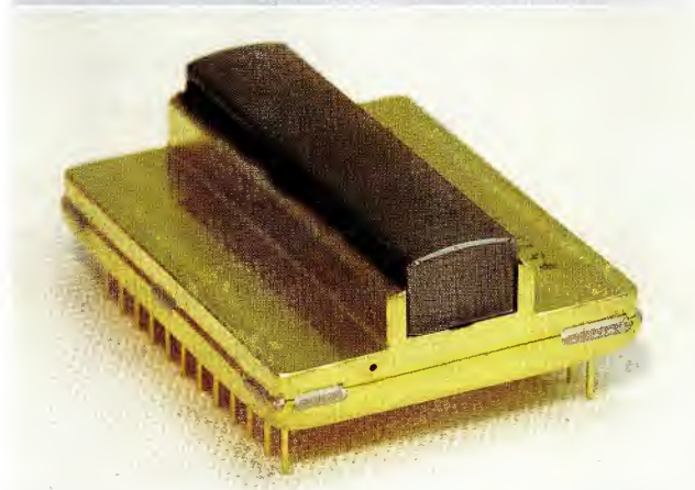
Fig. 3.11 The RETICON ( top ) and EPITAXX ( bottom ) linear detector arrays (Photo: SRON).
