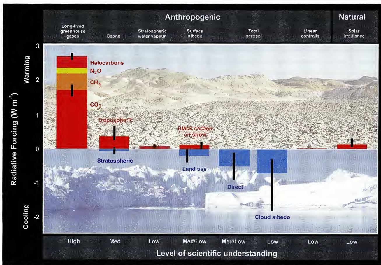
Fig. 1.5 Global, annual mean radiative forcings ( \text{W m}^{-2} ) due to a number of agents for the period from pre-industrial (1750) to present (2005). The height of each box denotes a central or best estimate value. The vertical bars visualise an estimate of the uncertainty range, for the most part guided by the spread in the published values of the forcing. A 'level of scientific understanding' index is associated to each forcing, with high, medium and low levels, respectively (Courtesy: adapted from IPCC 2007).
