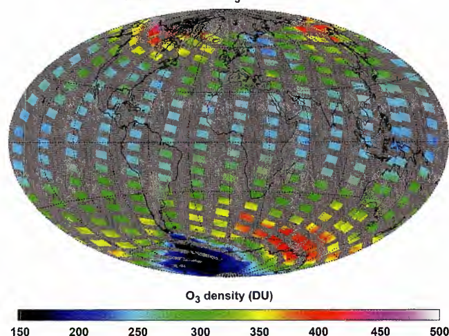
Fig. 7.6 One day of total ozone densities obtained with the TOSOMI algorithm (Courtesy: KNMI/ESA).
