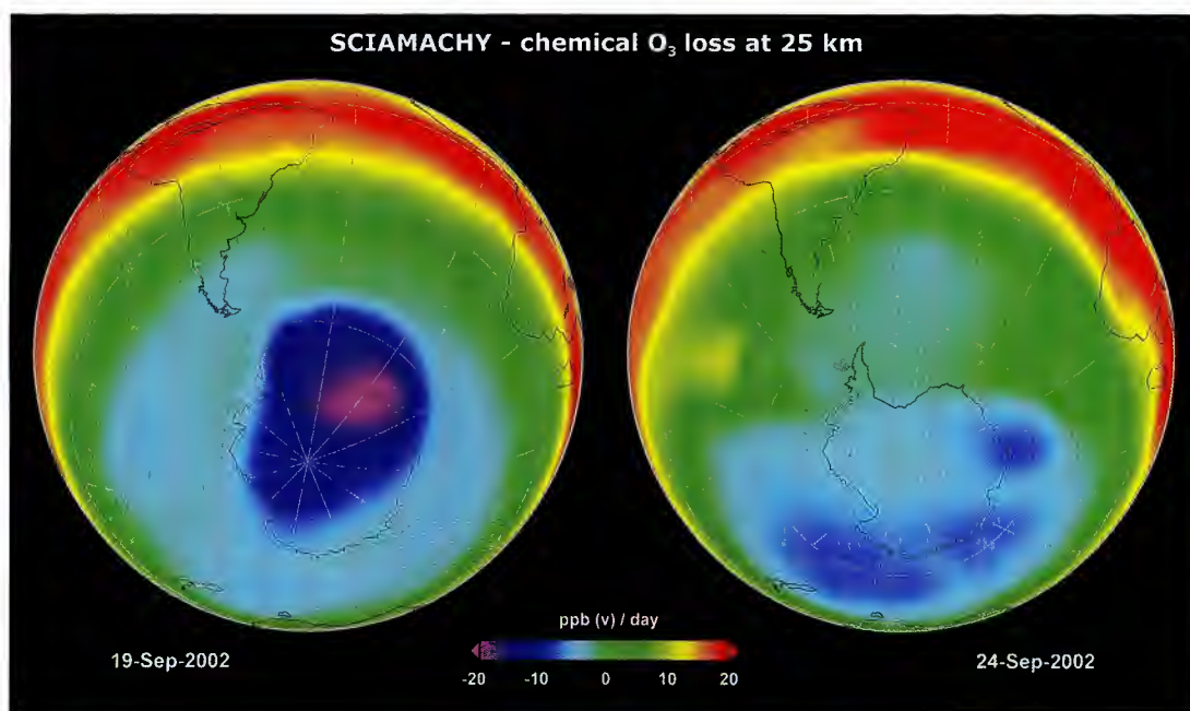
Fig. 10.21 Chemical ozone loss rates on two days in September 2002 in the mid-stratosphere at about 25 km, relative to the previous day. While on 19 September the ozone hole was still developing its usual shape, 5 days later the split-up of the vortex has reduced ozone loss rates (Courtesy: T. Erbertseder, DLR-DFD).
