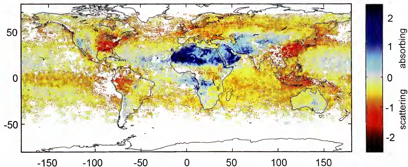
Fig. 7.12 Seasonal average of SCIAMACHY UV Aerosol Index for July–September, 2005. Blue indicates absorbing aerosols (mineral dust, biomass burning smoke); red/orange indicates weakly absorbing but scattering aerosols (sulphate and secondary organic aerosols) and remaining clouds. Only pixels with cloud fraction smaller than 5% are included in the average (Courtesy: M. Penning de Vries; MPI for Chemistry, Mainz).
