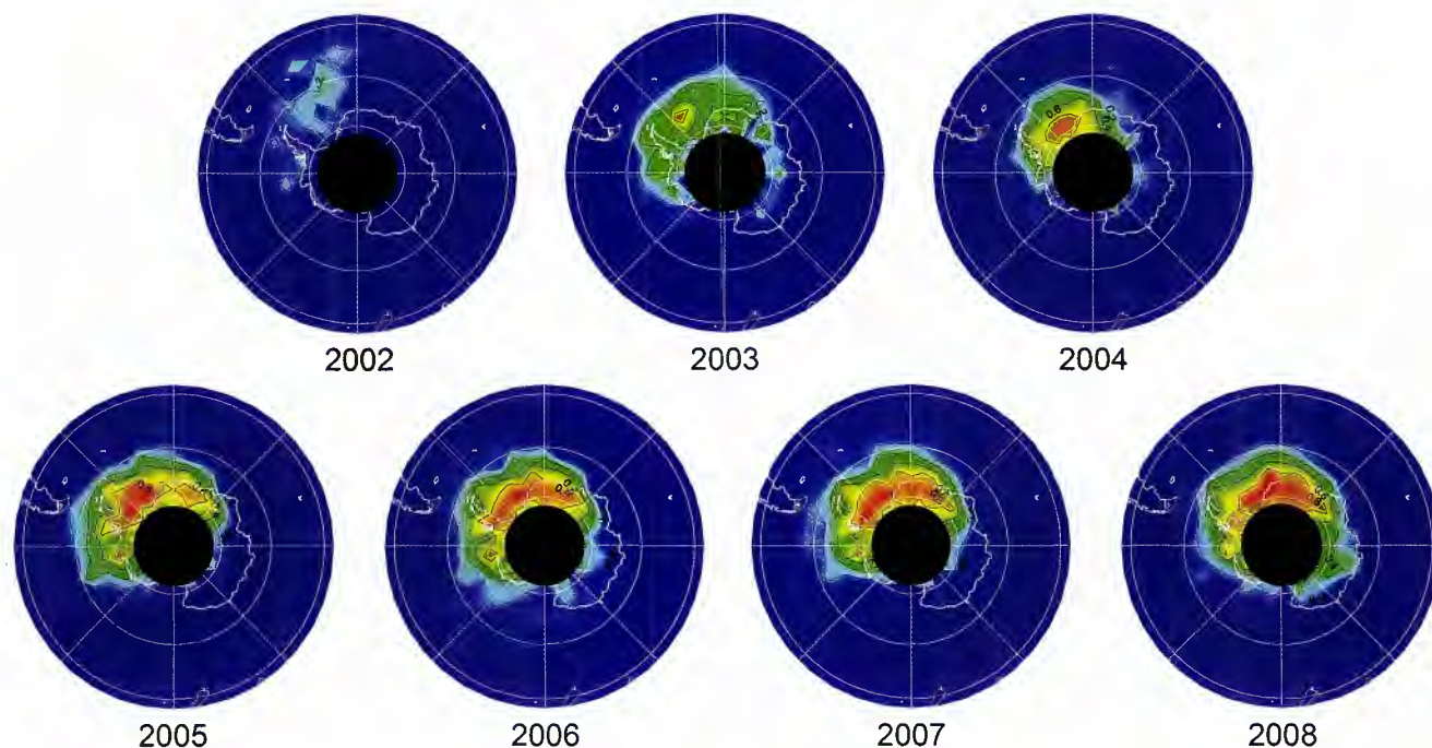
Fig. 10.29 Maps of PSC occurrence rates for September of the years 2002–2008. Contours levels correspond to 0.2, 0.4, 0.6, and 0.8. Red areas indicate occurrence rates exceeding 0.8 (Courtesy: C. von Savigny, IUP-IFE, University of Bremen).
