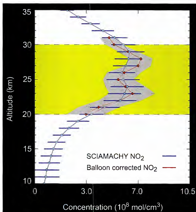
Fig. 9.17 Comparison between a SCIAMACHY NO 2 profile ( blue ) retrieved with the SCIATRAN V3.1 algorithm and co-located balloon NO 2 measurements at Kiruna ( red ). The grey shaded area shows the uncertainty of the balloon measurements, whereas the yellow region indicates the altitude range where both instruments are considered to probe similar air masses (Courtesy: R. Bauer IUP-IFE, University of Bremen).
