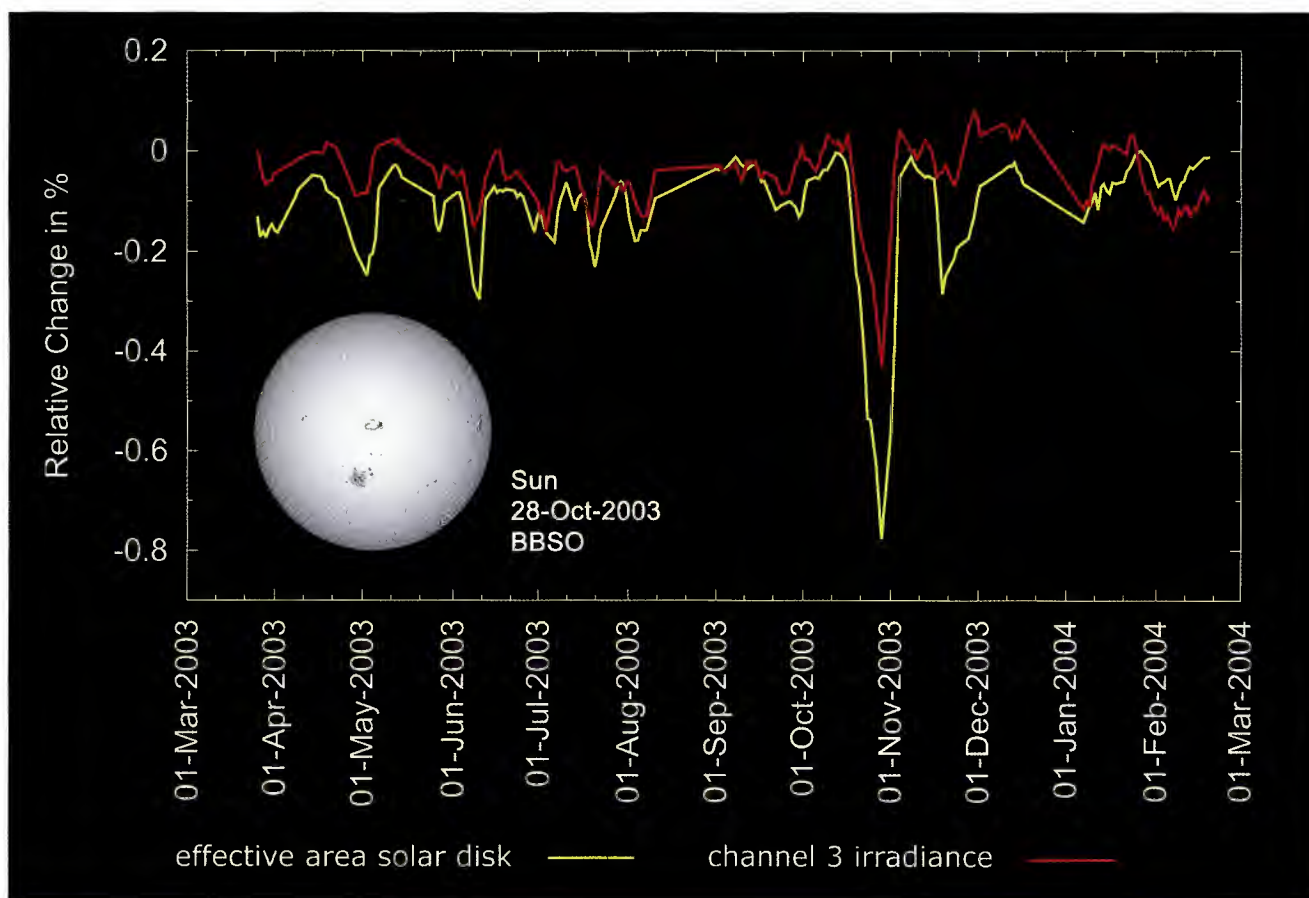
Fig. 6.3 Measured irradiance in channel 3 (red) and effective solardisk area (yellow) between March 2003 and March 2004. The large sunspots at the end of October caused a significantly reduced irradiance. The inset shows the active solar disk in white light on 28 October 2003 (Courtesy: IUP-IFE, University of Bremen; Sun photo: Big Bear Solar Observatory).
