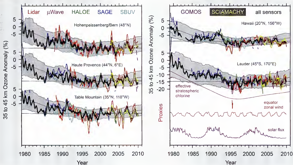
Fig. 10.25 Ozone anomalies from 1979 to 2009 derived from different datasets at five NDACC stations. The anomalies are averaged over the 35–45 km range. The all-instrument average is shown in black. All time series were smoothed by a 5-month running mean. At the bottom of the right hand panel three proxies are given: The negative 10 hPa zonal wind at the equator for the QBO, the 10.7 cm solar flux for the 11-year solar cycle and the inverted effective stratospheric chlorine for ozone destruction by chlorine. The grey line and the grey shaded area are showing model simulations and their 2-sigma standard deviation. (Courtesy: adapted from Steinbrecht et al. 2009. Reproduced/modified by permission of American Geophysical Union).
