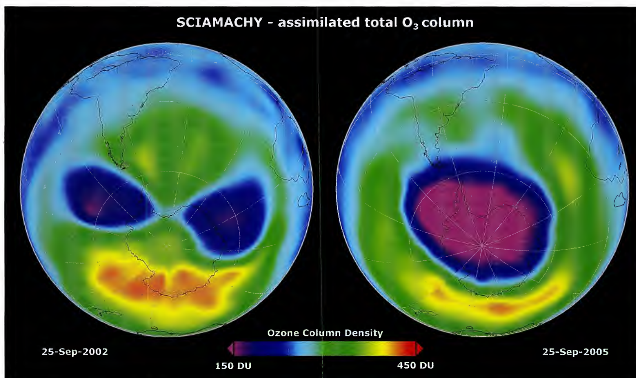
Fig. 10.19 The Antarctic ozone hole in 2002 ( left ) and 2005 ( right ). SCIAMACHY total column ozone measurements from 25 September have been analysed with the ROSE assimilation model to generate this view. Due to meteorological conditions the hole was split and reduced in size in 2002 but appeared 'as normal' in 2005 (Courtesy: T. Erbertseder, DLR-DFD).
