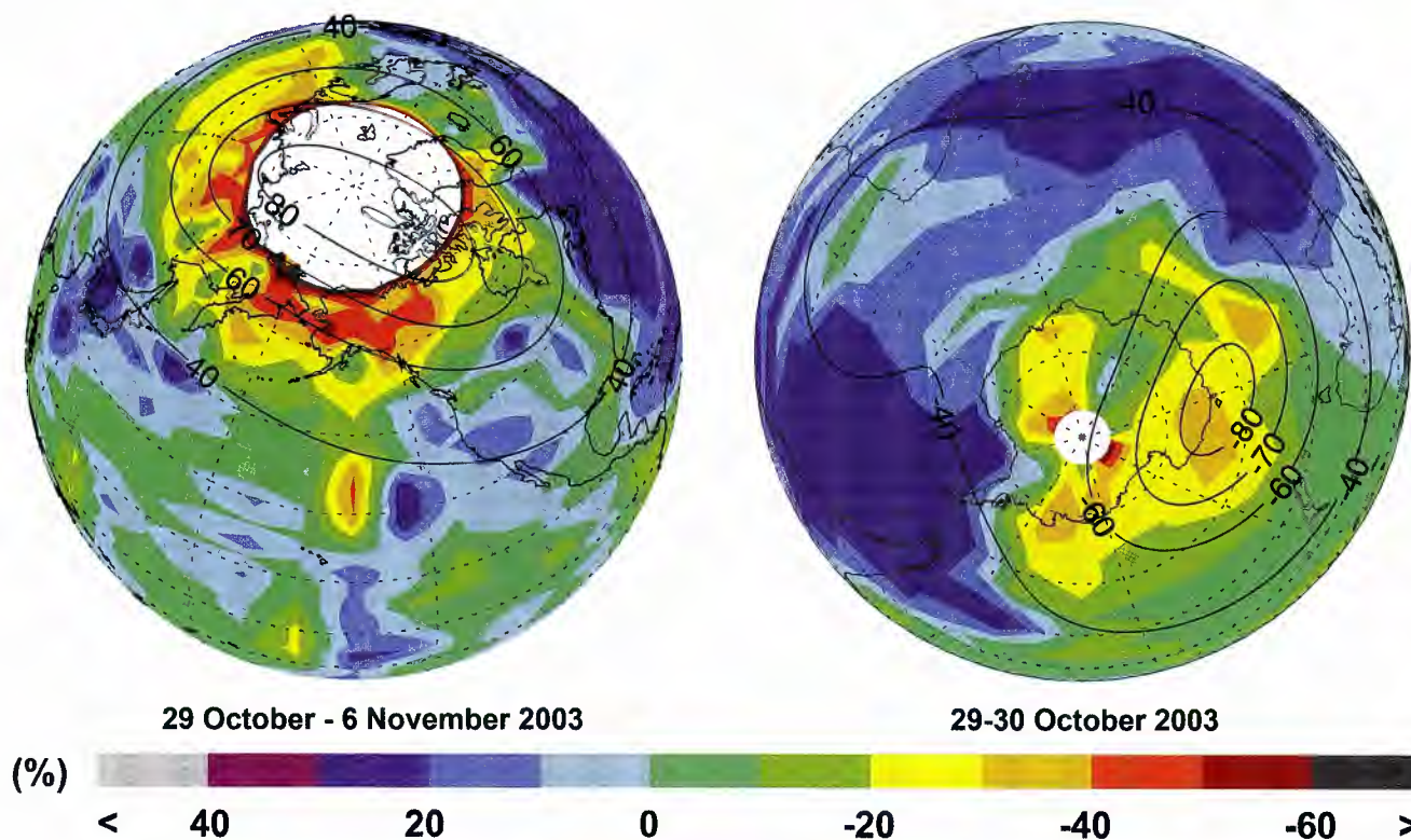
Fig. 10.33 Measured change of ozone concentration at 49 km altitude due to the strong solar proton events end of October 2003 in the northern and southern hemisphere relative to the reference period of 20–24 October 2003. White areas depict regions with no observations. The black solid lines are the Earth's magnetic latitudes at 60 km altitude for 2003 (Courtesy: Rohen et al. 2005).
