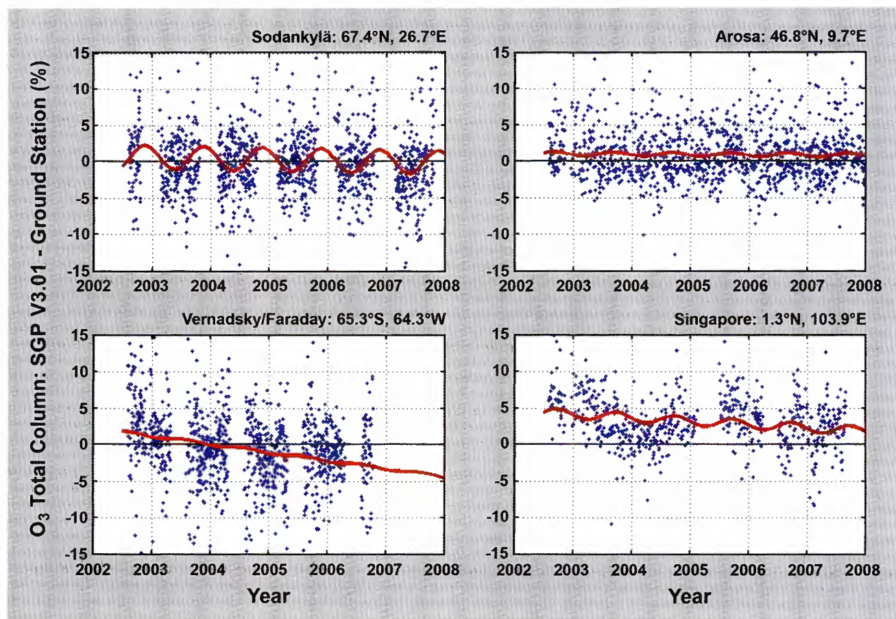
Fig. 9.10 The difference between total O_3 columns retrieved from SCIAMACHY and selected ground stations for the years 2002–2008. The red curve indicates seasonal variability and long-term trends obvious in the comparison. The trends range between -0.15\% and -1.1\% per year (Courtesy: adapted from Lerot et al. 2009).
