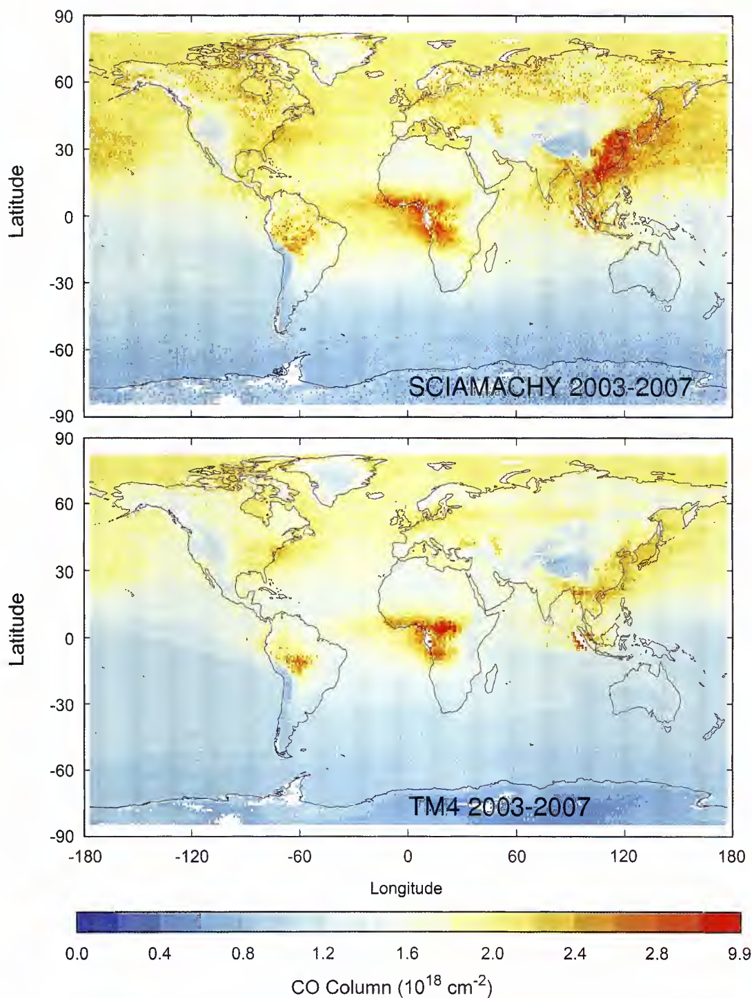
Fig. 10.15 Five year (2003–2007) average CO total columns on a 1^\circ \times 1^\circ grid as retrieved by SCIAMACHY ( top ) and the TM4 chemistry-transport model ( bottom ). The SCIAMACHY CO columns above low clouds over sea are filled up with TM4 CO densities below the cloud to obtain total columns (Courtesy: Gloudemans et al. 2009).
