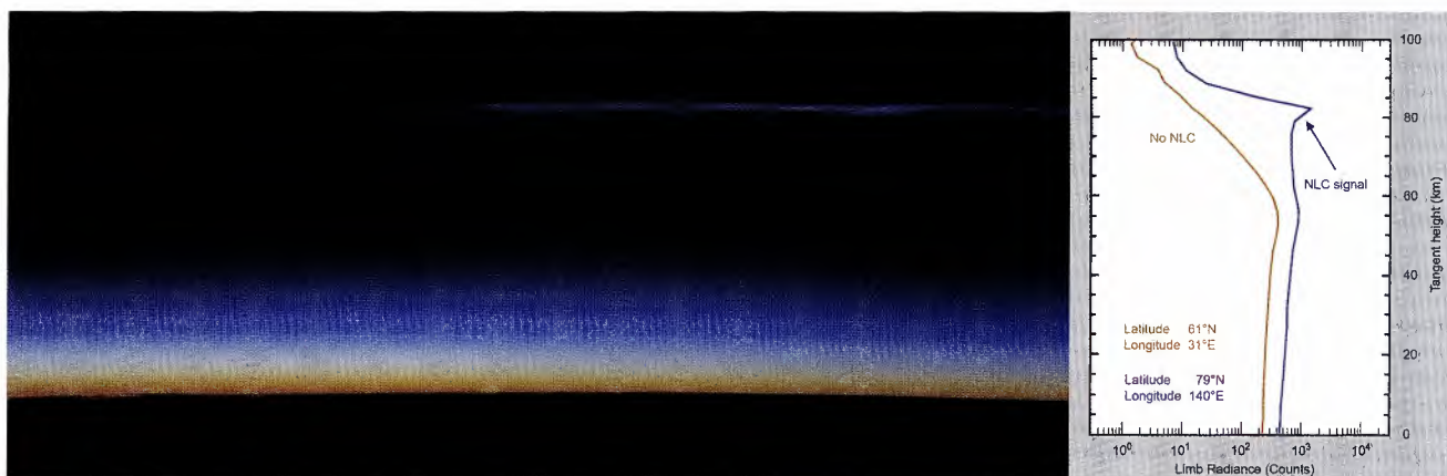
Fig. 10.30 NLC as seen from the International Space Station on 22 July 2008 (left panel) together with the NLC signature in a SCIAMACHY UV limb radiance profile from 3 July 2002 (right panel). The scattering by ice particles in the NLC leads to a significant increase of the observed limb radiance profile peaking at the characteristic NLC altitude of about 83–85 km (blue line). Shown in red is for comparison a limb radiance measurement without NLC being present (Courtesy: C. von Savigny, IUP-IFE, University of Bremen; ISS photo: NASA).
