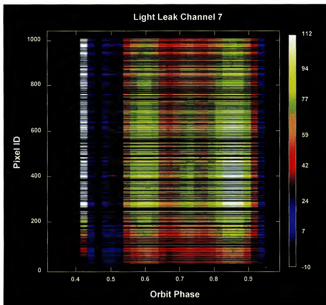
Fig. 6.10 Mean light leak signal for all pixels in channel 7 as a function of orbit phase. The x-axis shows the orbit phase (eclipse corresponds to phase 0.95–0.40, sunrise occurs at phase 0.41), the y-axis the pixel number in channel 7. The colours indicate the size of the light leak signal in BU/s (Courtesy: DLR-IMF/SRON).
