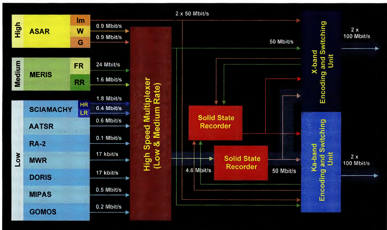
Fig. 2.5 Schematic view of the ENVISAT on-board data handling. SCIAMACHY shares HSM resources with the other instruments generating low rate data. Full orbit data of the Global Mission is stored on one of the solid state recorders and then disseminated to ground via X-band or Ka-band (Courtesy: DLR-IMF).
