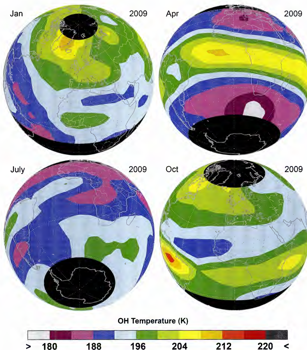
Fig. 10.34 Monthly averaged SCIAMACHY retrievals of OH rotational temperatures at about 87 km for January, April, July and October 2009 (Courtesy: K.-U. Eichmann, IUP-IFE, University of Bremen).
