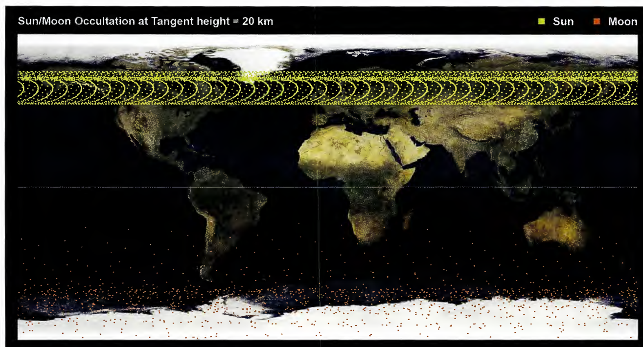
Fig. 4.4 Tangent point geolocation at an altitude of 20 km for all solar and lunar occultation measurements in the year 2009 (Courtesy: DLR-IMF/SRON).
