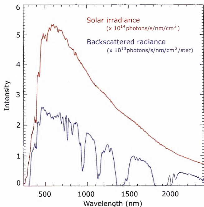
Fig. 7.2 The solar irradiance spectrum (red) and Earth radiance spectrum (blue) with a shape modified by absorption of trace gases and scattering in the atmosphere (Courtesy: IUP-IFE, University of Bremen).
