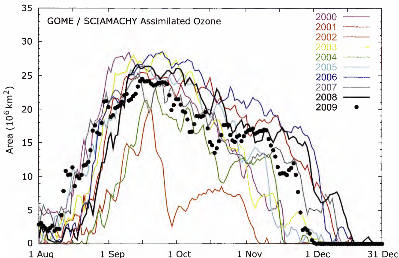
Fig. 10.22 Time series of the size of the Antarctic ozone hole from 2000–2009 based on observations of GOME and SCIAMACHY. The area includes ozone column values below 30^\circ\text{S} lower than 220 Dobson Units (Courtesy: TEMIS KNMI/ESA).
