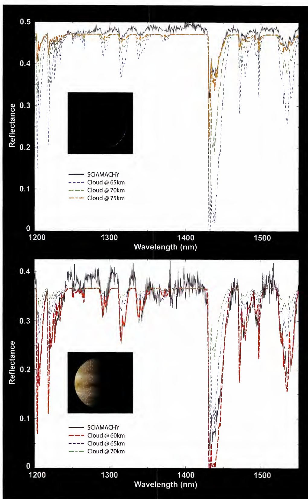
Fig. 10.42 Venus reflectance from 1200 to 1550 nm as measured in March ( top ) and June ( bottom ) 2009. Most absorption features are due to CO 2 . The spectra are modelled by using CO 2 as absorber and H 2 SO 4 clouds at different altitudes as scatterer. The illumination conditions in the insets have been derived from the NASA/JPL Solar System Simulator (Courtesy: M. Vasquez, DLR-IMF).
