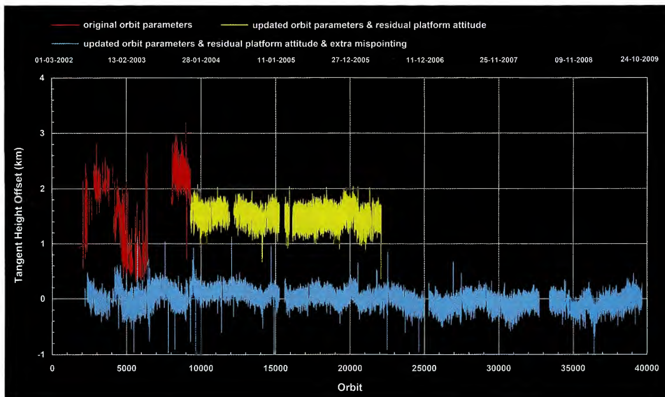
Fig. 6.16 Tangent height offsets as determined from operational data products and TRUE retrieved profile information. Prior to December 2003 the bias had a strong harmonic variation ( red ). After the update of the on-board propagator model and including residual platform mispointing the variation was reduced but a constant offset persisted ( yellow ). When the extra mispointing is introduced in geolocation retrieval this offset vanishes ( blue ) (Courtesy: IUP-IFE, University of Bremen).
