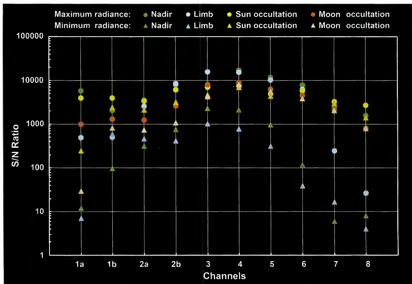
Fig. 3.12 The signal-to-noise ratios for all channels as obtained during OPTEC-5 tests. The ratios were determined for minimum and maximum radiance signals (Courtesy: DLR-IMF).
