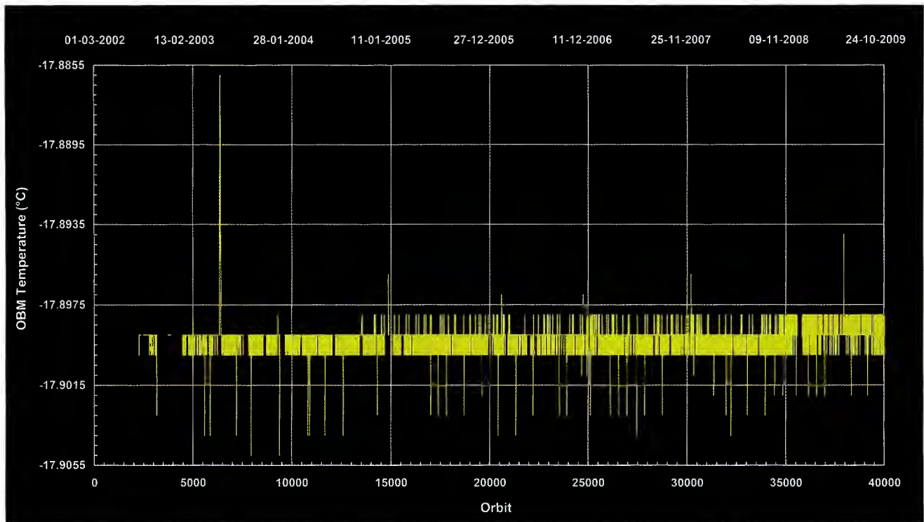
Fig. 6.12 Mean OBM temperature per orbit. On orbit average, the ATC system keeps the OBM within 0.001°C of the selected temperature (Courtesy: DLR-IMF).
