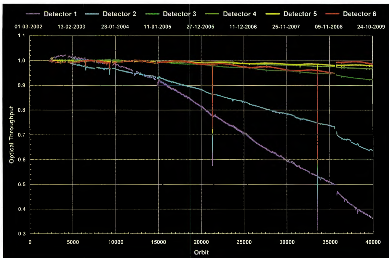
Fig. 6.5 Seven years of optical throughput for channels 1–6 starting with quasi-routine measurements on 2 August 2002. Decontamination intervals and periods after instrument saving are omitted. The information has been derived from the operational light path monitoring using the Sun via the ASM and ESM mirror. The two strong temporal reductions just before orbit 22000 and 34000 are caused by total solar eclipses (Courtesy: IUP-IFE, University of Bremen).
