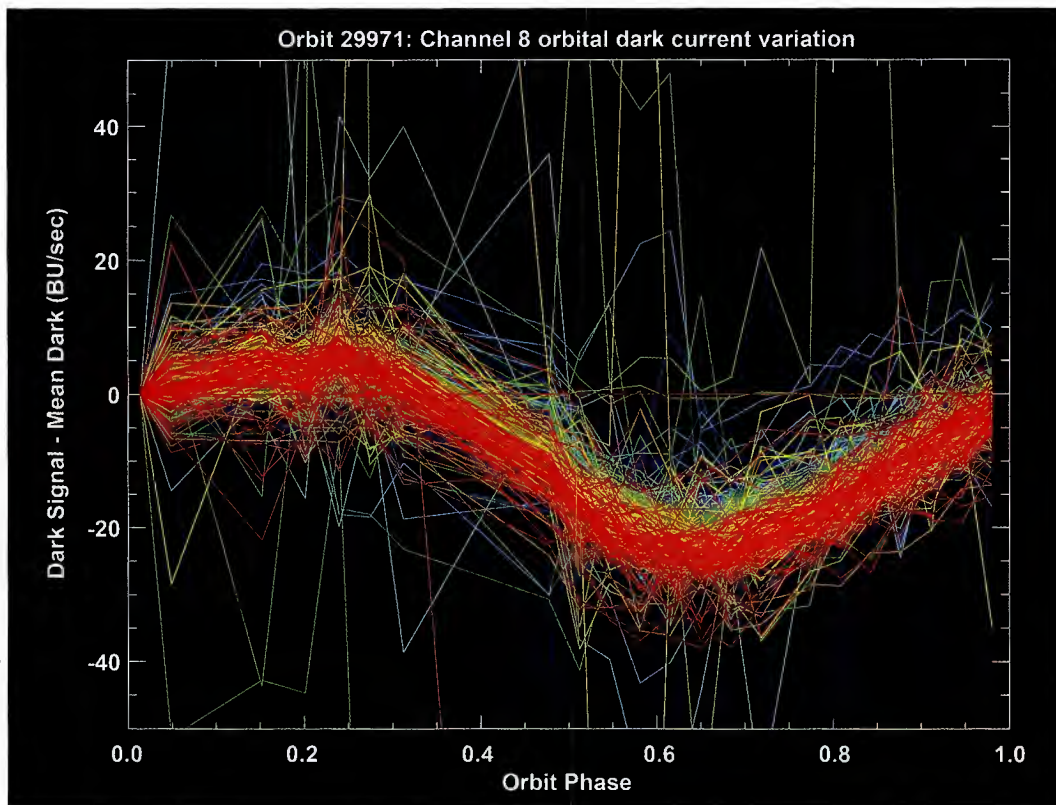
Fig. 8.4 Orbital variation of the thermally induced dark signal for each pixel in channel 8. Orbit phase = 0 corresponds to eclipse entry. The Mean Dark is the dark signal per pixel averaged over a complete dark current state close to phase 0. It permits to normalise the orbital variation at phase 0 (Courtesy: DLR-IMF).
