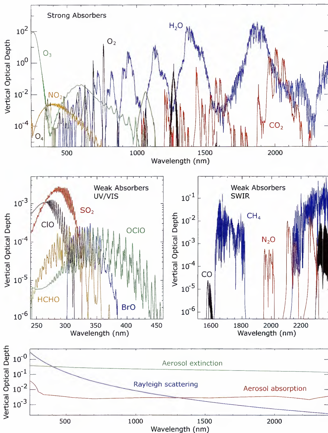
Fig. 7.3 Simulated vertical optical depth of the targeted constituents for 55°N around 10 a.m. The strong absorbers are plotted in the upper part and the relevant weak absorbers in the middle part. In the lower part the vertical optical depth due to Rayleigh scattering, aerosol extinction and absorption is given. Note the large dynamic range of the differential absorption structures used for retrieval of the constituents (Courtesy: IUP-IFE, University of Bremen).
