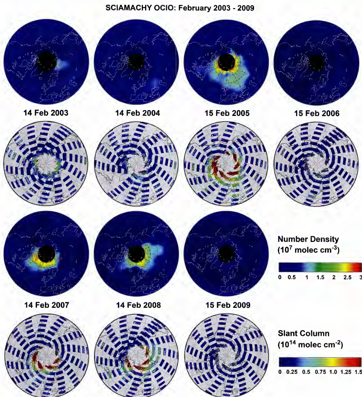
Fig. 10.27 OCIO number density at 19 km altitude above the northern hemisphere derived from SCIAMACHY limb observations (rows 1 and 3) and the corresponding total OCIO slant column derived from nadir views (rows 2 and 4) for mid of February in the Arctic winters 2002/2003–2008/2009 (Courtesy: S. Kühl; MPI for Chemistry, Mainz).
