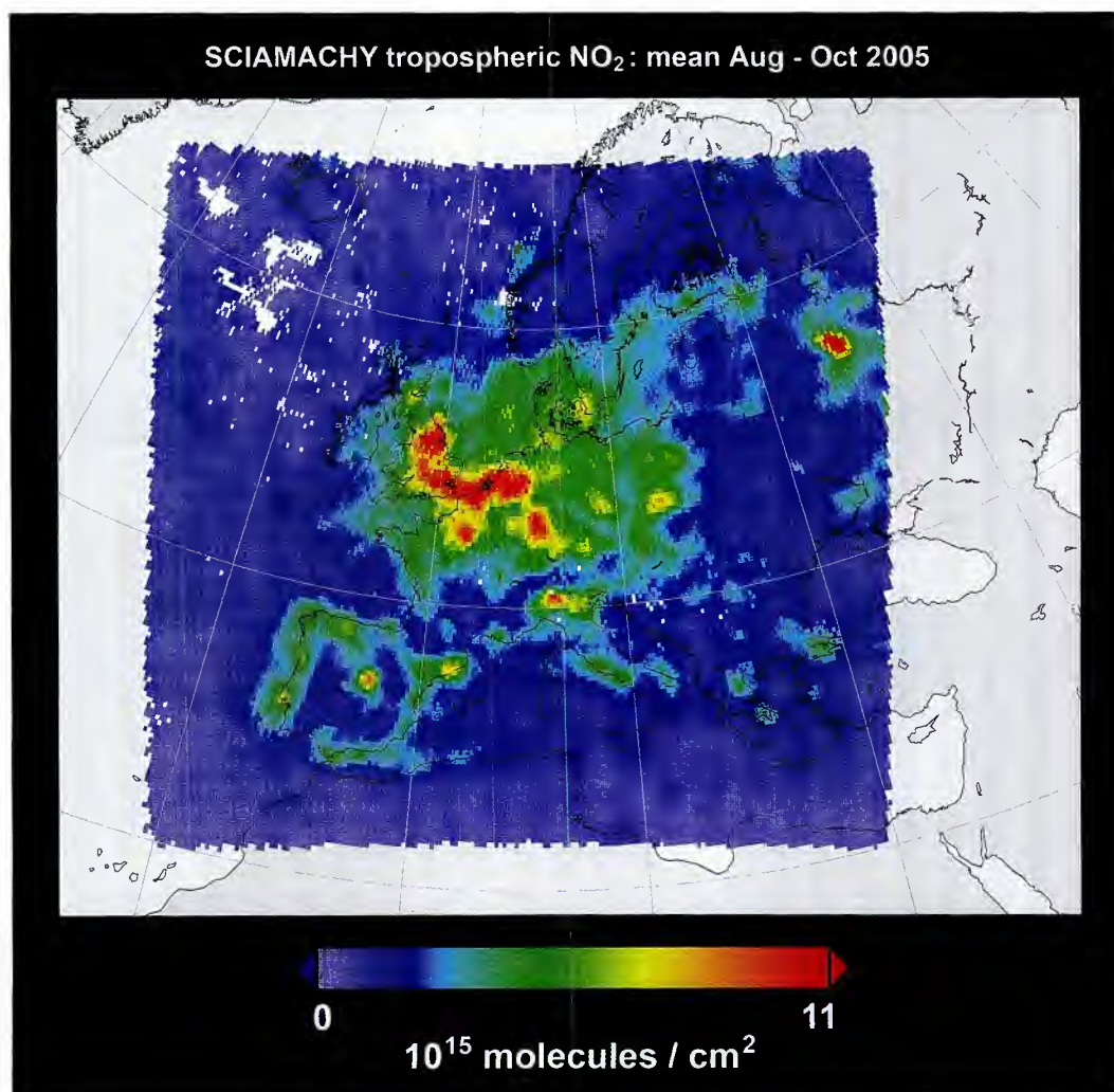
Fig. 7.17 Mean tropospheric \text{NO}_2 vertical column densities over Europe as derived from SCIAMACHY for August to October 2005 with the DLR-DFD assimilation approach (Courtesy: T. Erbertseder, DLR-DFD).
