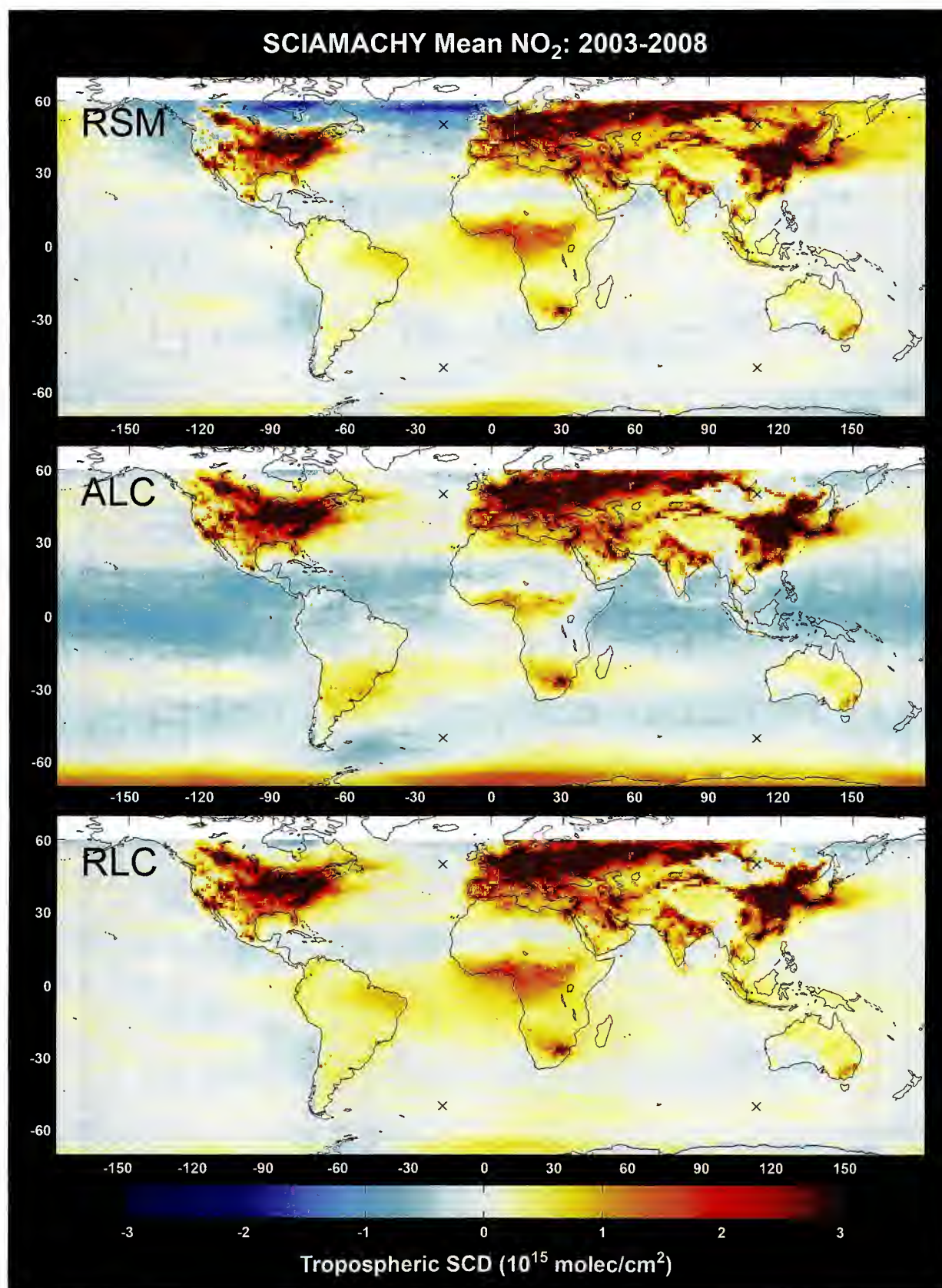
Fig. 7.16 Mean tropospheric NO 2 slant column densities as derived for the period 2003–2008 using the Reference Sector Method (RSM – top), Absolute Limb Correction (ALC – middle) and Relative Limb Correction (RLC – bottom) (Courtesy: S. Beirle, MPI for Chemistry, Mainz).
