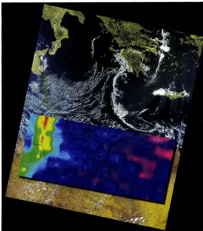
Fig. 10.12 The Mt. Etna volcanic eruption in 2002 with obvious \text{SO}_2 emissions (redish plume). The SCIAMACHY nadir measurement is overlaid on a MERIS image showing that the plume of \text{SO}_2 and the visible ash cloud match well (Courtesy: ESA and Brockmann Consult).
