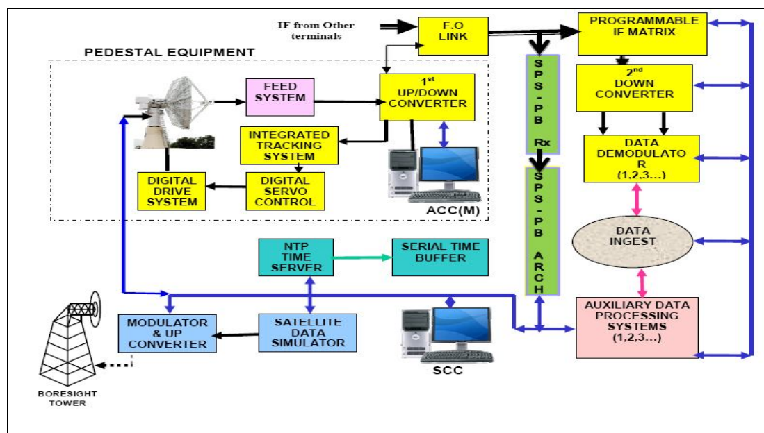
Fig. 5.5 Data Reception System Block
