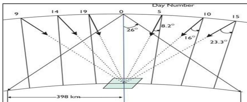
Figure 8.30 Steerability of LISS-IV camera
