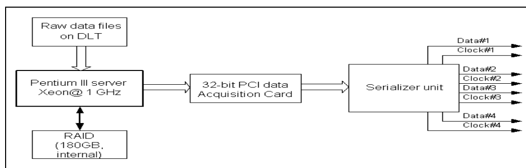
Fig. 5.14 Functional Block diagram of data serializer system
