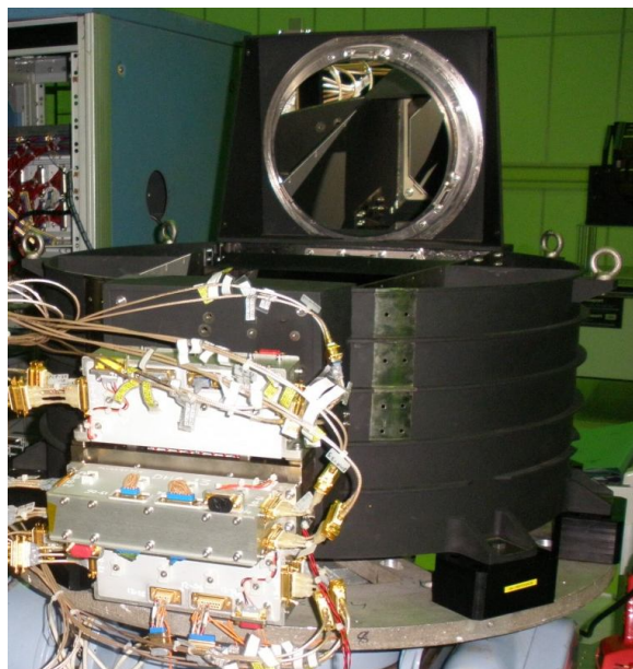
Figure 2.2 LISS-IV Payload
