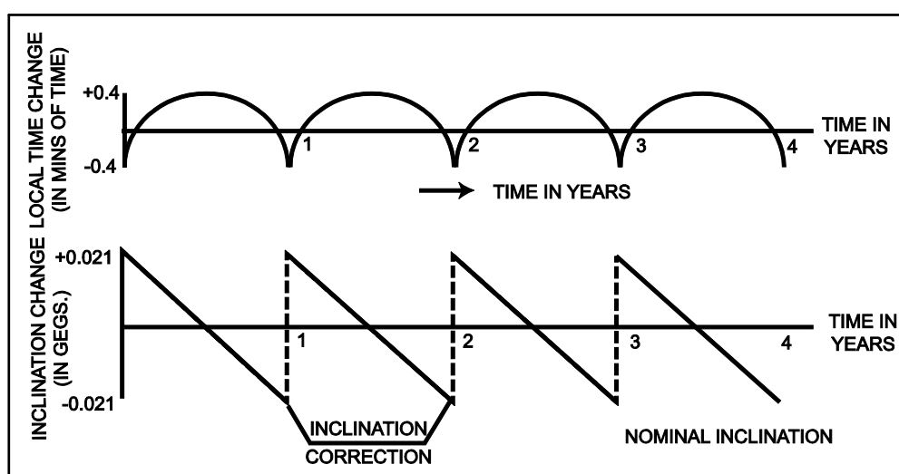
Figure 3.11 Local time control by inclination correction
