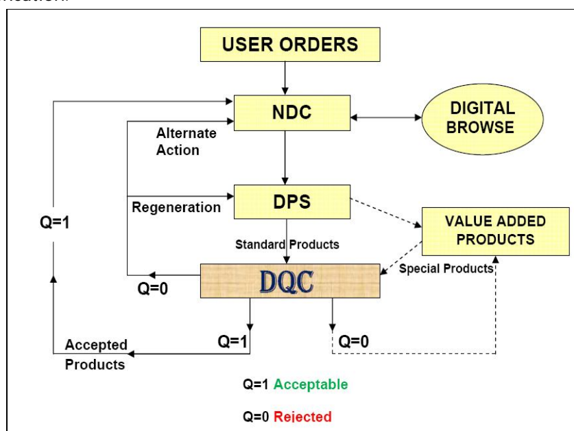
Fig. 7.3 Flow Chart for Generation of Digital products
