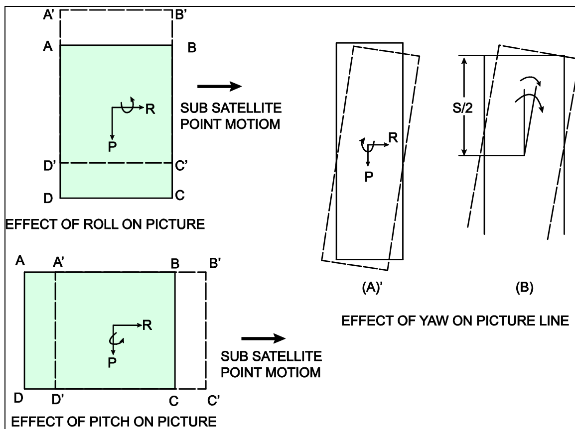
Figure 3.12 Effect of attitude errors on image
