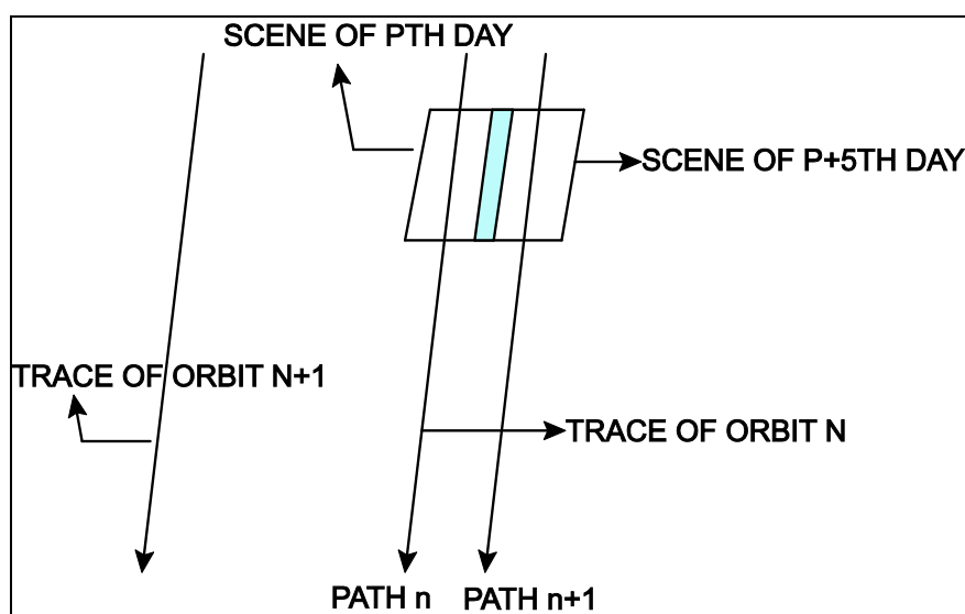
Figure 3.4 LISS-III coverage pattern.
