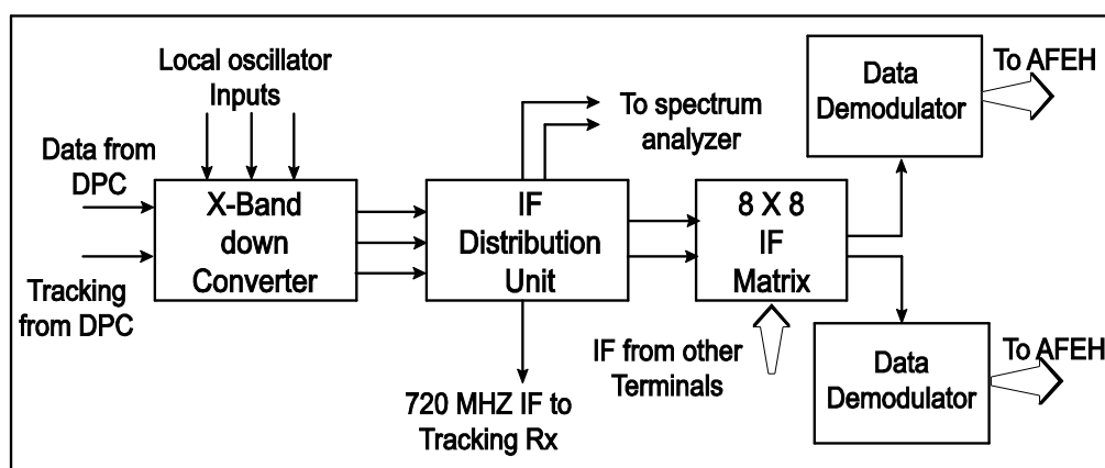
Figure 5.1 Block Diagram of IF and Base Band Systems
