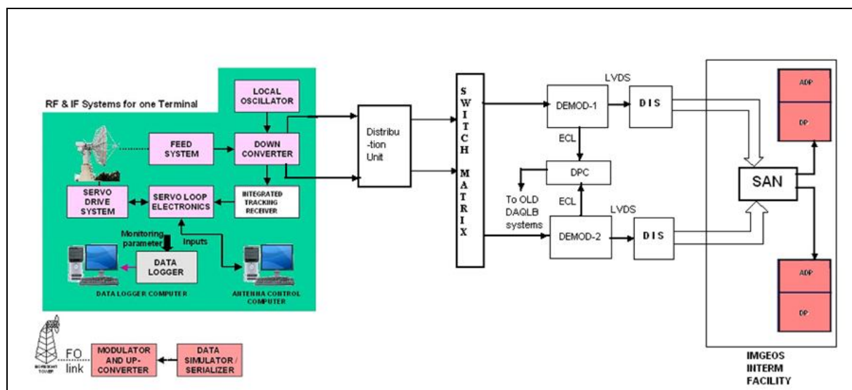
Fig. 5.4 Shadnagar Ground Station Configuration
