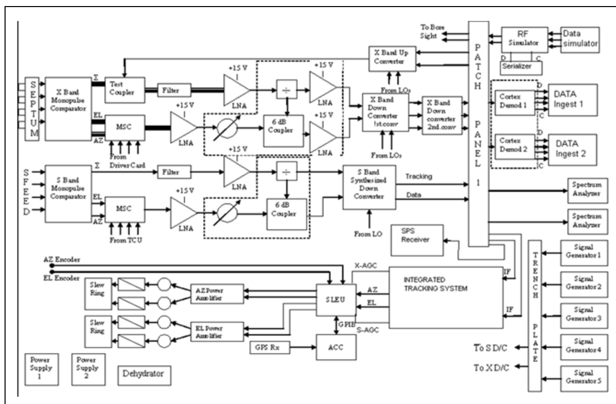
Fig. 5.6 Block Schematic of Data Receive system
