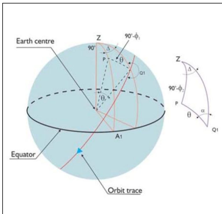
Figure 3.9 Calculations of coordinates of a point P on the earth surface.
