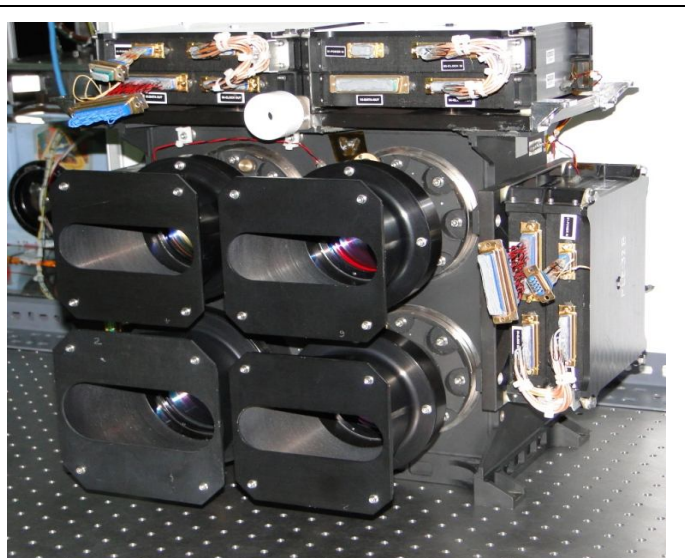
Figure 2.4 AWiFS Payload
