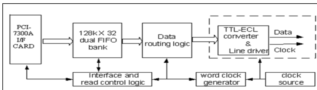
Fig. 5.15 Functional Block diagram of serializer
