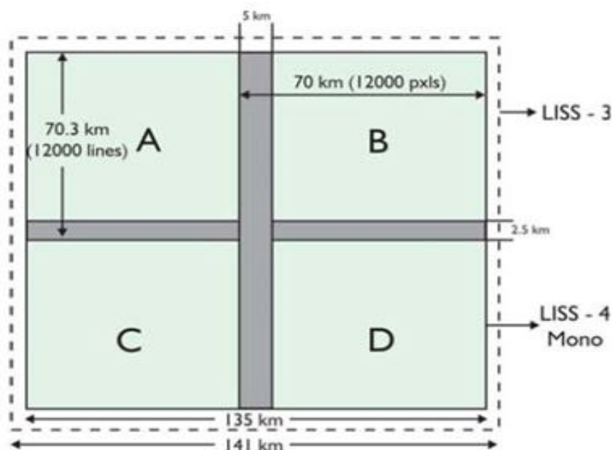
Figure 3.6 LISS-IV scene (Mono) within a LISS-3 scene
