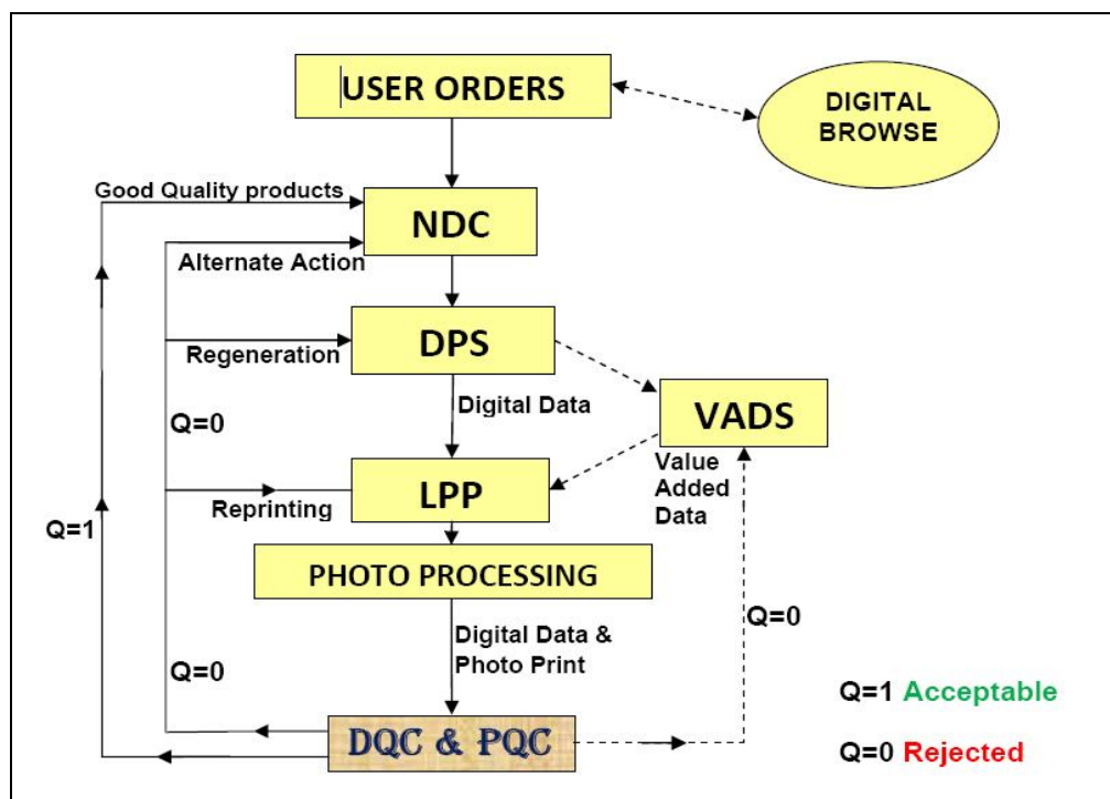
Fig. 7.2 Flow Chart for QC of photo products
