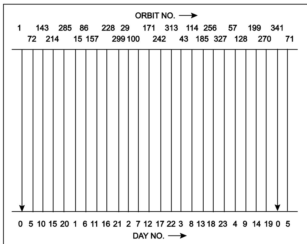
Figure 3.1 Ground Trace Pattern
