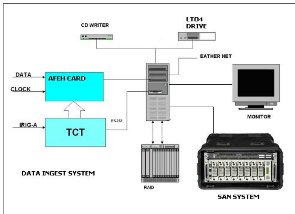
Fig. 5.8 Direct Ingest System
