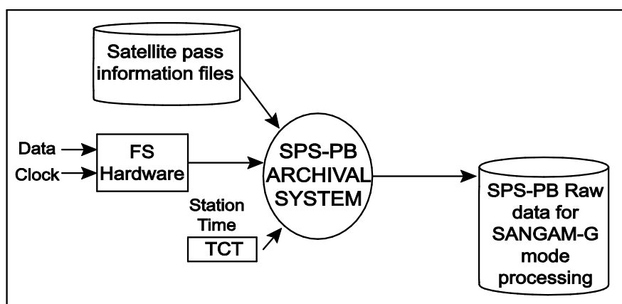
Fig. 5.9 Context diagram of SPS-PB data
