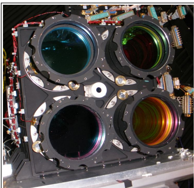
Figure 2.3 LISS-III Payload
