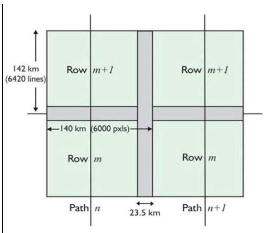
Figure 3.5 LISS-III scene layout
