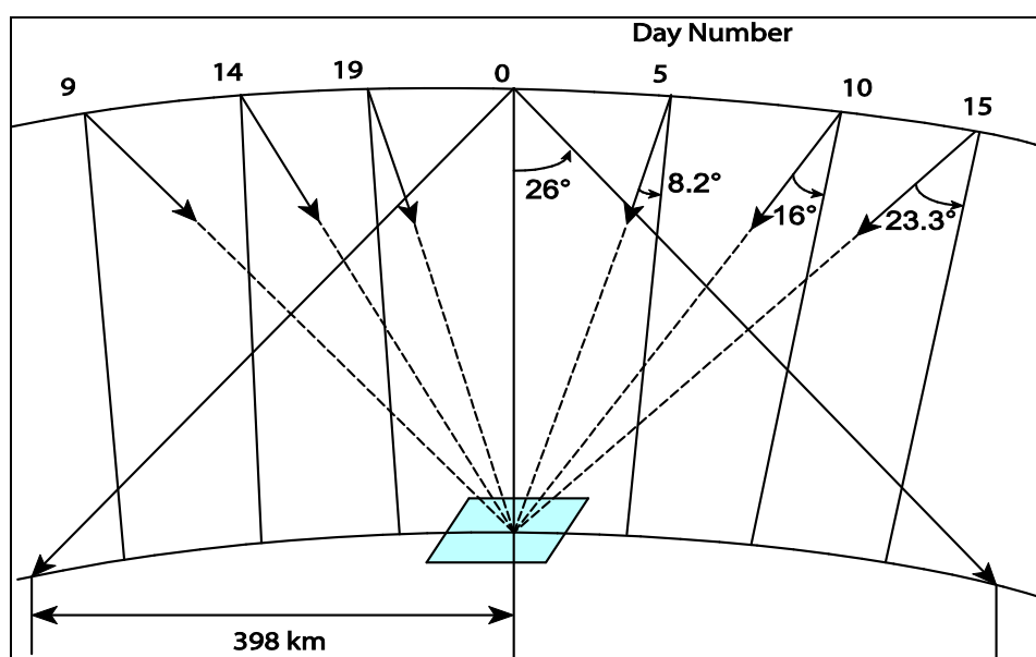
Figure 3.3 Coverage due to LISS-IV off-nadir capability
