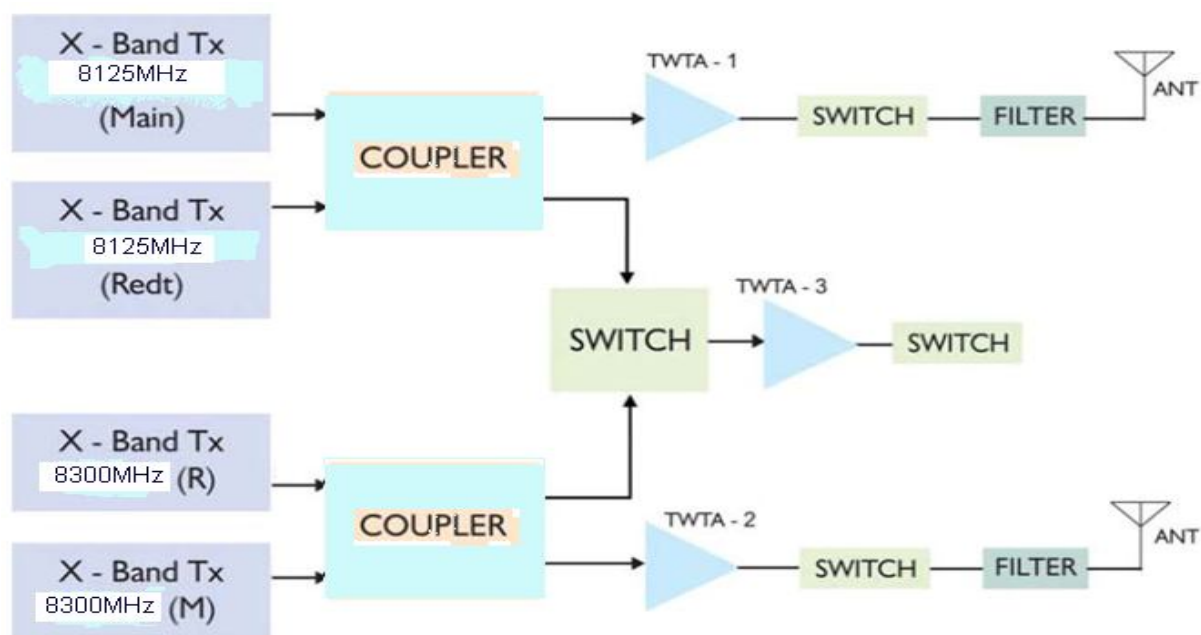
Figure 2.5 Schematic Diagram of DH(RF)
