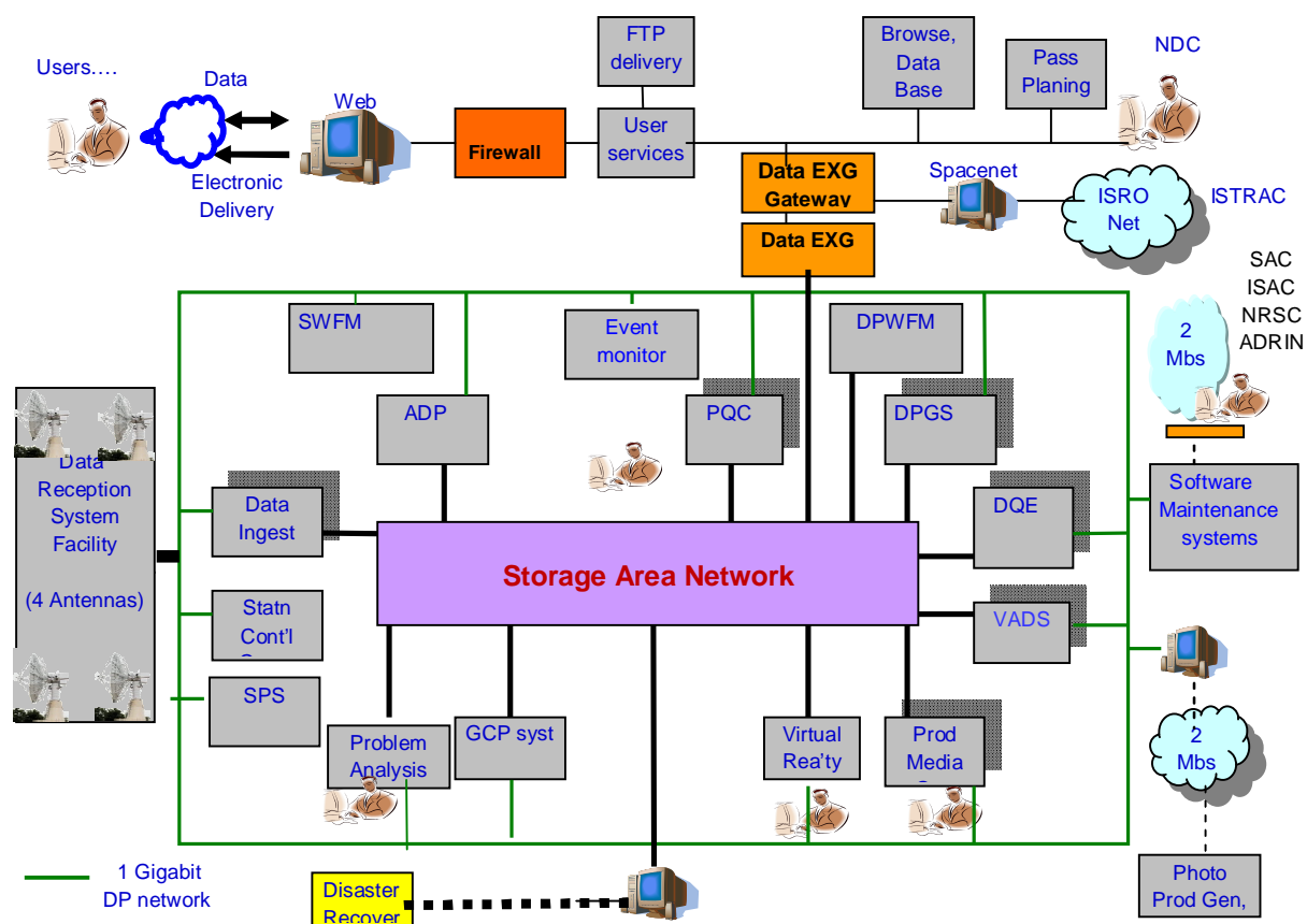
Fig. 6.1 Overview of Ground Segment Processing
