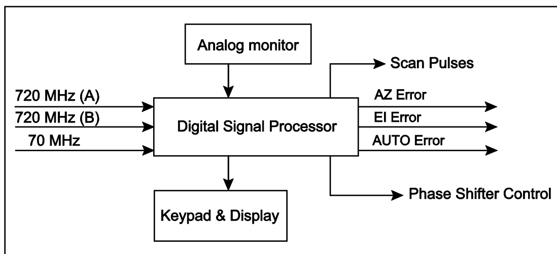
Fig. 5.3 Block Diagram of Integrated Tracking Systems (ITS)
