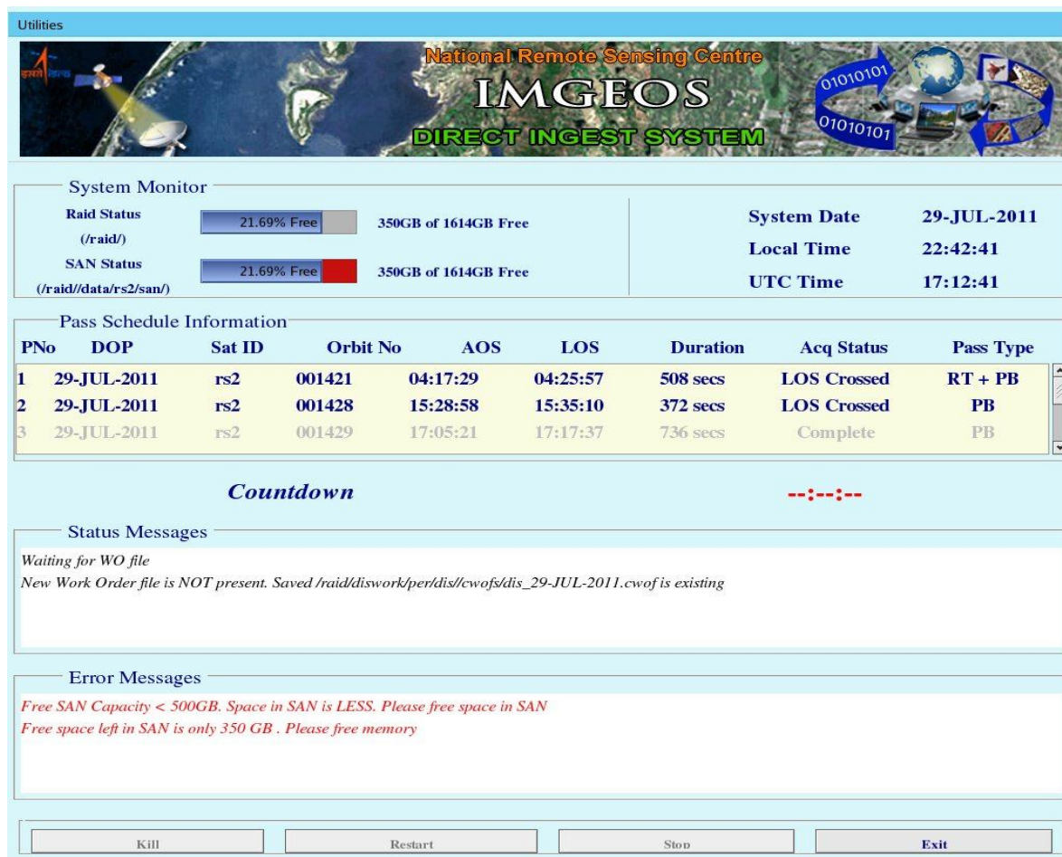
Fig. 6.4 Event Monitor System
