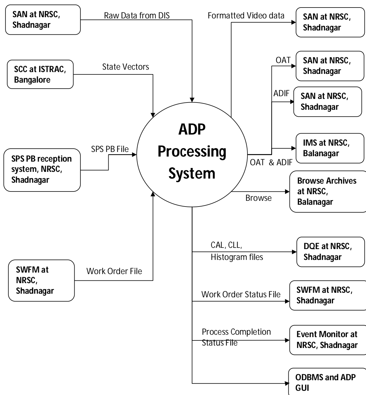
Fig. 6.5 Overview of ADP Processing System
