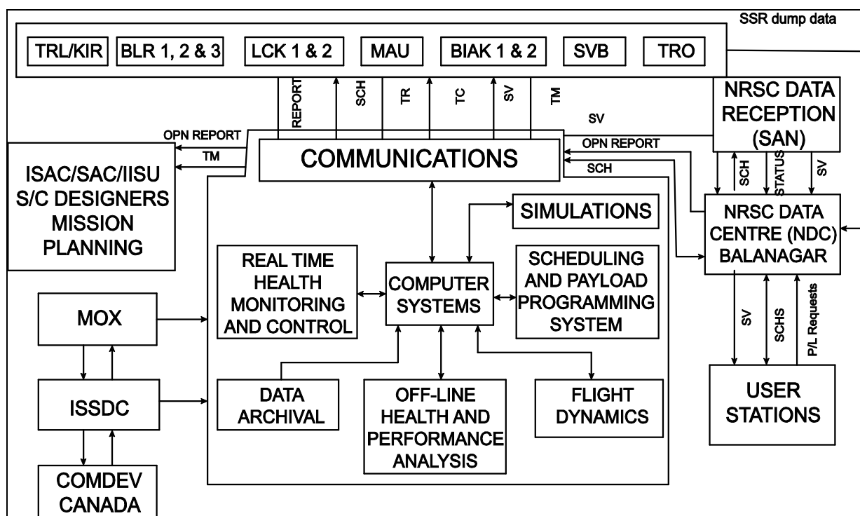
Figure 4.2. Organization of ground segment operations
