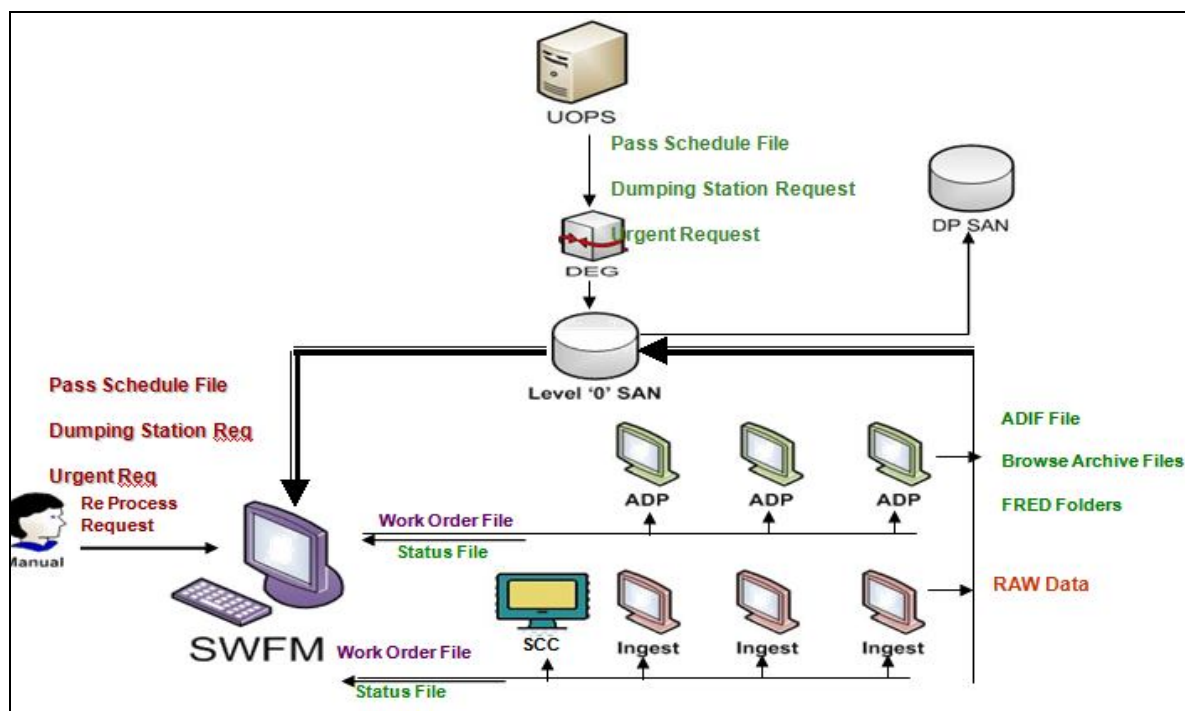
Fig. 6.2 Overview of Station Work Flow Manager
