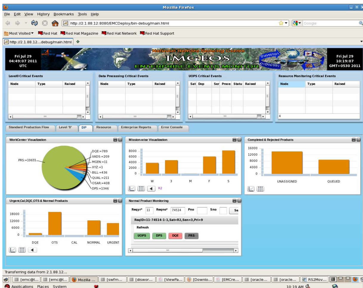
Fig. 6.9 Product status monitoring through EMC
