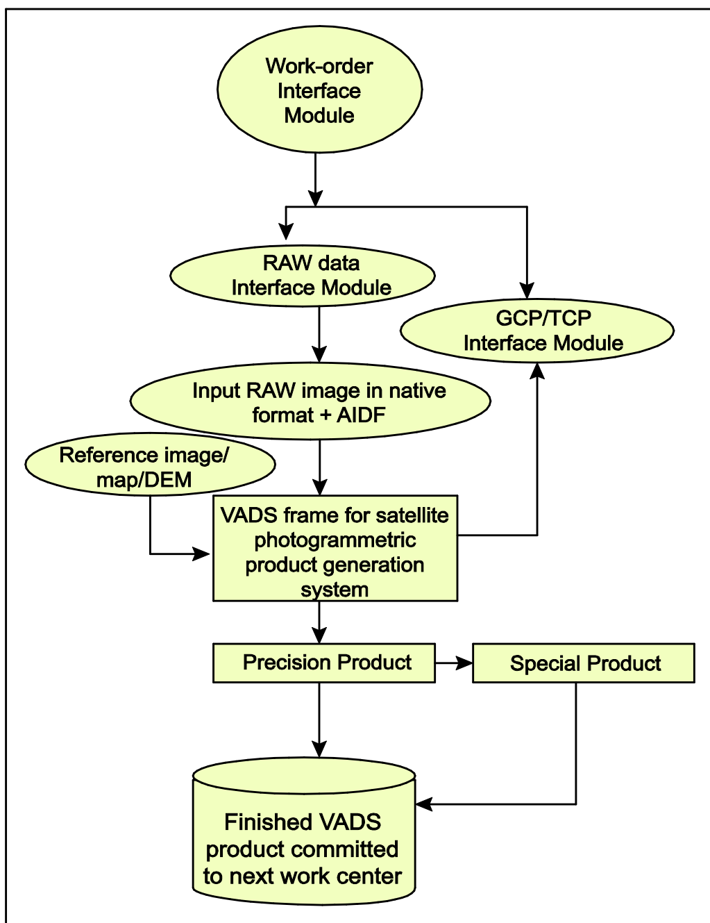
Figure 6.13 Satellite Photogrammetric products generation
