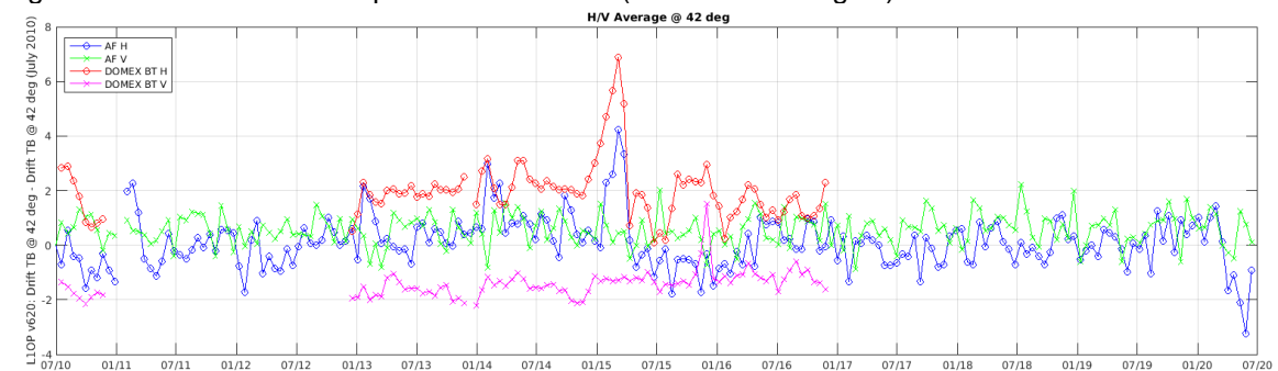
Figure 37: Dome-C H and V polarization trends in Alias Free zone (incidence angle 42°)
