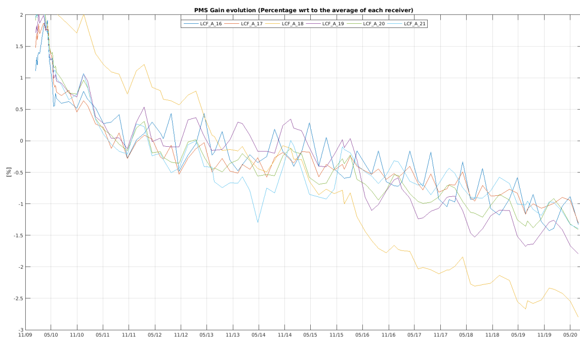
Figure 12 Evolution of the \Delta PMS Gain of the LICEFS in CMN A3
