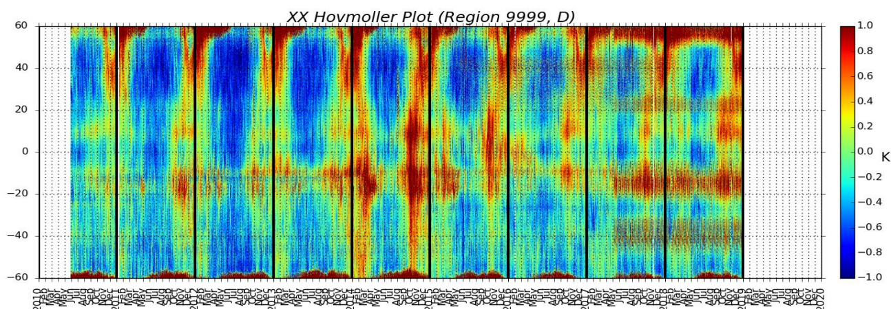
Figure 41: BT stability over the ocean, for XX polarization and Descending passes.
