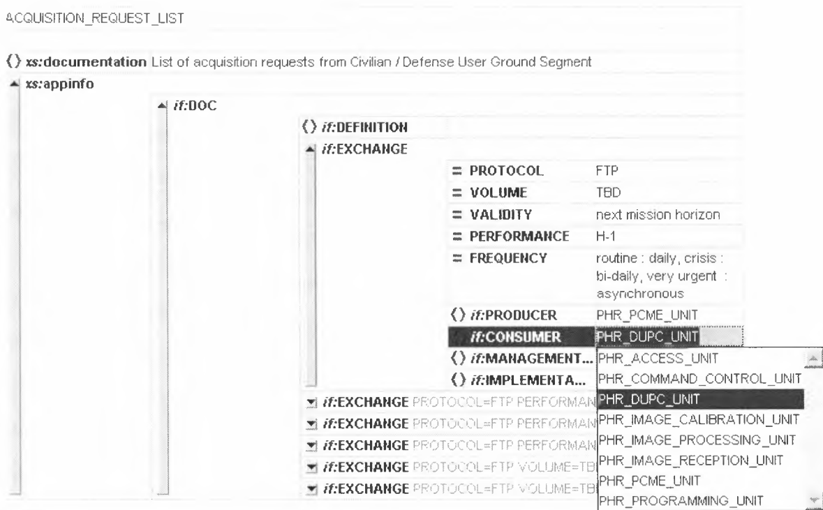
XML Spy editor help with specific schema [fig 3]
