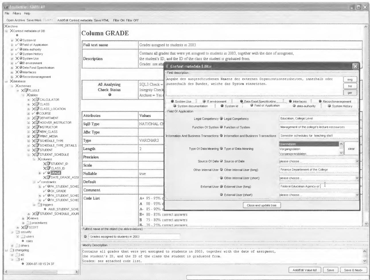
FIG. 3: AI’s workbench to add complementary narrative and context metadata to the database archive. For a single database object (selected in the object tree on the left-hand side) metadata is entered in the right-hand pane, while context metadata on the database level is entered in a multi-tab “Context Metadata Editor” window (shown in front of the right-hand pane).
