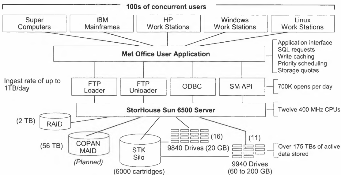
Fig.1. MASS System Today
