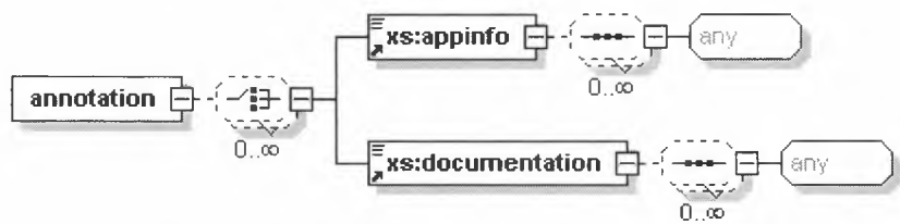
Generated with XMLSpy Schema Editor www.xmlspy.com Original annotation element [fig 1]
