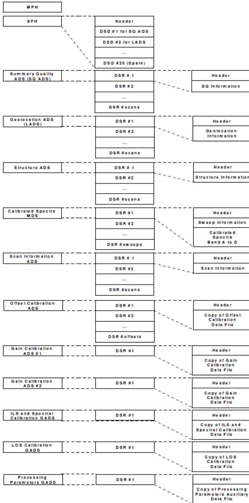
Figure 4.1-2 MIPAS level 1B product file structure
