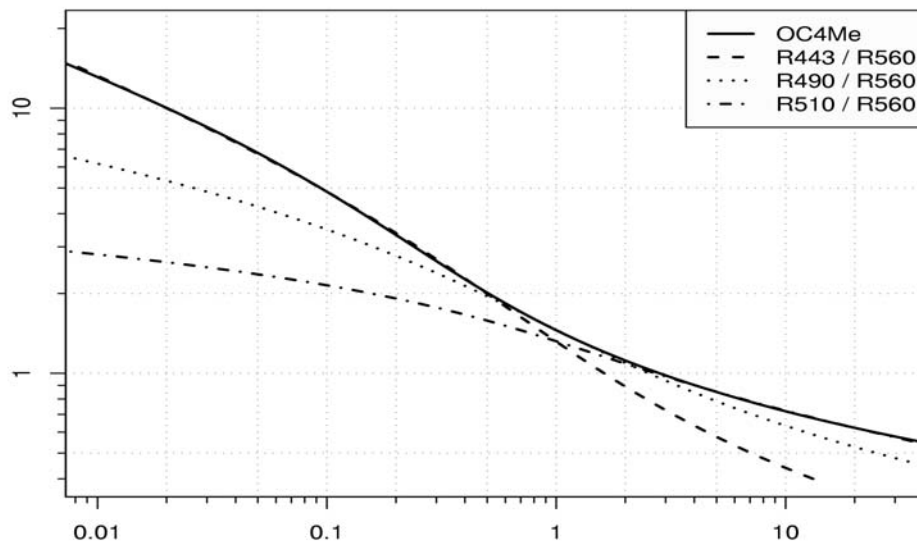
Figure 6. The three reflectance ratios (\rho_{2,5})_0 , (\rho_{3,5})_0 , (\rho_{4,5})_0 (as indicated), as a function of the algal pigment concentration, [Chl] ( mg\ m^{-3} ). They are derived from the revised reflectance model and when each reflectance takes its (minimal) value when the sun is at zenith (with f_0(\lambda) , corresponding to \theta_s = 0 ). The envelope for the three curves correspond to the maximum band ratio, and its polynomial best fit provides the algorithm OC4Me
