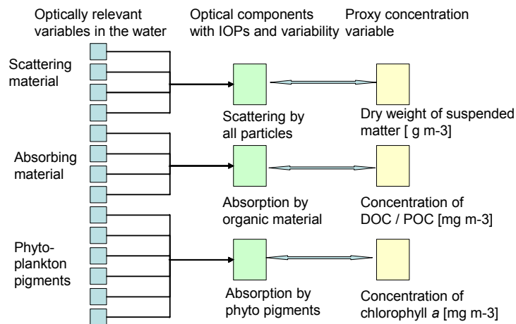
Fig. 2: Relationship between water constituents, components of a bio-optical model and concentrations
