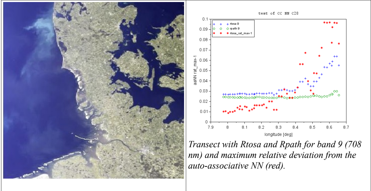
Fig. 38: Transect C28 (12.6.2006) between Cuxhaven and Helgoland with the track in the MERIS L1b scene of this day (left) and the reflectance along this track of Rtosa (blue) and the path radiance Rpath (green).
