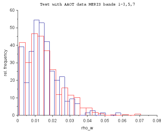
Fig. 51: Relative frequency distribution of the water reflectances, blue: AAOT, red: MERIS NN data
