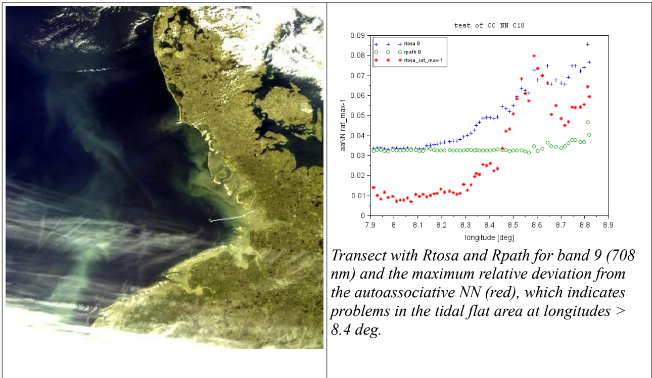
Fig. 14: Transect C18 (20.4.2014) between Büsum and Helgoland with the track in the MERIS L1b scene of this day (left) and the reflectance along this track of Rtosa (blue) and the path radiance Rpath (green).
