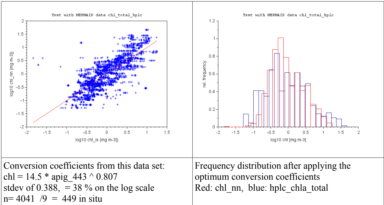
Fig. 57: Test after determining conversion coefficients from this data set
