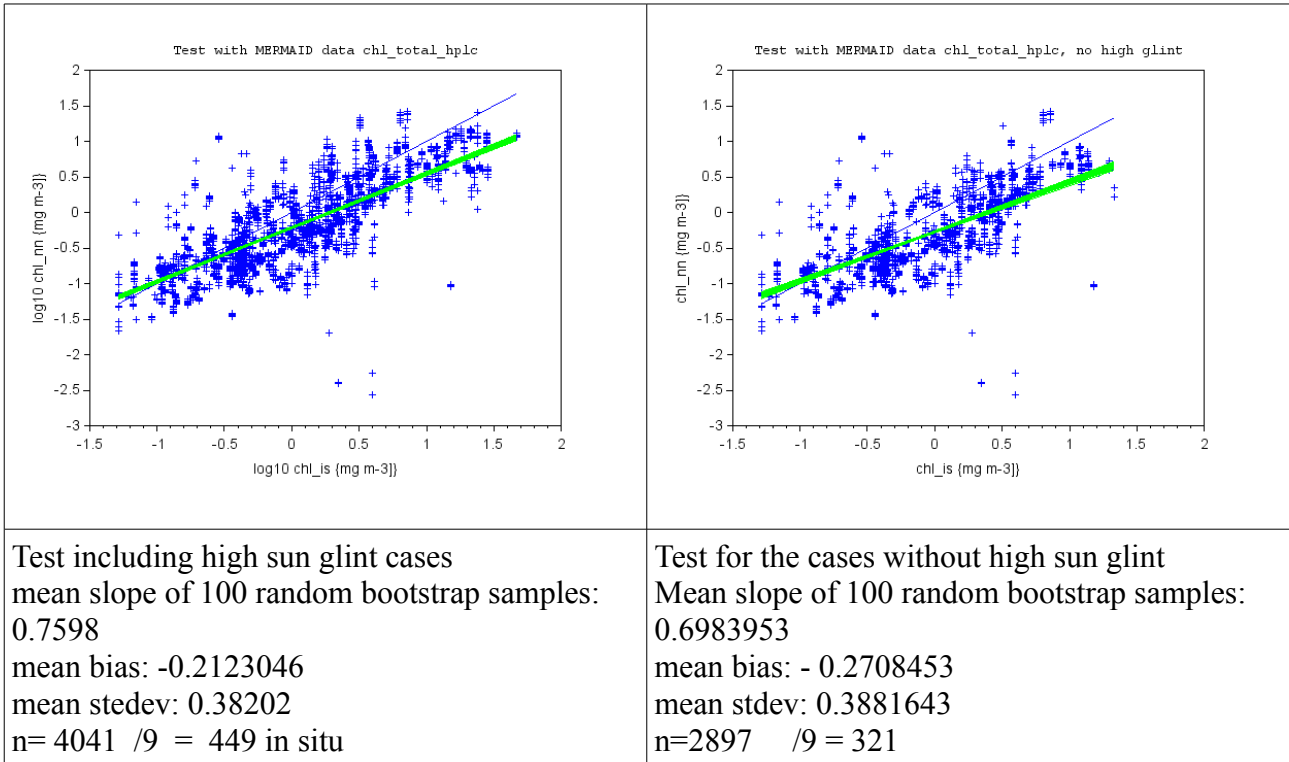
Fig. 56: Test using the hplc_total in situ data with and without high sun glint pixels
