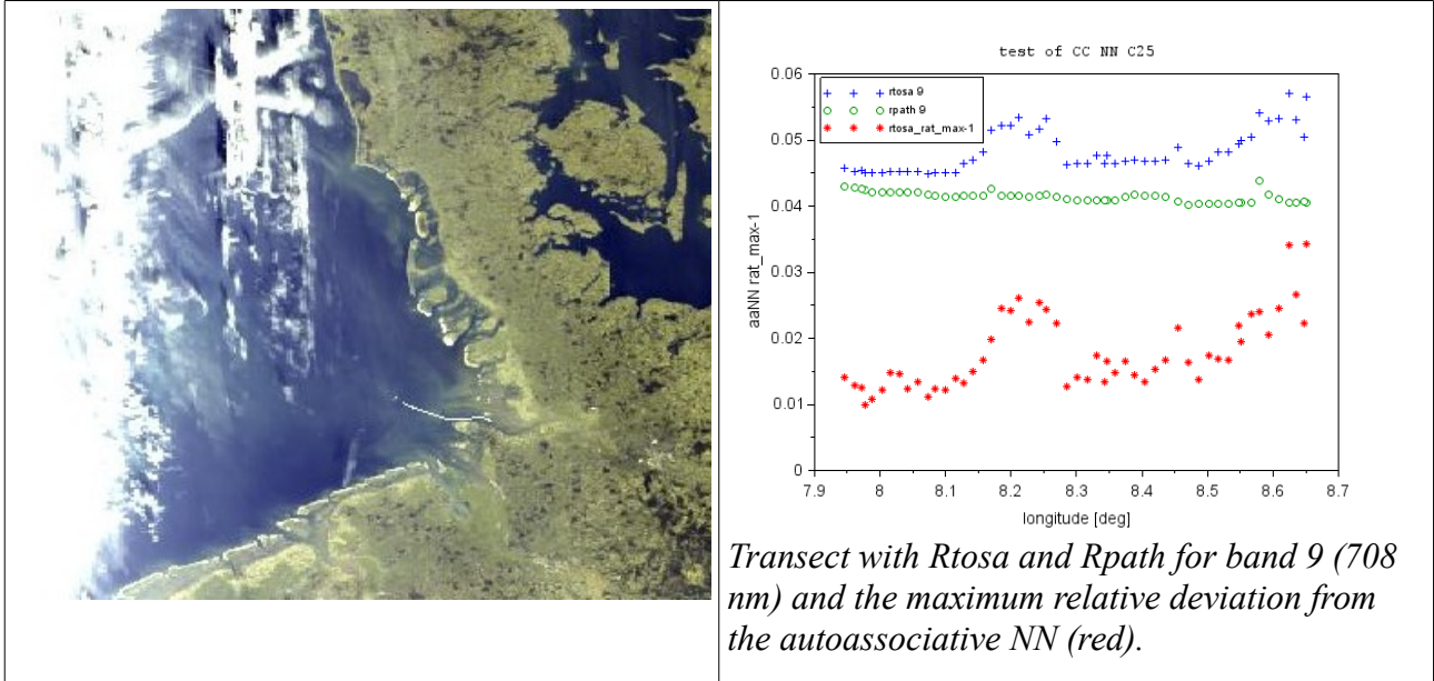
Fig. 26: Transect C25 (13.10.2005) between Cuxhaven and Helgoland with the track in the MERIS L1b scene of this day (left) and the reflectance along this track of Rtos (blue) and the path radiance Rpath (green).
