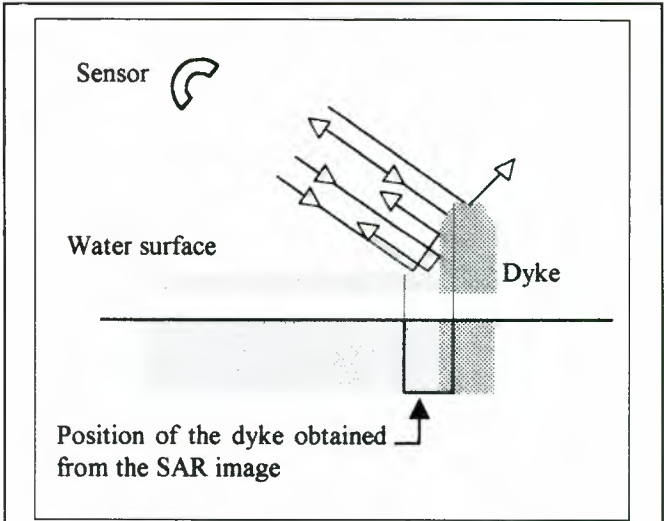
Fig. 6. Interaction of radar beams with a dyke.
