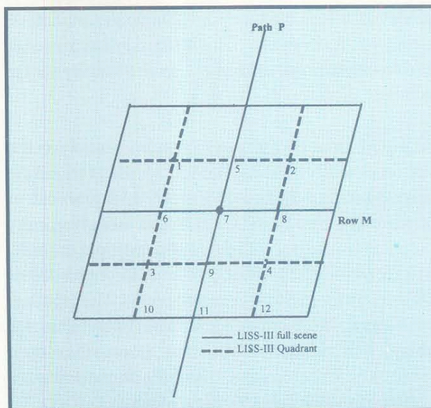
Figure 4.3.3.3.1 LISS-III Quadrants
