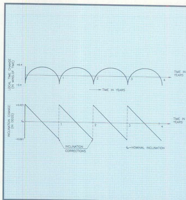
Figure 4.2.15.2 Local time control by inclination corrections
