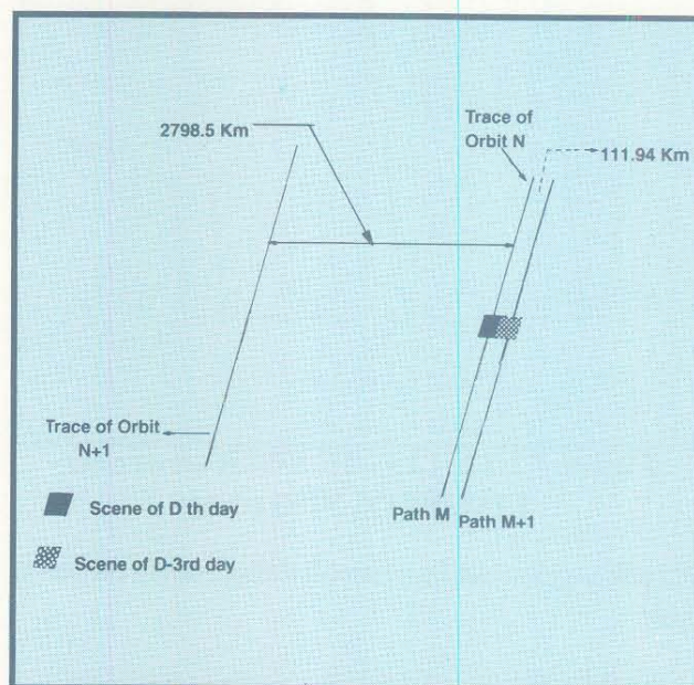
Figure 4.2.7.1. LISS-III coverage pattern
