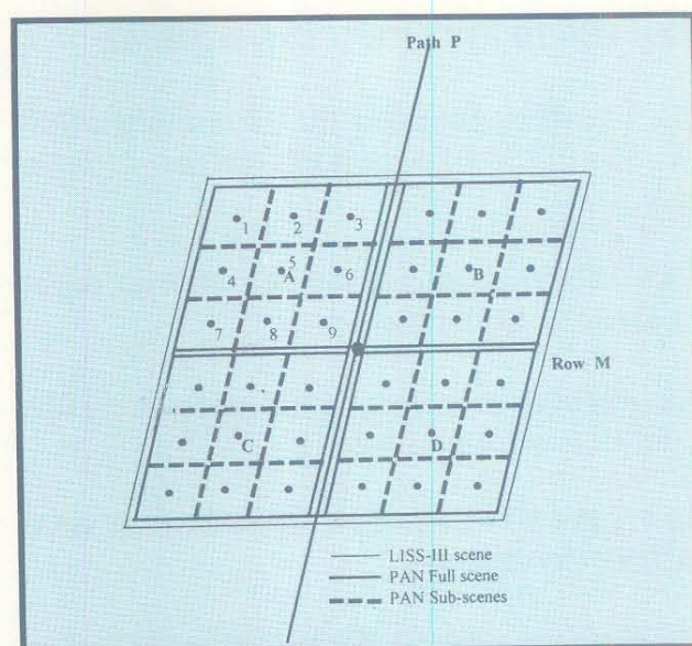
Figure 4.2.8.1. PAN subscenes
