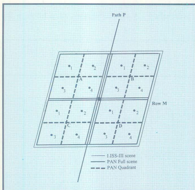
Figure 4.3.3.3.2 PAN Quadrants
