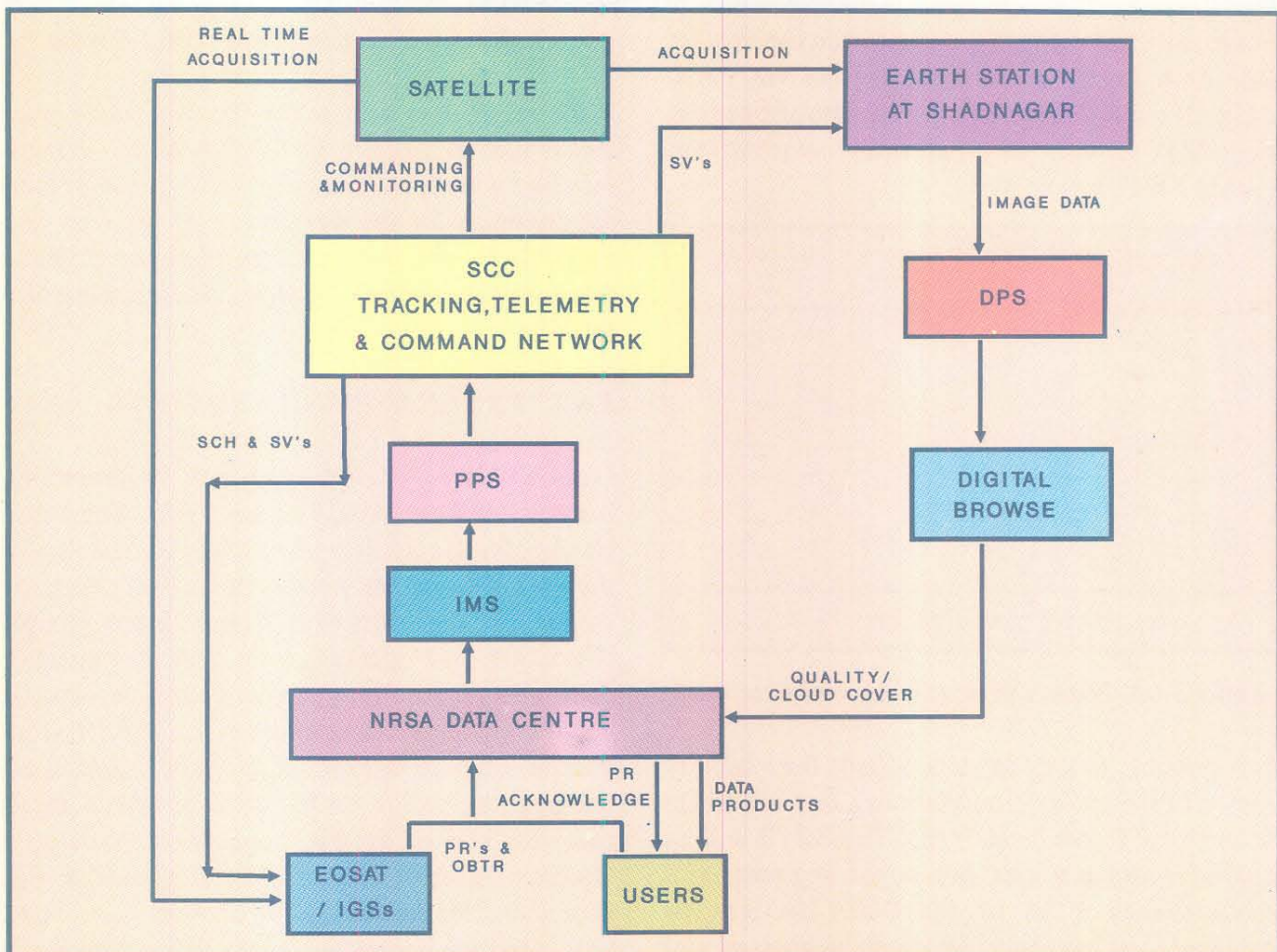
Figure 5.6.2.1 Programming activities
