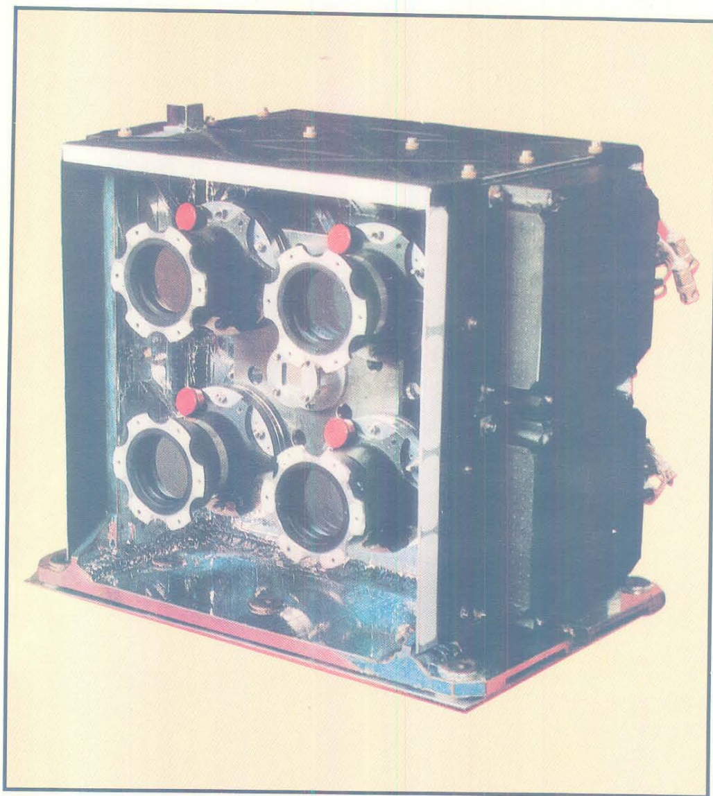
LISS-III camera
