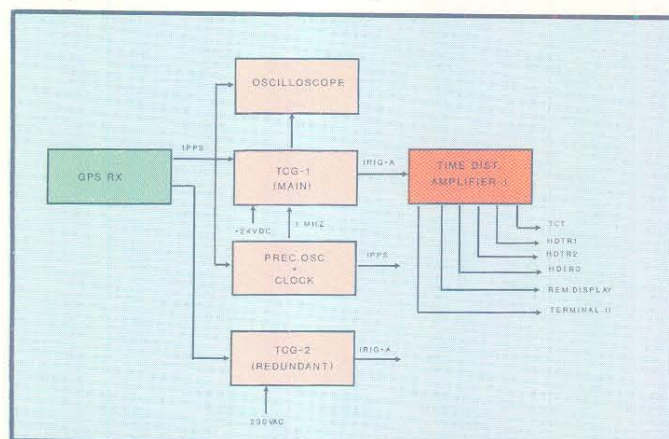
Figure 3.3.2 Block diagram of timing system
