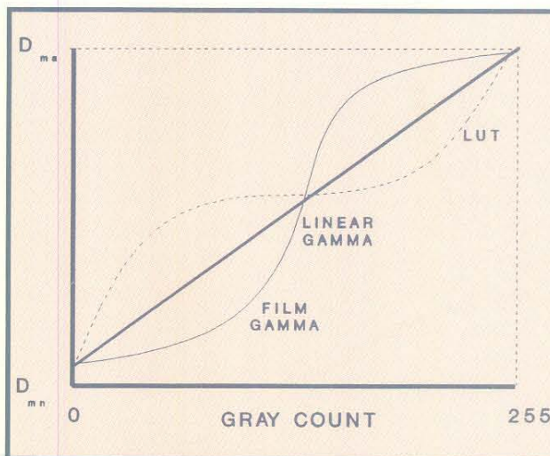
Figure 3.5.2 Film gamma correction
