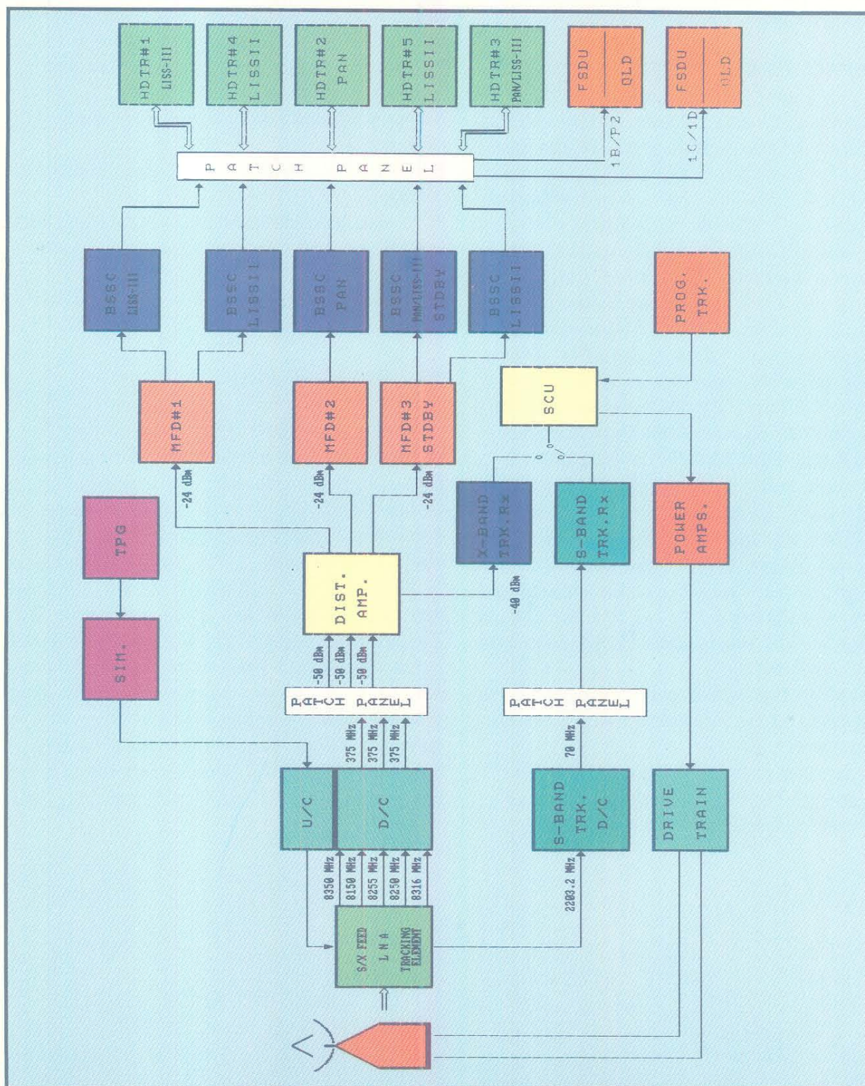
Figure. 3.2.1 Typical ground station configuration
