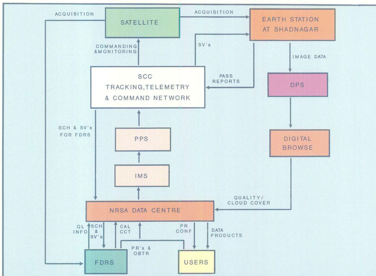
Figure 5.9.1 Programming activities
