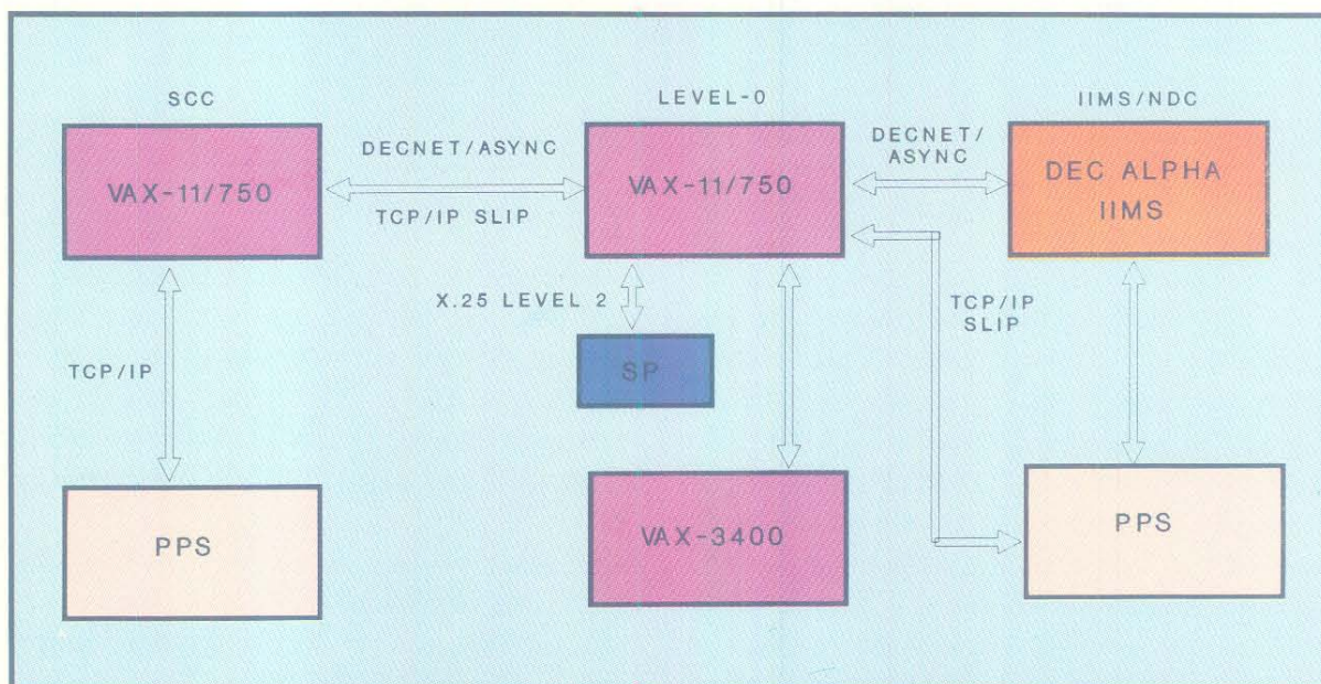
Figure 3.3.4 Block diagram of SCC-Shadnagar-Balanagar Networking interfaces
