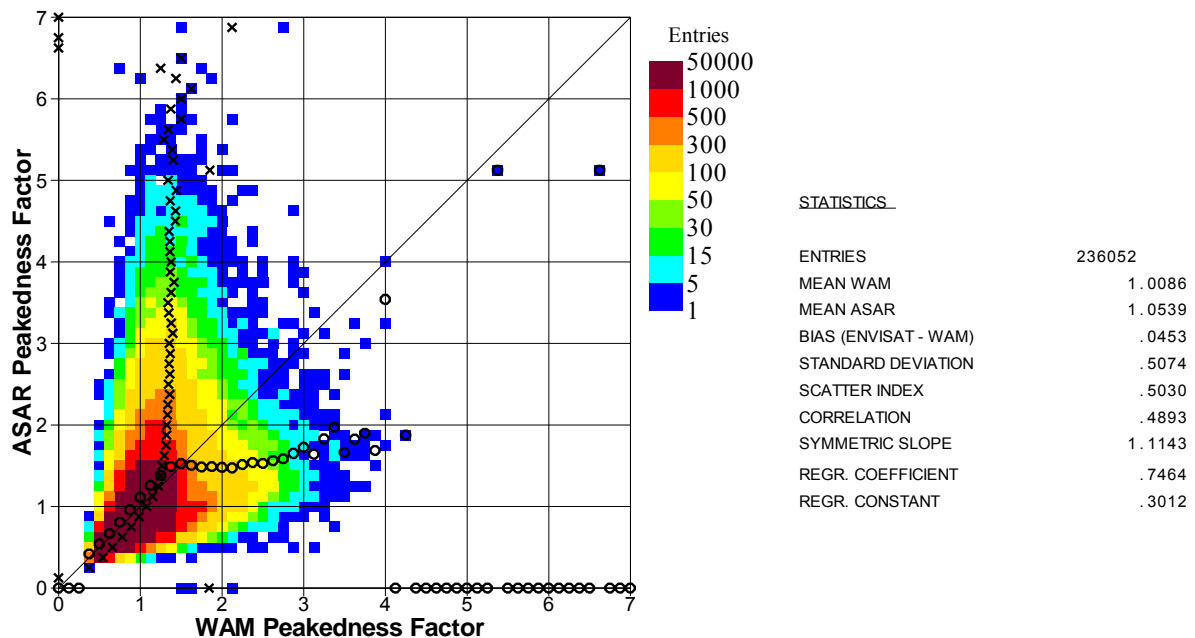
Fig. II.8. Global comparison between inverted ASAR level 1b and ECMWF model WPF during the period from 11 April to 31 August 2005.
