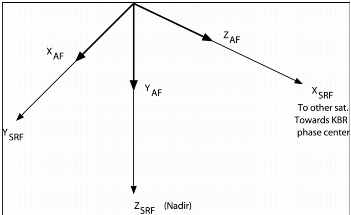
Figure 1-1 Satellite body-fixed frames
