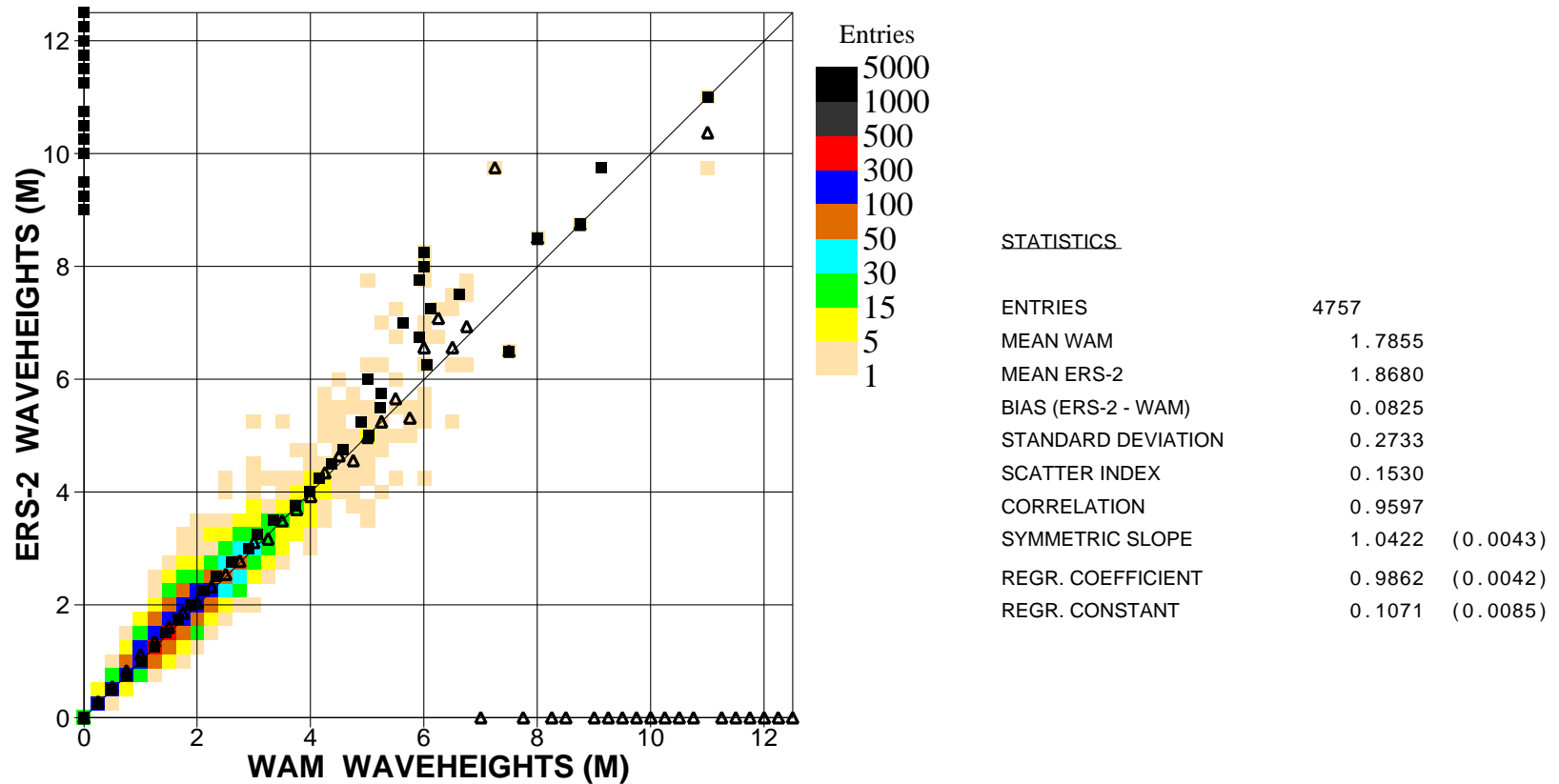
Figure 2: Comparison of ECMWF wave height results with ERS2 SAR wave height data for September 2003 (global)
