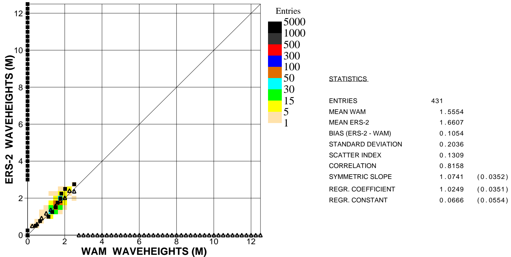
Figure 4: Comparison of ECMWF wave height results with ERS2 SAR wave height data for September 2003 (tropics)
