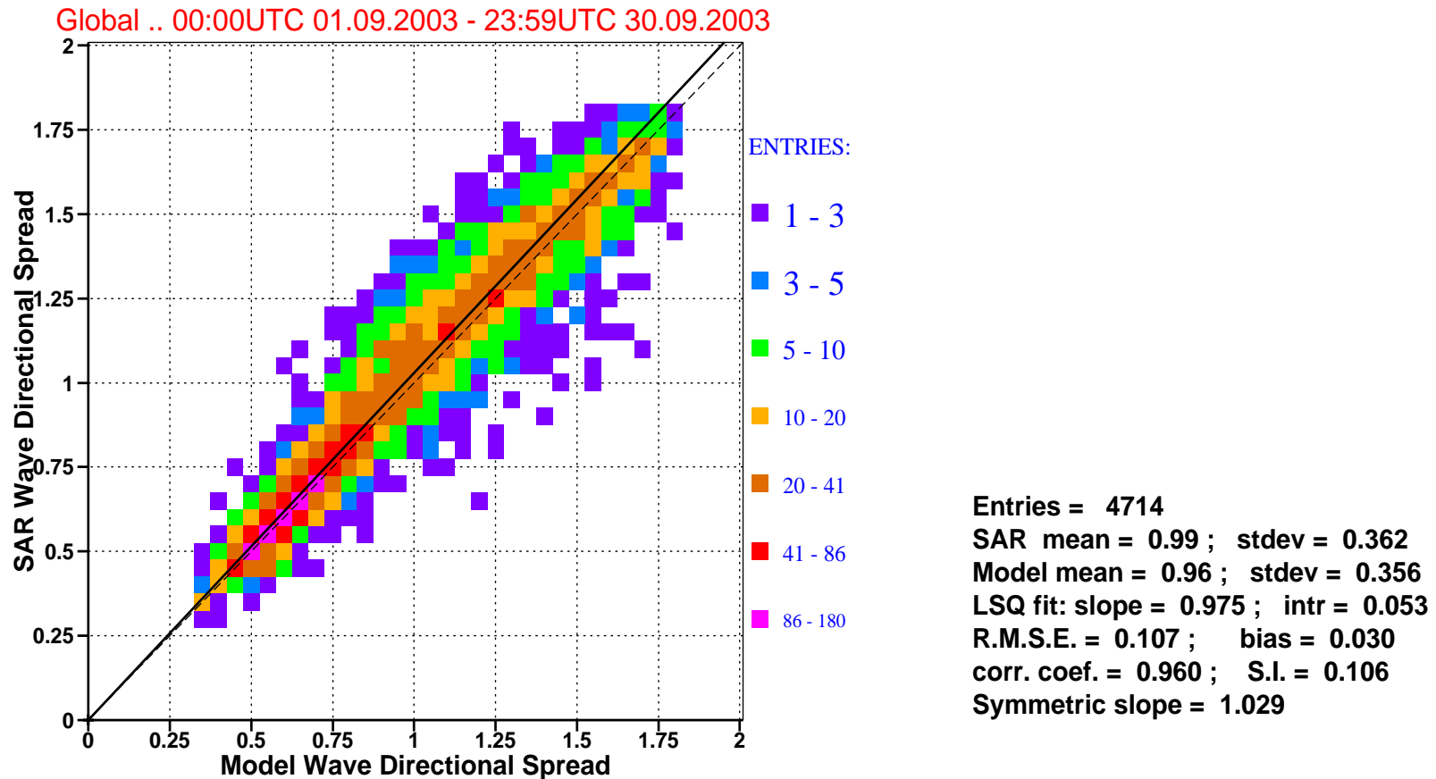
Figure 8: Comparison of ECMWF wave directional spread with that of ERS-2 SAR for september 2003 (global).
