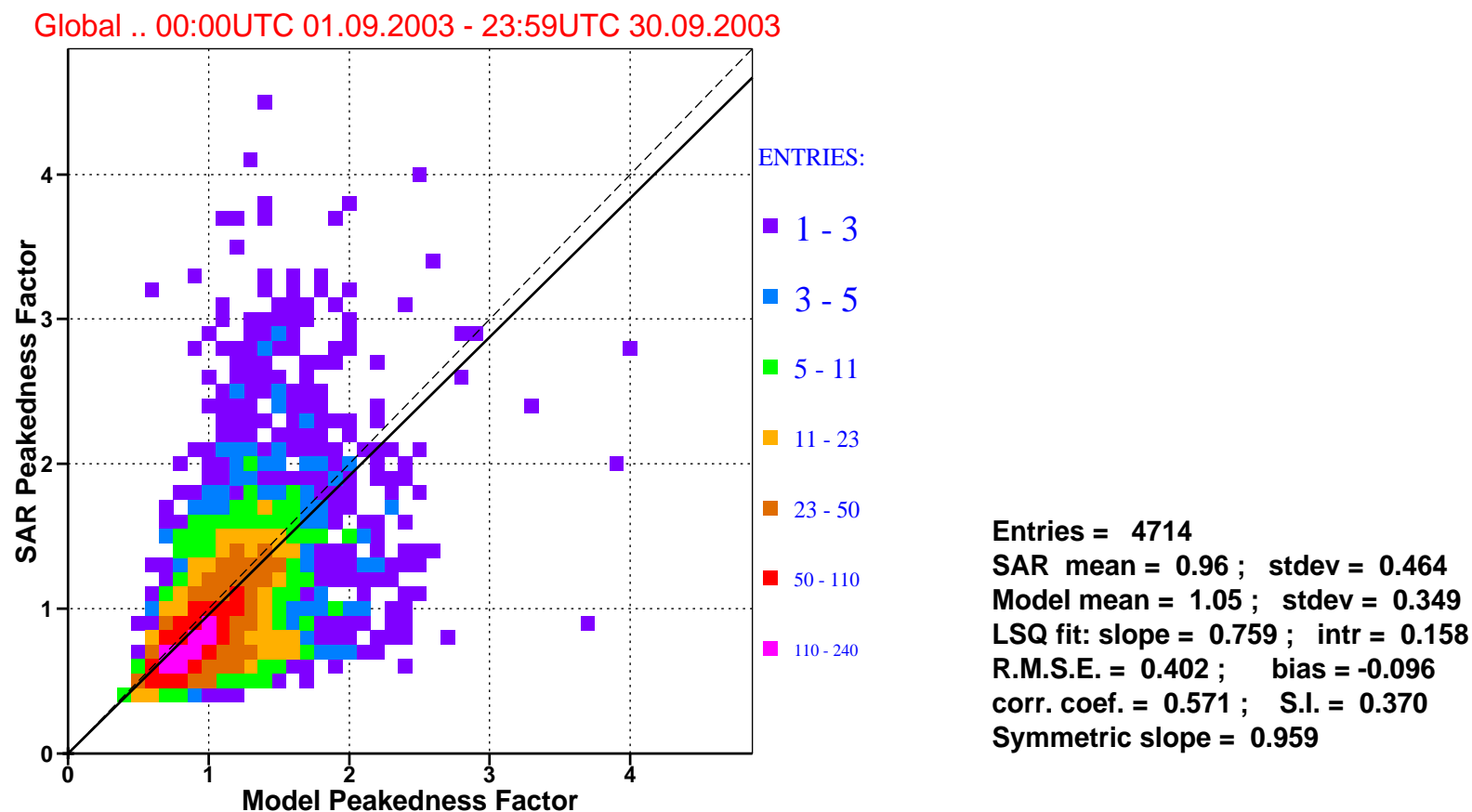
Figure 10: : Comparison of ECMWF wave peakedness factor with that of ERS-2 SAR for september 2003 (global).
