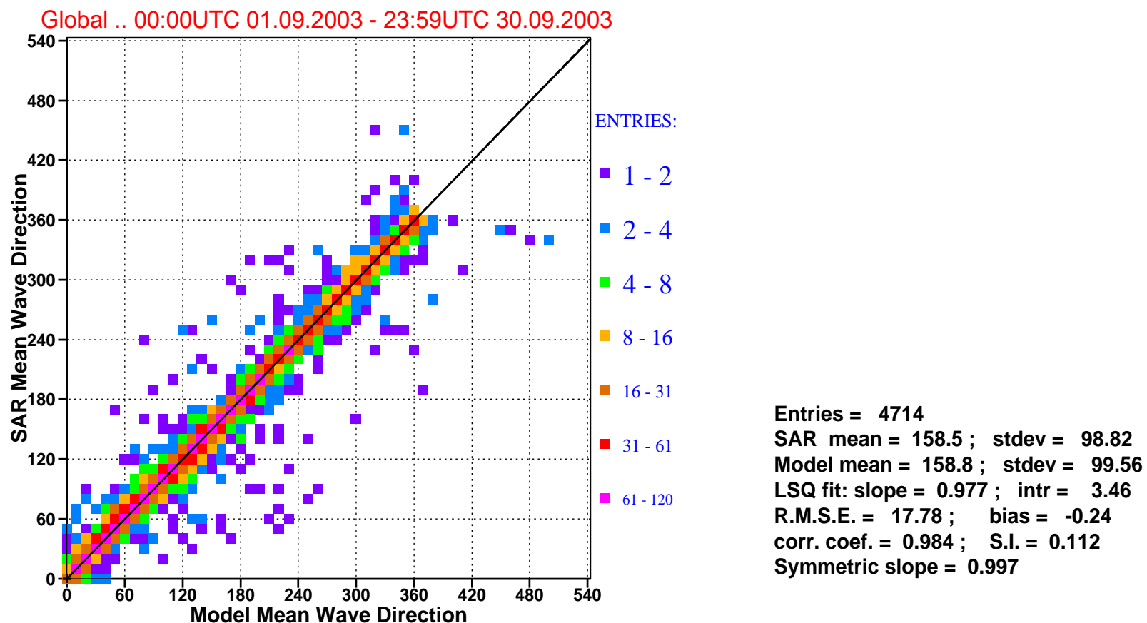
Figure 9: Comparison of ECMWF mean wave directions with that of ERS-2 SAR for september 2003 (global).
