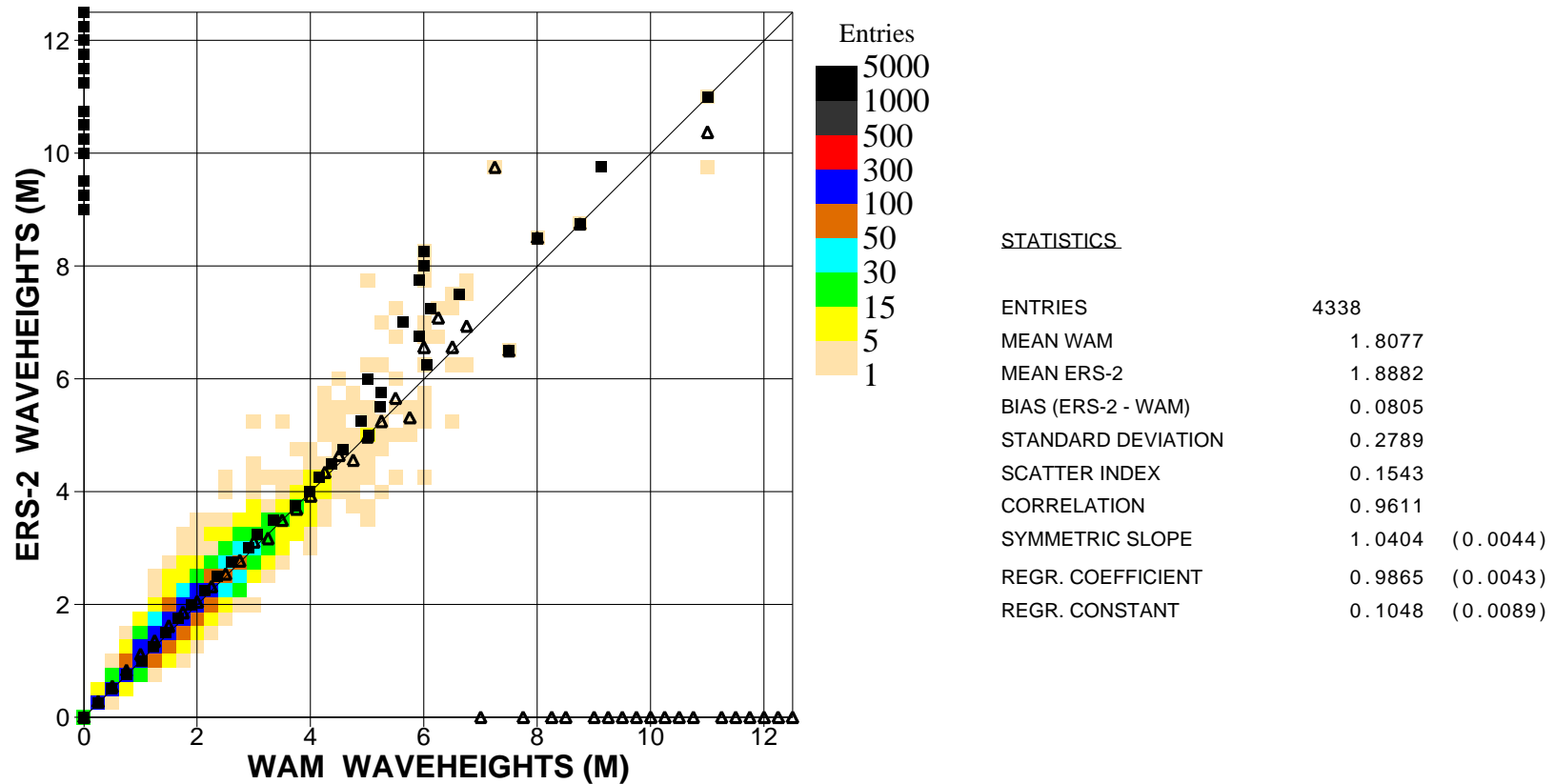
Figure 3: Comparison of ECMWF wave height results with ERS2 SAR wave height data for September 2003 (n.hem.)
