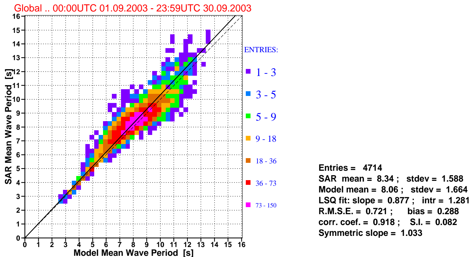
Figure 7: Comparison of ECMWF mean wave periods with ERS-2 SAR mean wave periods for september 2003 (global).
