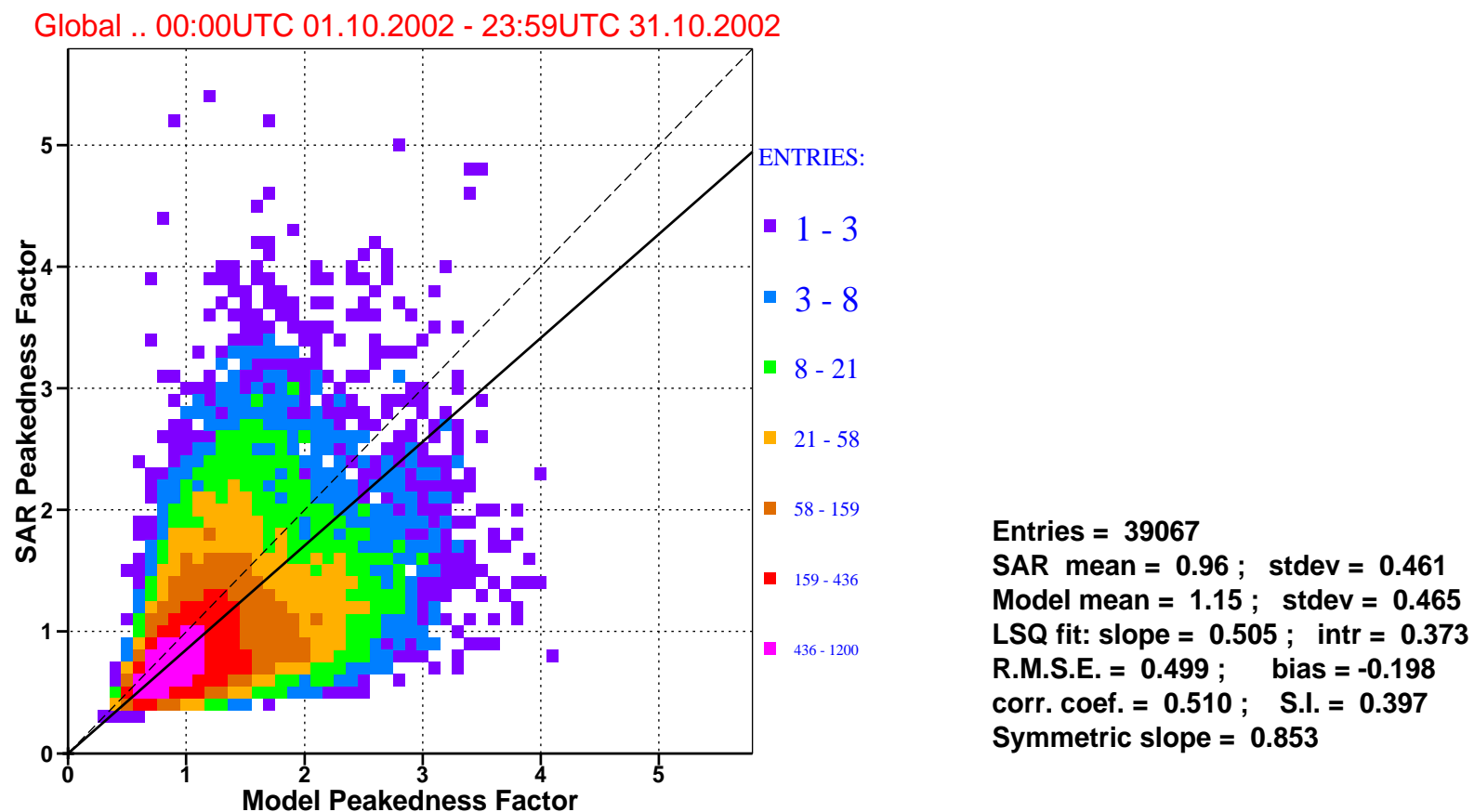
Figure 10: : Comparison of ECMWF wave peakedness factor with that of ERS-2 SAR for october 2002 (global).
