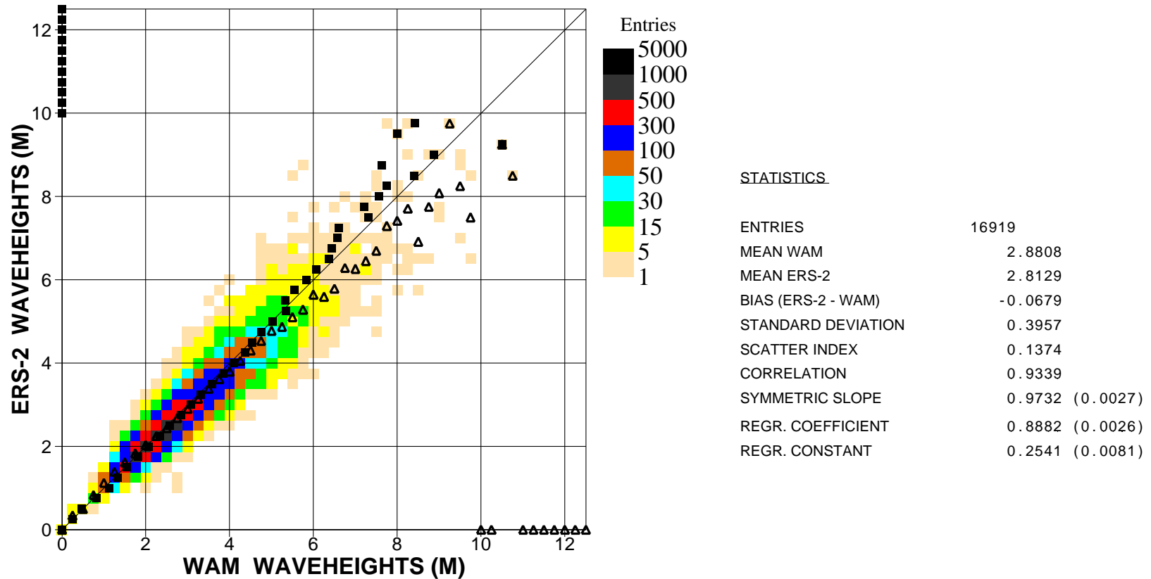
Figure 5: Comparison of ECMWF wave height results with ERS2 SAR wave height data for October 2002 (s.hem.)
