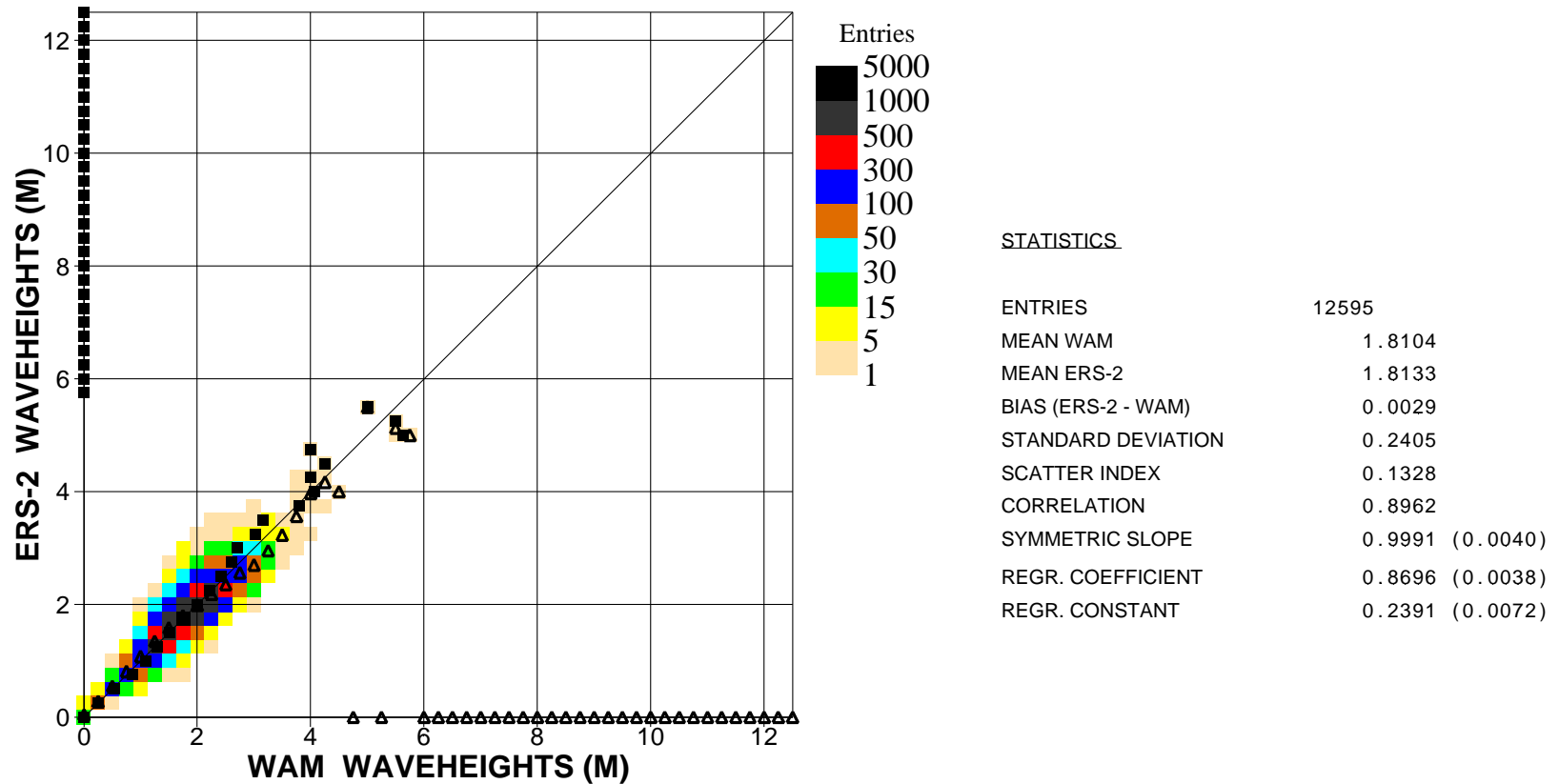
Figure 4: Comparison of ECMWF wave height results with ERS2 SAR wave height data for October 2002 (tropics)
