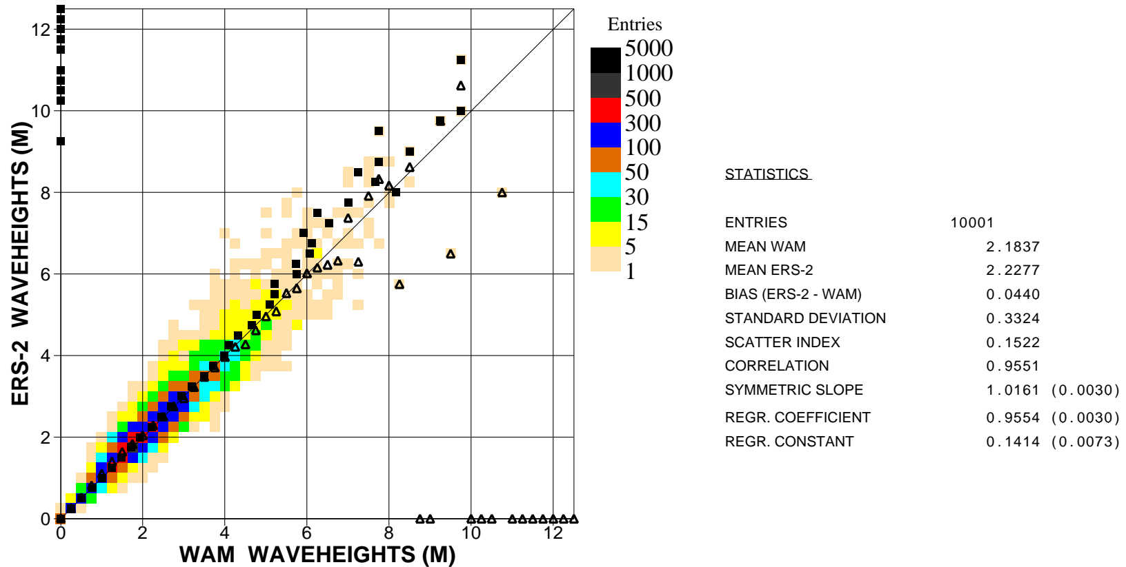
Figure 3: Comparison of ECMWF wave height results with ERS2 SAR wave height data for October 2002 (n.hem.)
