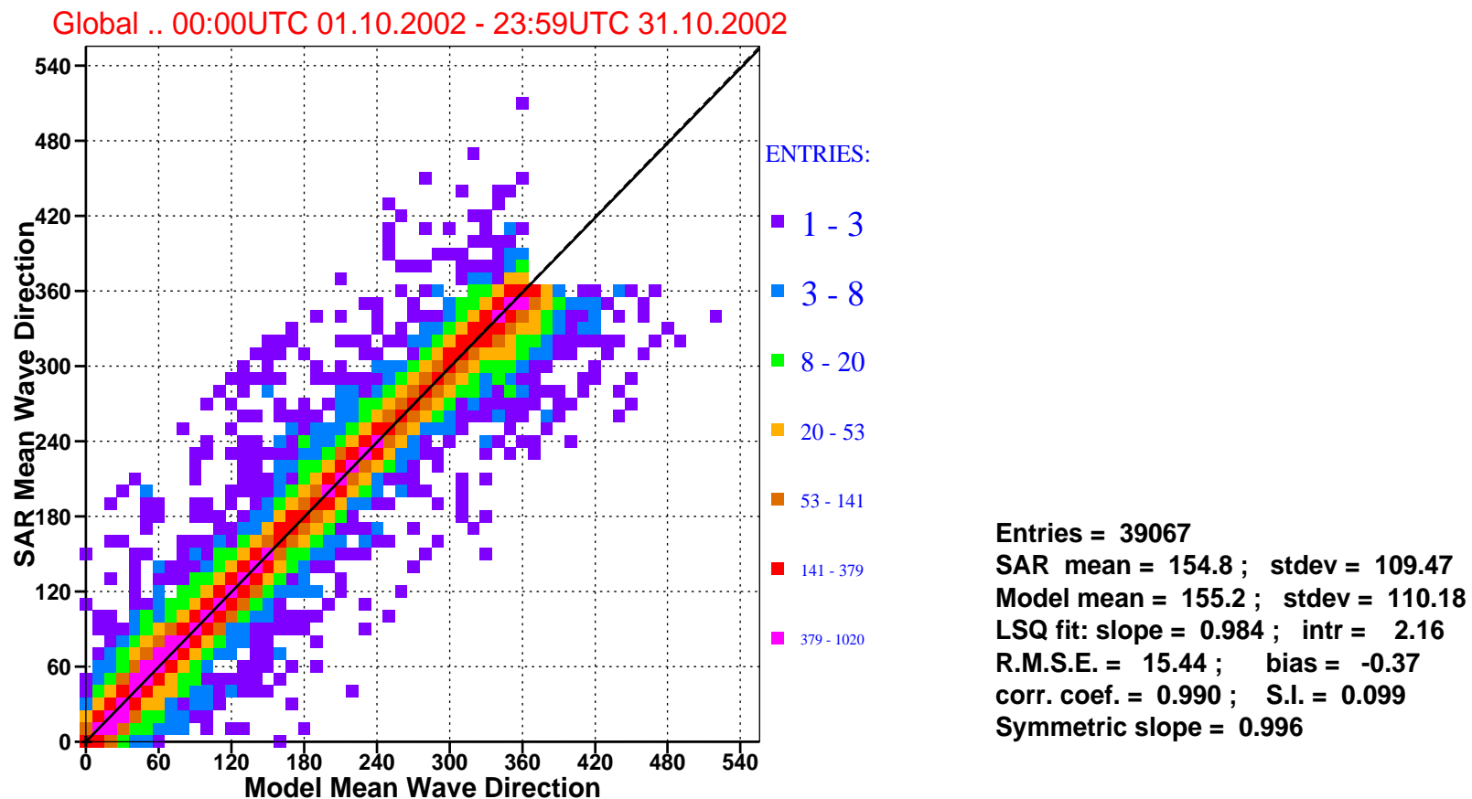
Figure 9: Comparison of ECMWF mean wave directions with that of ERS-2 SAR for october 2002 (global).
