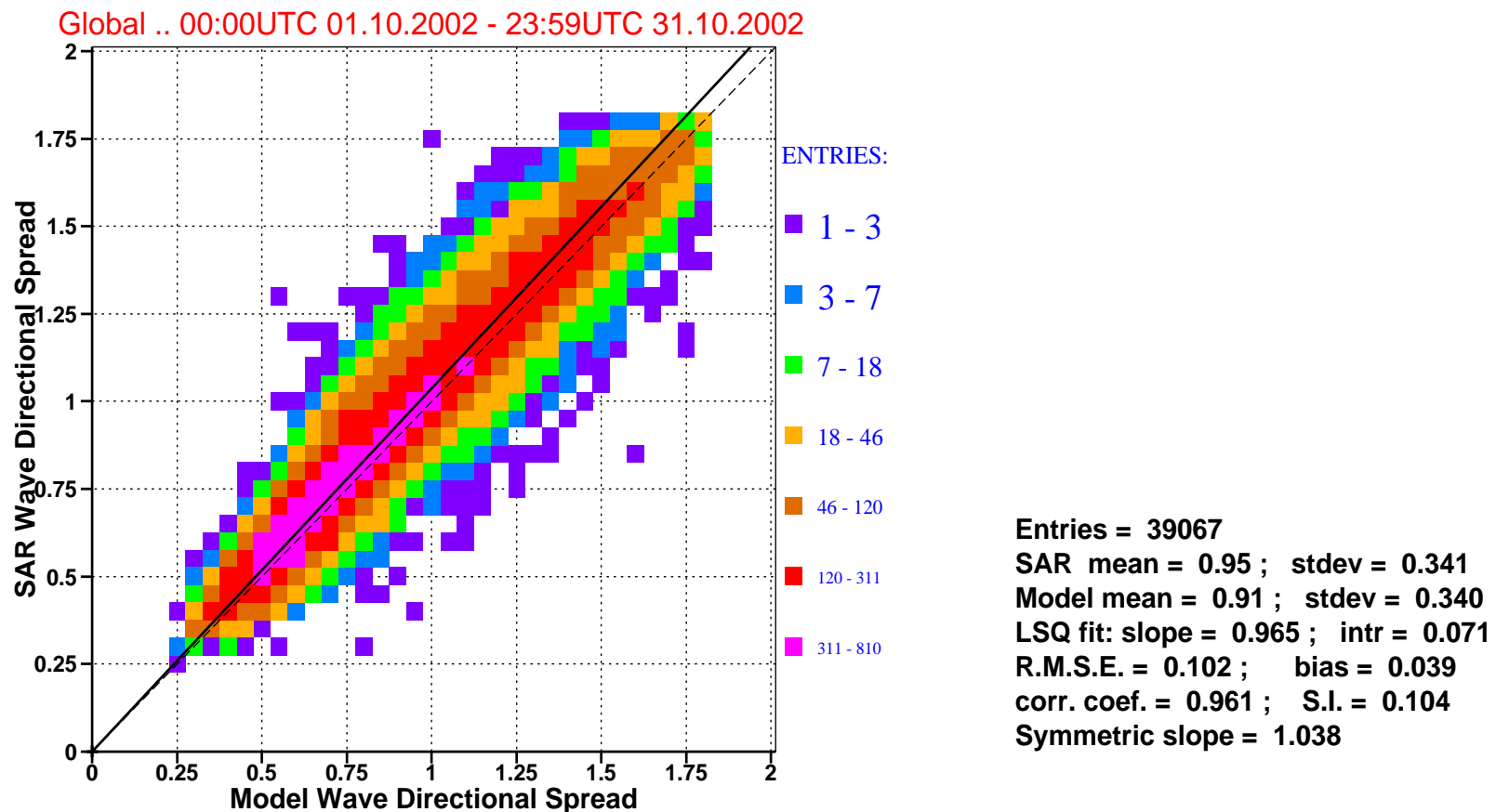
Figure 8: Comparison of ECMWF wave directional spread with that of ERS-2 SAR for october 2002 (global).
