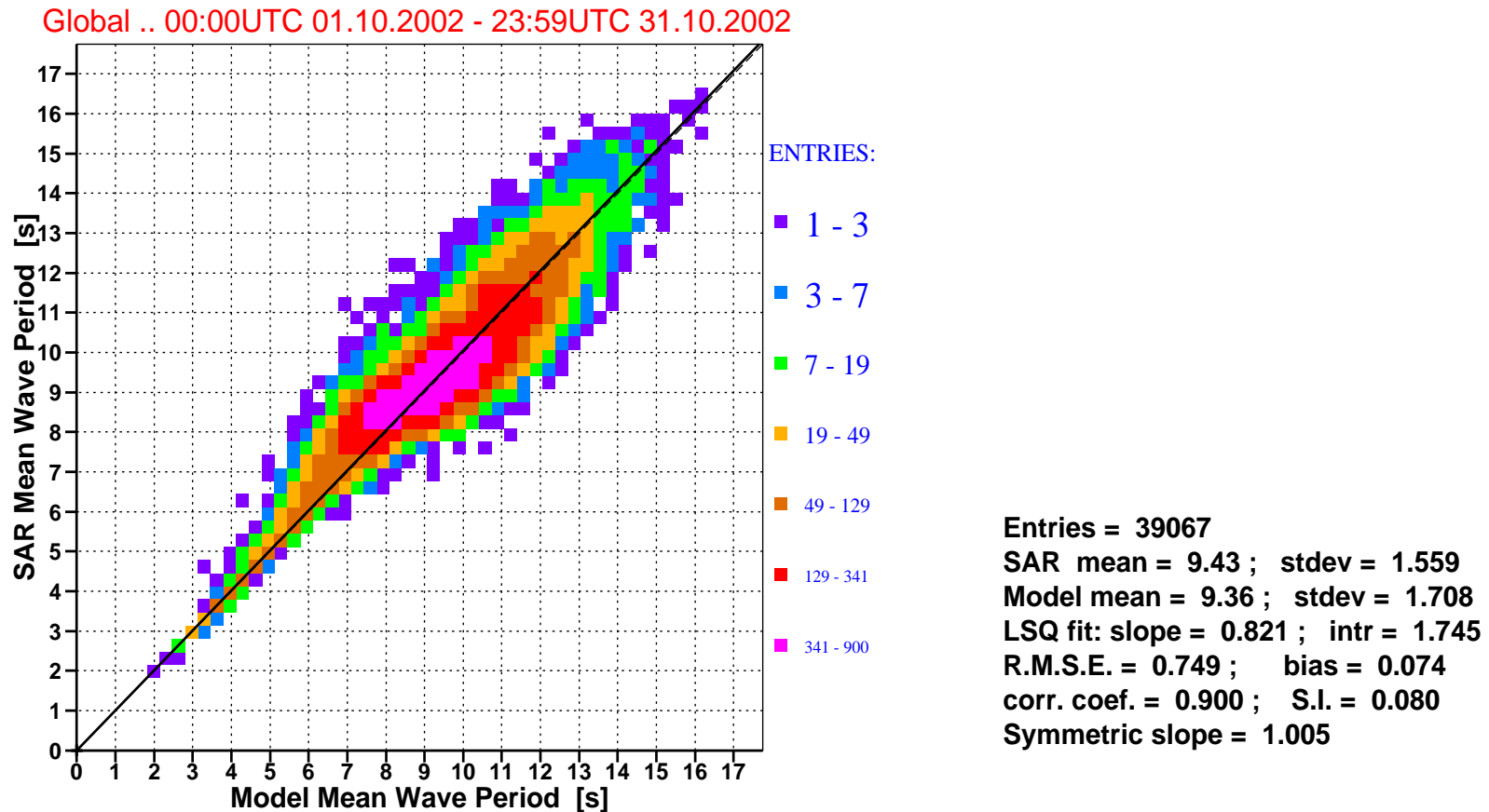
Figure 7: Comparison of ECMWF mean wave periods with ERS-2 SAR mean wave periods for october 2002 (global).
