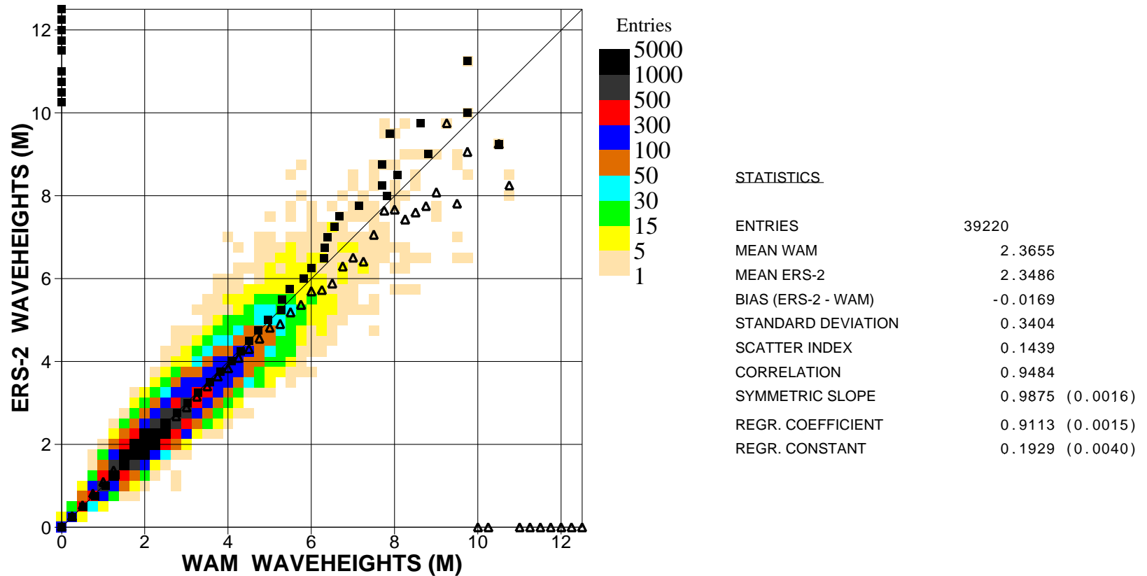
Figure 2: Comparison of ECMWF wave height results with ERS2 SAR wave height data for October 2002 (global)
