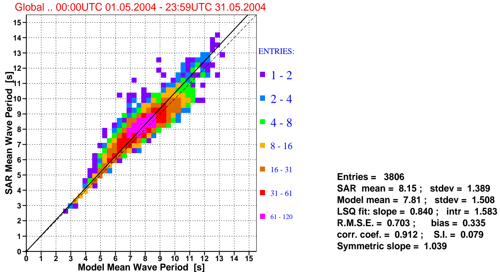
Figure 7: Comparison of ECMWF mean wave periods with ERS-2 SAR mean wave periods for may 2004 (global).
