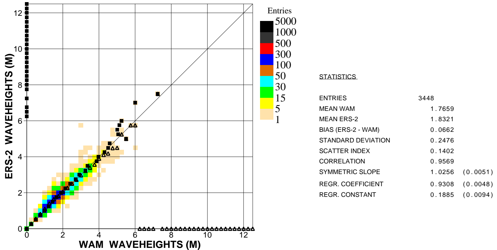
Figure 3: Comparison of ECMWF wave height results with ERS2 SAR wave height data for May 2004 (n.hem.)
