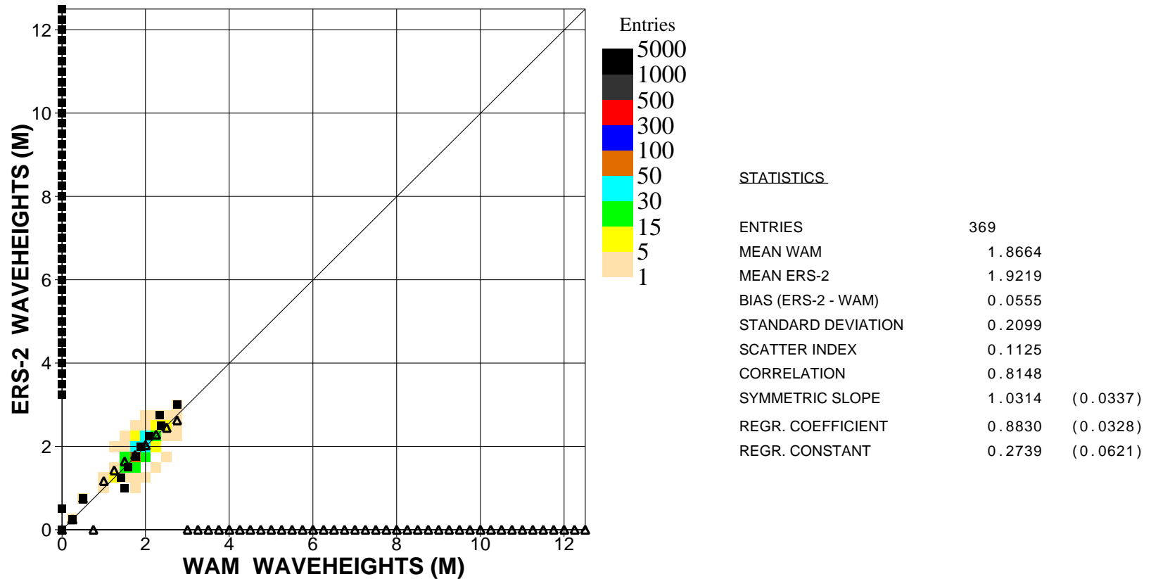
Figure 4: Comparison of ECMWF wave height results with ERS2 SAR wave height data for May 2004 (tropics)
