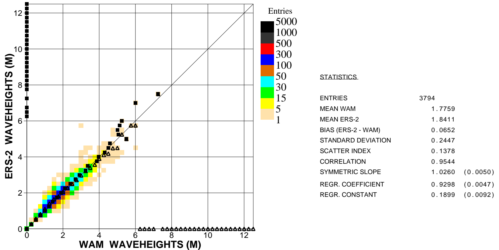
Figure 2: Comparison of ECMWF wave height results with ERS2 SAR wave height data for May 2004 (global)
