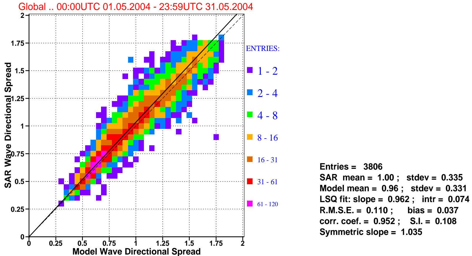
Figure 8: Comparison of ECMWF wave directional spread with that of ERS-2 SAR for may 2004 (global).
