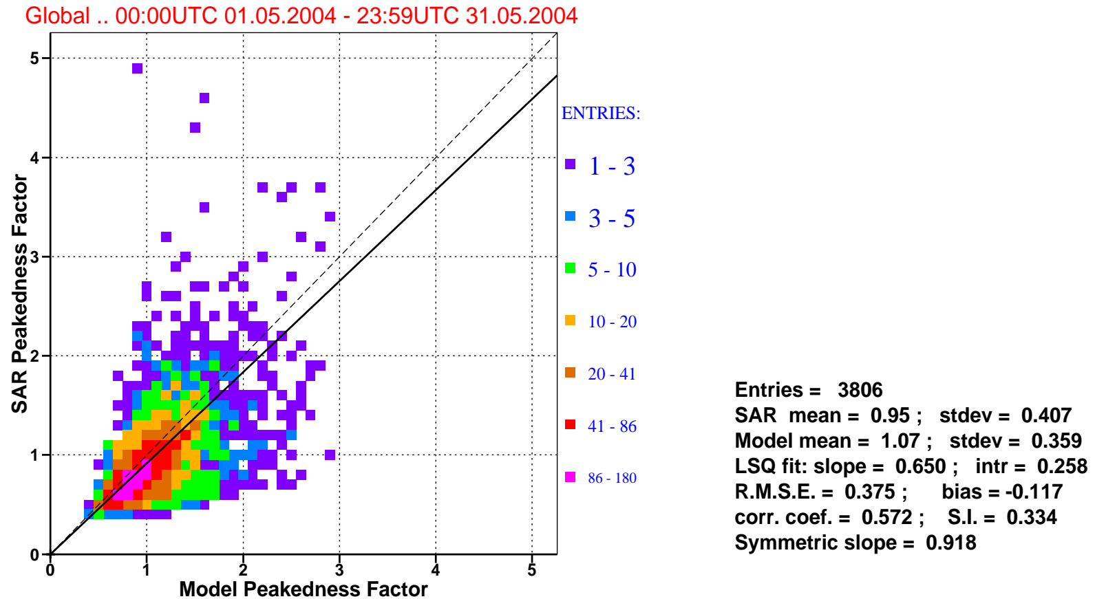
Figure 10: : Comparison of ECMWF wave peakedness factor with that of ERS-2 SAR for may 2004 (global).
