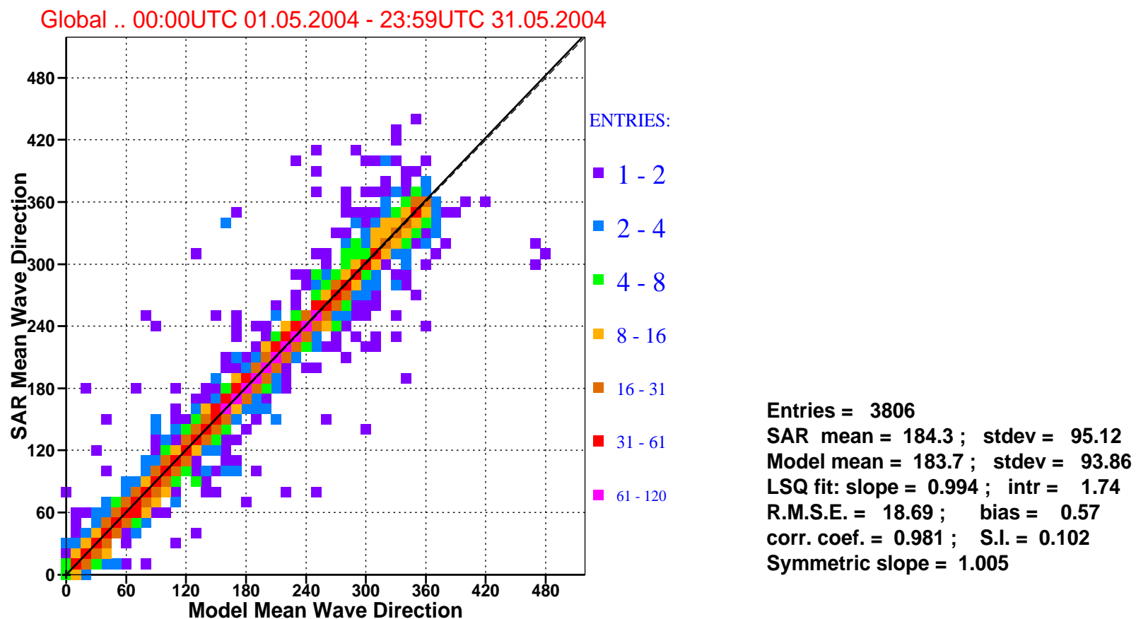
Figure 9: Comparison of ECMWF mean wave directions with that of ERS-2 SAR for may 2004 (global).
