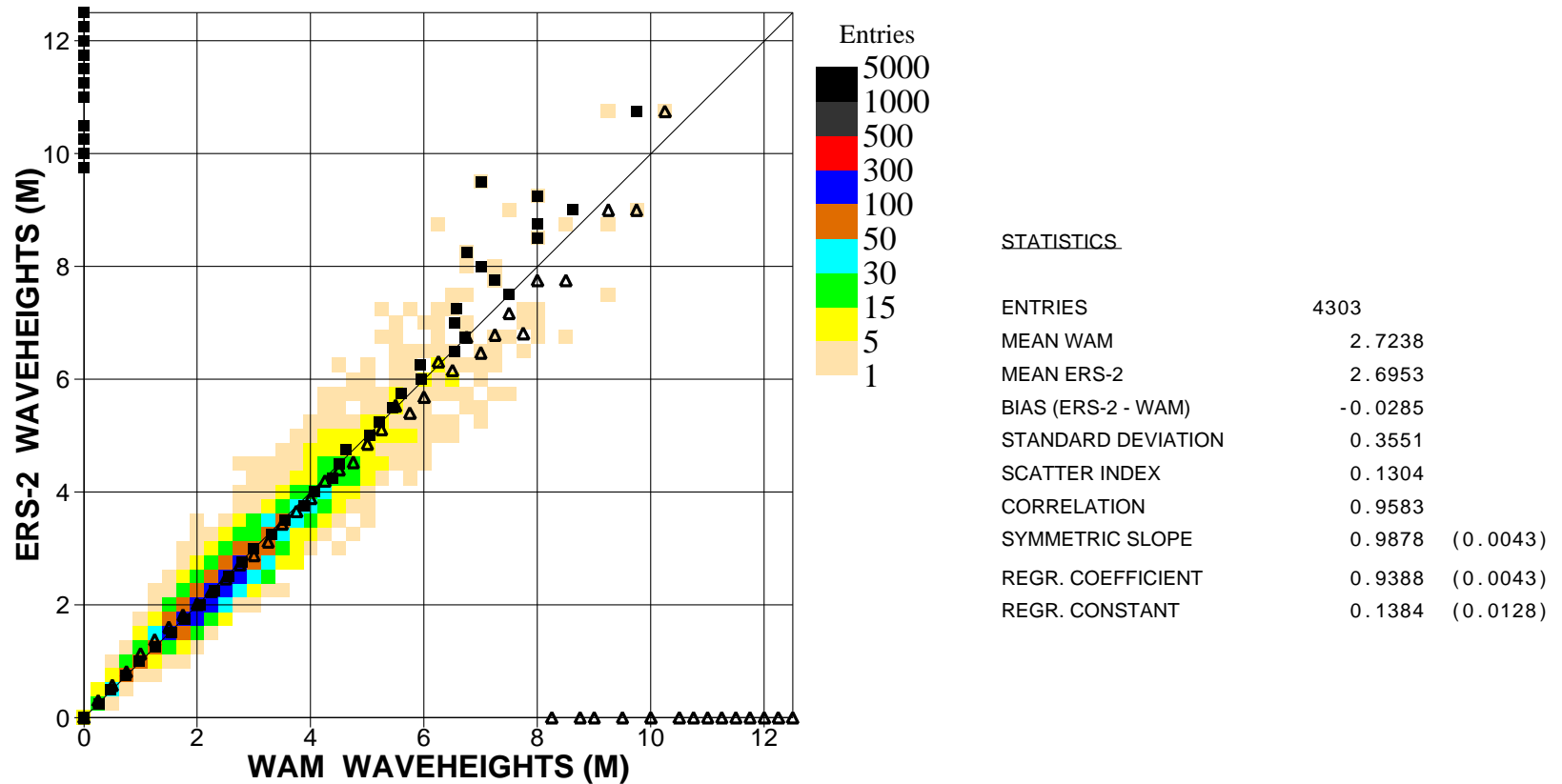
Figure 2: Comparison of ECMWF wave height results with ERS2 SAR wave height data for March 2004 (global)
