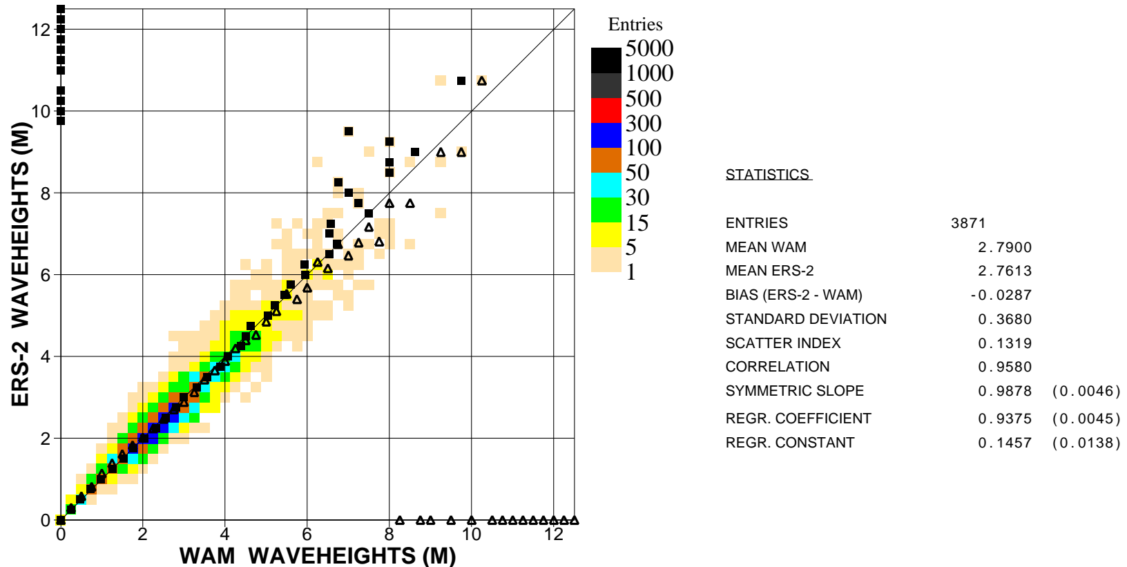
Figure 3: Comparison of ECMWF wave height results with ERS2 SAR wave height data for March 2004 (n.hem.)
