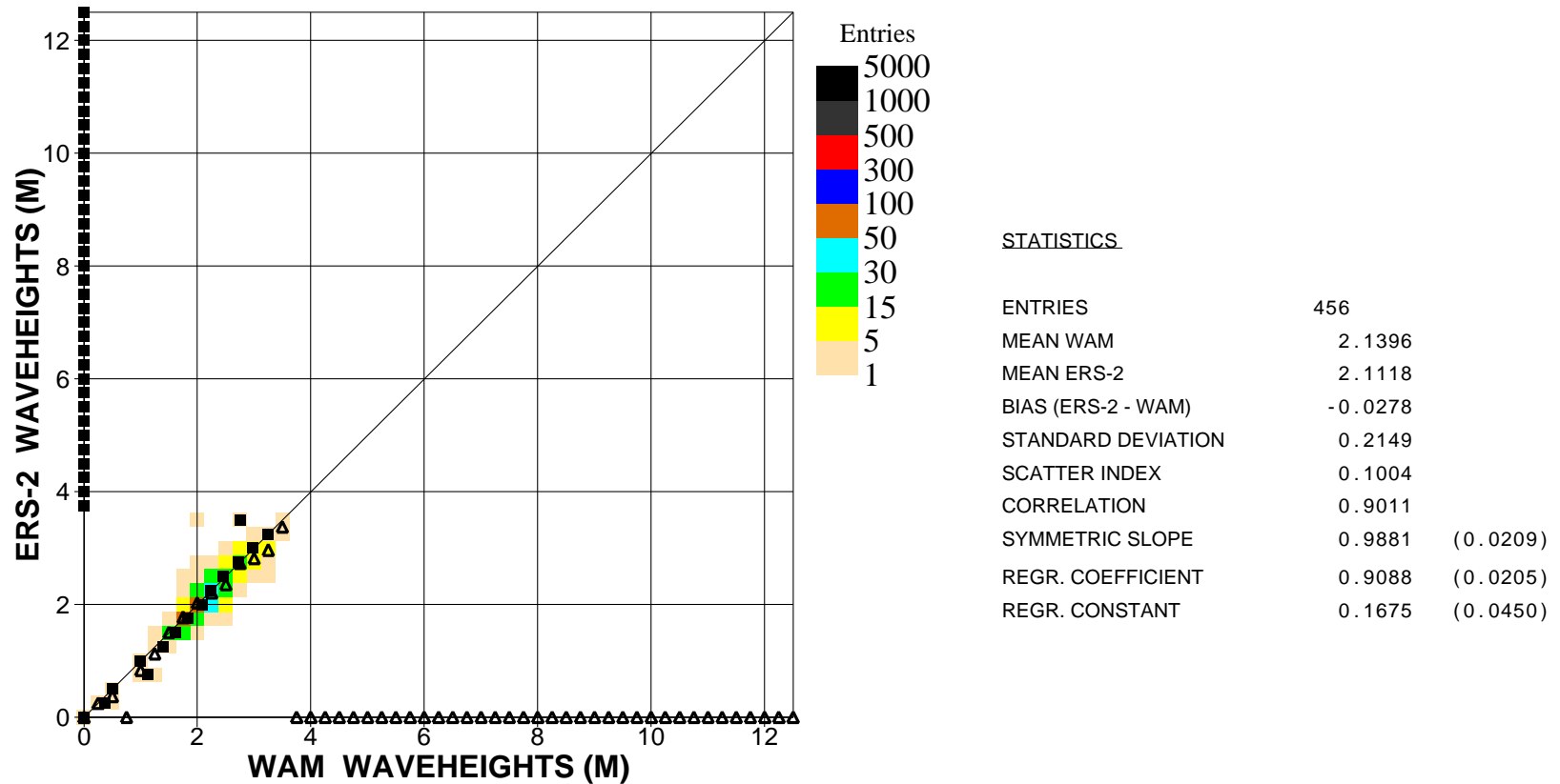
Figure 4: Comparison of ECMWF wave height results with ERS2 SAR wave height data for March 2004 (tropics)
