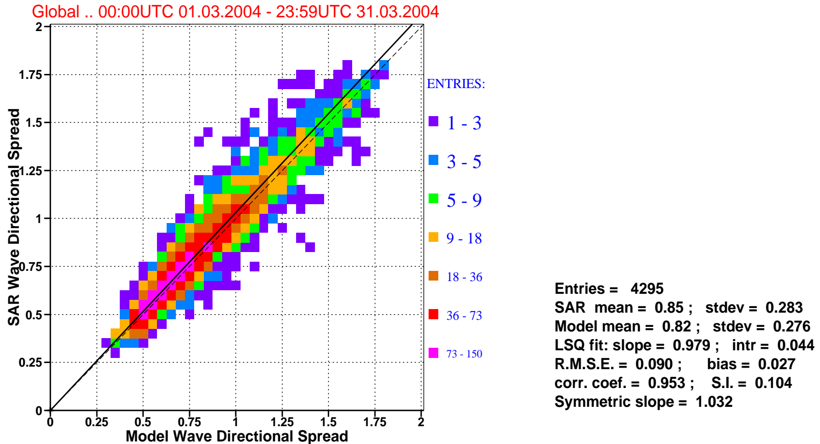
Figure 8: Comparison of ECMWF wave directional spread with that of ERS-2 SAR for march 2004 (global).
