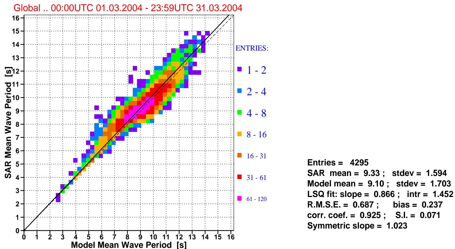
Figure 7: Comparison of ECMWF mean wave periods with ERS-2 SAR mean wave periods for march 2004 (global).
