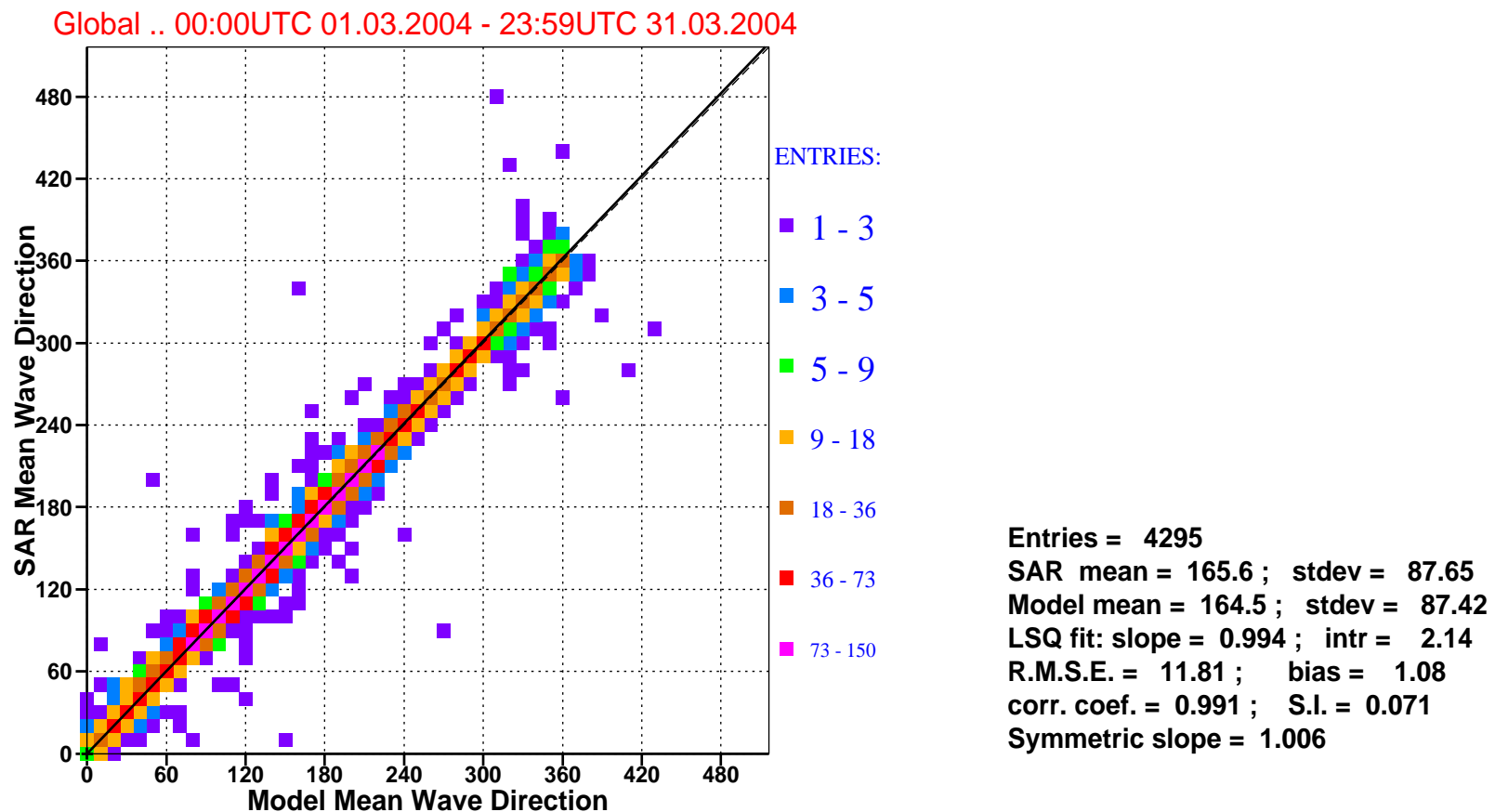
Figure 9: Comparison of ECMWF mean wave directions with that of ERS-2 SAR for march 2004 (global).
