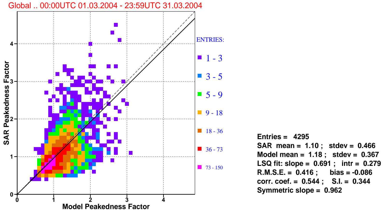
Figure 10: : Comparison of ECMWF wave peakedness factor with that of ERS-2 SAR for march 2004 (global).
