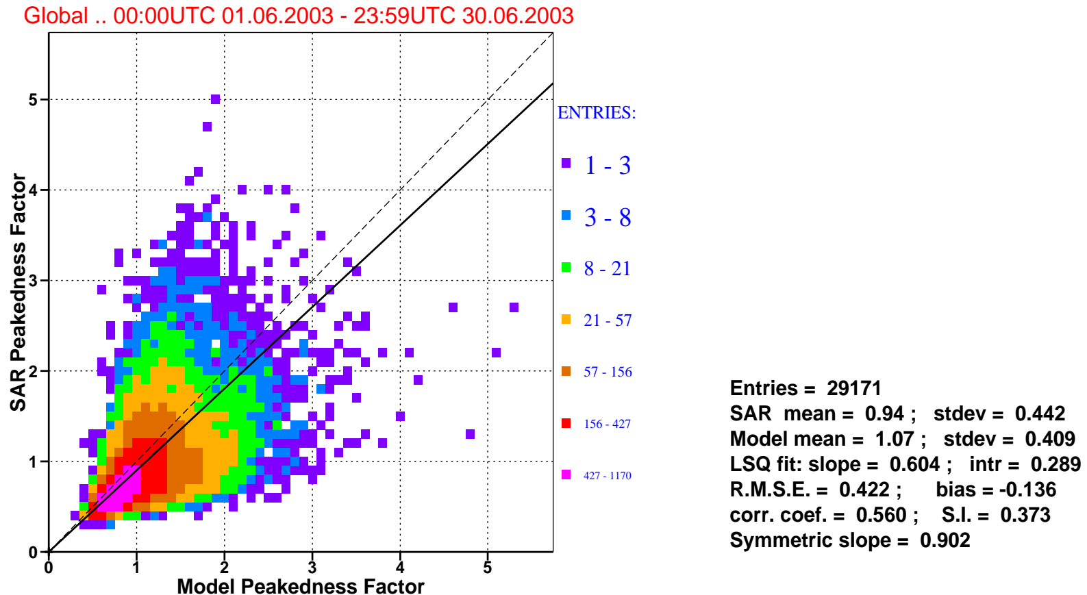
Figure 10: : Comparison of ECMWF wave peakedness factor with that of ERS-2 SAR for june 2003 (global).
