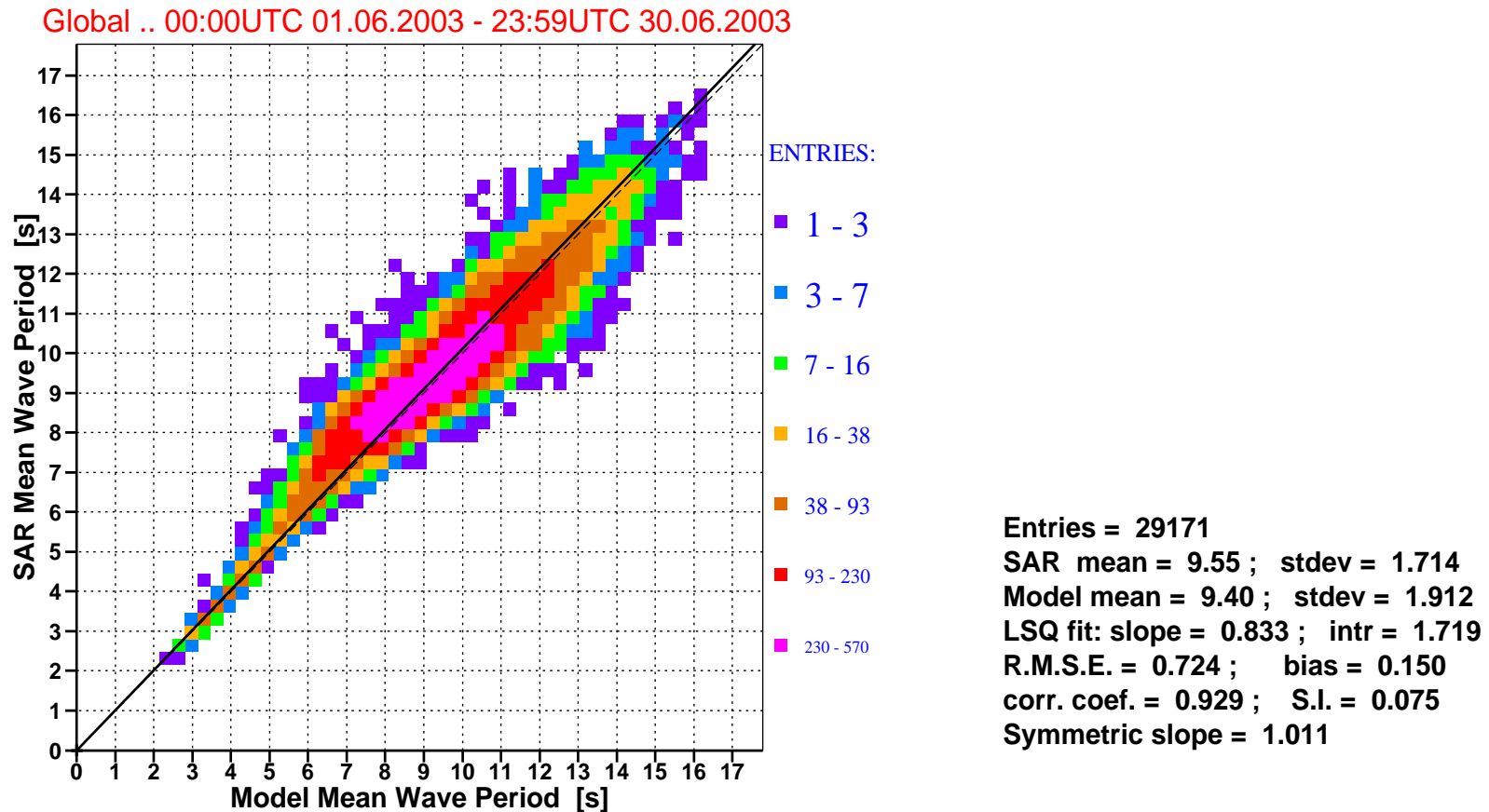
Figure 7: Comparison of ECMWF mean wave periods with ERS-2 SAR mean wave periods for June 2003 (global).
