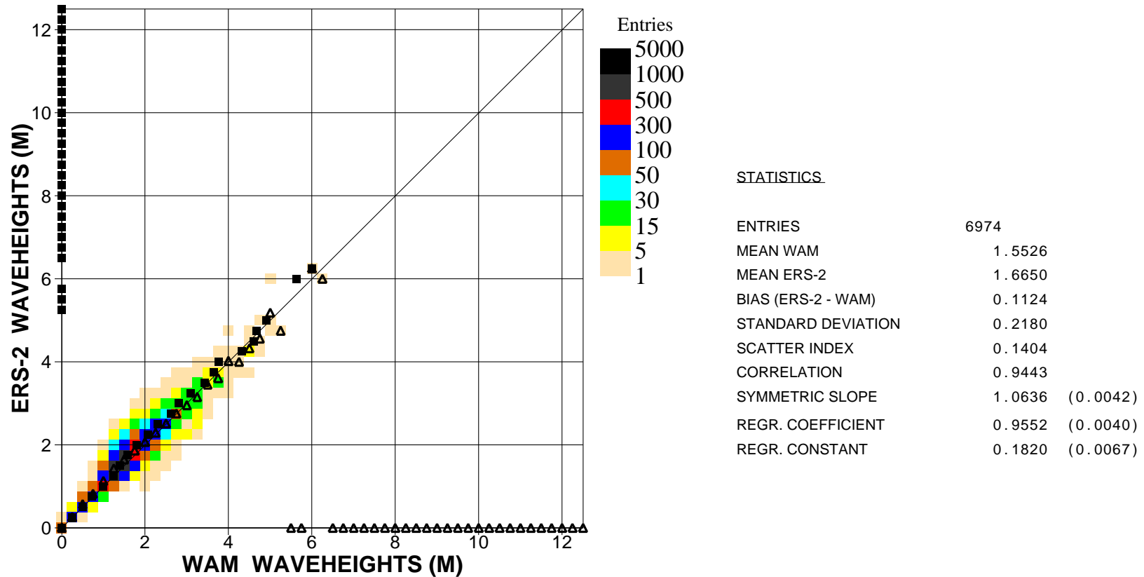
Figure 3: Comparison of ECMWF wave height results with ERS2 SAR wave height data for June 2003 (n.hem.)
