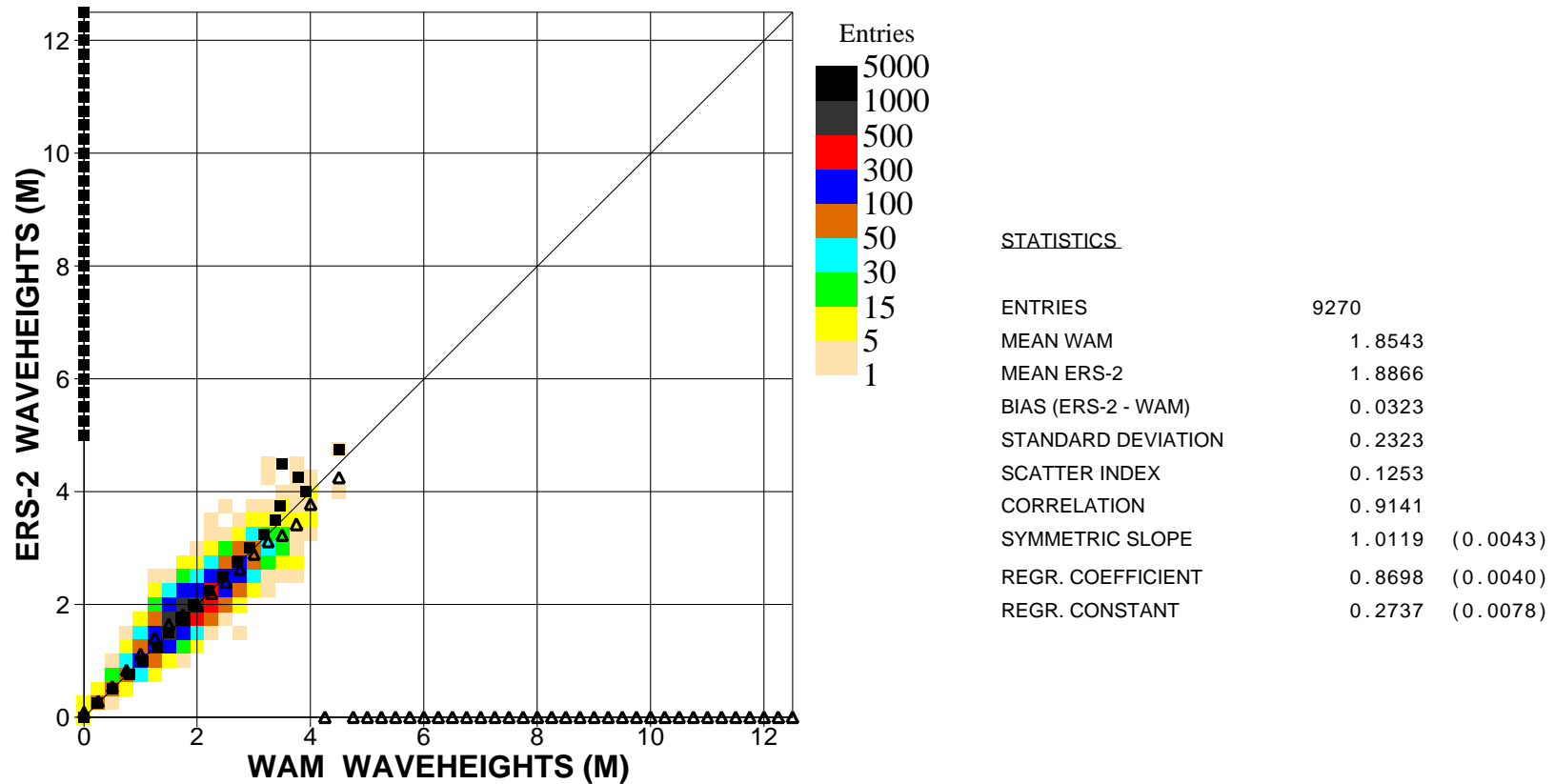
Figure 4: Comparison of ECMWF wave height results with ERS2 SAR wave height data for June 2003 (tropics)
