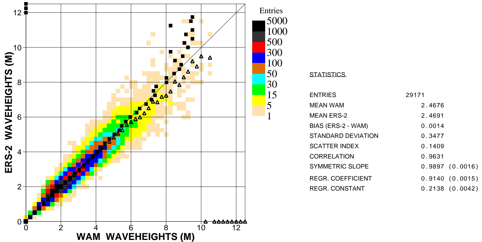
Figure 2: Comparison of ECMWF wave height results with ERS2 SAR wave height data for June 2003 (global)
