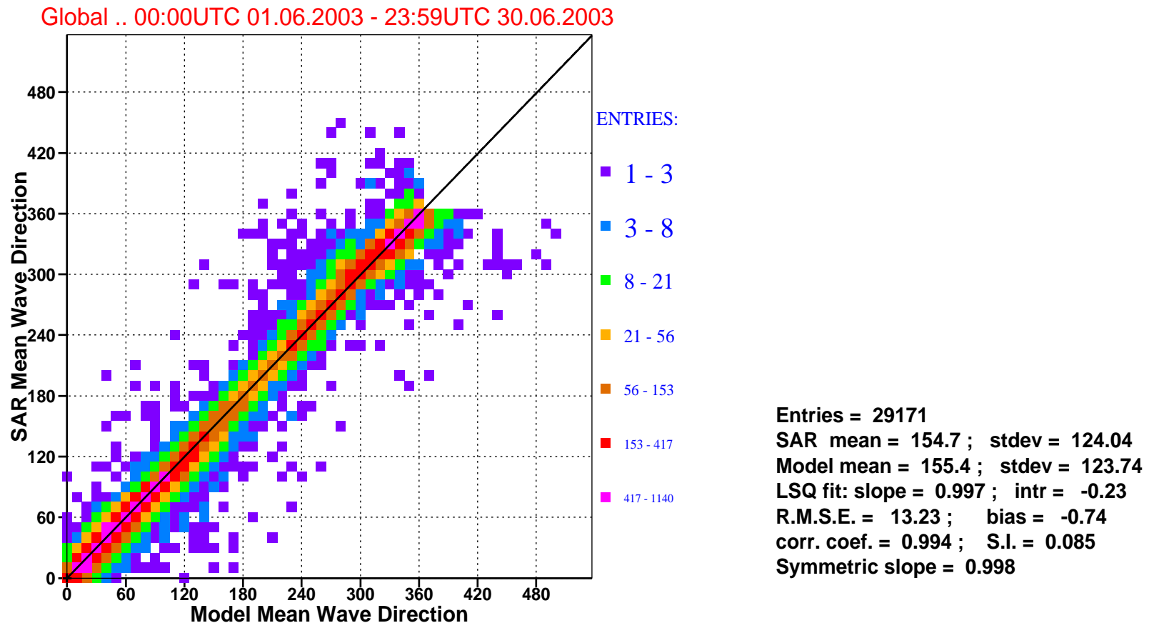
Figure 9: Comparison of ECMWF mean wave directions with that of ERS-2 SAR for June 2003 (global).
