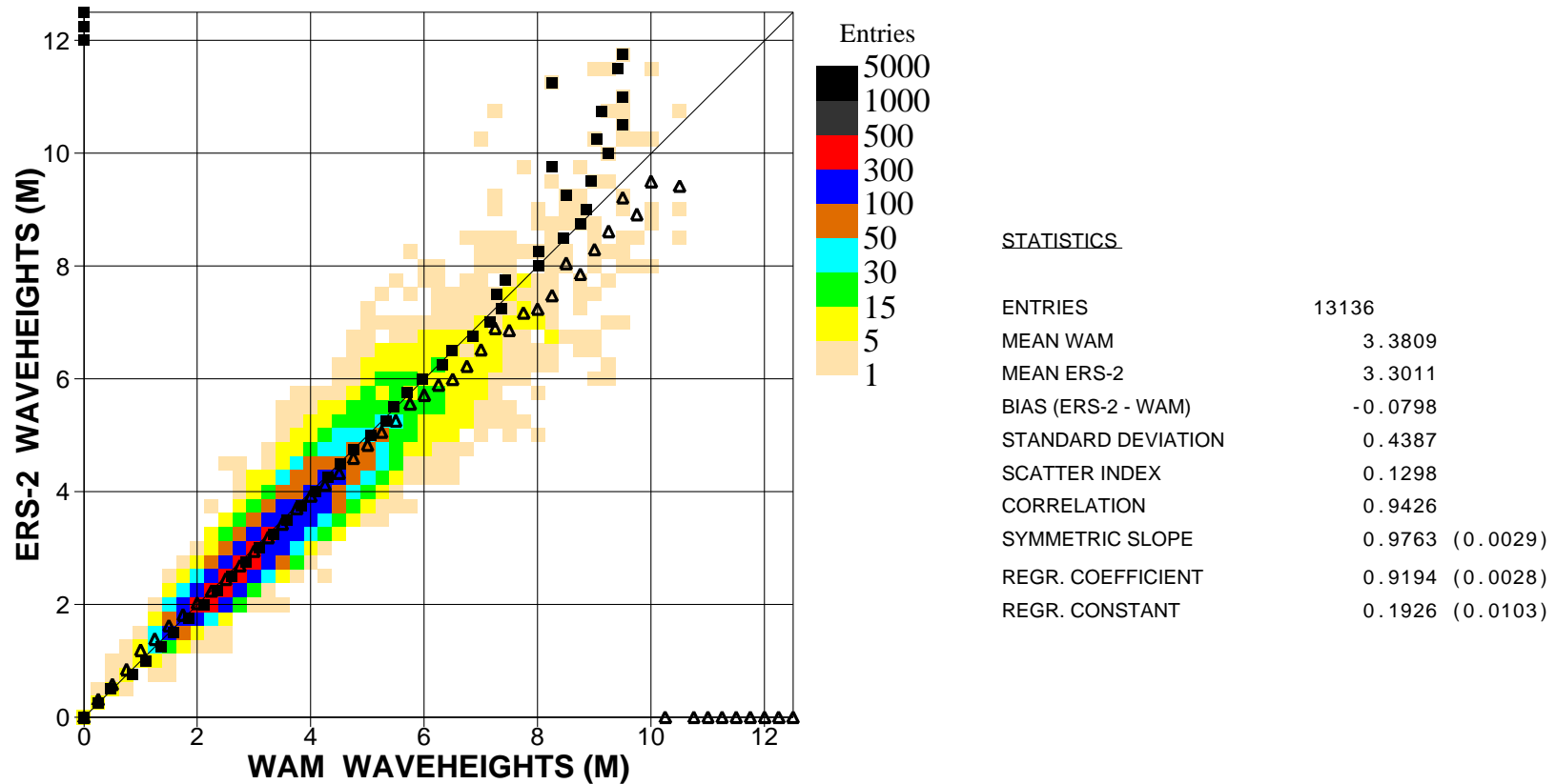
Figure 5: Comparison of ECMWF wave height results with ERS2 SAR wave height data for June 2003 (s.hem.)
