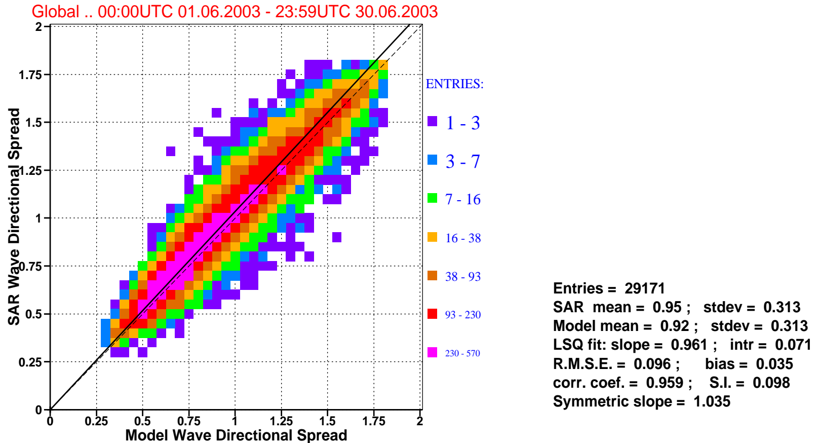
Figure 8: Comparison of ECMWF wave directional spread with that of ERS-2 SAR for june 2003 (global).
