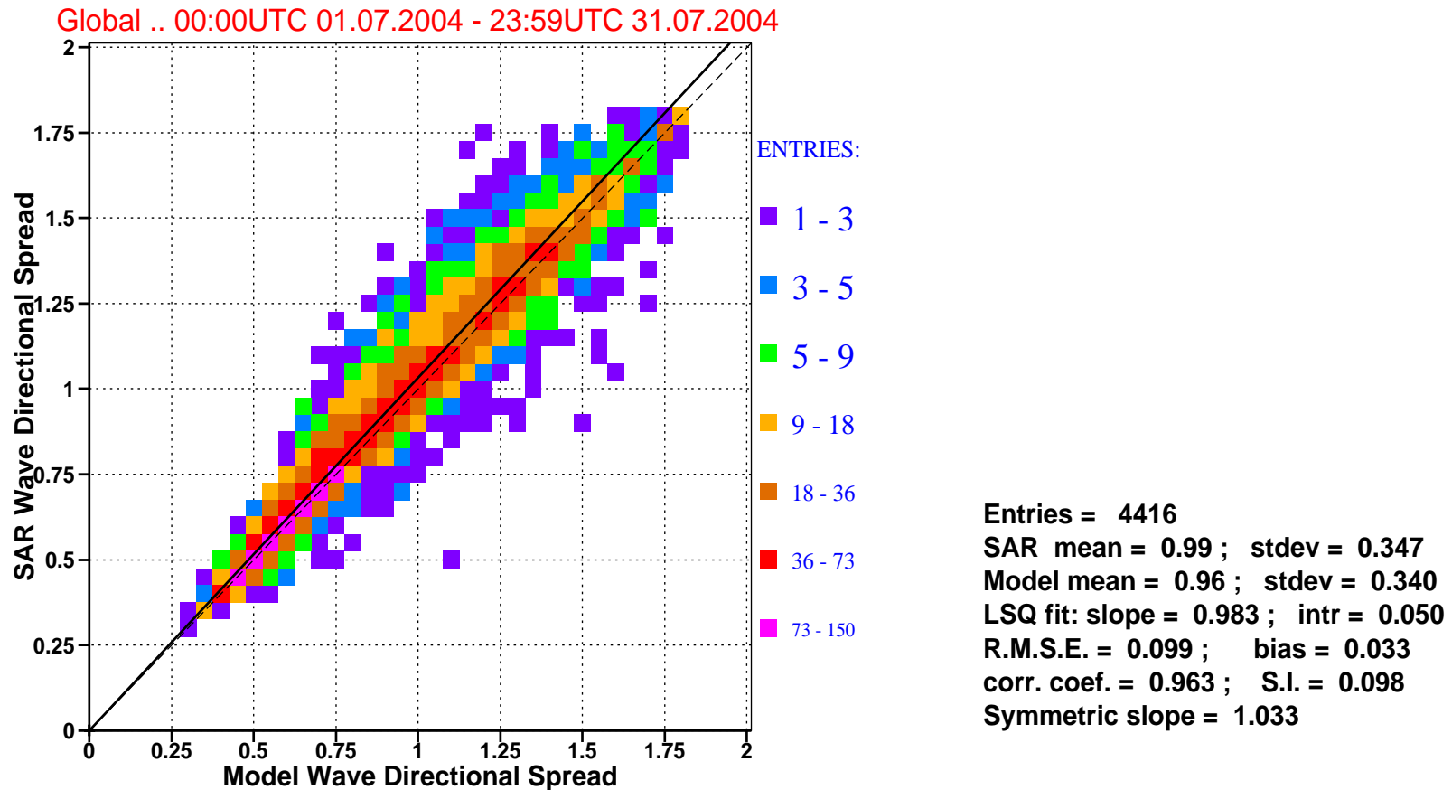
Figure 8: Comparison of ECMWF wave directional spread with that of ERS-2 SAR for July 2004 (global).
