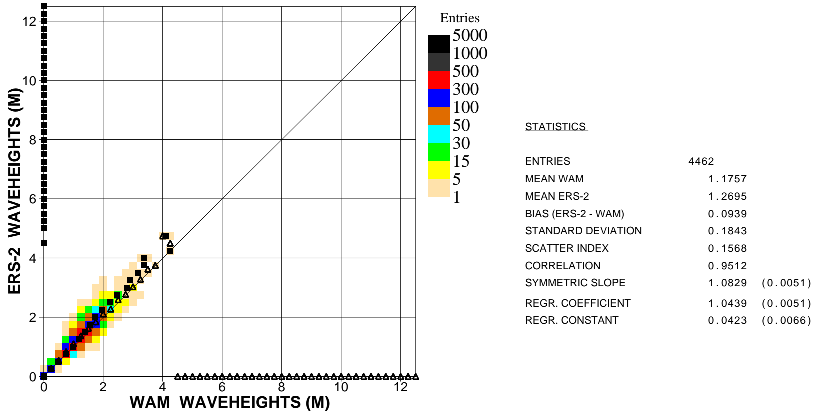
Figure 2: Comparison of ECMWF wave height results with ERS2 SAR wave height data for July 2004 (global)
