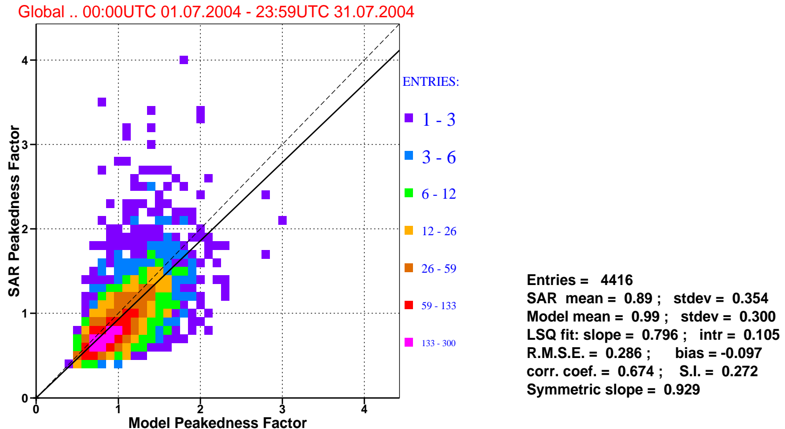
Figure 10: : Comparison of ECMWF wave peakedness factor with that of ERS-2 SAR for July 2004 (global).
