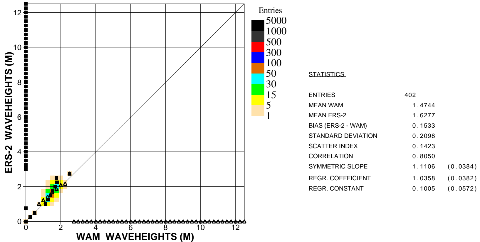
Figure 4: Comparison of ECMWF wave height results with ERS2 SAR wave height data for July 2004 (tropics)
