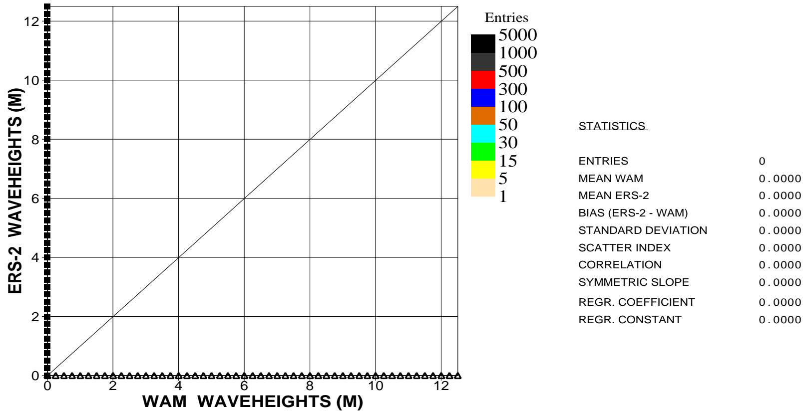
Figure 5: Comparison of ECMWF wave height results with ERS2 SAR wave height data for July 2004 (s.hem.)
