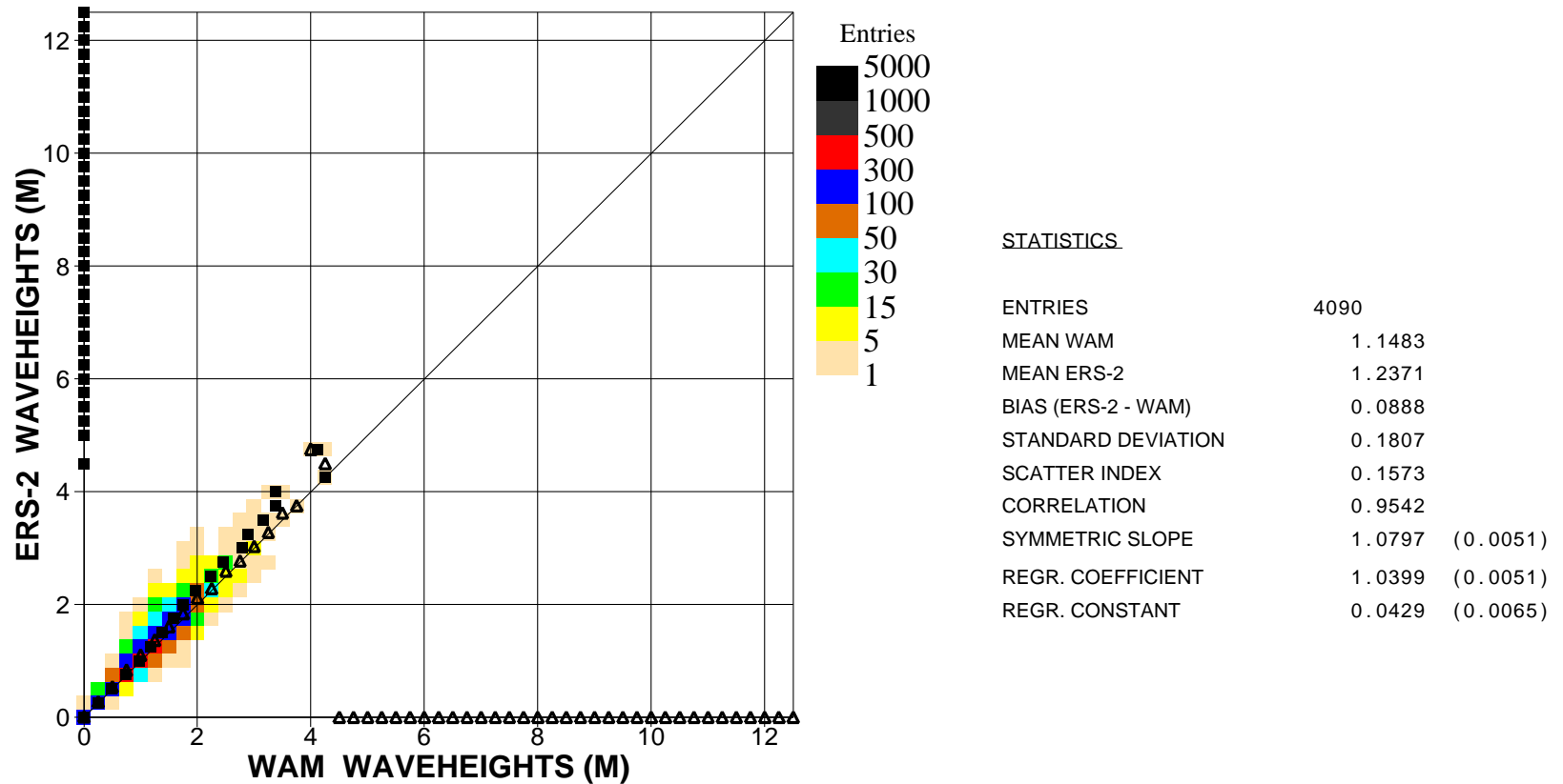
Figure 3: Comparison of ECMWF wave height results with ERS2 SAR wave height data for July 2004 (n.hem.)
