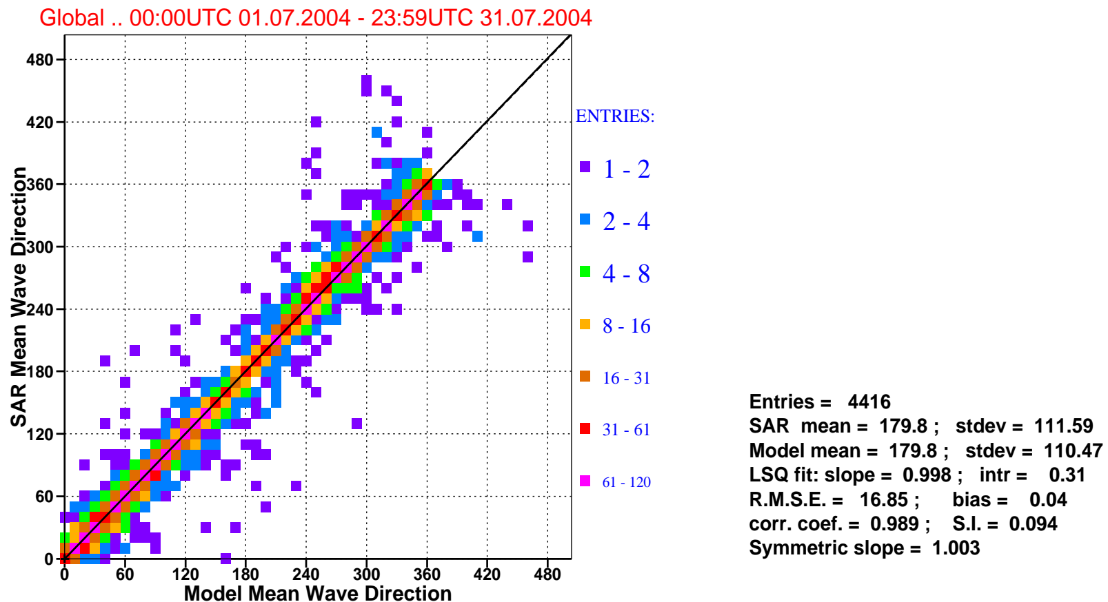
Figure 9: Comparison of ECMWF mean wave directions with that of ERS-2 SAR for July 2004 (global).
