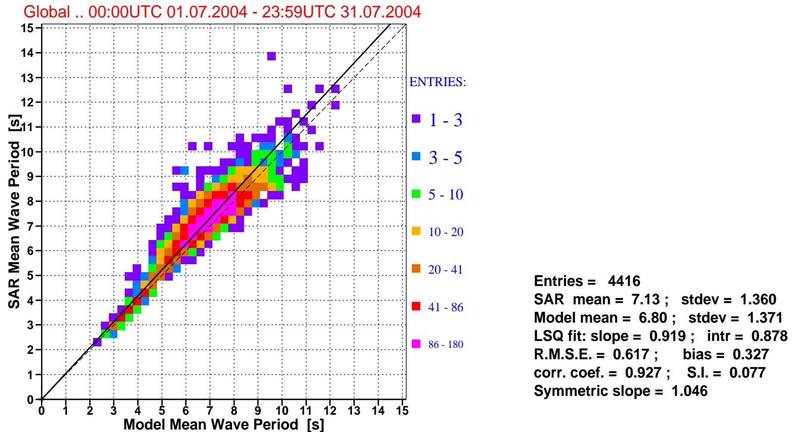
Figure 7: Comparison of ECMWF mean wave periods with ERS-2 SAR mean wave periods for July 2004 (global).
