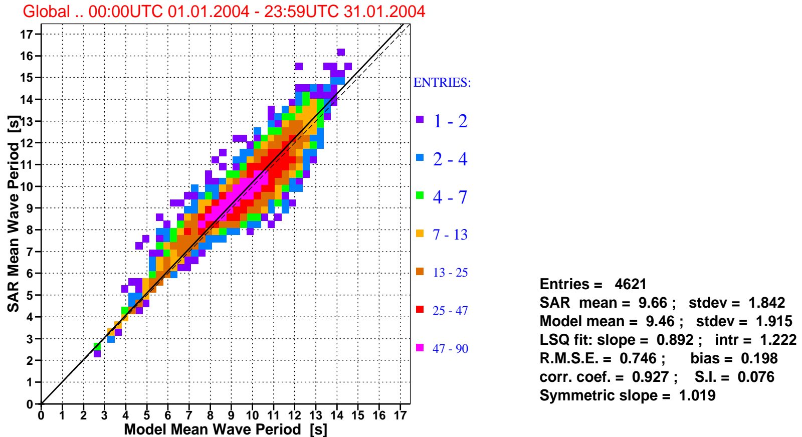
Figure 7: Comparison of ECMWF mean wave periods with ERS-2 SAR mean wave periods for January 2004 (global).
