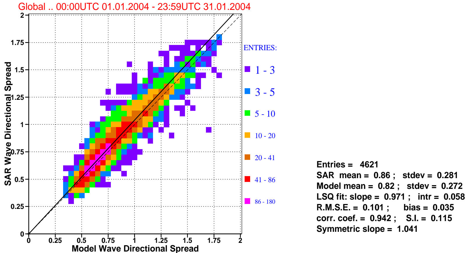
Figure 8: Comparison of ECMWF wave directional spread with that of ERS-2 SAR for January 2004 (global).
