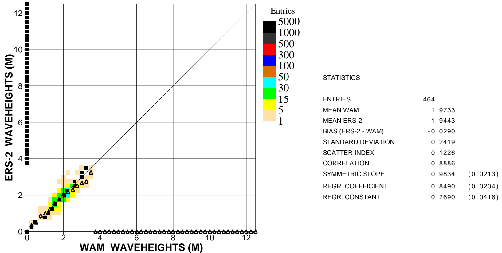
Figure 4: Comparison of ECMWF wave height results with ERS2 SAR wave height data for January 2004 (tropics)
