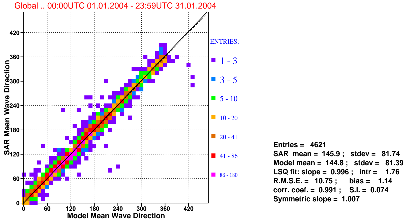
Figure 9: Comparison of ECMWF mean wave directions with that of ERS-2 SAR for January 2004 (global).
