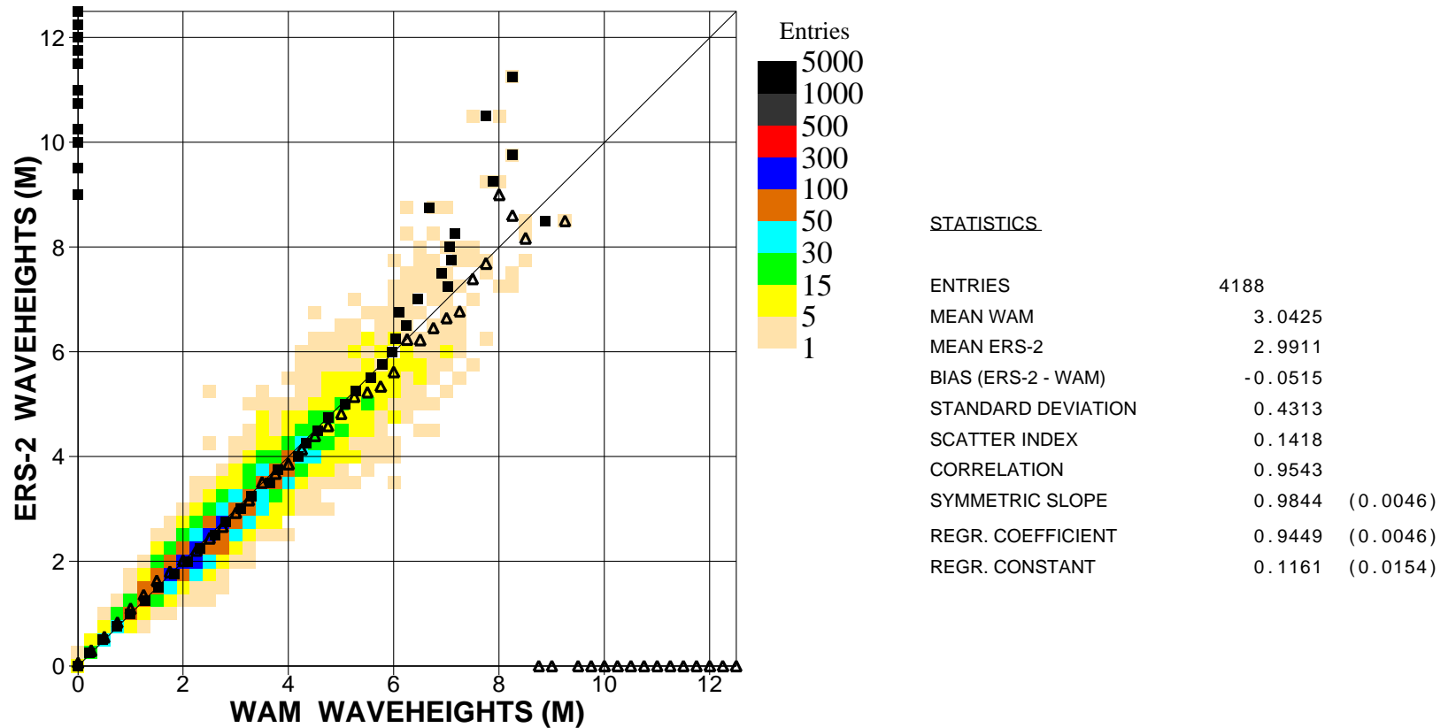
Figure 3: Comparison of ECMWF wave height results with ERS2 SAR wave height data for January 2004 (n.hem.)
