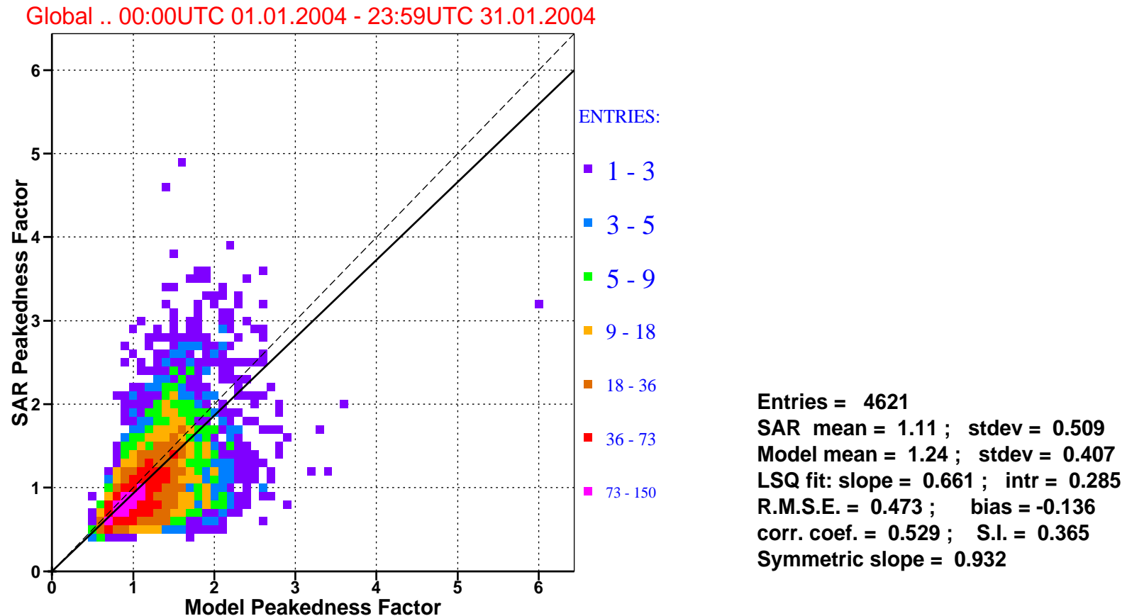
Figure 10: : Comparison of ECMWF wave peakedness factor with that of ERS-2 SAR for january 2004 (global).
