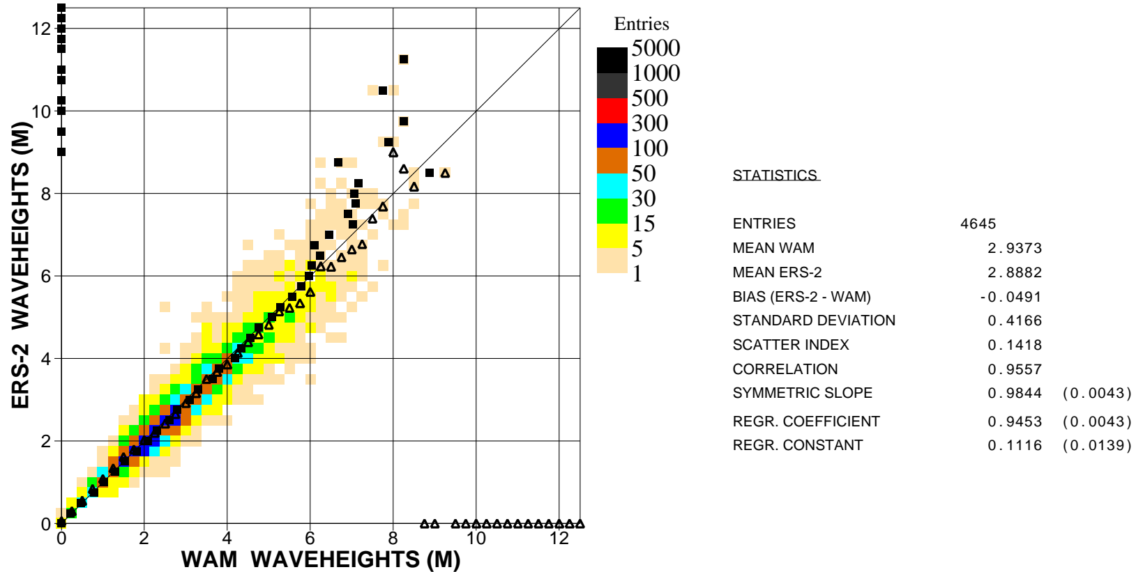
Figure 2: Comparison of ECMWF wave height results with ERS2 SAR wave height data for January 2004 (global)
