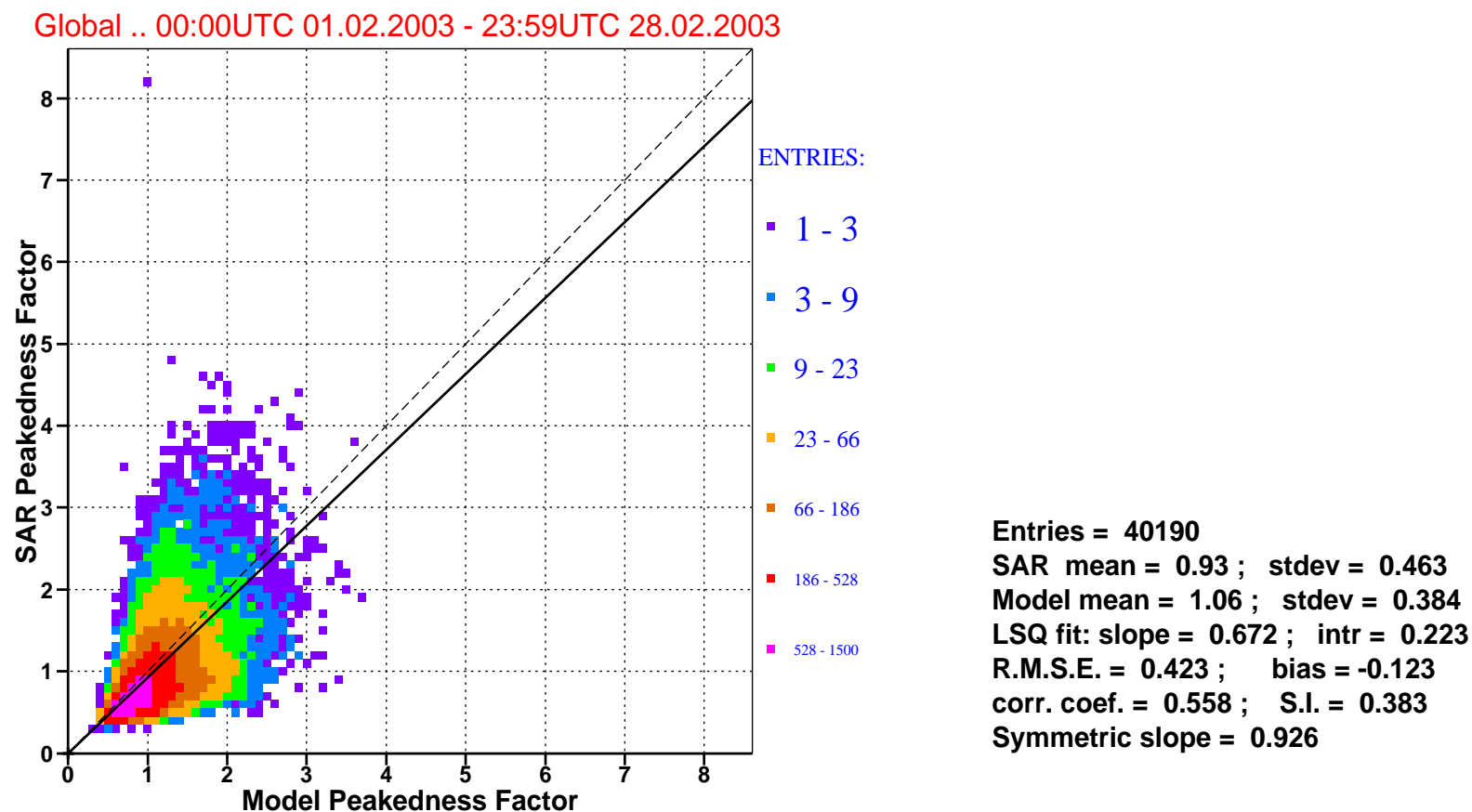
Figure 10: : Comparison of ECMWF wave peakedness factor with that of ERS-2 SAR for february 2003 (global).
