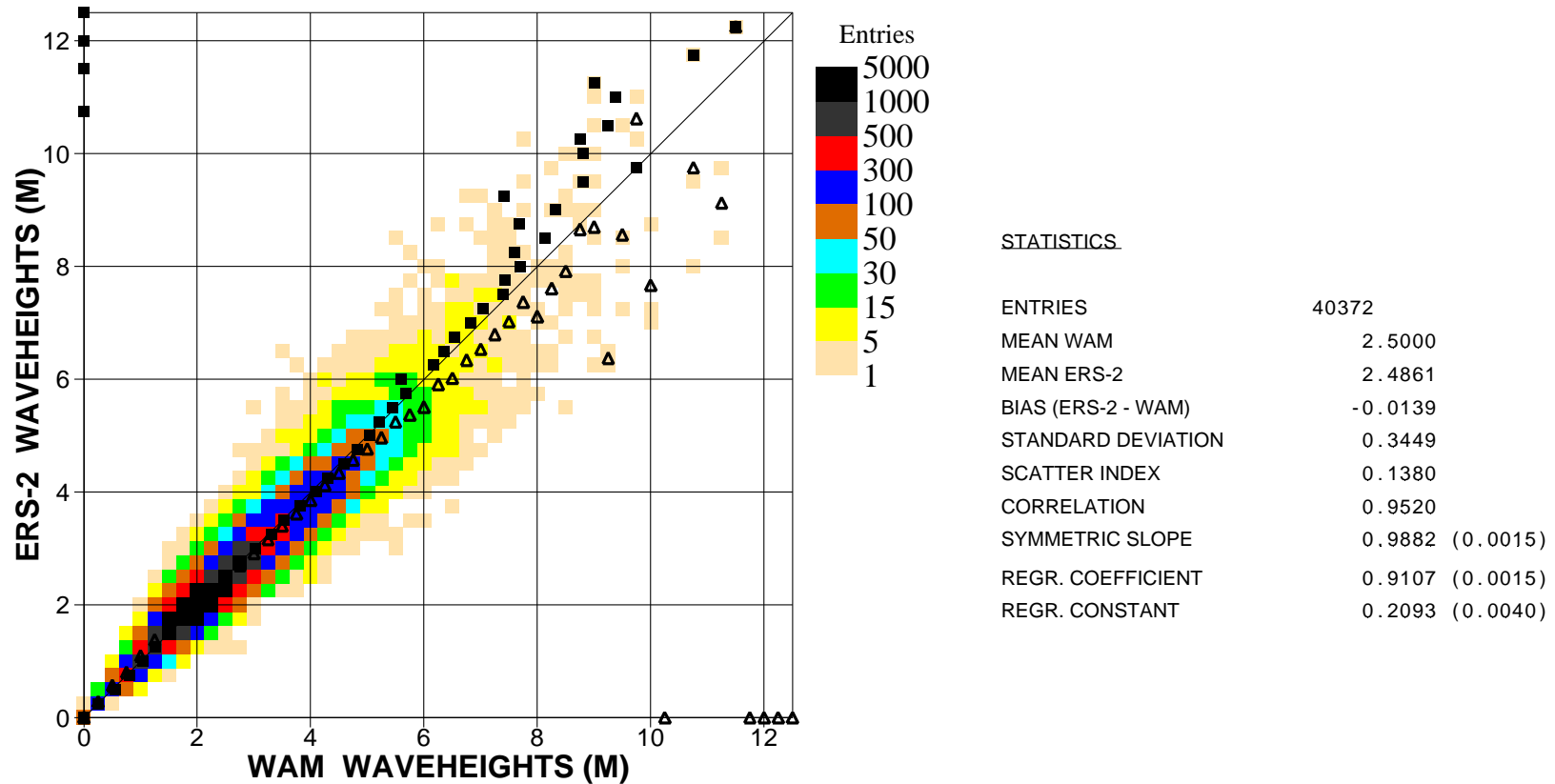
Figure 2: Comparison of ECMWF wave height results with ERS2 SAR wave height data for February 2003 (global)
