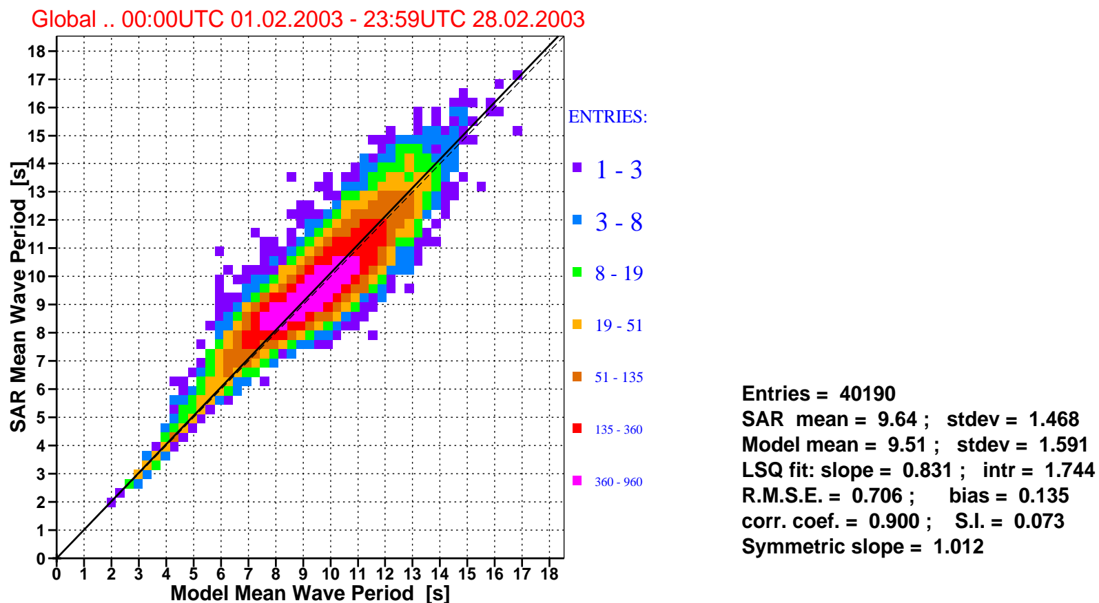
Figure 7: Comparison of ECMWF mean wave periods with ERS-2 SAR mean wave periods for february 2003 (global).
