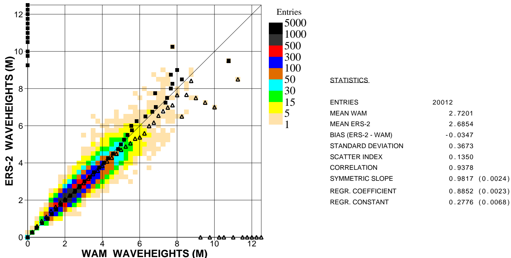
Figure 5: Comparison of ECMWF wave height results with ERS2 SAR wave height data for February 2003 (s.hem.)
