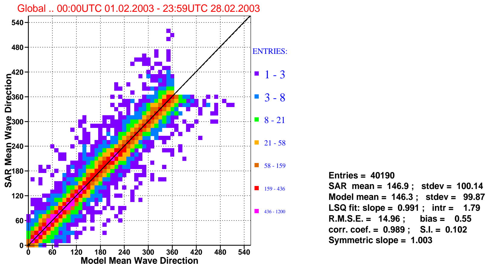
Figure 9: Comparison of ECMWF mean wave directions with that of ERS-2 SAR for february 2003 (global).
