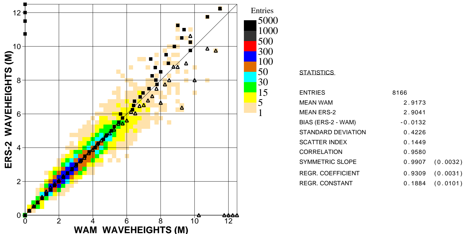
Figure 3: Comparison of ECMWF wave height results with ERS2 SAR wave height data for February 2003 (n.hem.)
