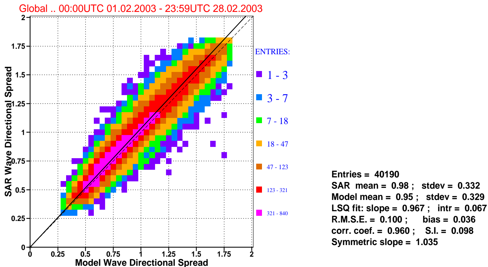
Figure 8: Comparison of ECMWF wave directional spread with that of ERS-2 SAR for february 2003 (global).
