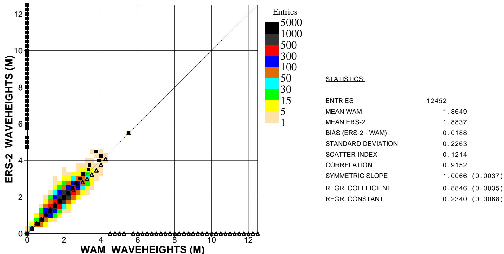
Figure 4: Comparison of ECMWF wave height results with ERS2 SAR wave height data for February 2003 (tropics)
