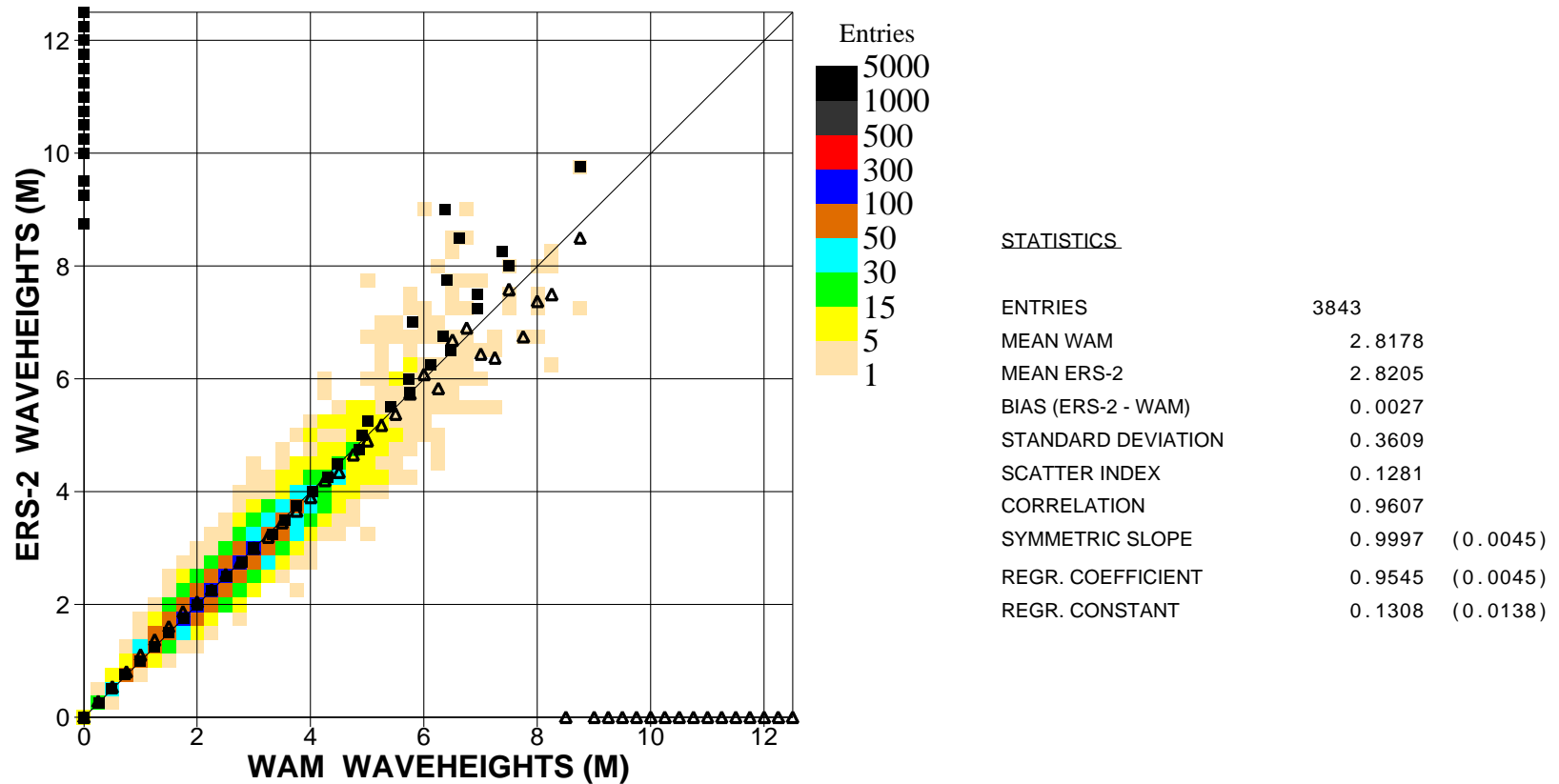
Figure 3: Comparison of ECMWF wave height results with ERS2 SAR wave height data for December 2003 (n.hem.)
