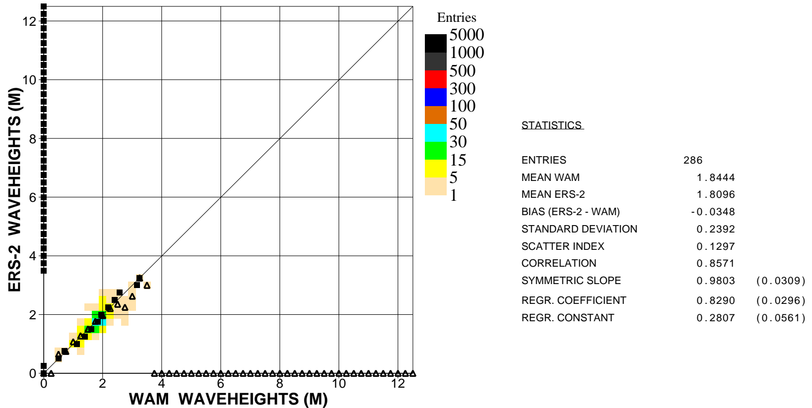
Figure 4: Comparison of ECMWF wave height results with ERS2 SAR wave height data for December 2003 (tropics)
