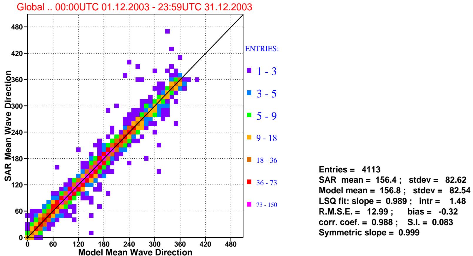
Figure 9: Comparison of ECMWF mean wave directions with that of ERS-2 SAR for decemeber 2003 (global).
