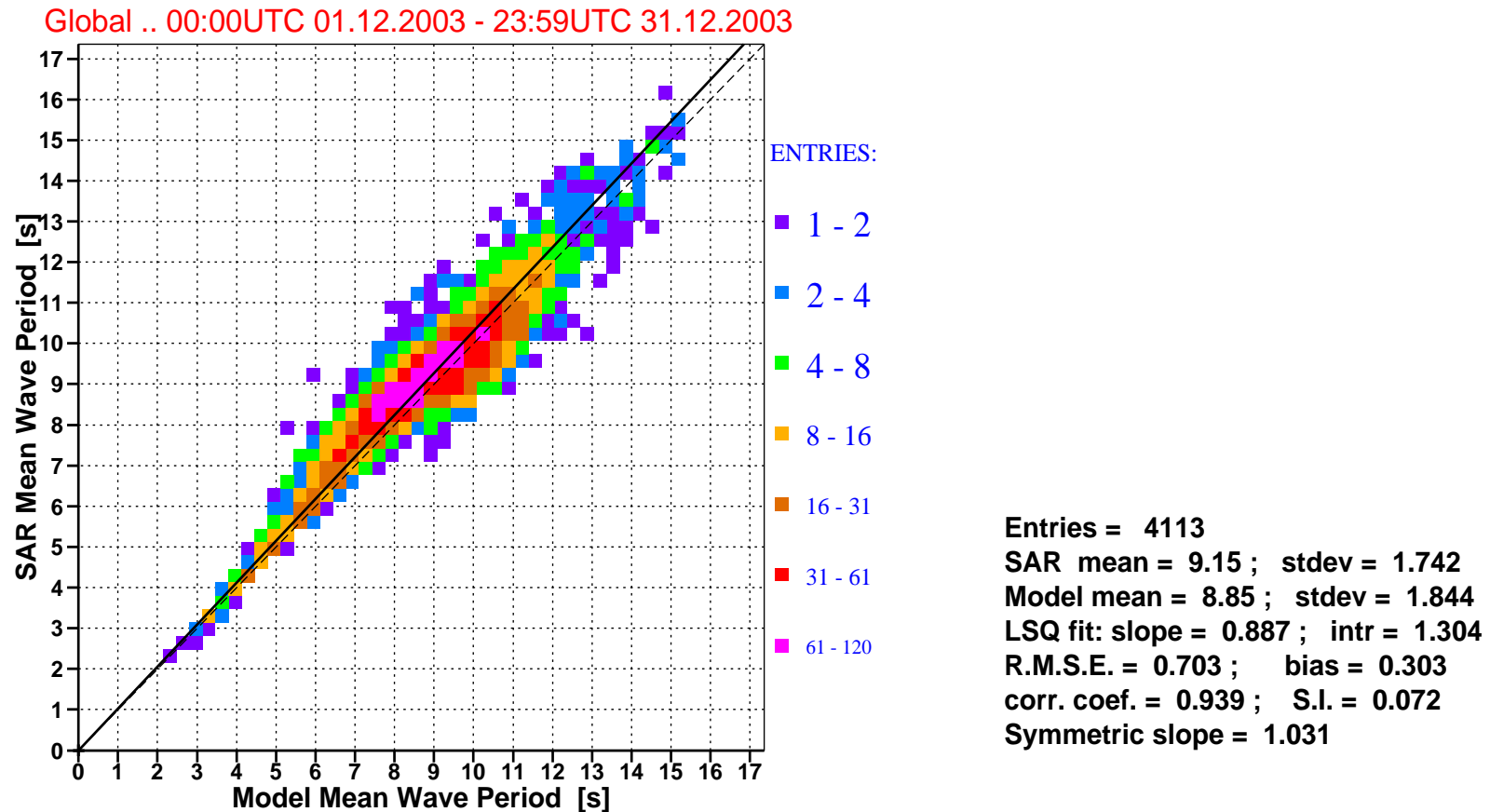
Figure 7: Comparison of ECMWF mean wave periods with ERS-2 SAR mean wave periods for decemeber 2003 (global).
