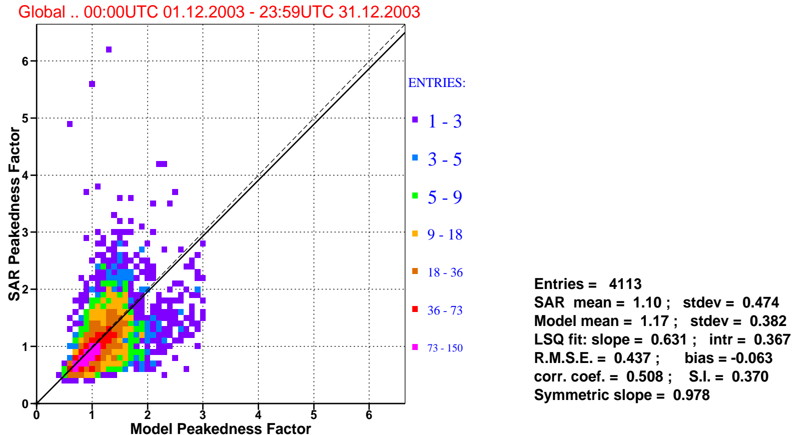
Figure 10: : Comparison of ECMWF wave peakedness factor with that of ERS-2 SAR for decemeber 2003 (global).
