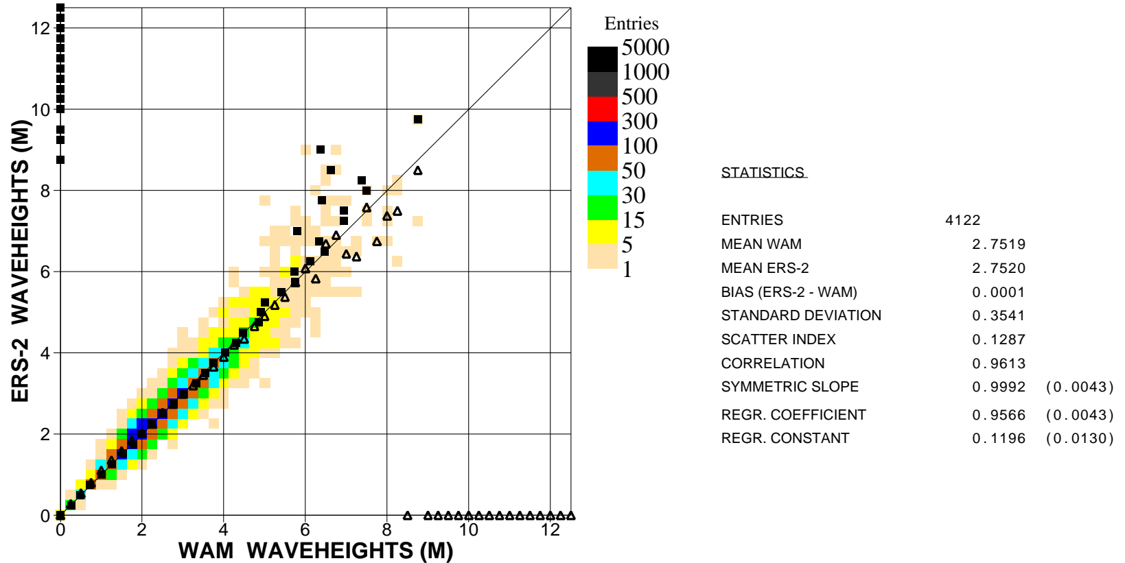
Figure 2: Comparison of ECMWF wave height results with ERS2 SAR wave height data for December 2003 (global)
