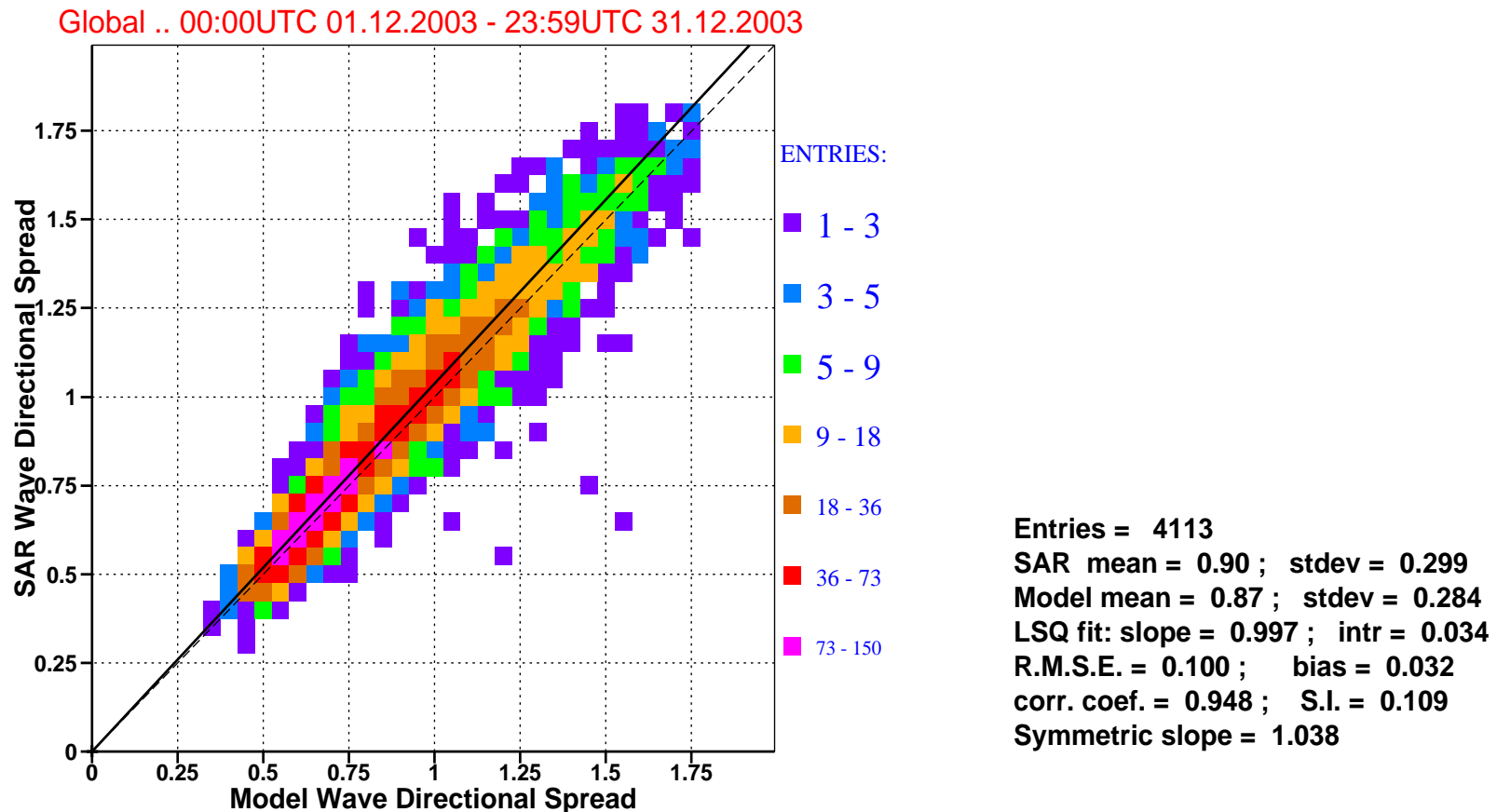
Figure 8: Comparison of ECMWF wave directional spread with that of ERS-2 SAR for decemeber 2003 (global).
