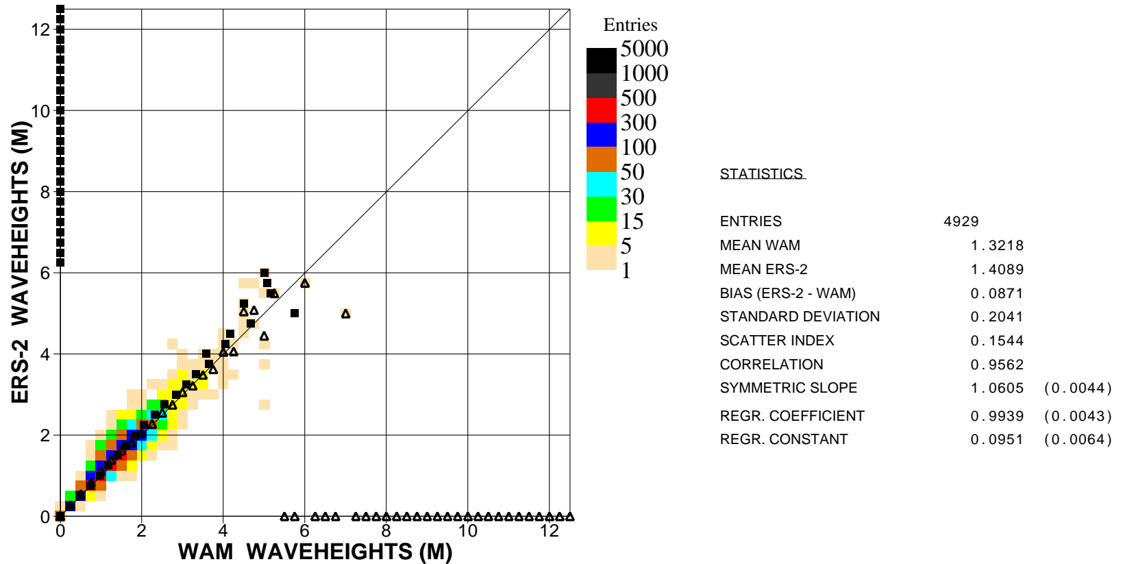
Figure 2: Comparison of ECMWF wave height results with ERS2 SAR wave height data for August 2004 (global)
