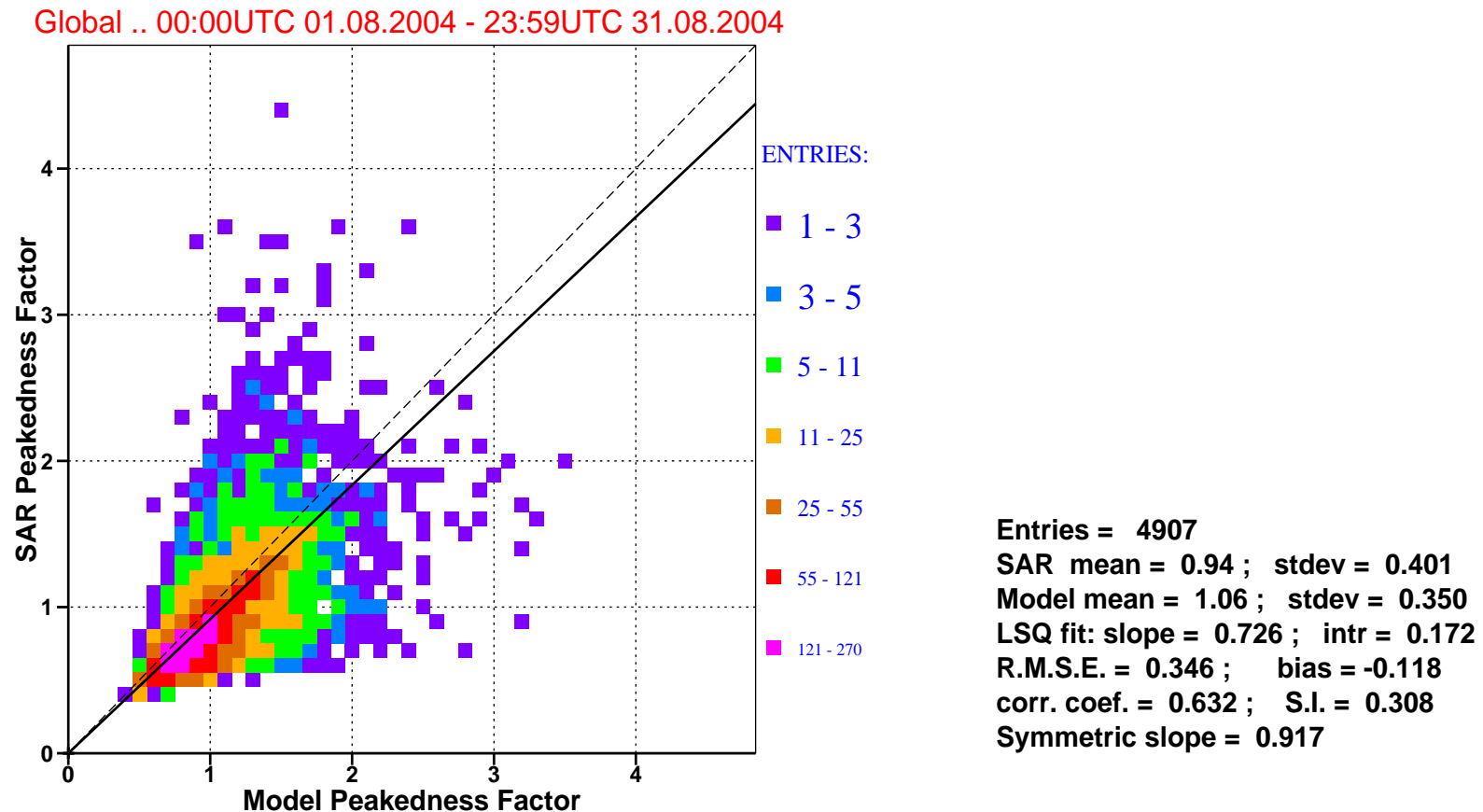
Figure 10: : Comparison of ECMWF wave peakedness factor with that of ERS-2 SAR for august 2004 (global).
