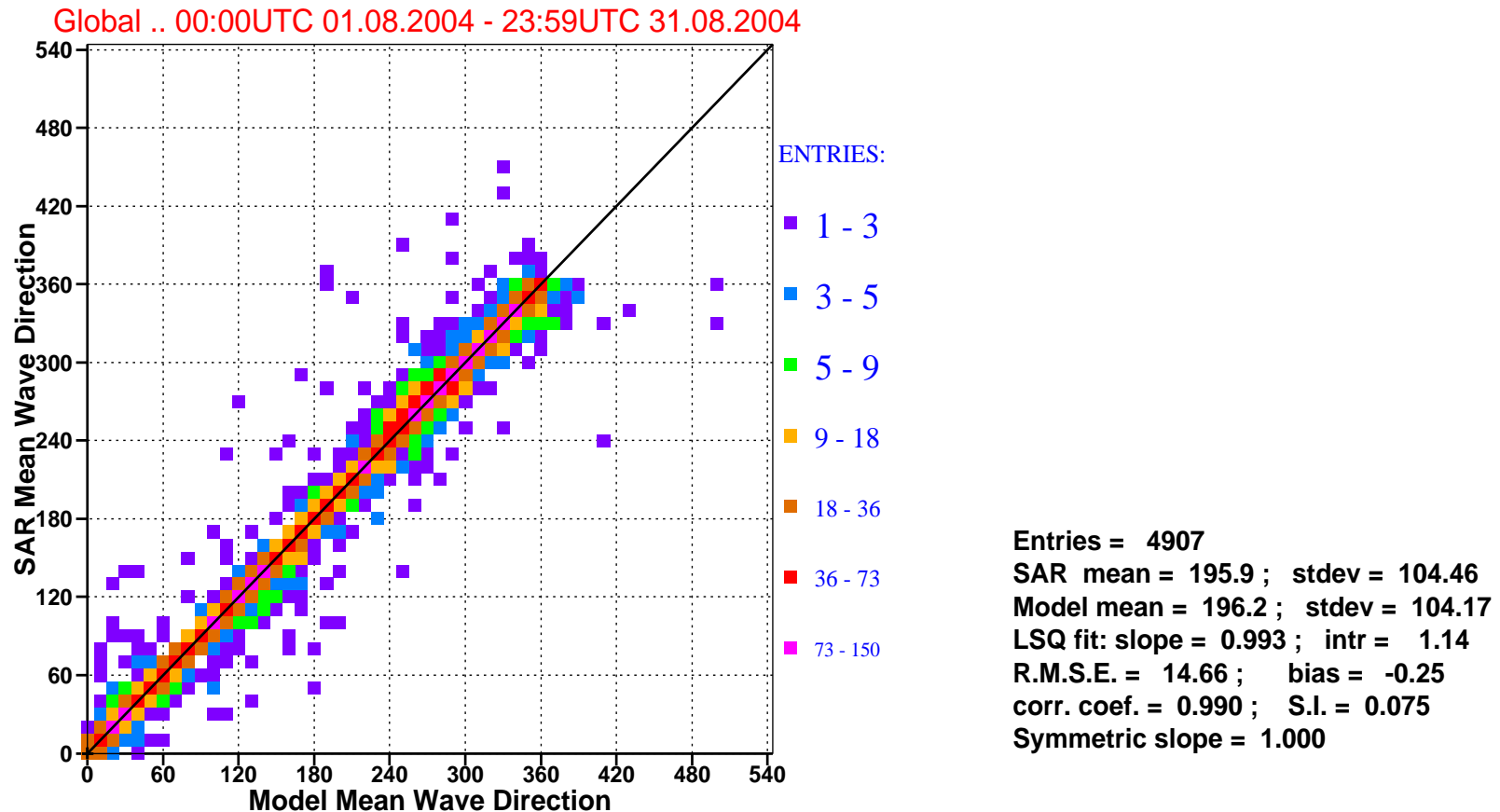
Figure 9: Comparison of ECMWF mean wave directions with that of ERS-2 SAR for august 2004 (global).
