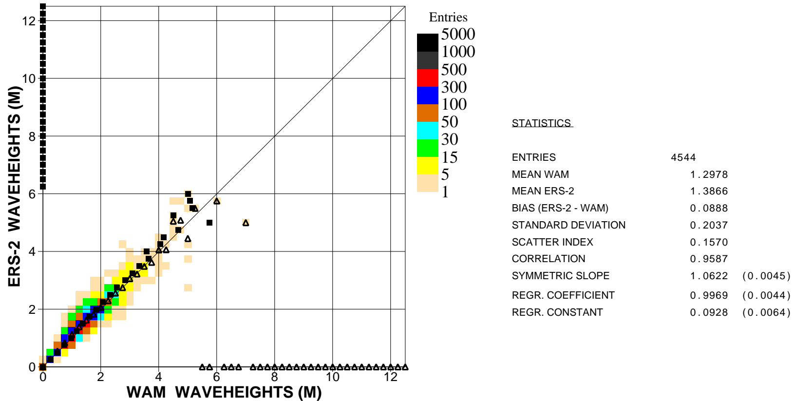
Figure 3: Comparison of ECMWF wave height results with ERS2 SAR wave height data for August 2004 (n.hem.)
