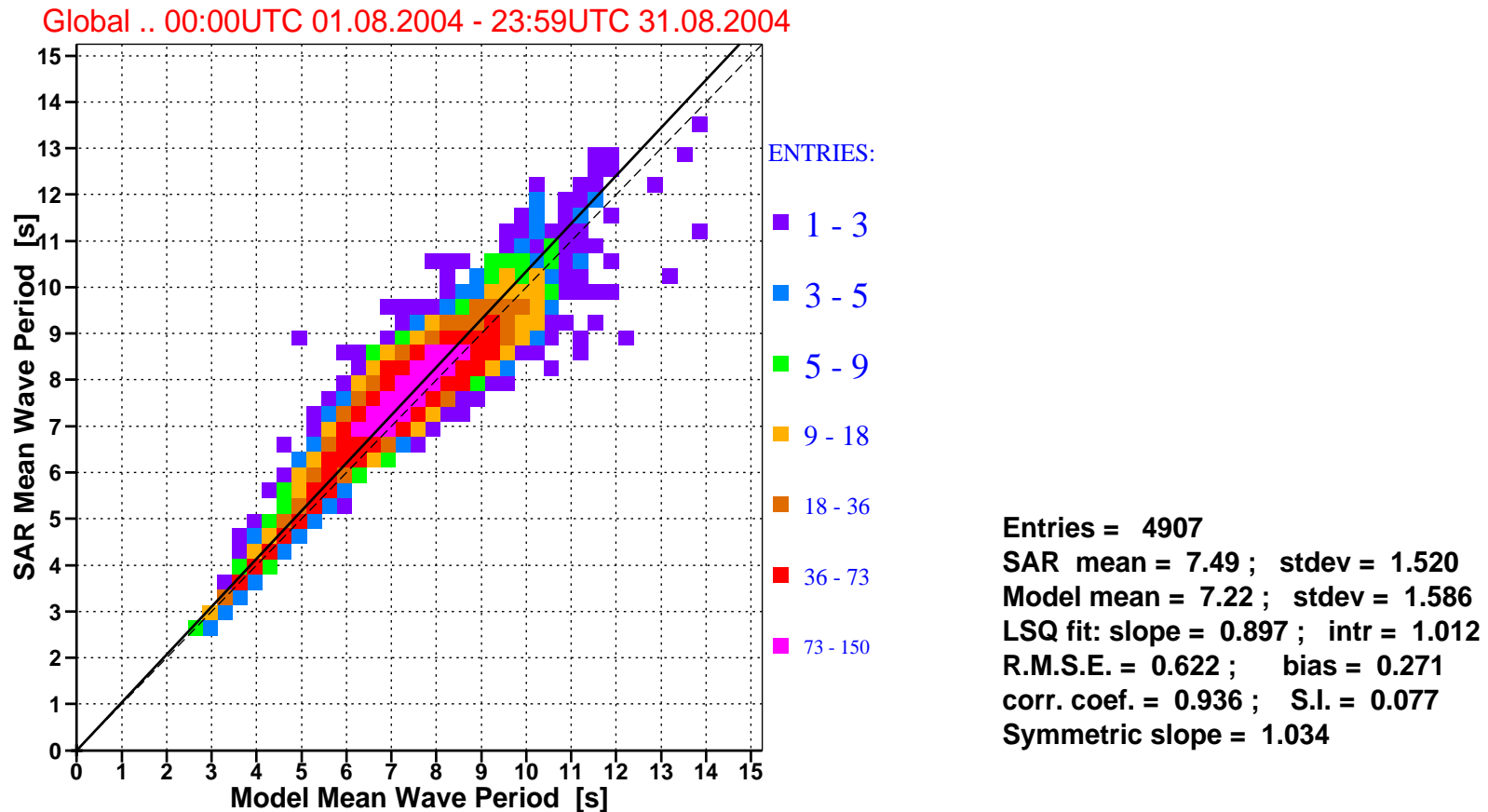
Figure 7: Comparison of ECMWF mean wave periods with ERS-2 SAR mean wave periods for august 2004 (global).
