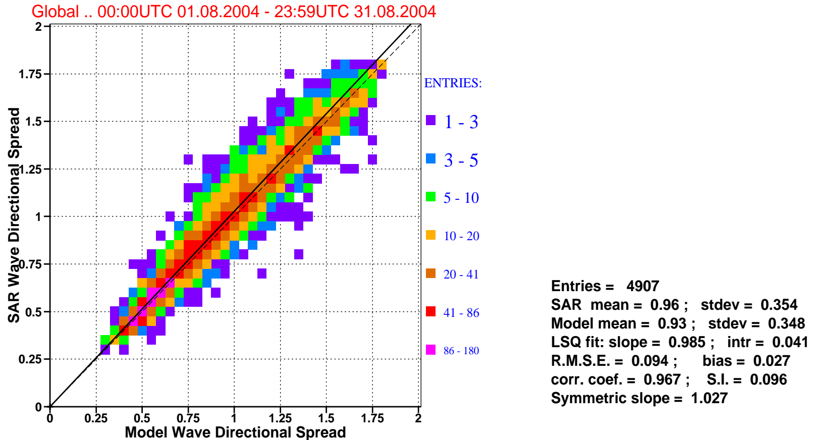
Figure 8: Comparison of ECMWF wave directional spread with that of ERS-2 SAR for august 2004 (global).
