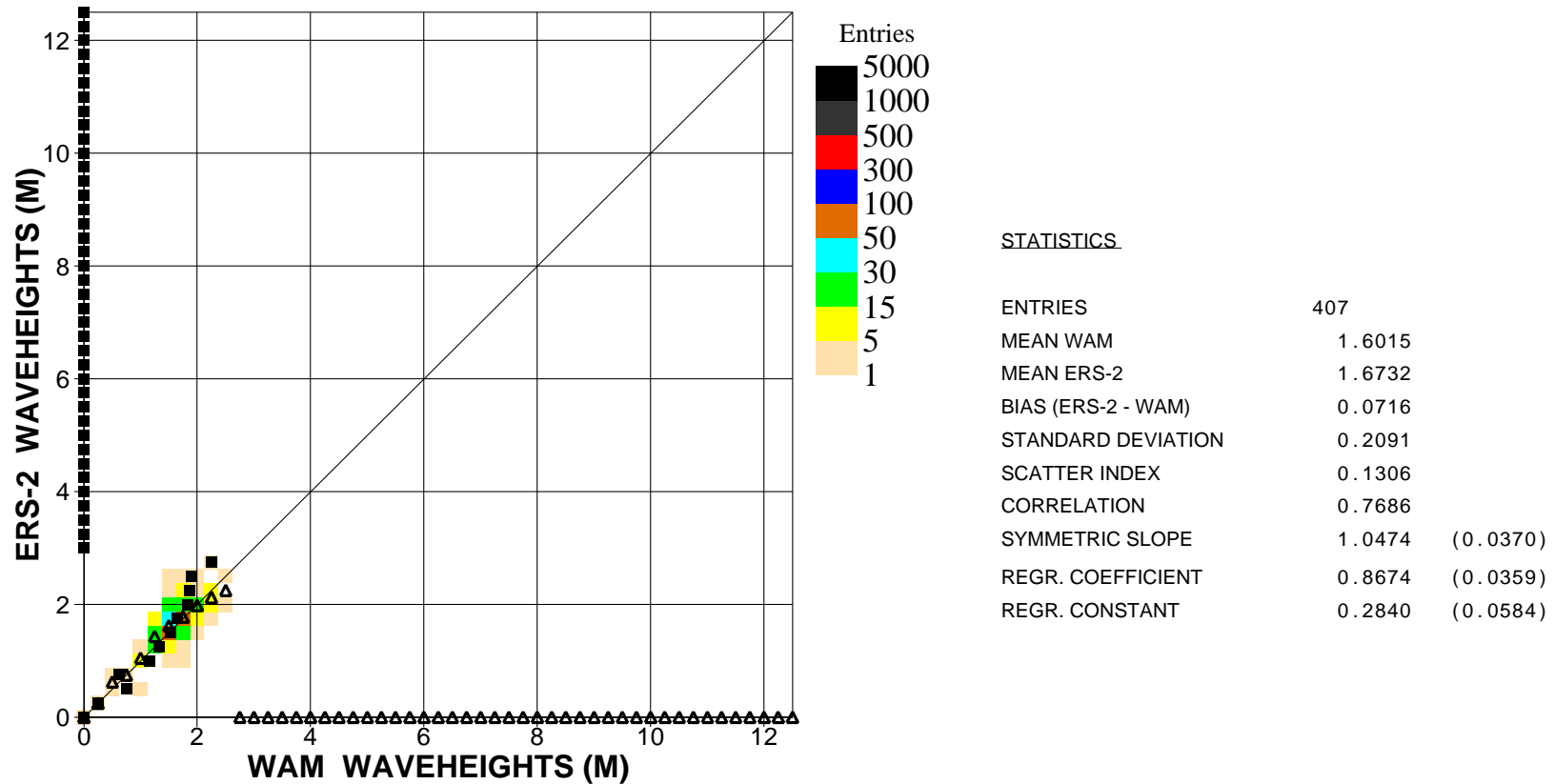
Figure 4: Comparison of ECMWF wave height results with ERS2 SAR wave height data for August 2004 (tropics)
