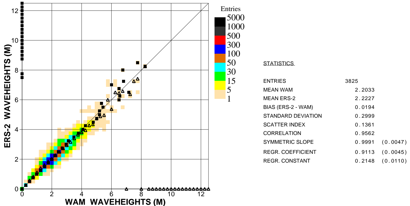
Figure 3: Comparison of ECMWF wave height results with ERS2 SAR wave height data for April 2004 (n.hem.)
