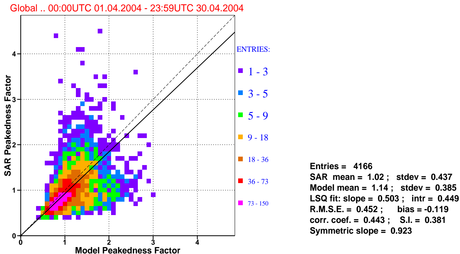
Figure 10: : Comparison of ECMWF wave peakedness factor with that of ERS-2 SAR for april 2004 (global).
