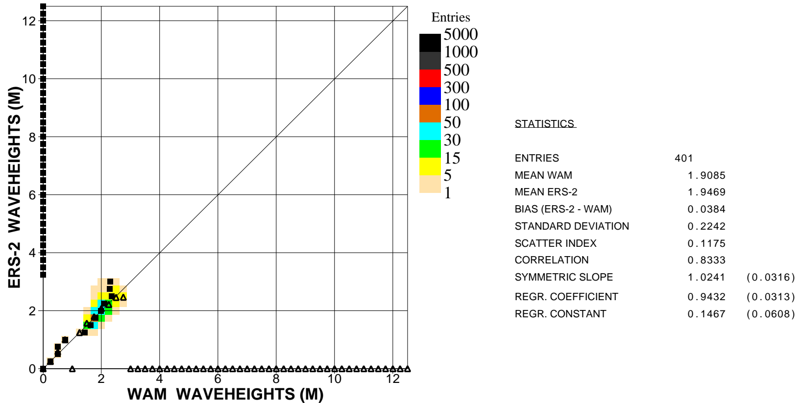
Figure 4: Comparison of ECMWF wave height results with ERS2 SAR wave height data for April 2004 (tropics)
