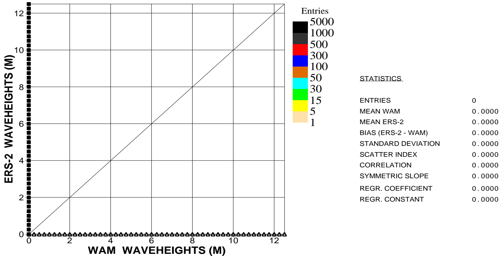
Figure 5: Comparison of ECMWF wave height results with ERS2 SAR wave height data for April 2004 (s.hem.)
