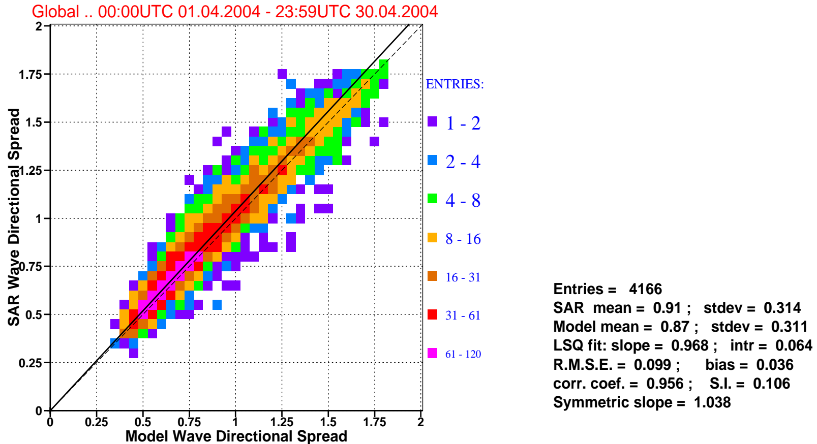
Figure 8: Comparison of ECMWF wave directional spread with that of ERS-2 SAR for april 2004 (global).
