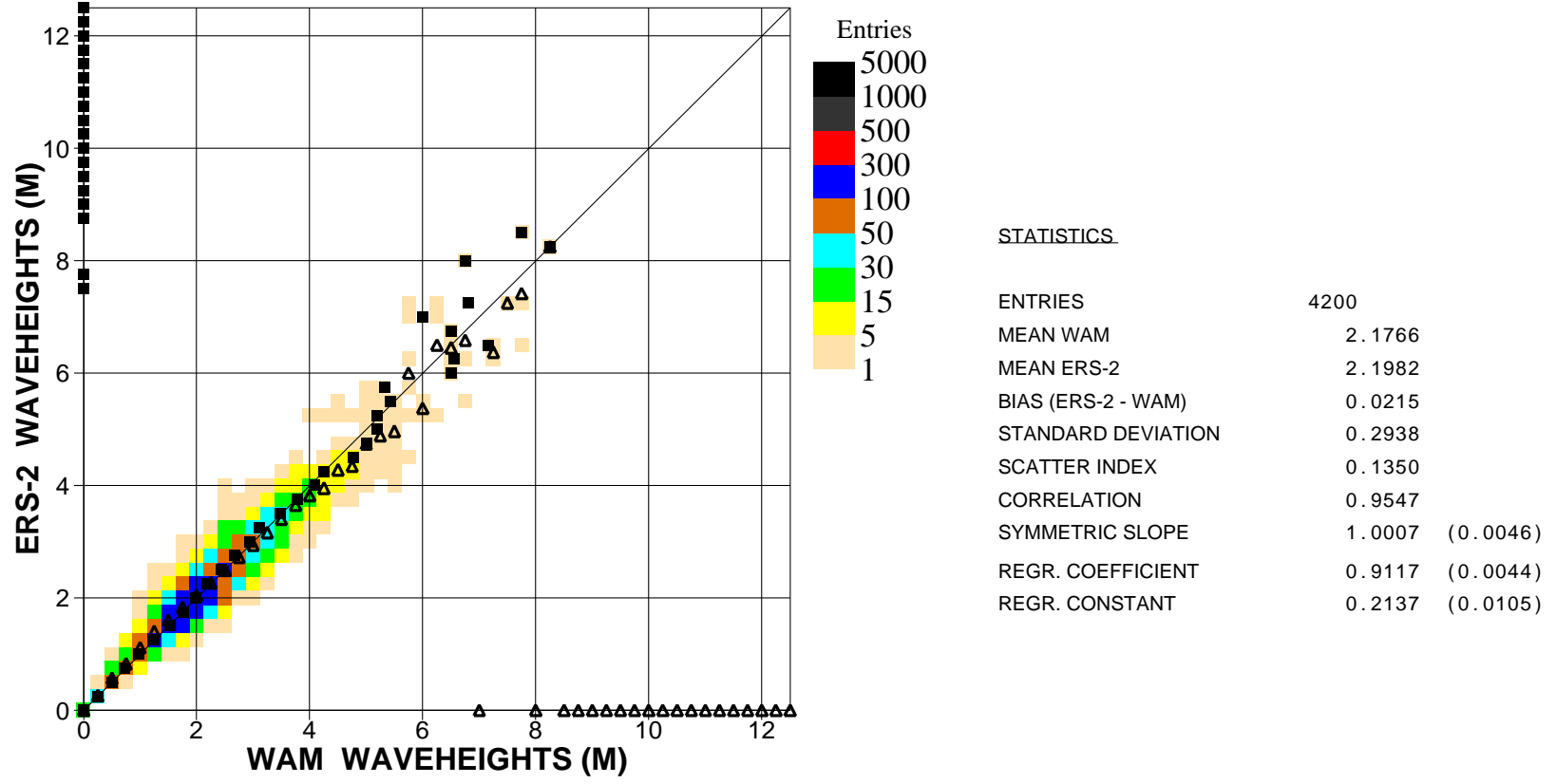
Figure 2: Comparison of ECMWF wave height results with ERS2 SAR wave height data for April 2004 (global)
