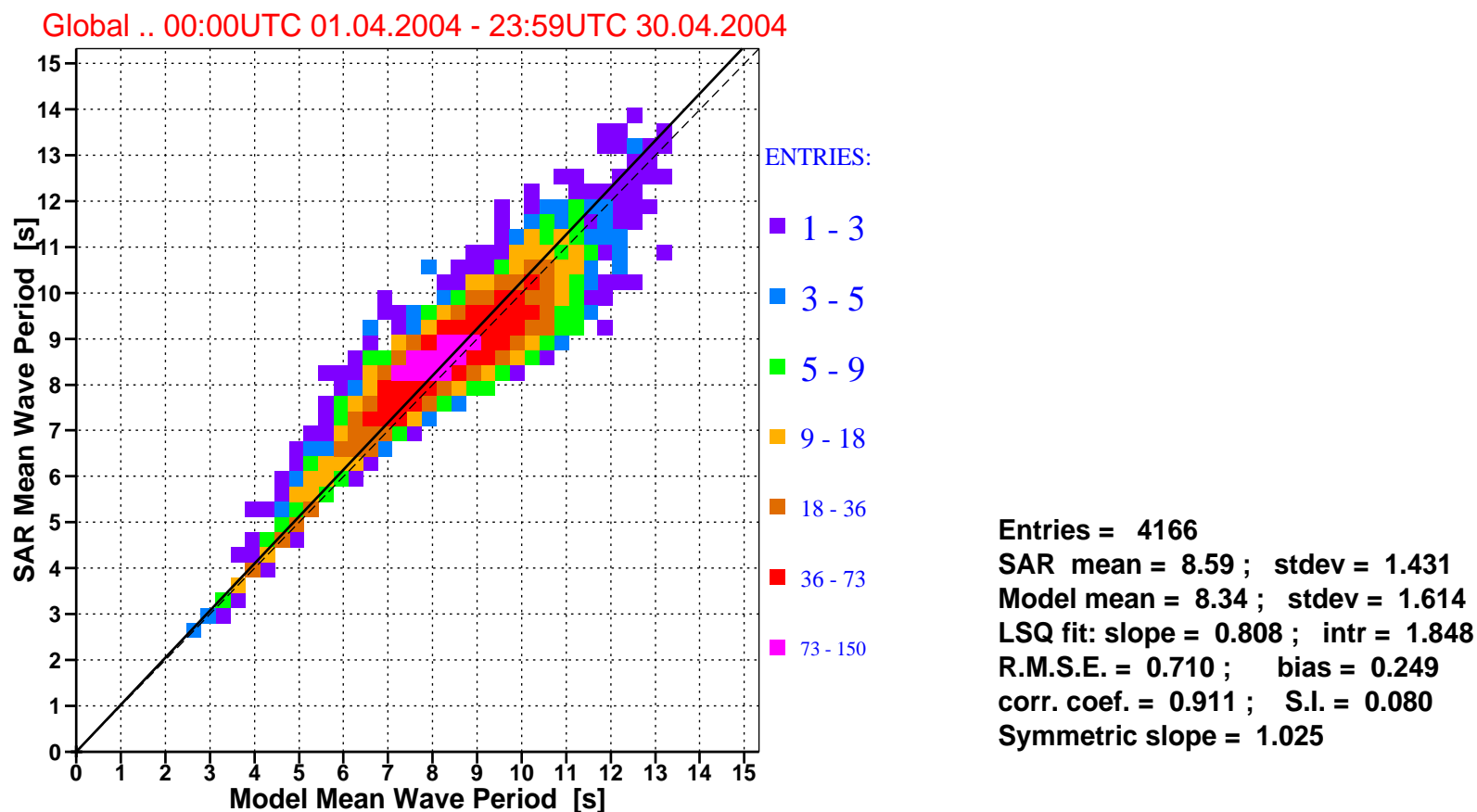
Figure 7: Comparison of ECMWF mean wave periods with ERS-2 SAR mean wave periods for april 2004 (global).
