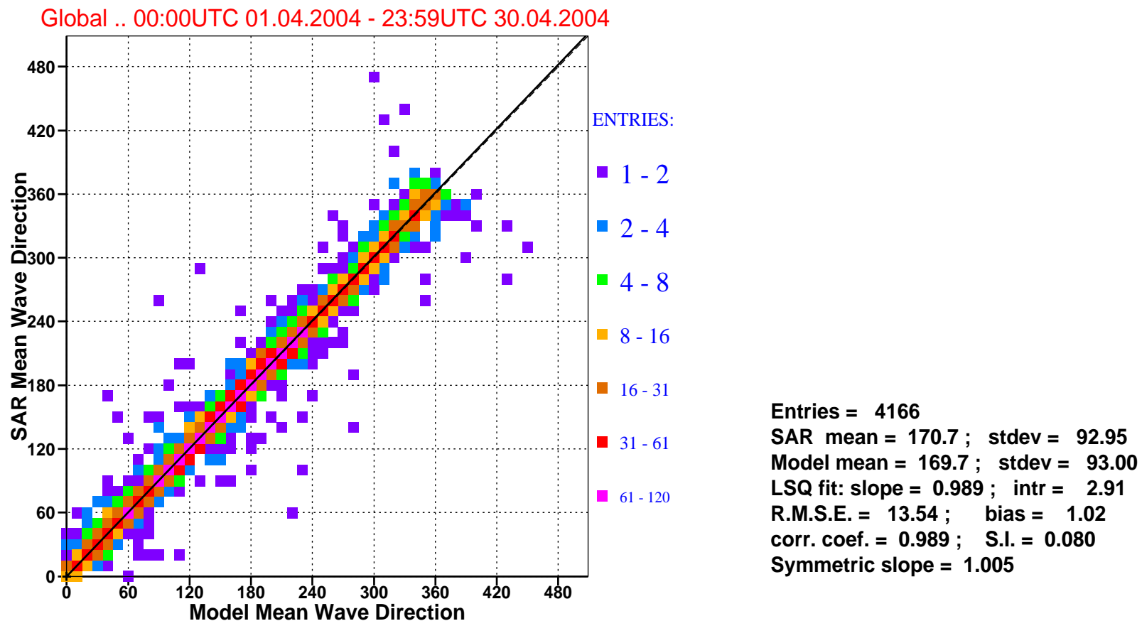
Figure 9: Comparison of ECMWF mean wave directions with that of ERS-2 SAR for april 2004 (global).
