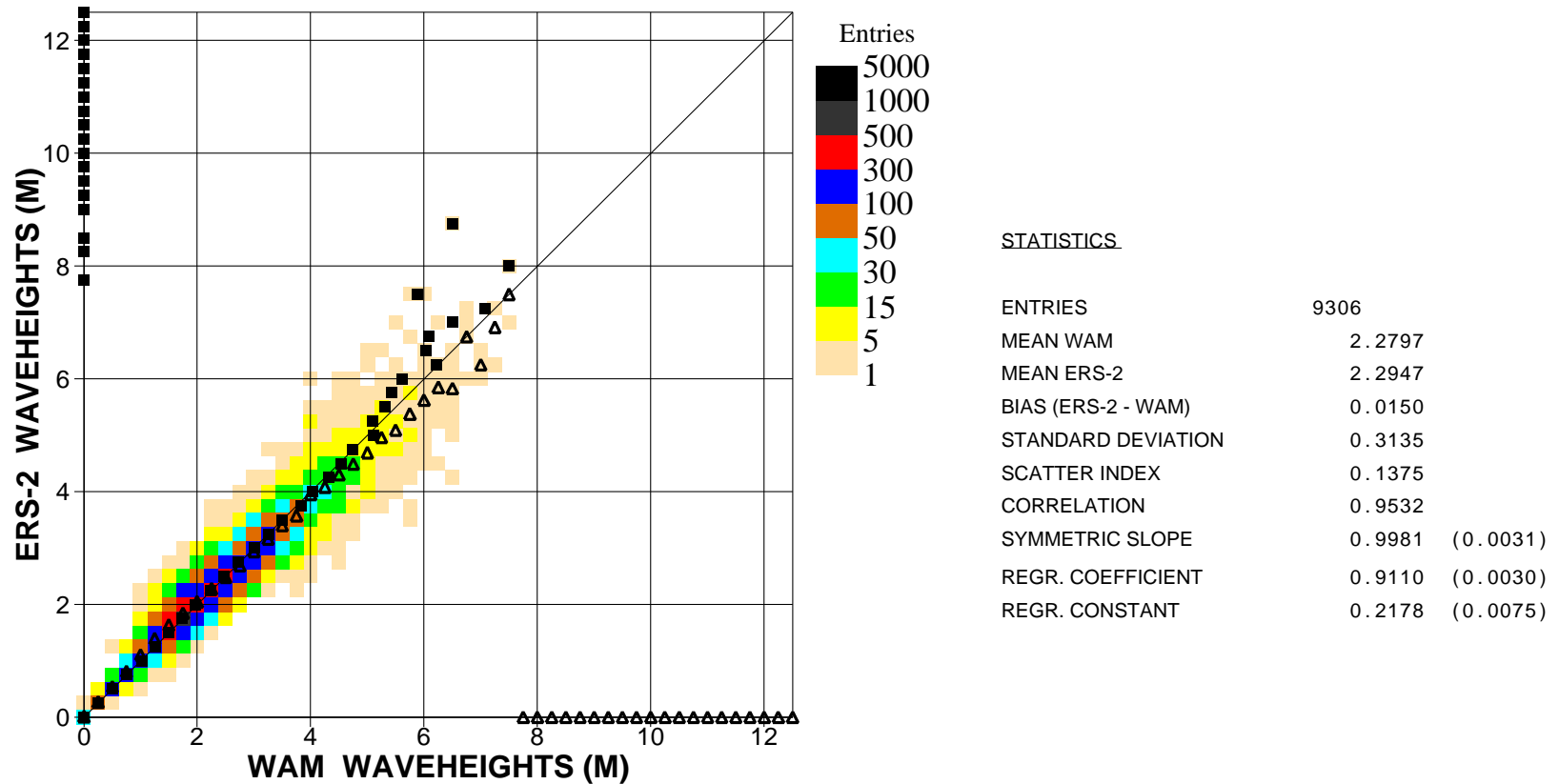
Figure 3: Comparison of ECMWF wave height results with ERS2 SAR wave height data for April 2003 (n.hem.)
