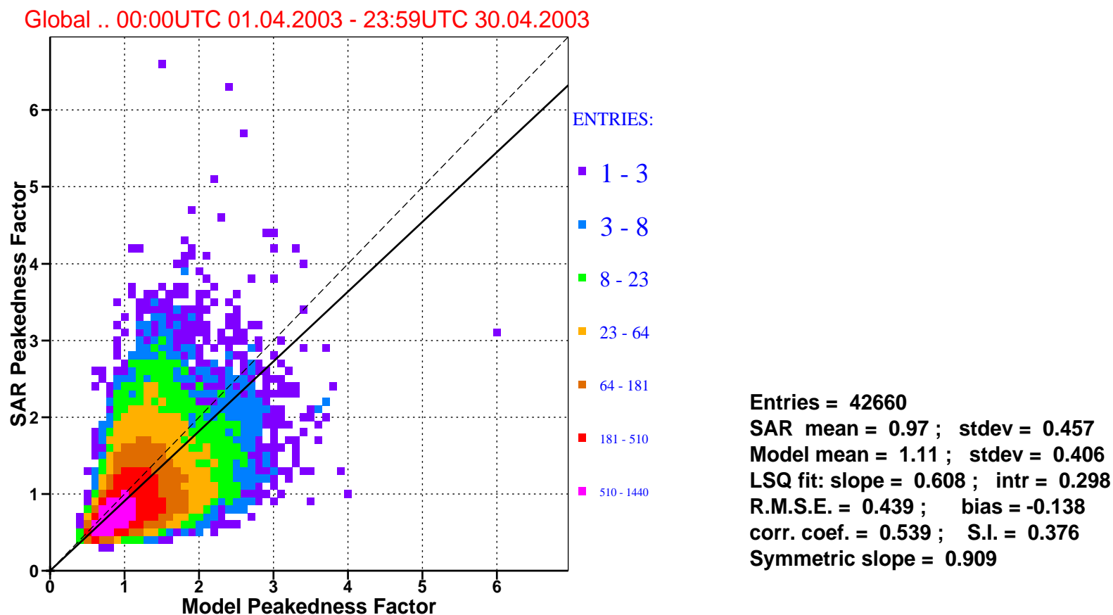
Figure 10: : Comparison of ECMWF wave peakedness factor with that of ERS-2 SAR for april 2003 (global).
