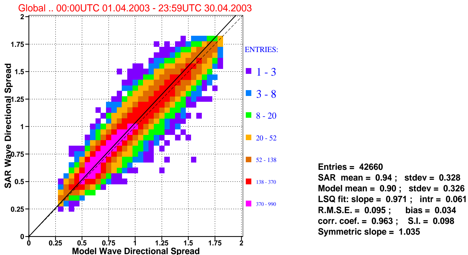
Figure 8: Comparison of ECMWF wave directional spread with that of ERS-2 SAR for april 2003 (global).
