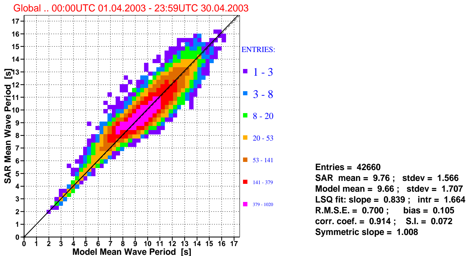
Figure 7: Comparison of ECMWF mean wave periods with ERS-2 SAR mean wave periods for april 2003 (global).
