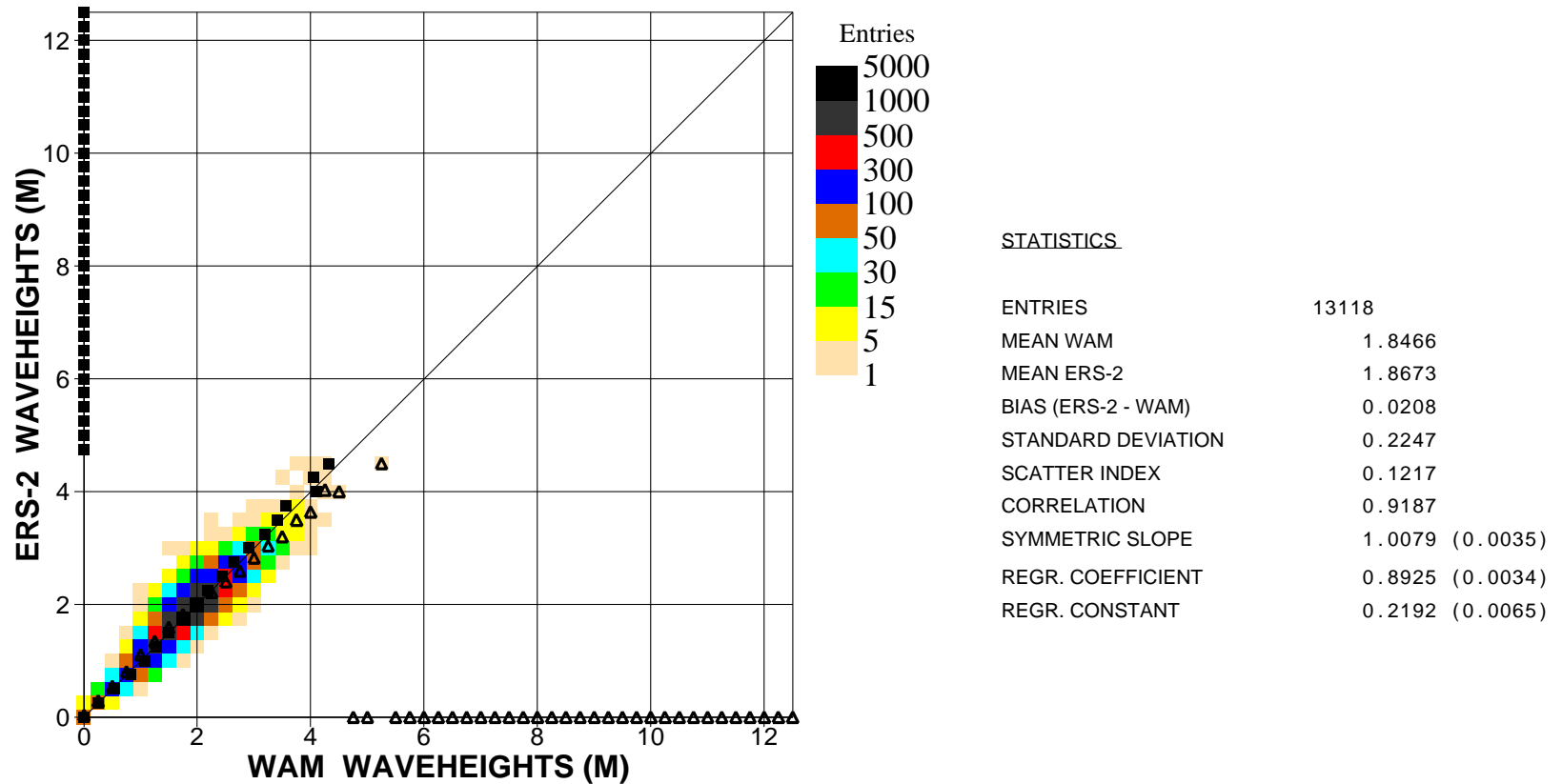
Figure 4: Comparison of ECMWF wave height results with ERS2 SAR wave height data for April 2003 (tropics)
