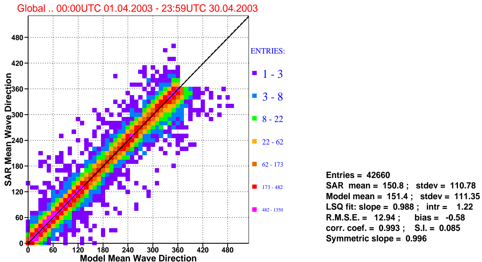
Figure 9: Comparison of ECMWF mean wave directions with that of ERS-2 SAR for april 2003 (global).
