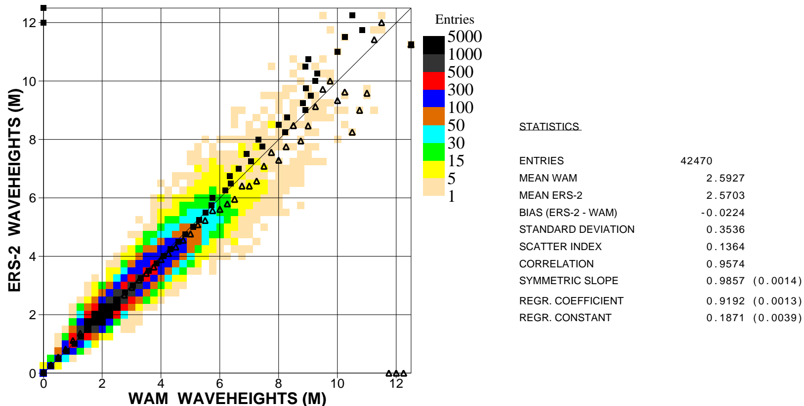
Figure 2: Comparison of ECMWF wave height results with ERS2 SAR wave height data for April 2003 (global)
