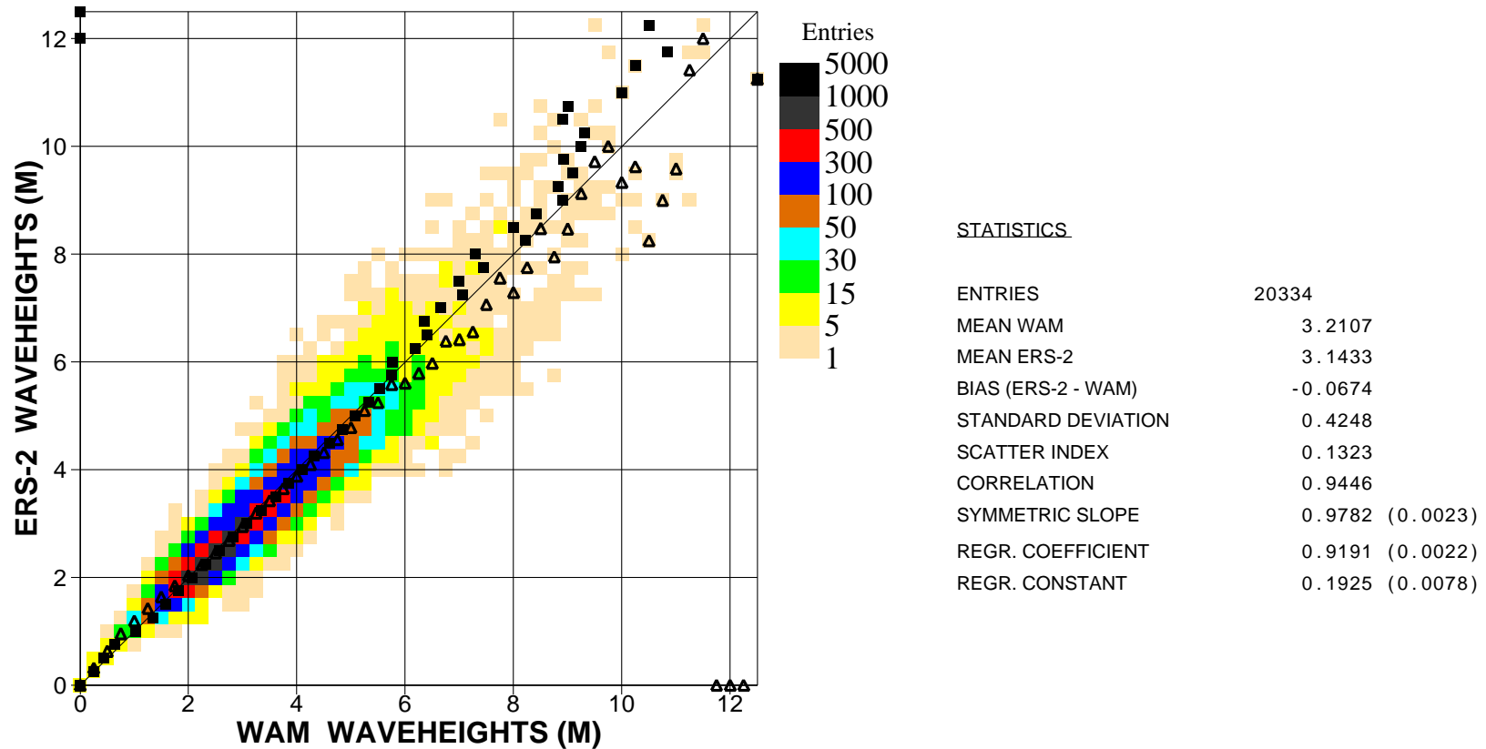
Figure 5: Comparison of ECMWF wave height results with ERS2 SAR wave height data for April 2003 (s.hem.)
