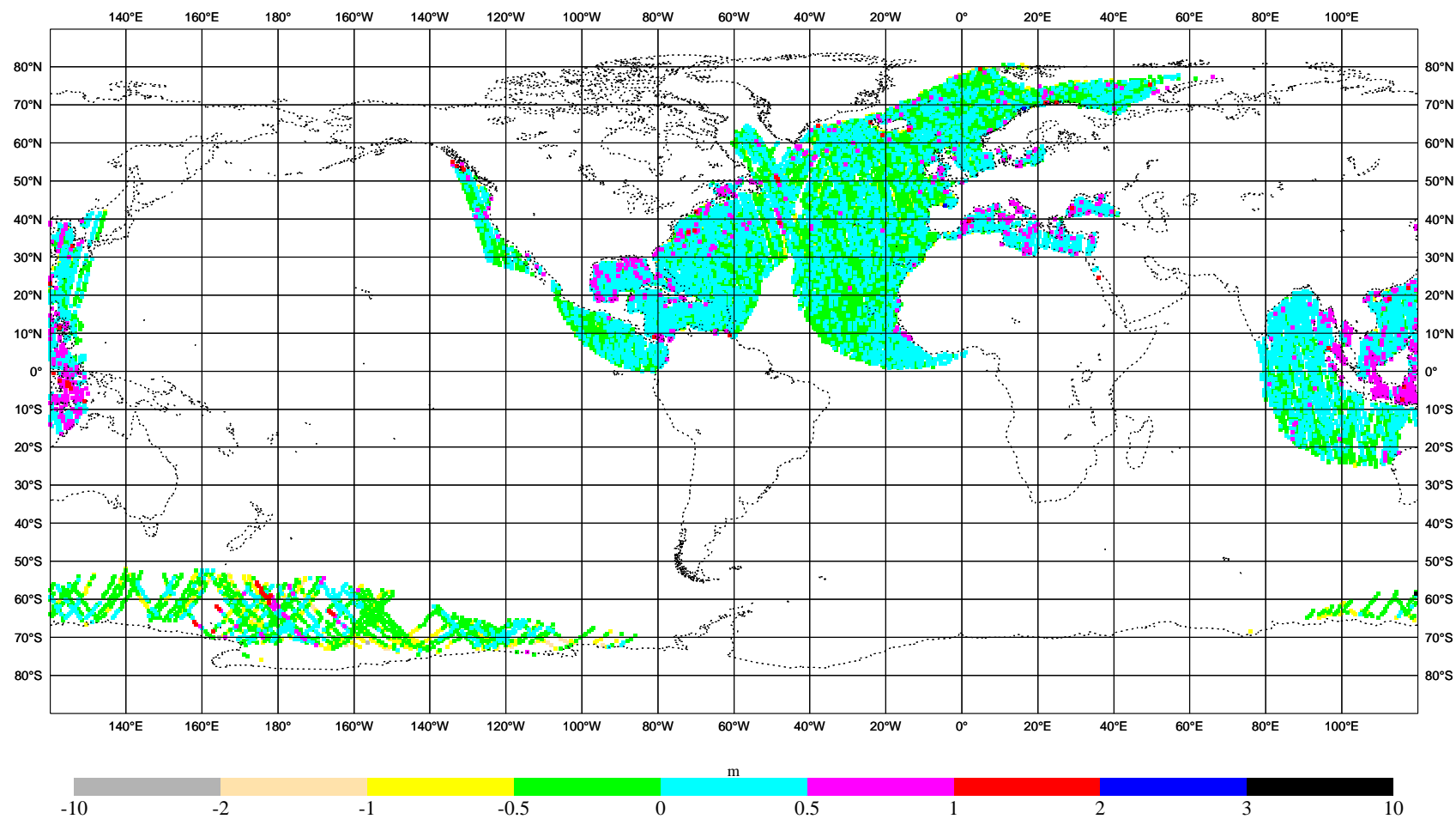
Figure 27: Significant wave height: Monthly mean difference of ERS-2 altimeter data minus wave model results for March 2010.
