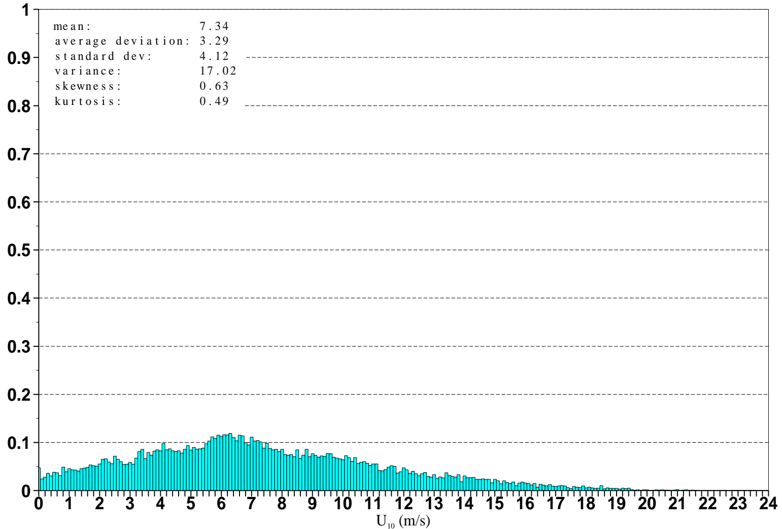
Figure 4: Distribution of ERS-2 Altimeter wind speeds after along track averaging for March 2010
