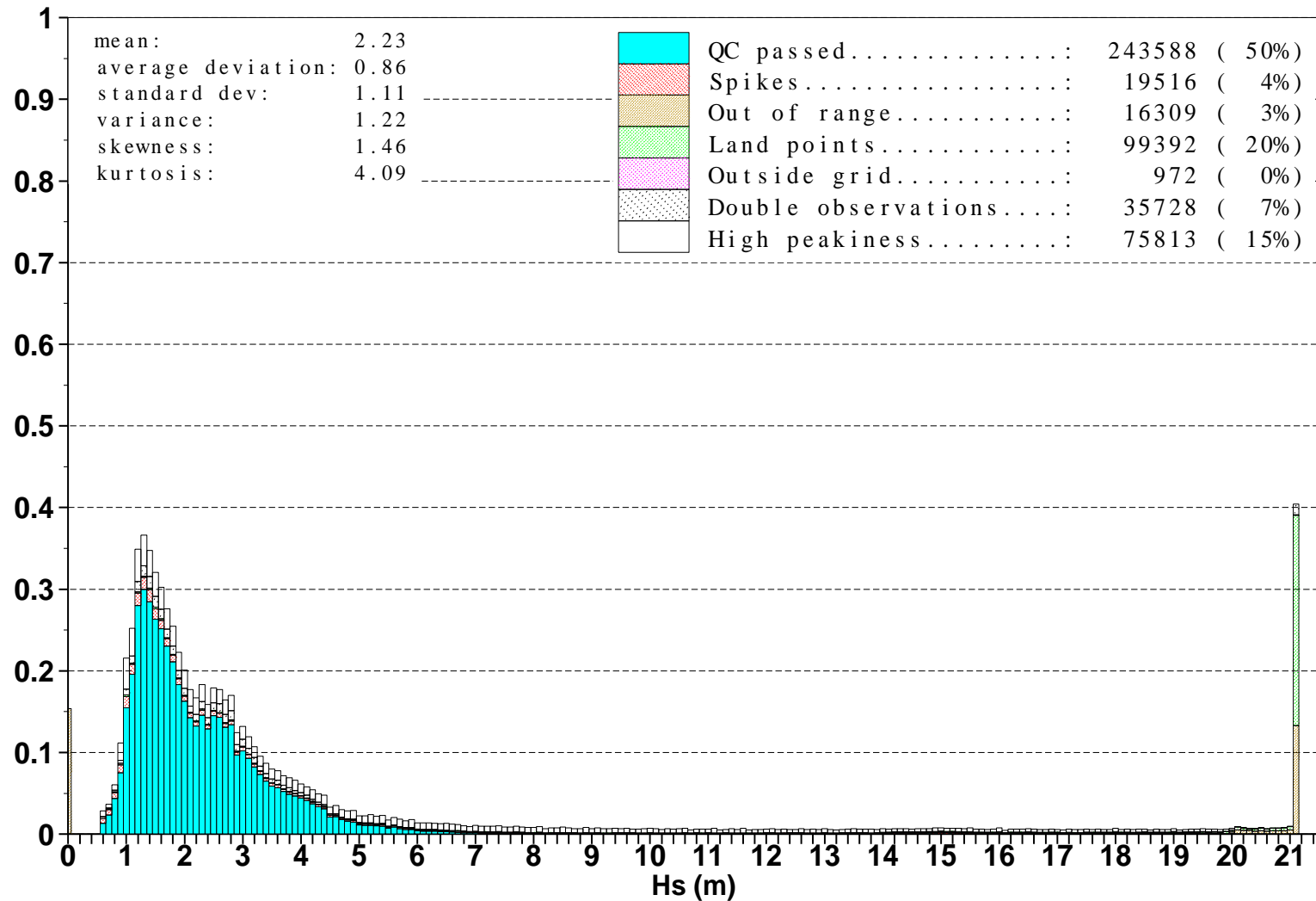
Figure 14: Distribution of the ERS-2 Altimeter wave heights after QC for March 2010
