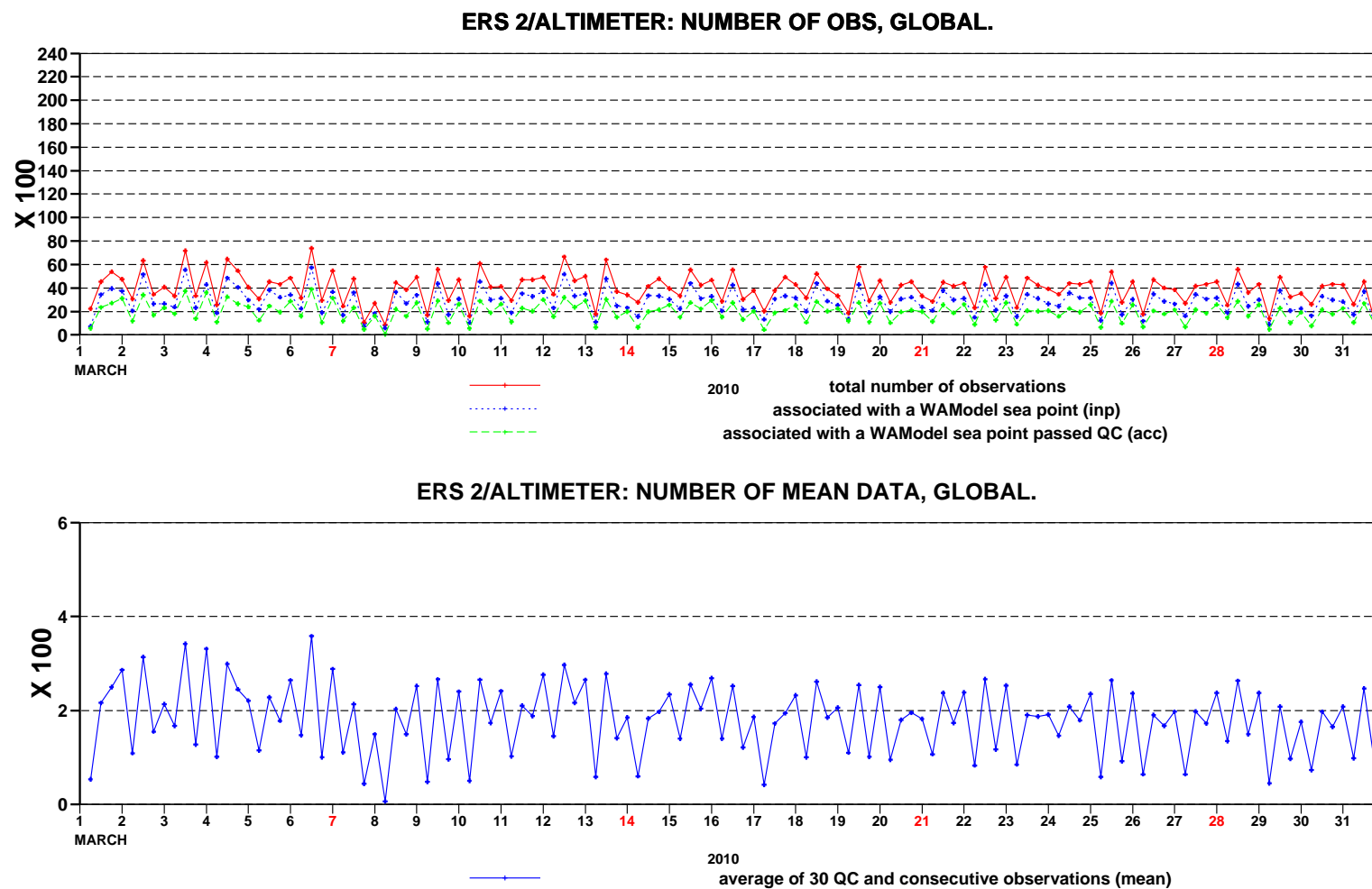
Figure 1: Time series of data reception for ERS-2 Altimeter data for March 2010
