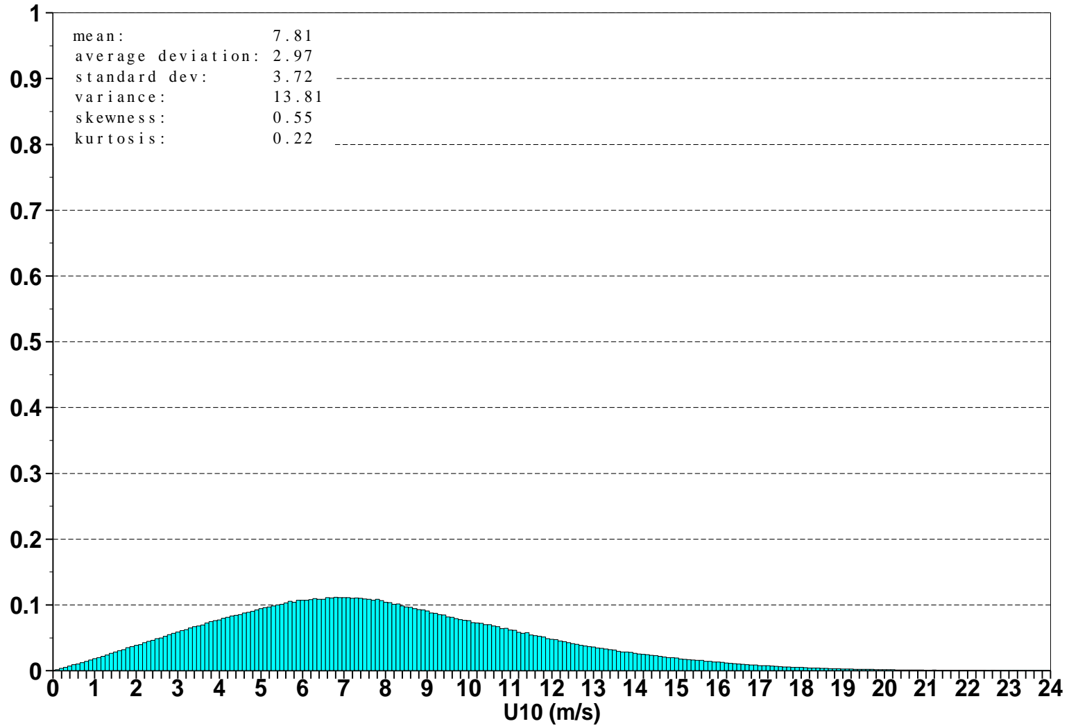
Figure 5: Global distribution of ECMWF ocean surface wind speeds for March 2010
