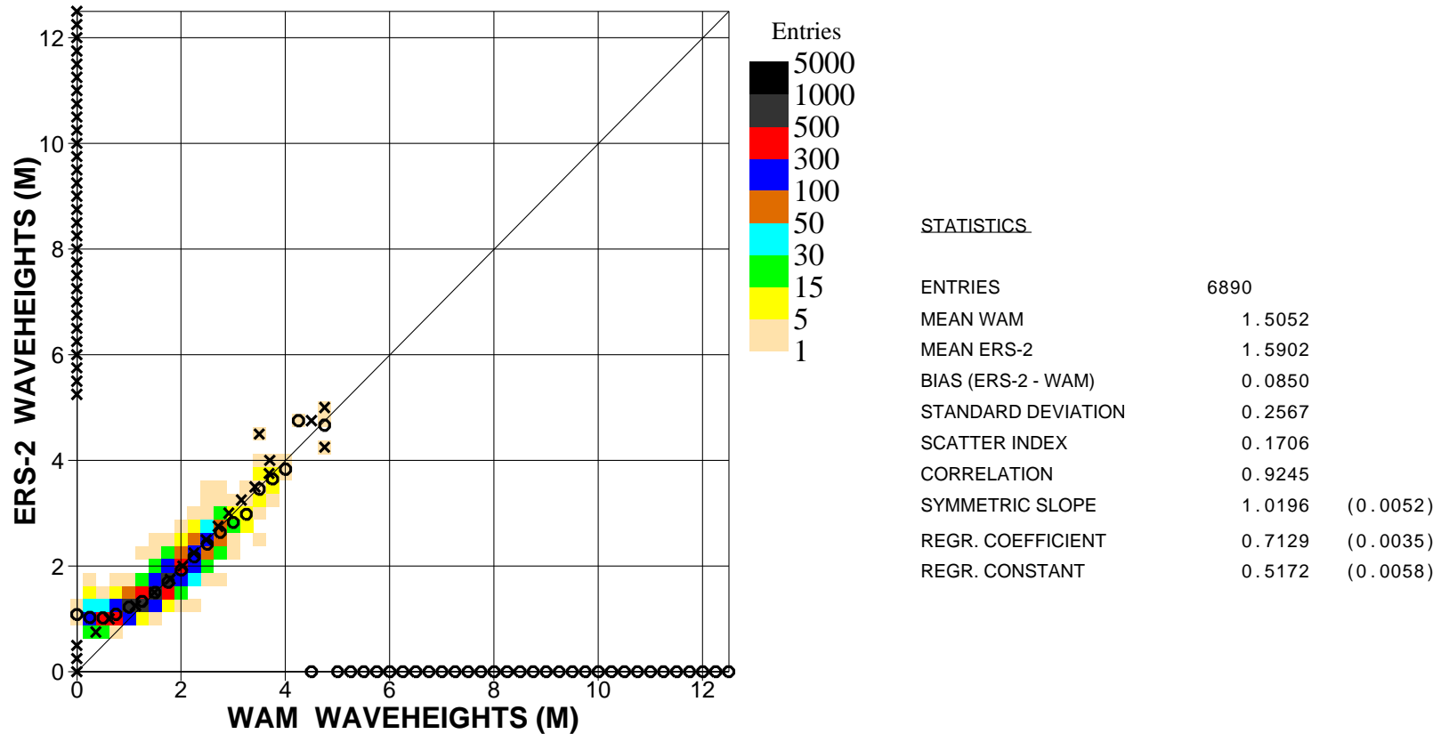
Figure 19. Comparison of ECMWF wave height results with ERS2 Altimeter wave height data for March 2010 (tropics)
