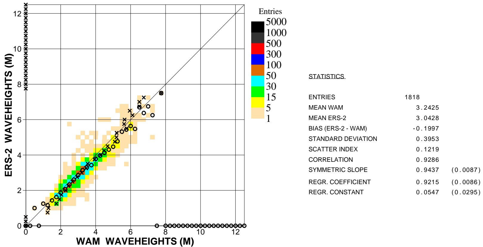
Figure 20. Comparison of ECMWF wave height results with ERS2 Altimeter wave height data for March 2010 (s.hem.)
