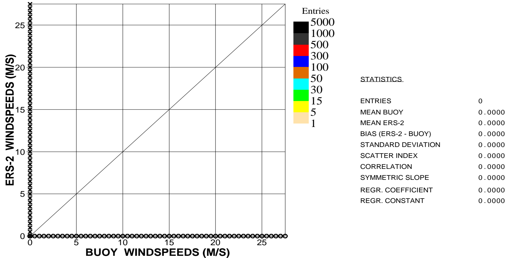
Figure 12. Comparison of buoy wind speed observations with ERS2 Altimeter wind speed data for March 2010 (hawaii)
