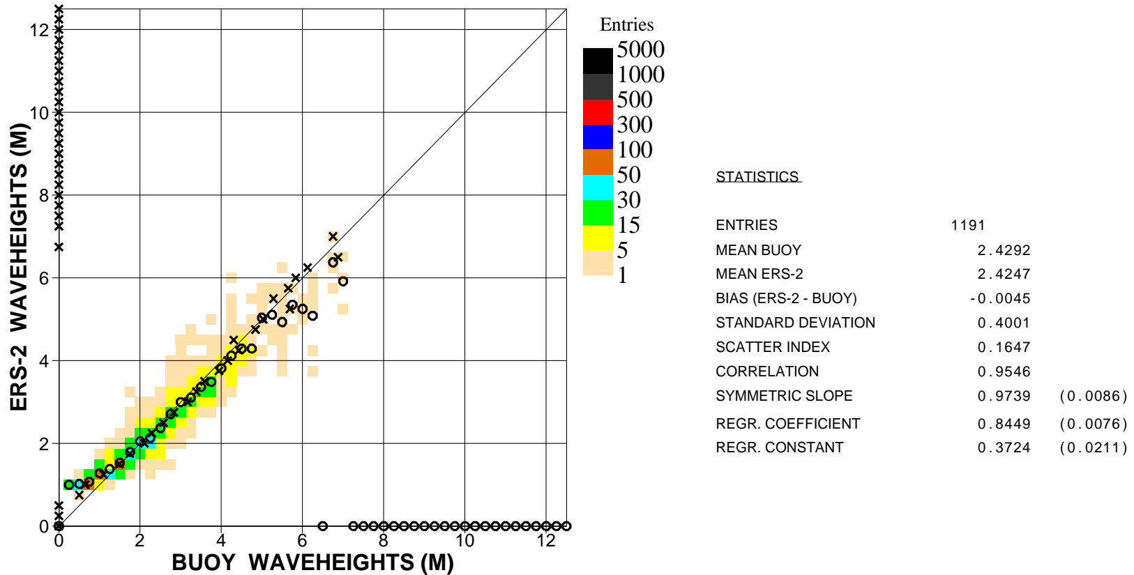
Figure 22. Comparison of buoy wave height observations with ERS2 Altimeter wave height data for March 2010 (n.hem.)
