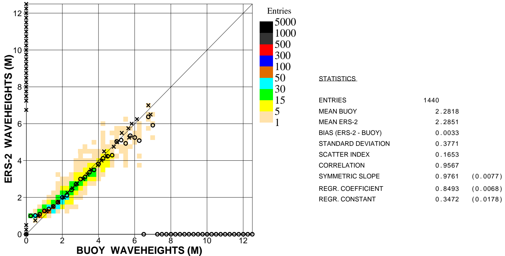
Figure 21. Comparison of buoy wave height observations with ERS2 Altimeter wave height data for March 2010 (global)
