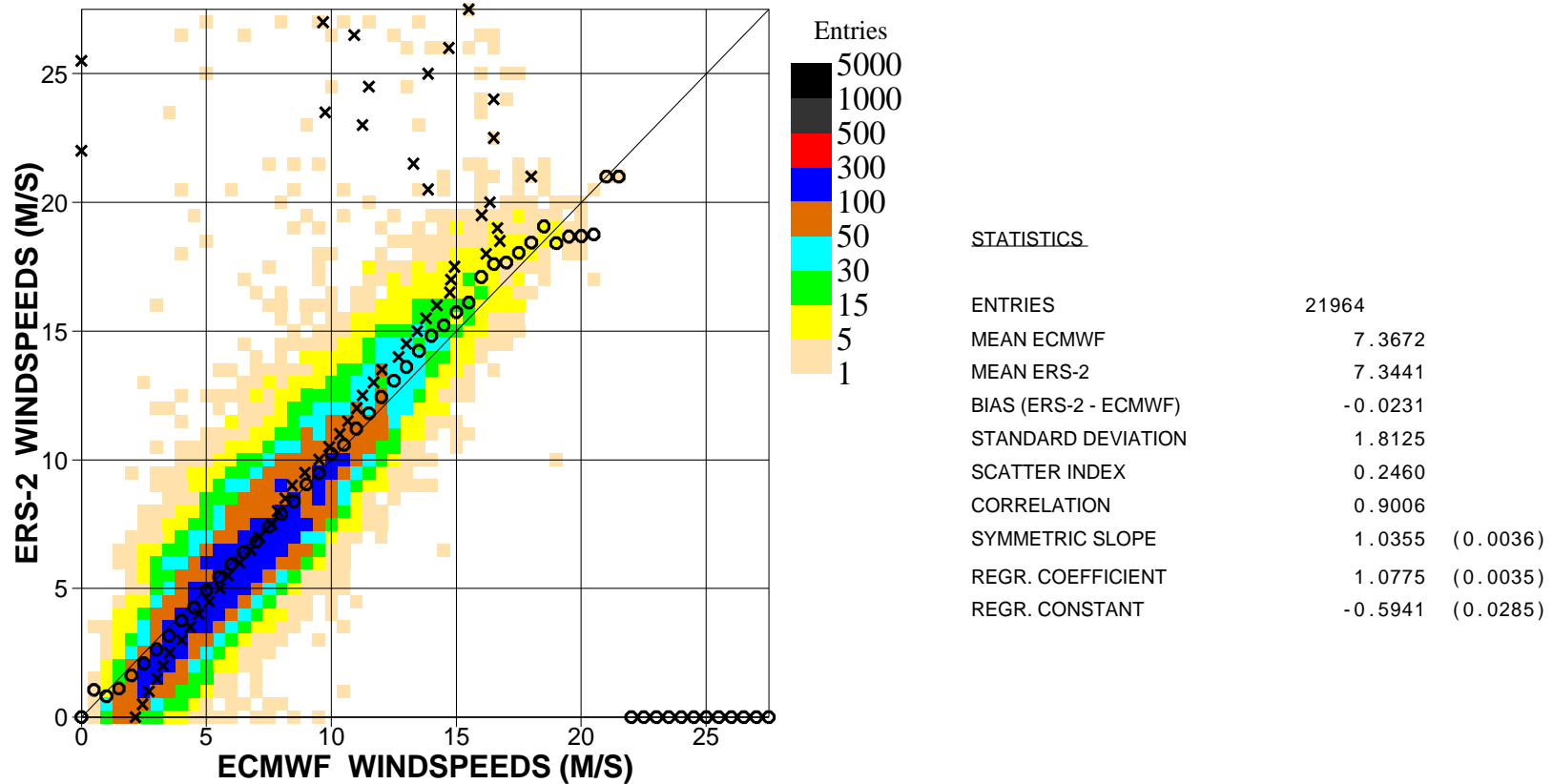
Figure 6. Comparison of ECMWF wind speed results with ERS2 Altimeter wind speed data for March 2010 (global)
