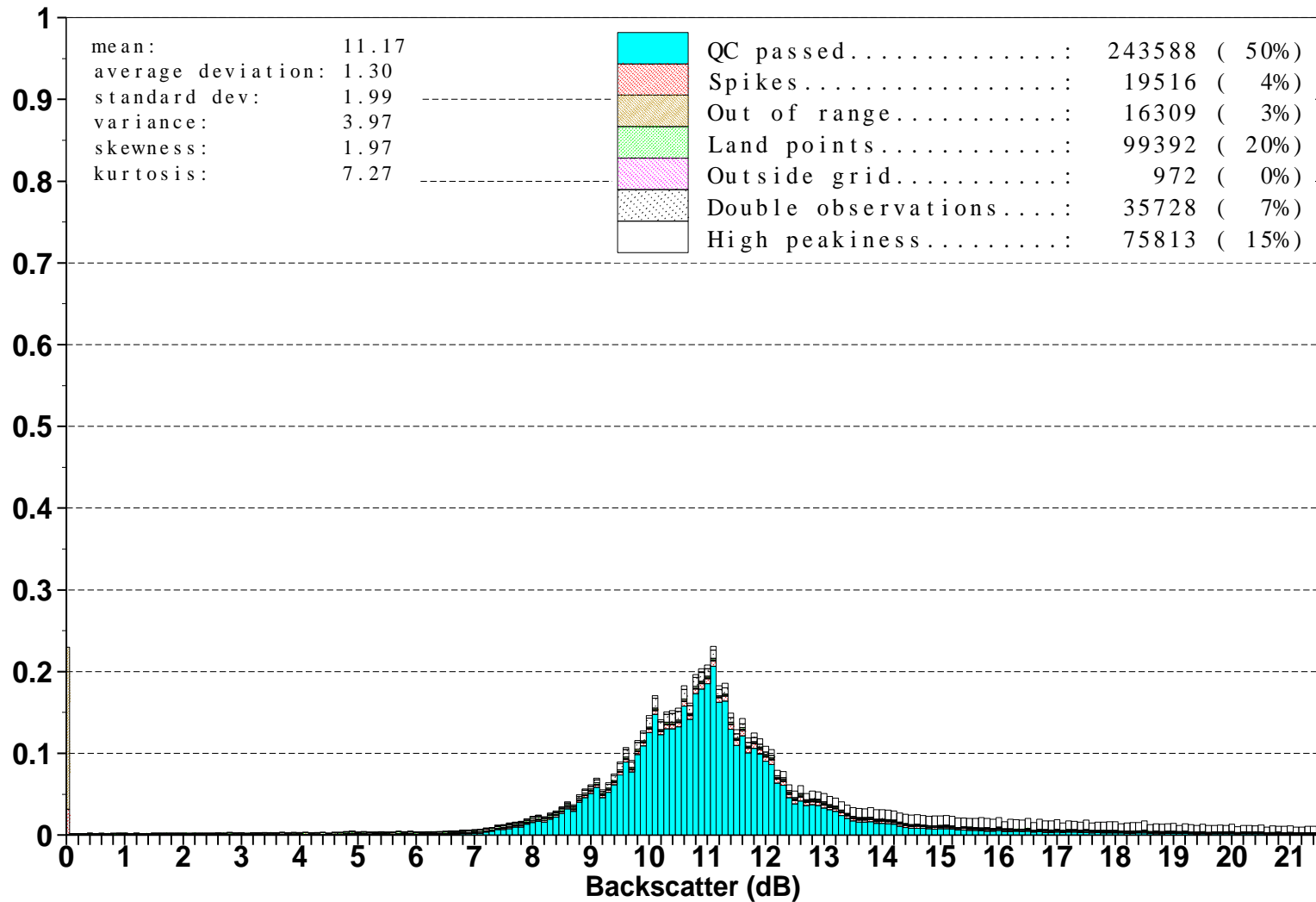
Figure 2: Distribution of the ERS-2 Altimeter backscatter after QC for March 2010
