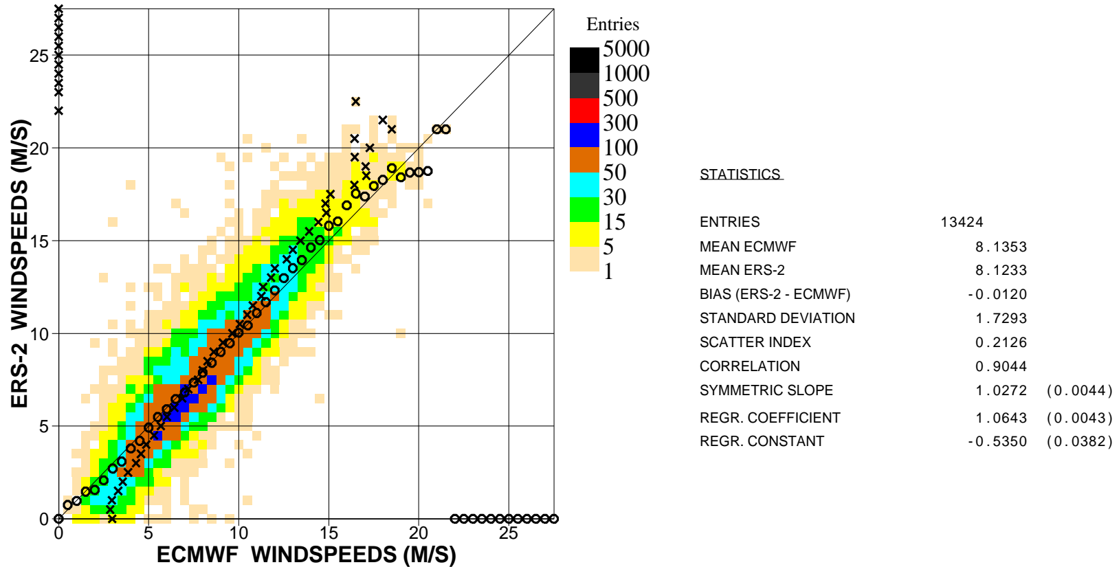
Figure 7. Comparison of ECMWF wind speed results with ERS2 Altimeter wind speed data for March 2010 (n.hem.)
