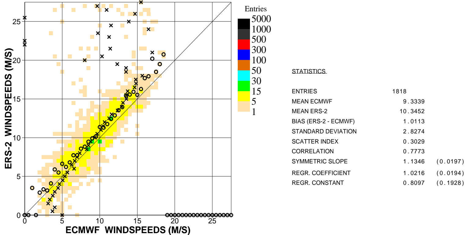
Figure 9. Comparison of ECMWF wind speed results with ERS2 Altimeter wind speed data for March 2010 (s.hem.)
