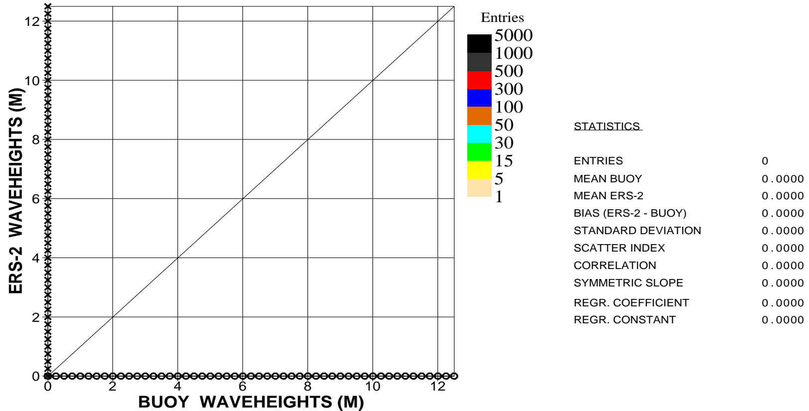
Figure 23. Comparison of buoy wave height observations with ERS2 Altimeter wave height data for March 2010 (hawaii)
