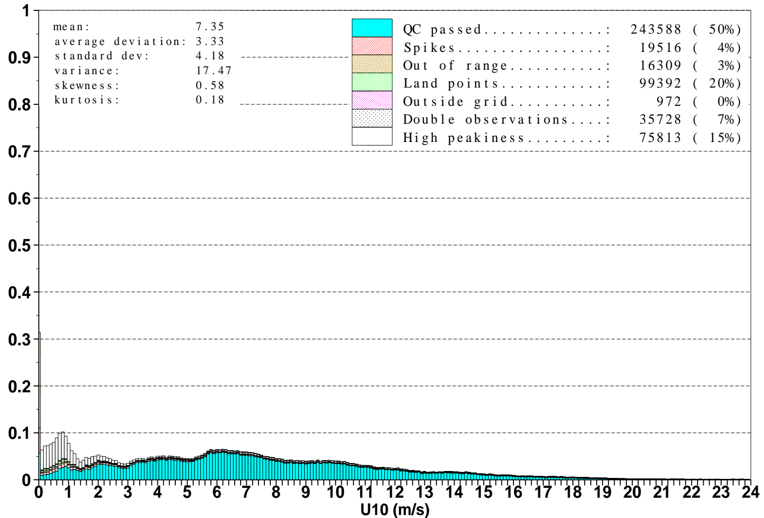
Figure 3: Distribution of the ERS-2 Altimeter wind speeds after QC for March 2010
