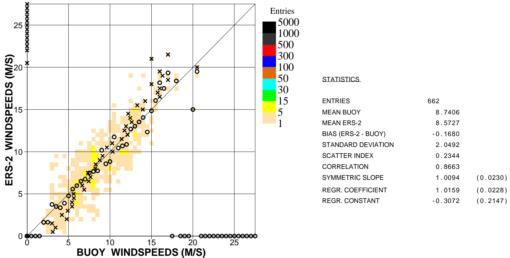
Figure 11. Comparison of buoy wind speed observations with ERS2 Altimeter wind speed data for March 2010 (n.hem.)
