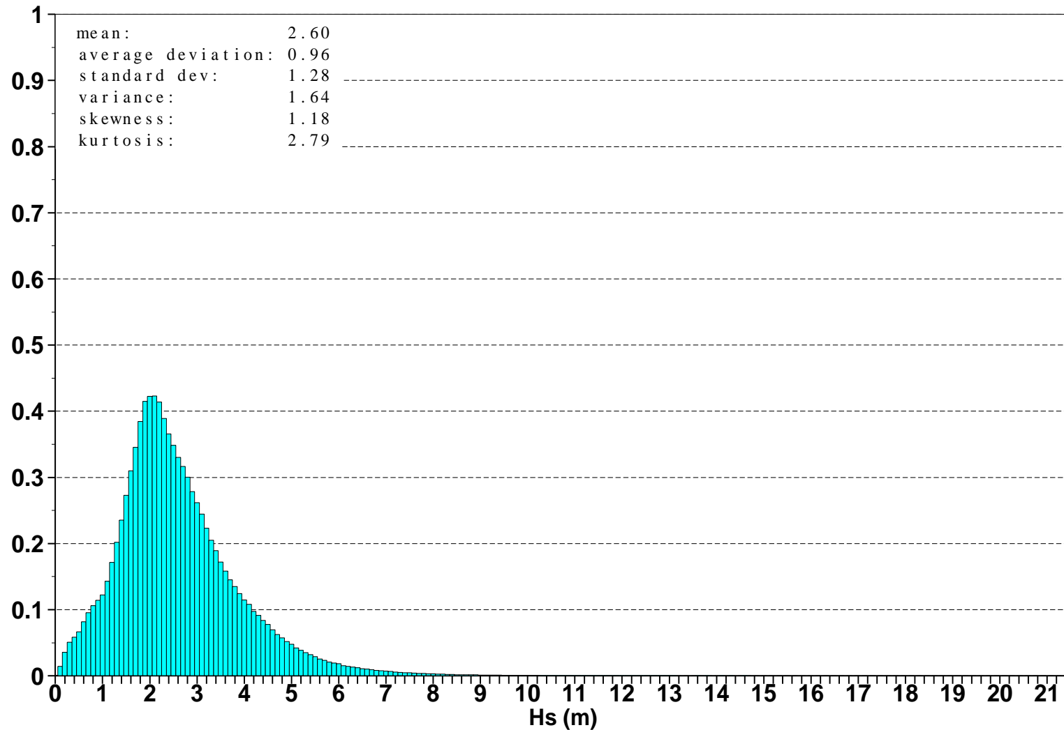
Figure 16: Global distribution of ECMWF wave heights for March 2010
