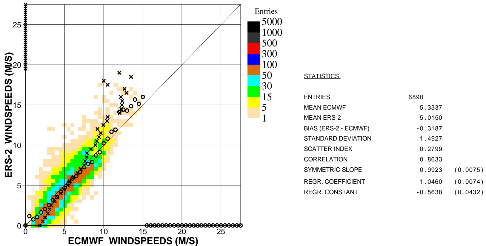
Figure 8. Comparison of ECMWF wind speed results with ERS2 Altimeter wind speed data for March 2010 (tropics)
