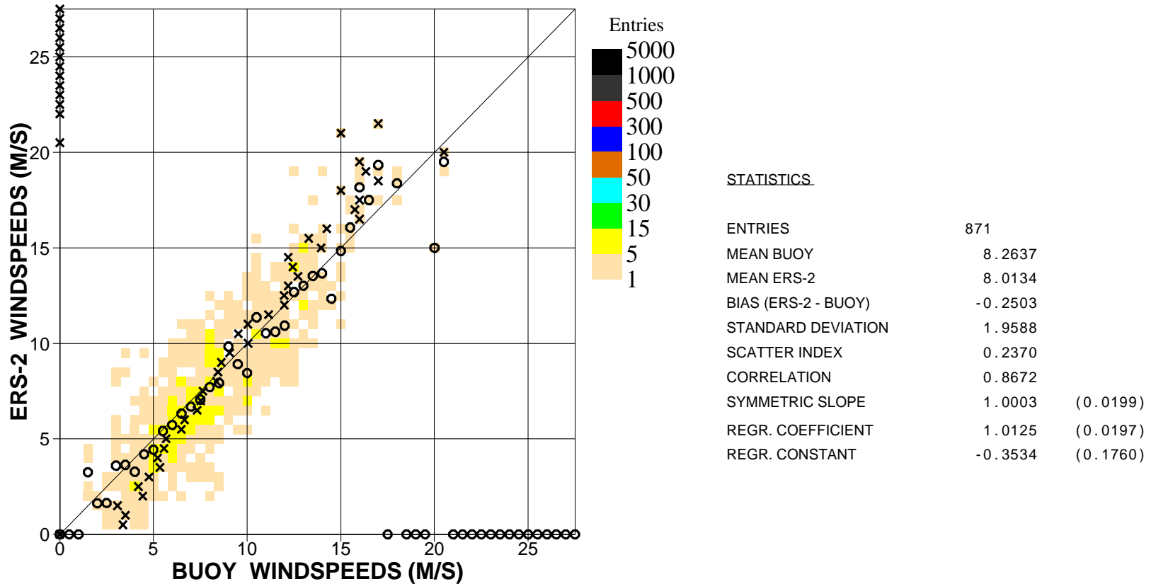
Figure 10. Comparison of buoy wind speed observations with ERS2 Altimeter wind speed data for March 2010 (global)
