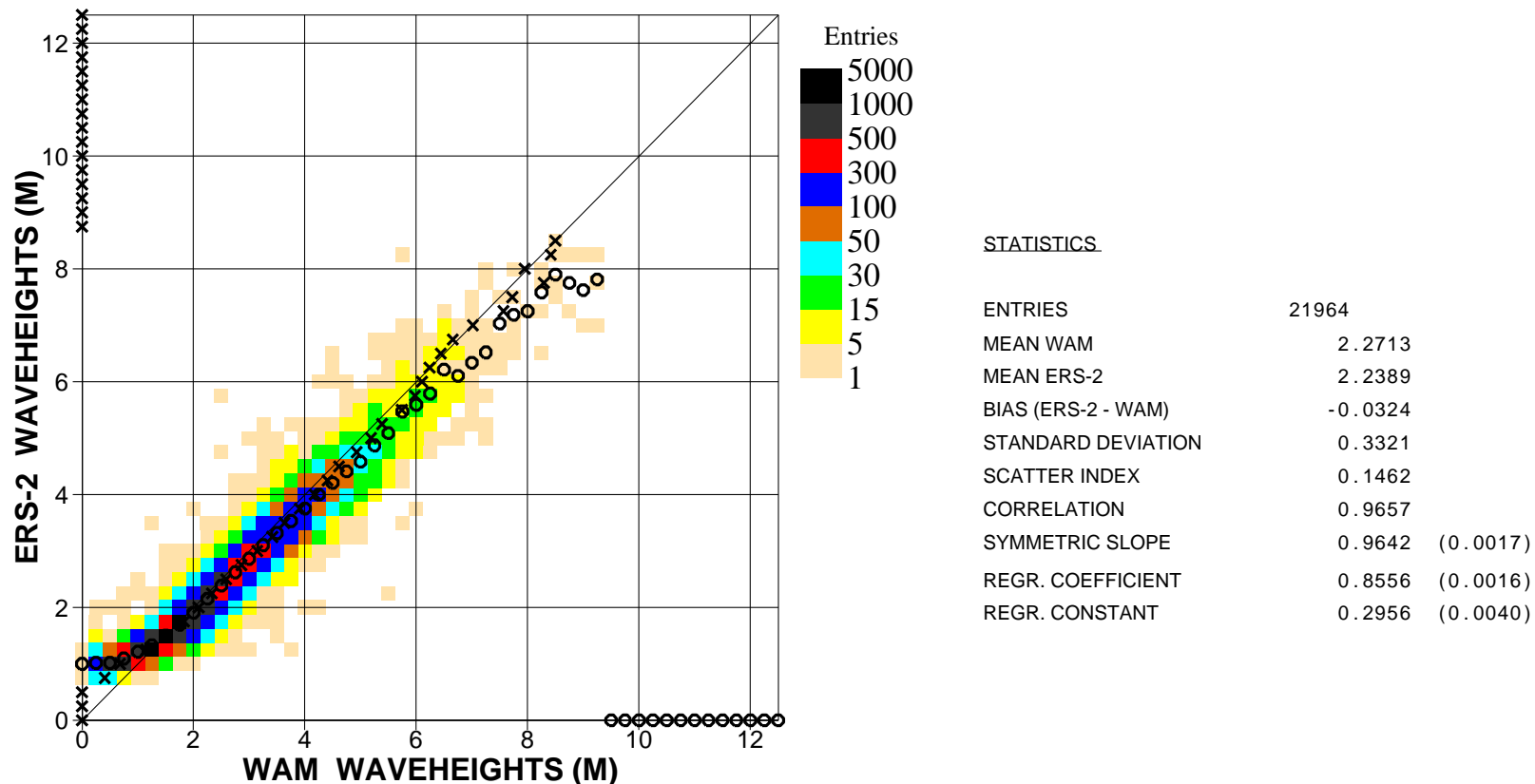
Figure 17. Comparison of ECMWF wave height results with ERS2 Altimeter wave height data for March 2010 (global)
