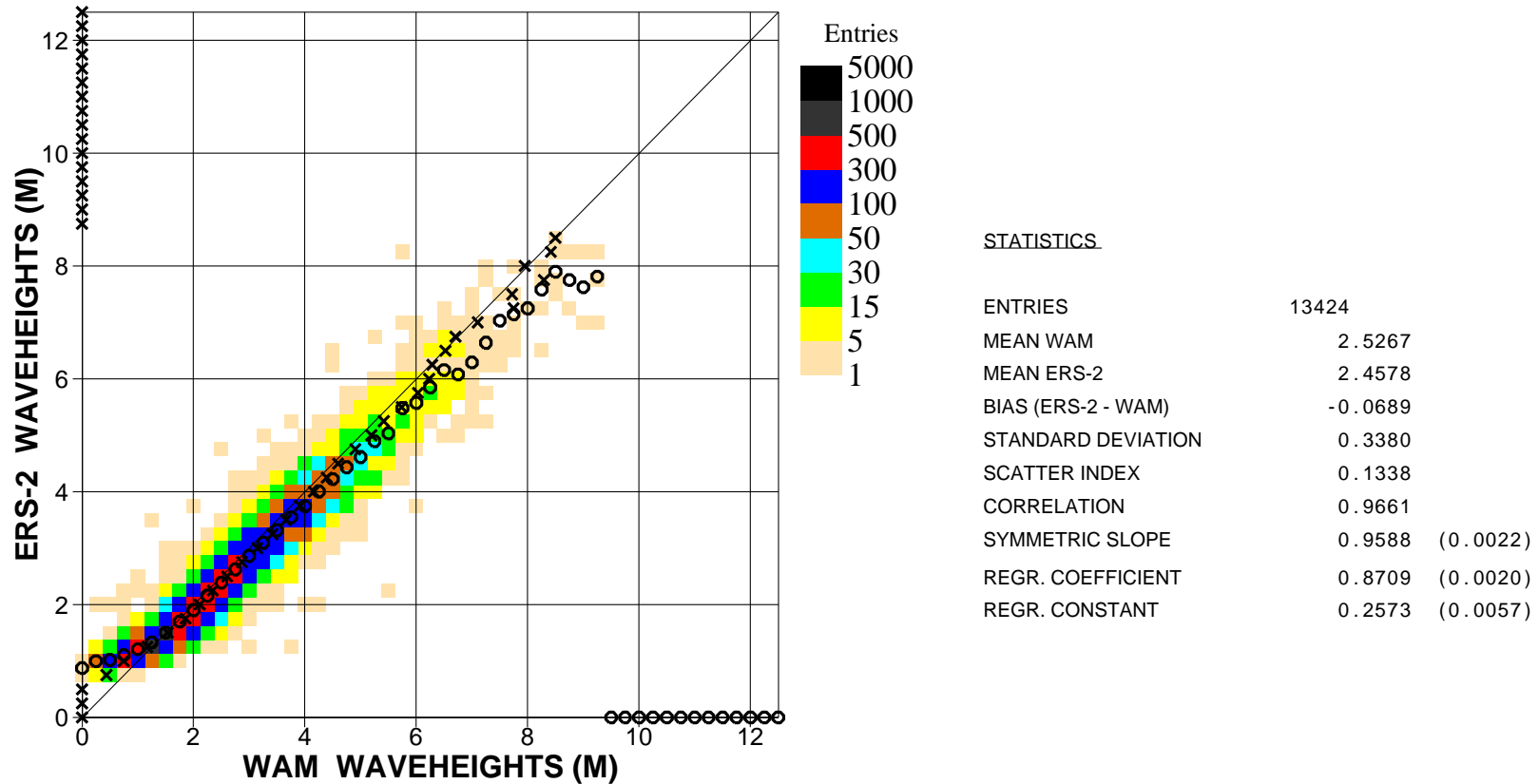
Figure 18. Comparison of ECMWF wave height results with ERS2 Altimeter wave height data for March 2010 (n.hem.)
