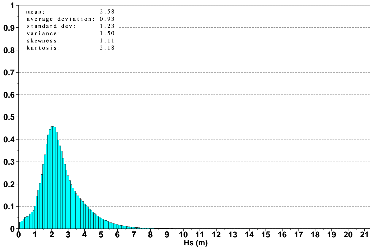
Figure 16: Global distribution of ECMWF wave heights for April 2001
