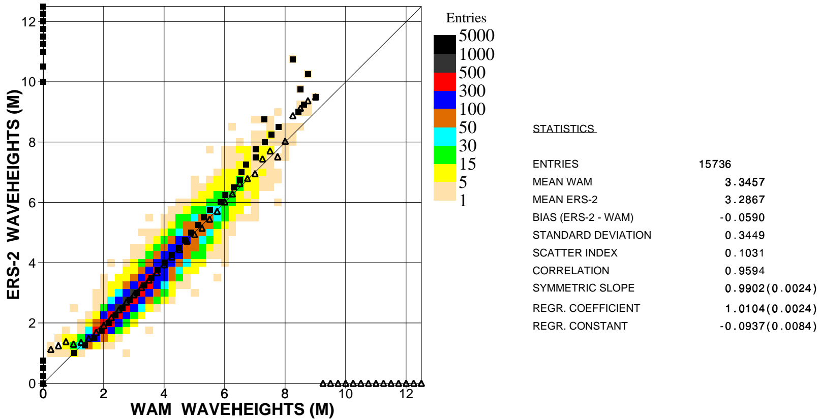
Figure 20. Comparison of ECMWF wave height results with ERS2 Altimeter wave height data for April 2001 (s.hem.)
