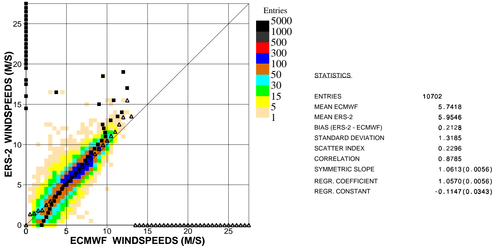
Figure 8. Comparison of ECMWF wind speed results with ERS2 Altimeter wind speed data for April 2001 (tropics)
