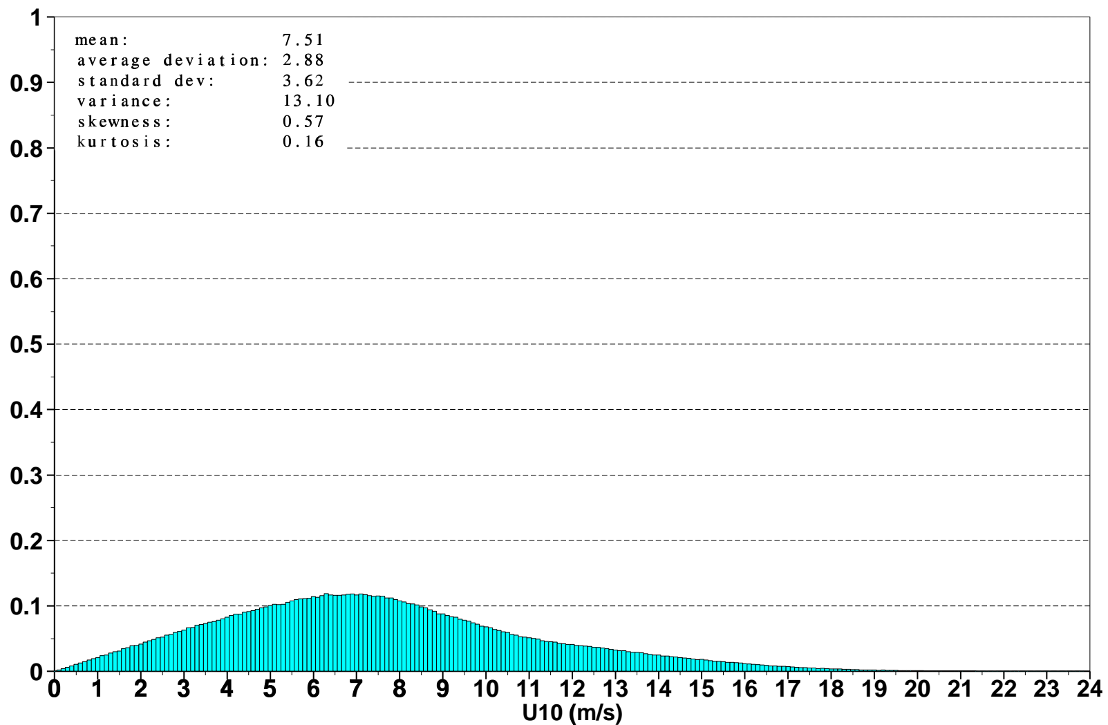
Figure 5: Global distribution of ECMWF ocean surface wind speeds for April 2001
