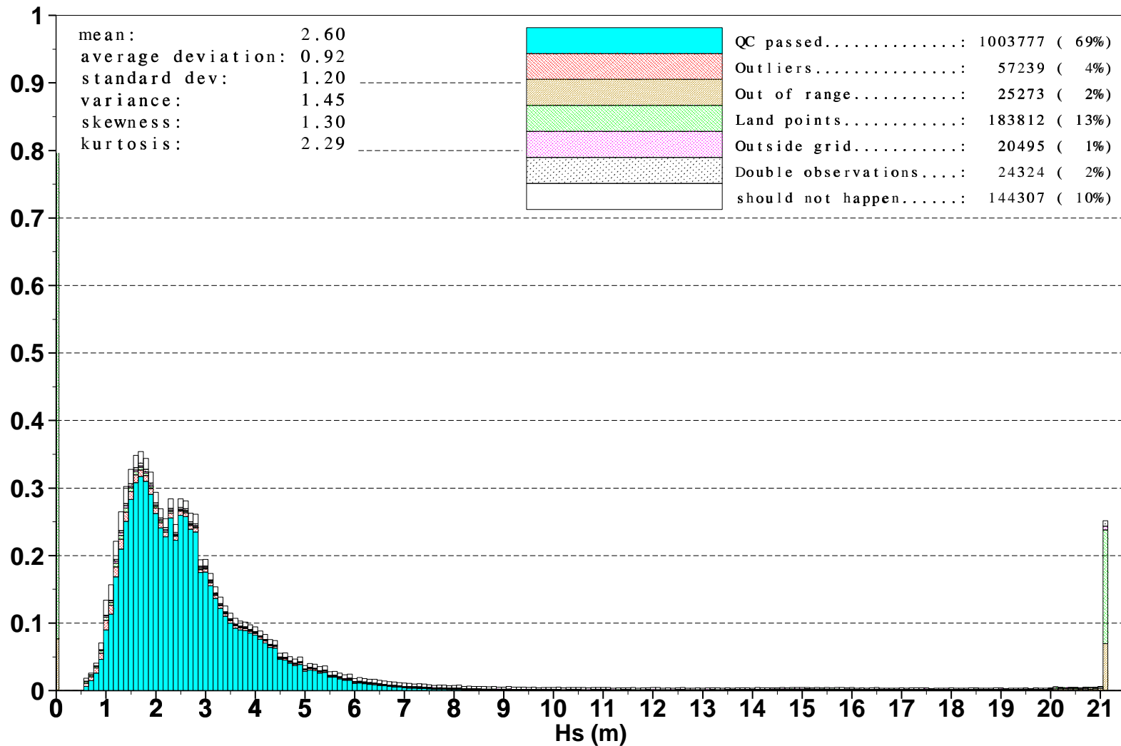
Figure 14: Distribution of the ERS-2 Altimeter wave heights after QC for April 2001
