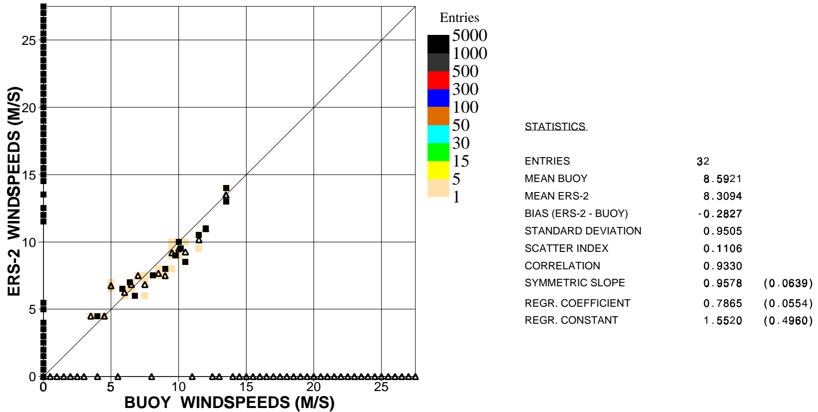
Figure 12. Comparison of buoy wind speed observations with ERS2 Altimeter wind speed data for April 2001 (hawaii)
