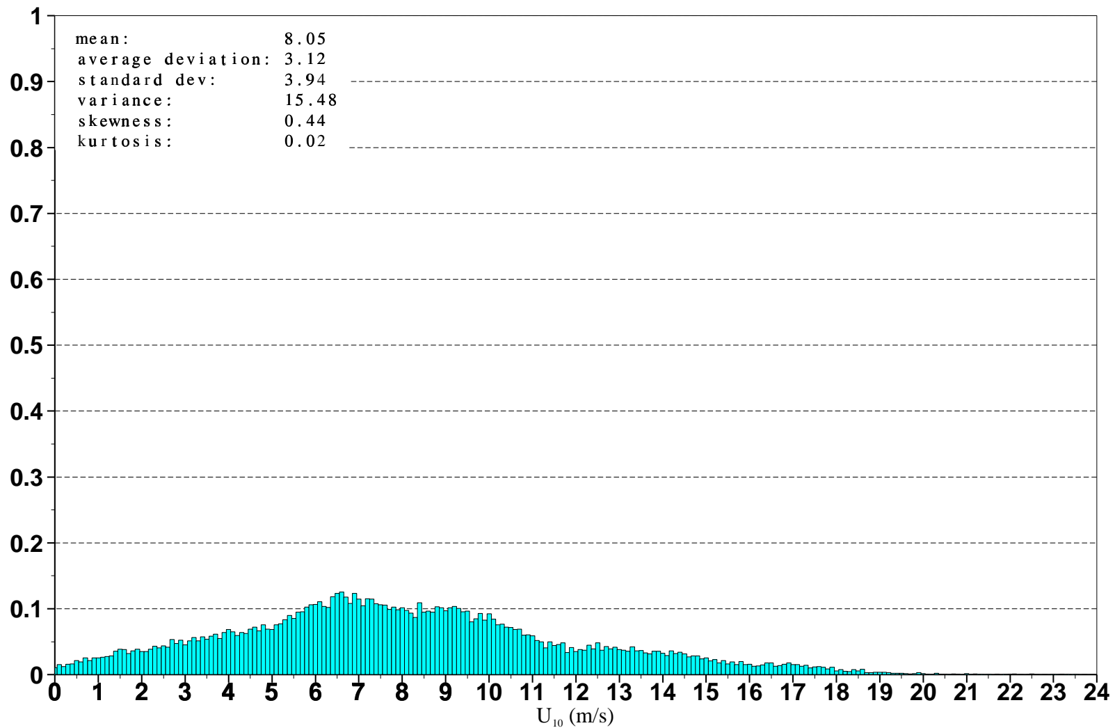
Figure 4: Distribution of ERS-2 Altimeter wind speeds after along track averaging for April 2001
