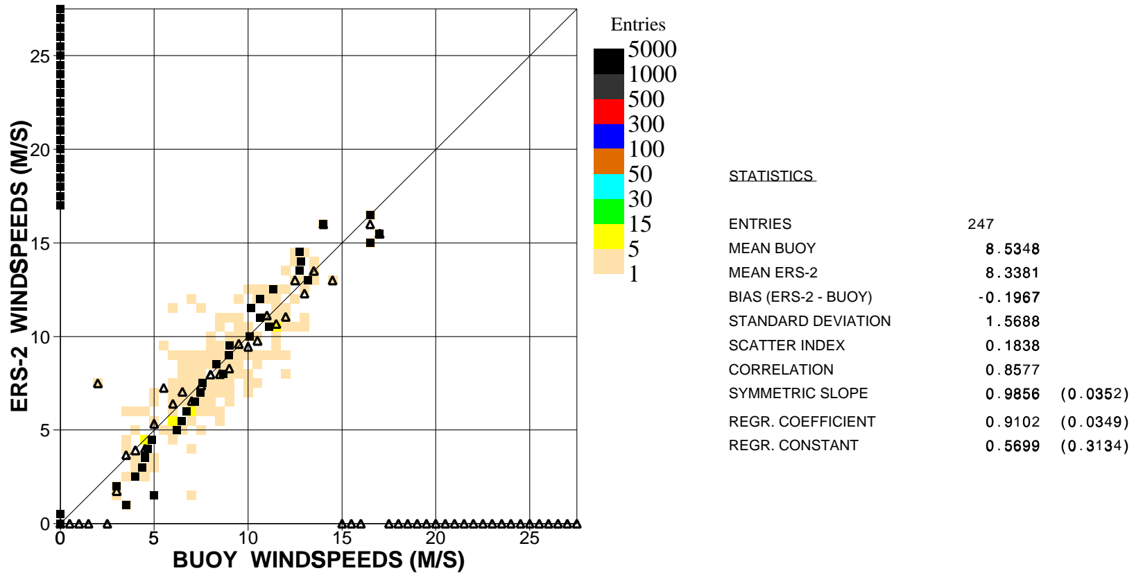
Figure 10. Comparison of buoy wind speed observations with ERS2 Altimeter wind speed data for April 2001 (global)
