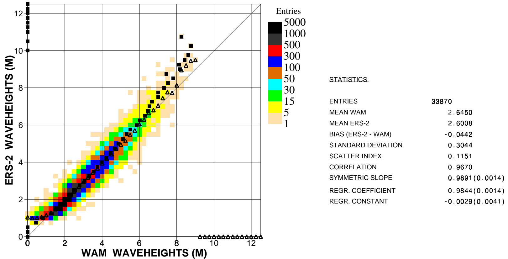
Figure 17. Comparison of ECMWF wave height results with ERS2 Altimeter wave height data for April 2001 (global)
