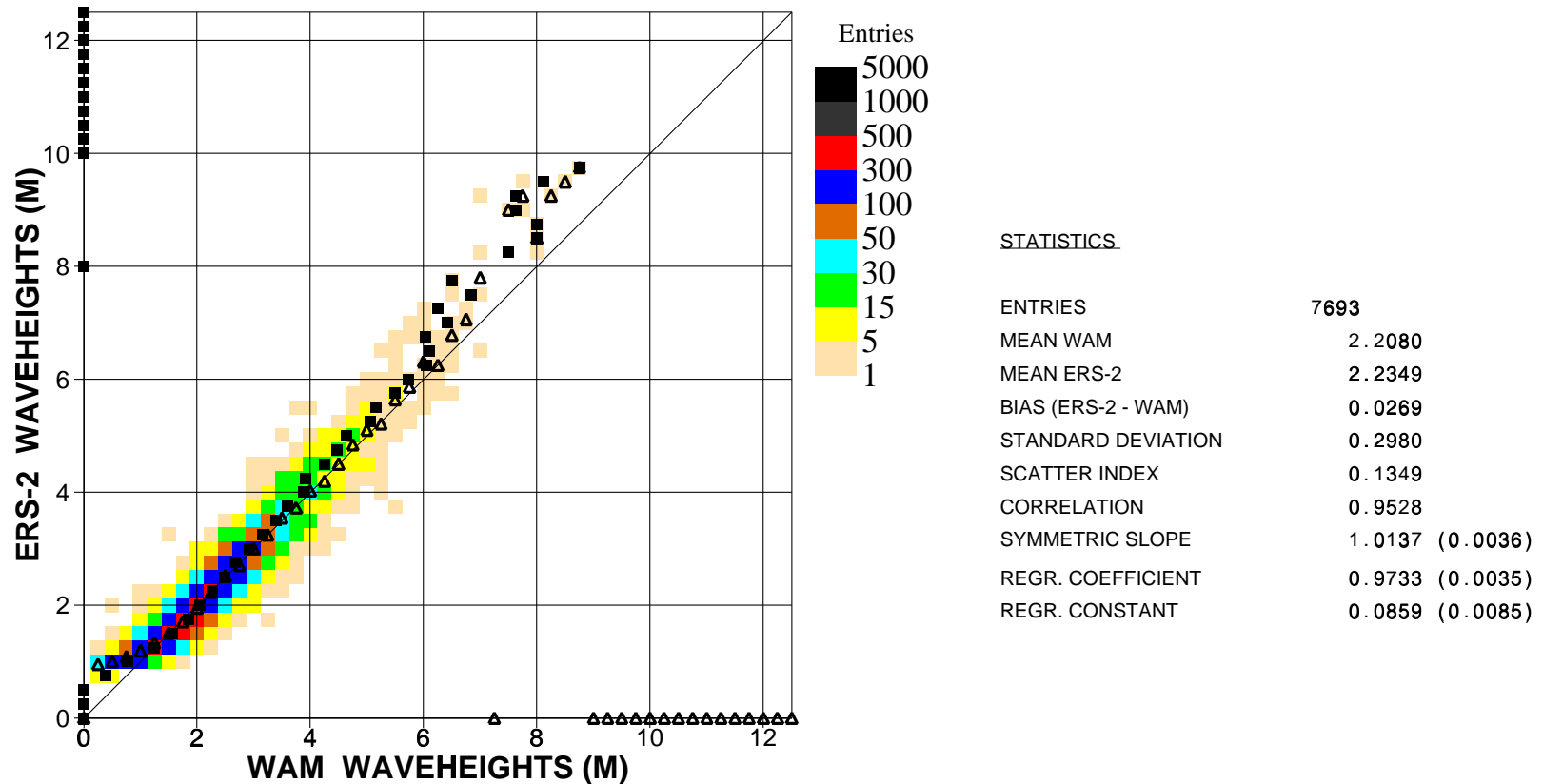
Figure 18. Comparison of ECMWF wave height results with ERS2 Altimeter wave height data for April 2001 (n.hem.)
