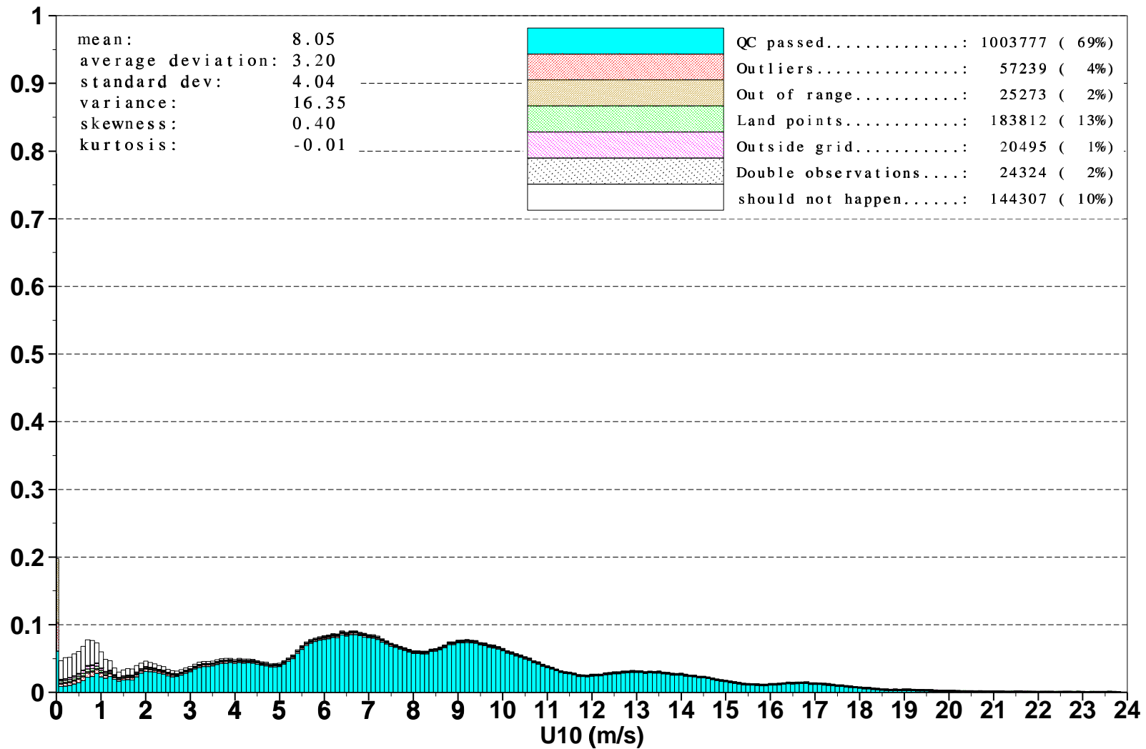
Figure 3: Distribution of the ERS-2 Altimeter wind speeds after QC for April 2001
