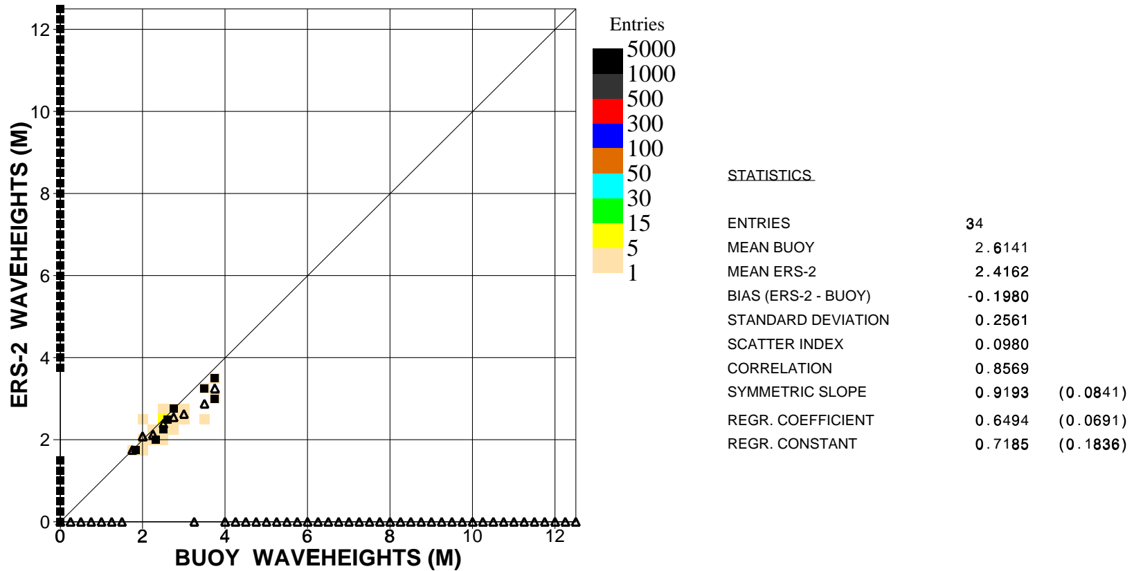
Figure 23. Comparison of buoy wave height observations with ERS2 Altimeter wave height data for April 2001 (hawaii)
