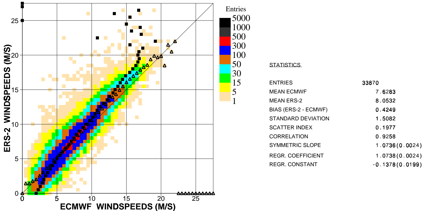
Figure 6. Comparison of ECMWF wind speed results with ERS2 Altimeter wind speed data for April 2001 (global)
