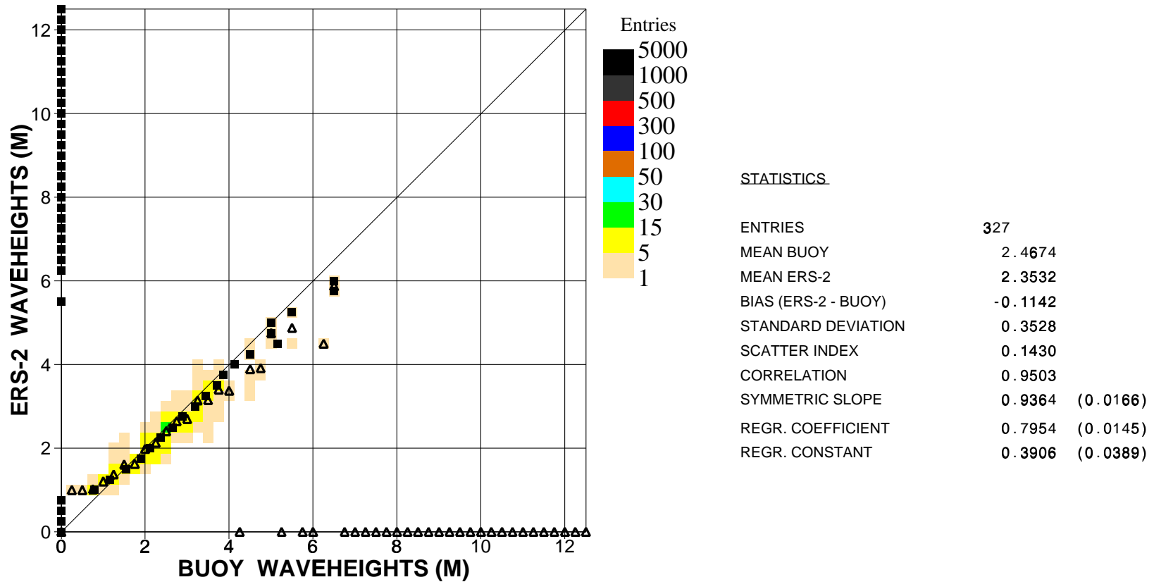
Figure 21. Comparison of buoy wave height observations with ERS2 Altimeter wave height data for April 2001 (global)
