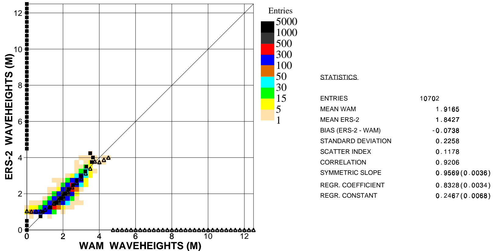
Figure 19. Comparison of ECMWF wave height results with ERS2 Altimeter wave height data for April 2001 (tropics)
