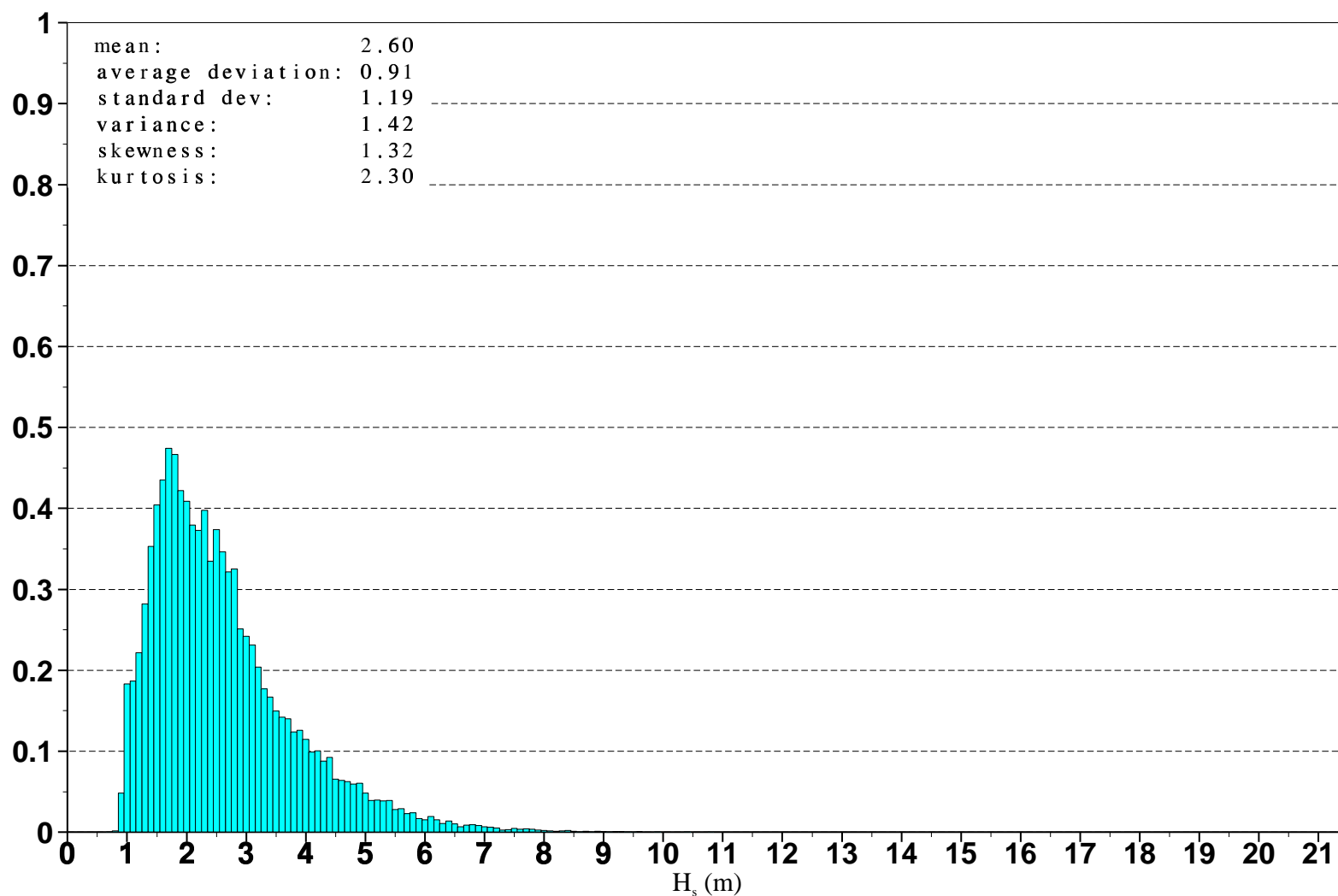
Figure 15: Distribution of ERS-2 Altimeter wave heights after along track averaging for April 2001
