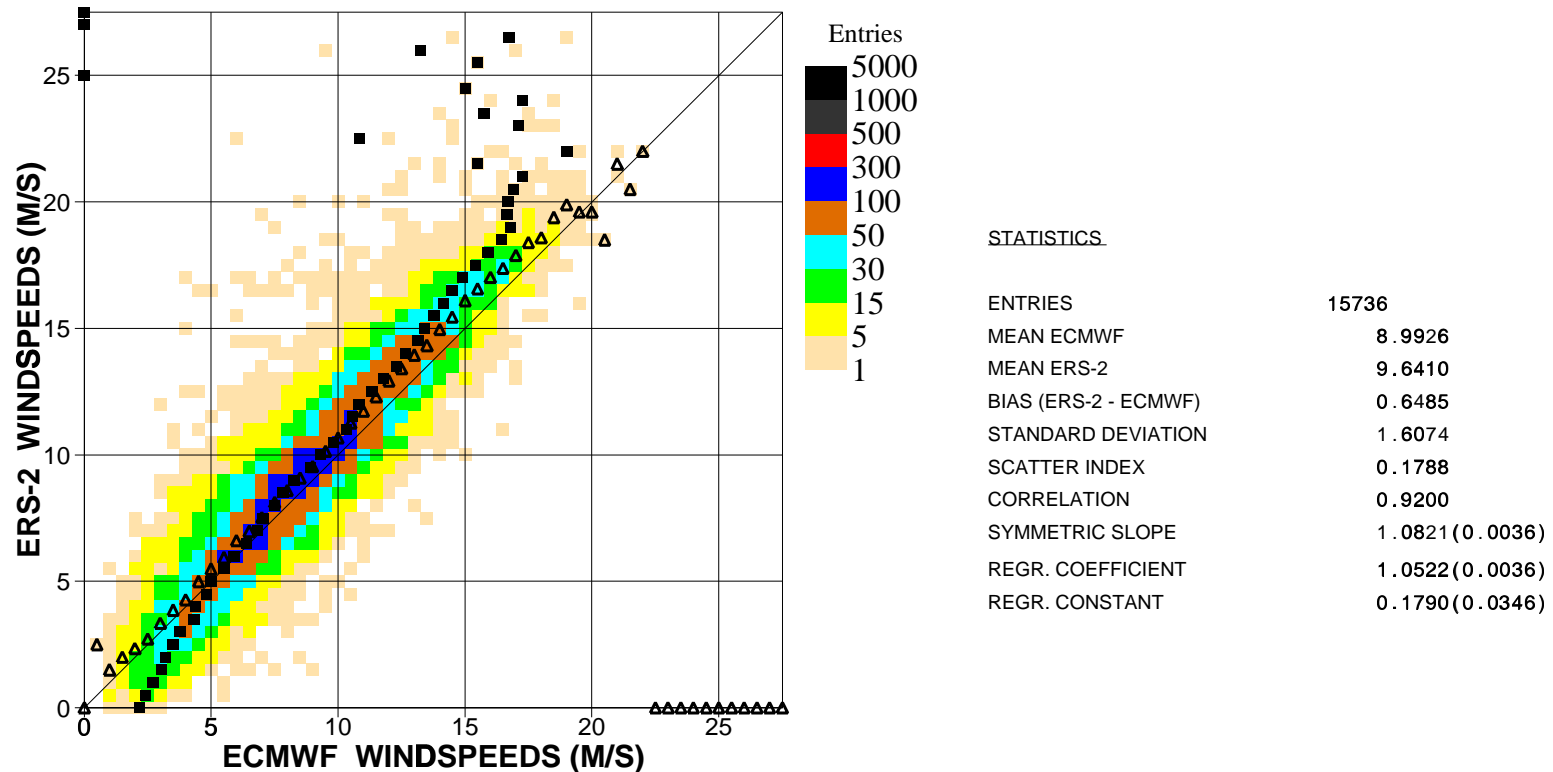
Figure 9. Comparison of ECMWF wind speed results with ERS2 Altimeter wind speed data for April 2001 (s.hem.)
