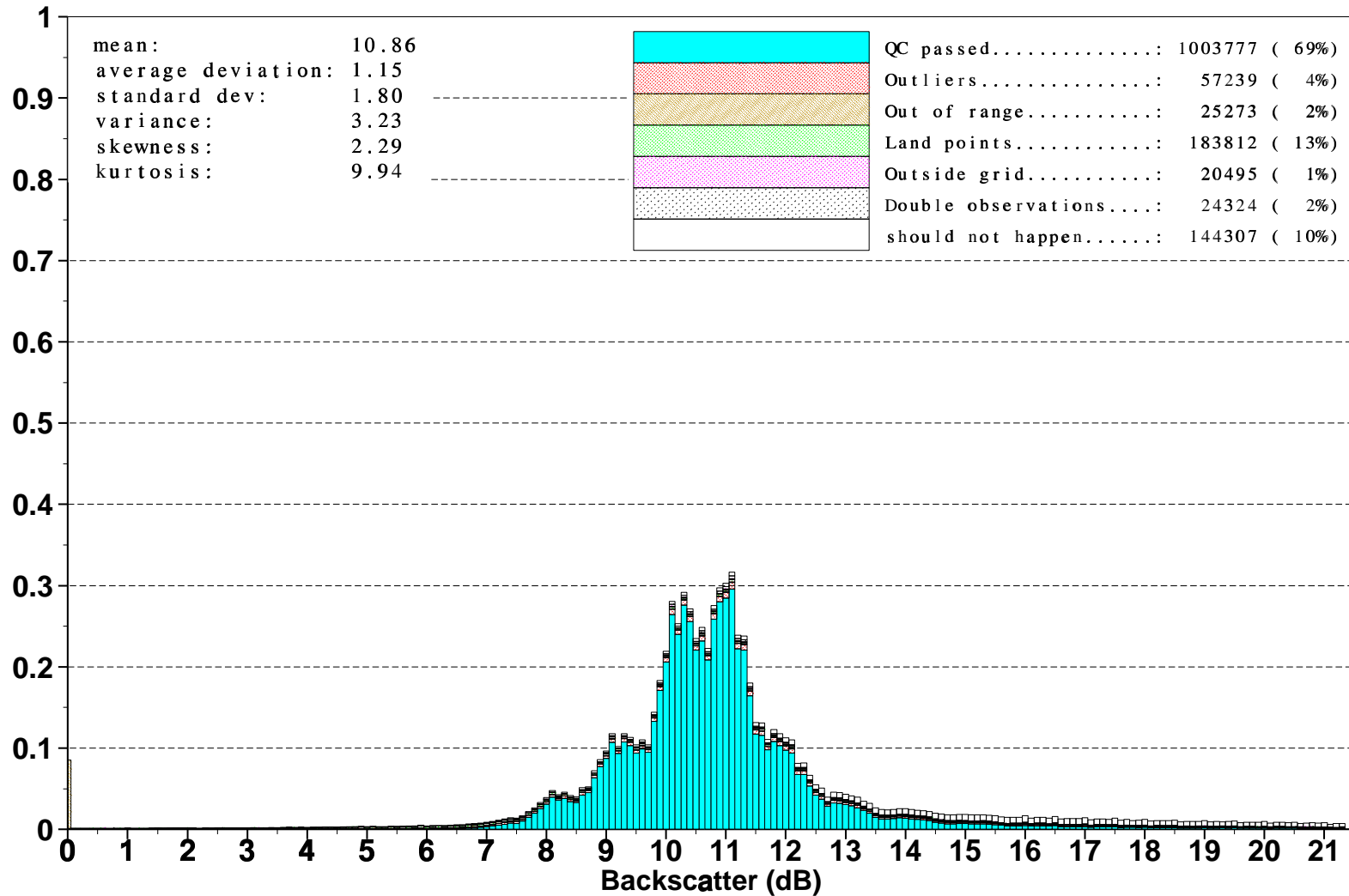
Figure 2: Distribution of the ERS-2 Altimeter backscatter after QC for April 2001
