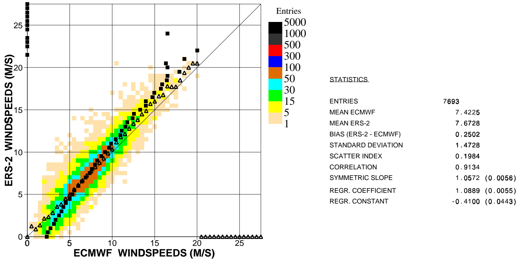
Figure 7. Comparison of ECMWF wind speed results with ERS2 Altimeter wind speed data for April 2001 (n.hem.)
