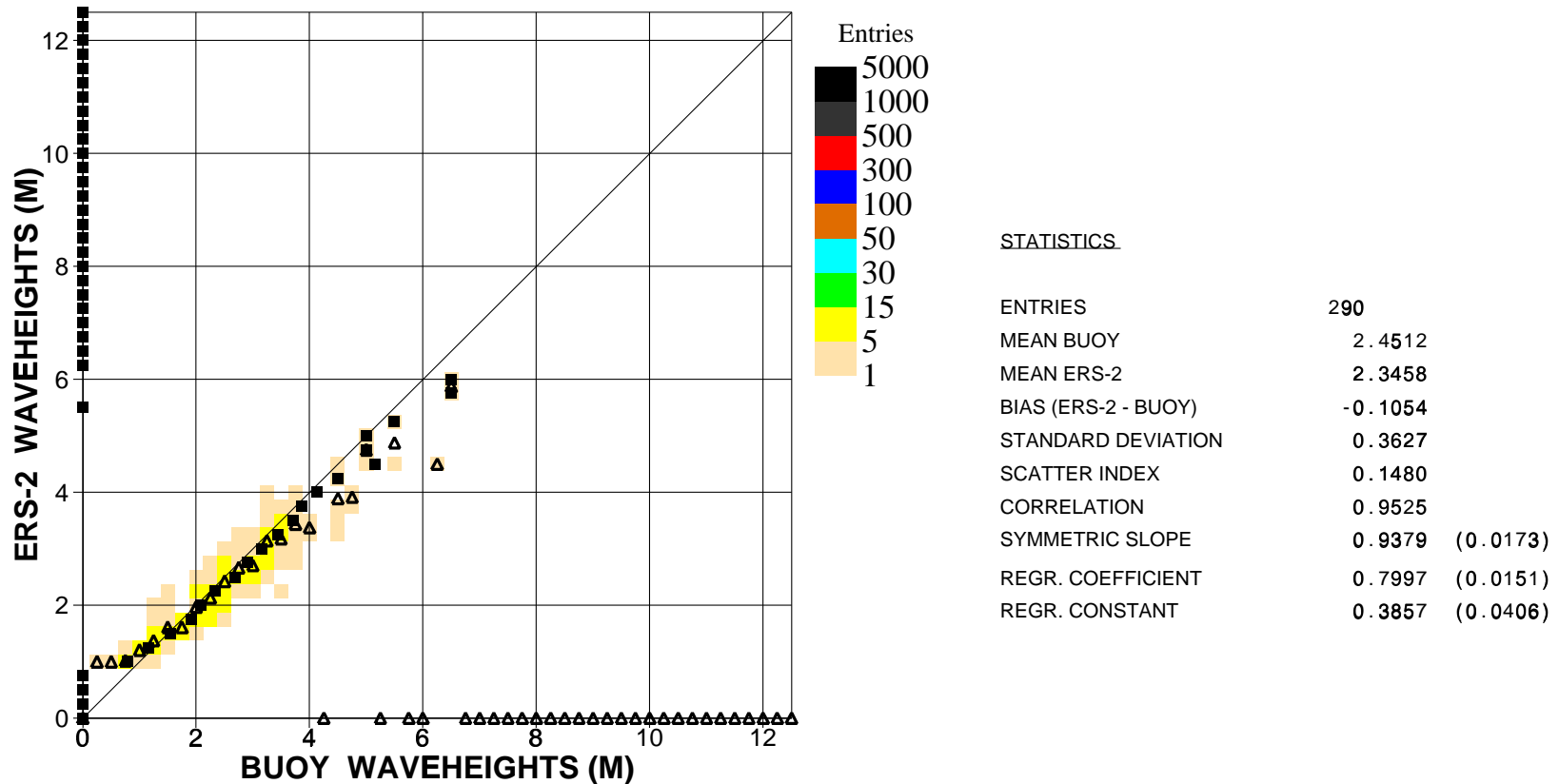
Figure 22. Comparison of buoy wave height observations with ERS2 Altimeter wave height data for April 2001 (n.hem.)
