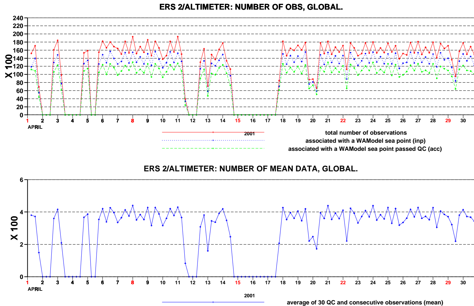
Figure 1: Time series of data reception for ERS-2 Altimeter data for April 2001
