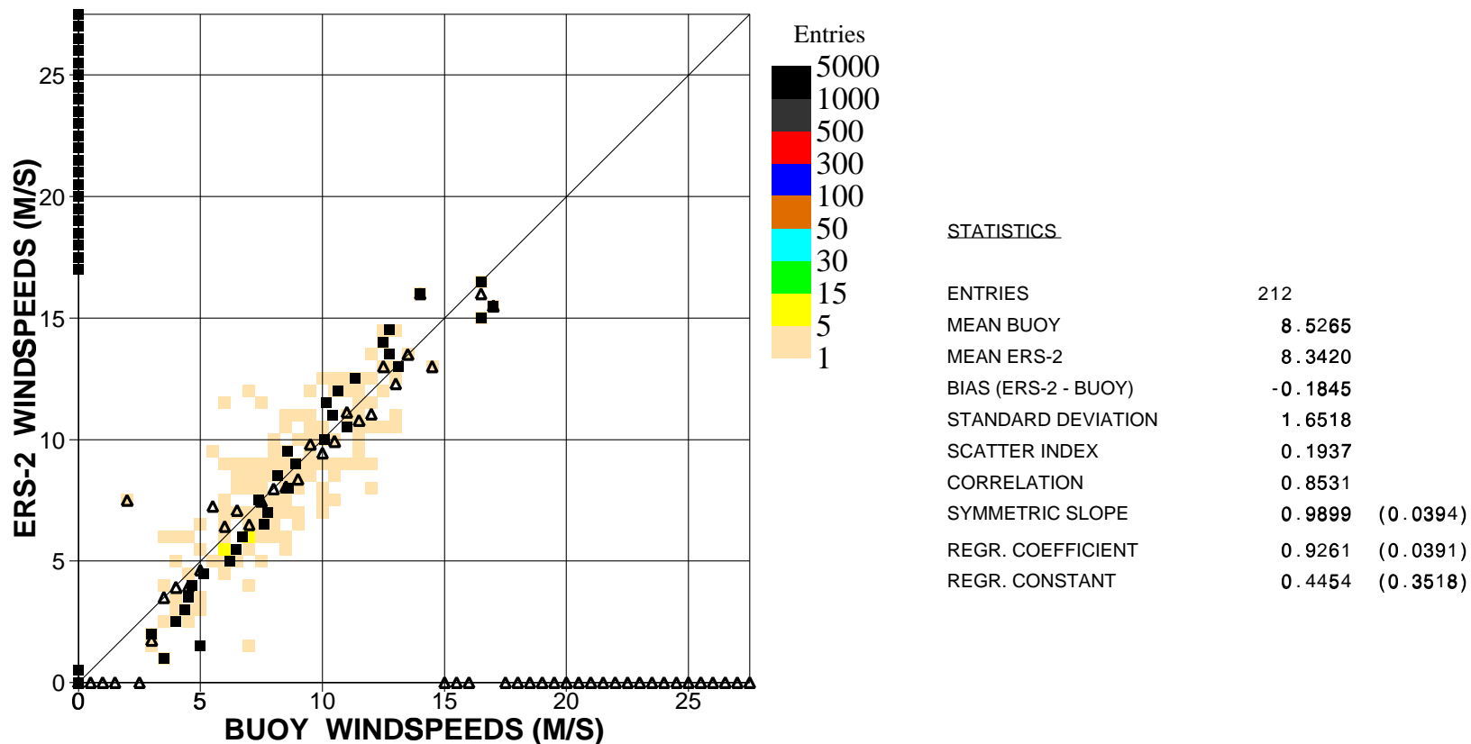
Figure 11. Comparison of buoy wind speed observations with ERS2 Altimeter wind speed data for April 2001 (n.hem.)
