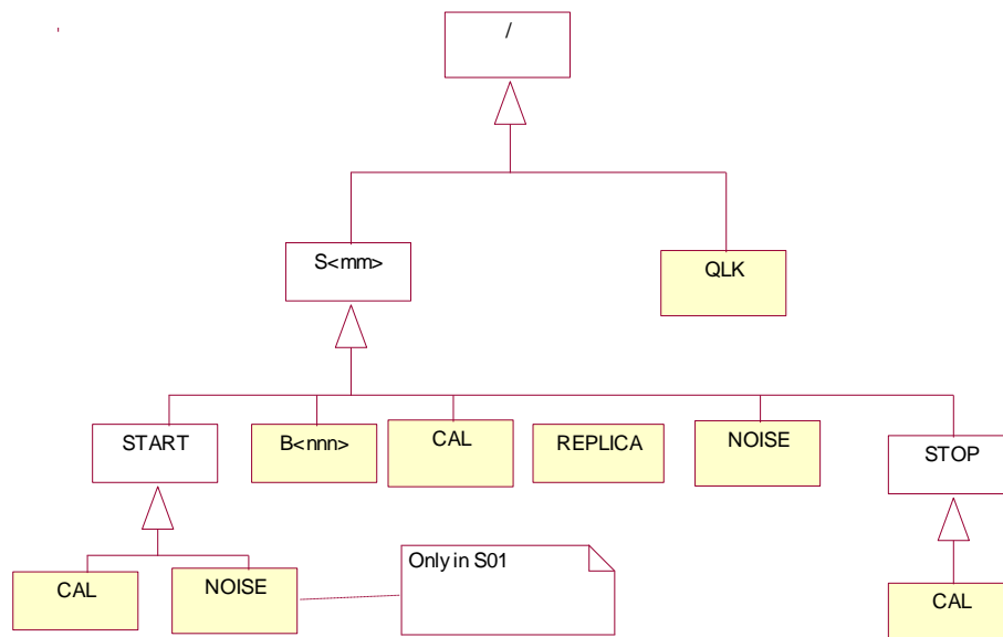
Figure 20 – ScanSAR Mode – Level 0
