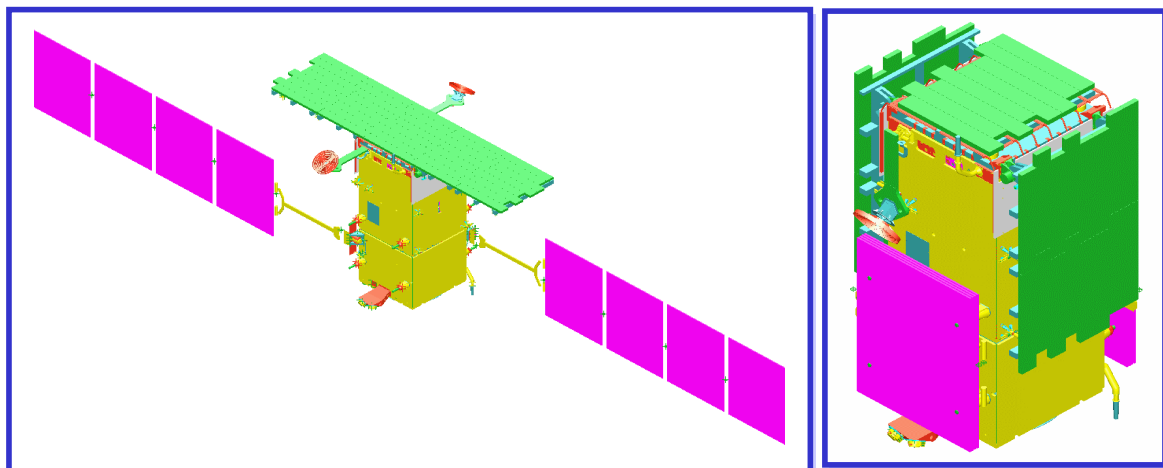
Figure 3 - SAR Satellite (Deployed and Stowed Configurations)
