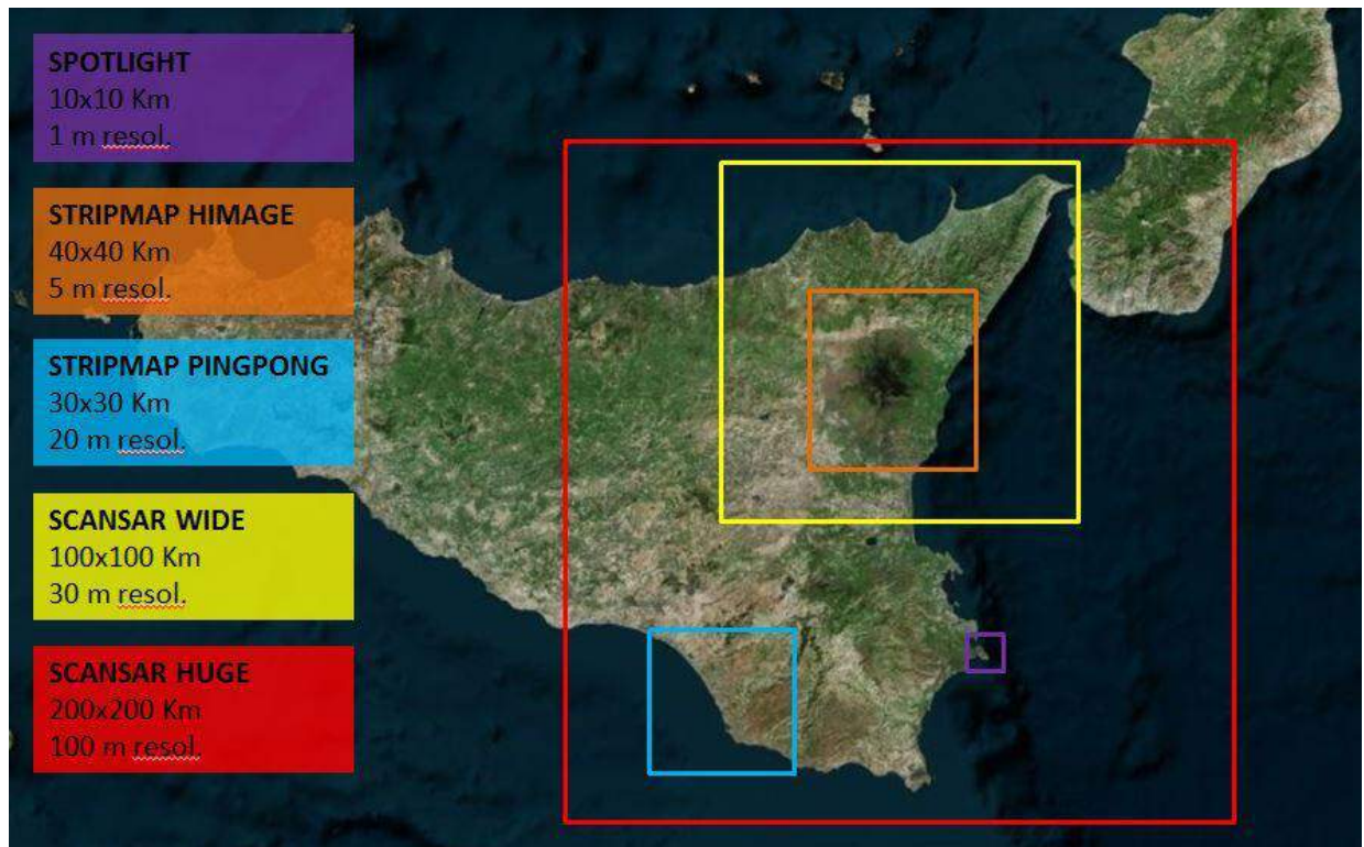
Figure 12 – A pictorial view of the 5 major types of COSMO-SkyMed Acquisition Modes
