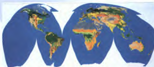
This landcover map shows global vegetation at 1km resolution. Multispectral imagers are an important source of inventory information for monitoring climate change
