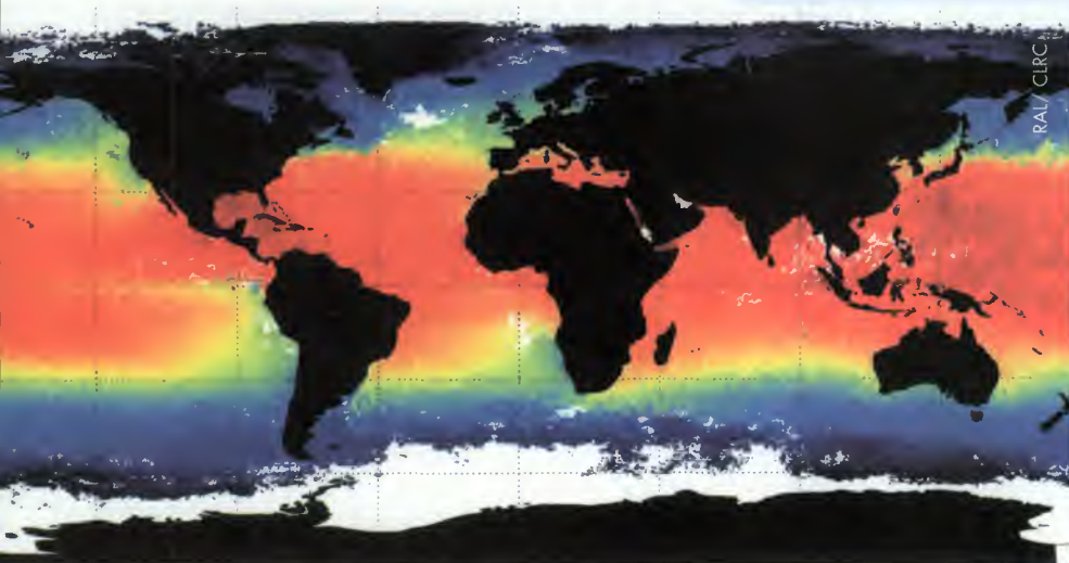
Global sea surface temperature map produced using ATSR-2 data - inaccuracies caused by atmospheric effects can be removed from multi-directional radiometer data enabling precise measurements to be made
