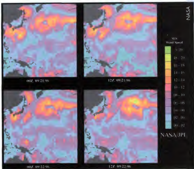
Scatterometer data can measure the horizontal wind speed and direction over sea surfaces. NSCAT data was used in September 1996 to monitor the size and movement of Typhoons Violet and Tom in the western Pacific
