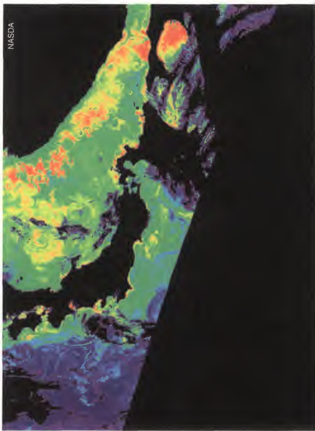
Ocean colour instruments provide information on marine photosynthesis and productivity. The wide-area coverage of these instruments is important for studying ocean processes
