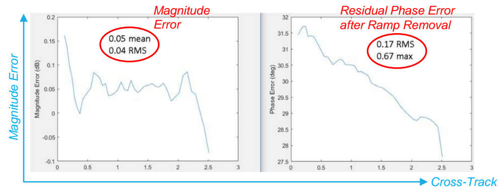
SLC point-target response differences across the swath of simulations using “nominal” and “deformed” antenna patterns; (left) small <0.1dB magnitude difference, (right) an approximate linear phase ramp, which when removed resulting in small (<0.2°) residual phase error
