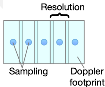
Figure 12: Difference between sampling and Doppler footprint
