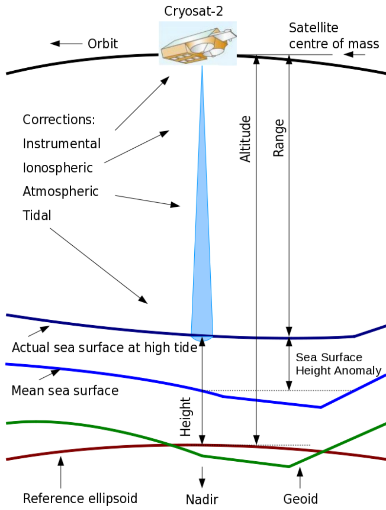
Figure 1: Basic altimetry terms and applicable corrections over open ocean
