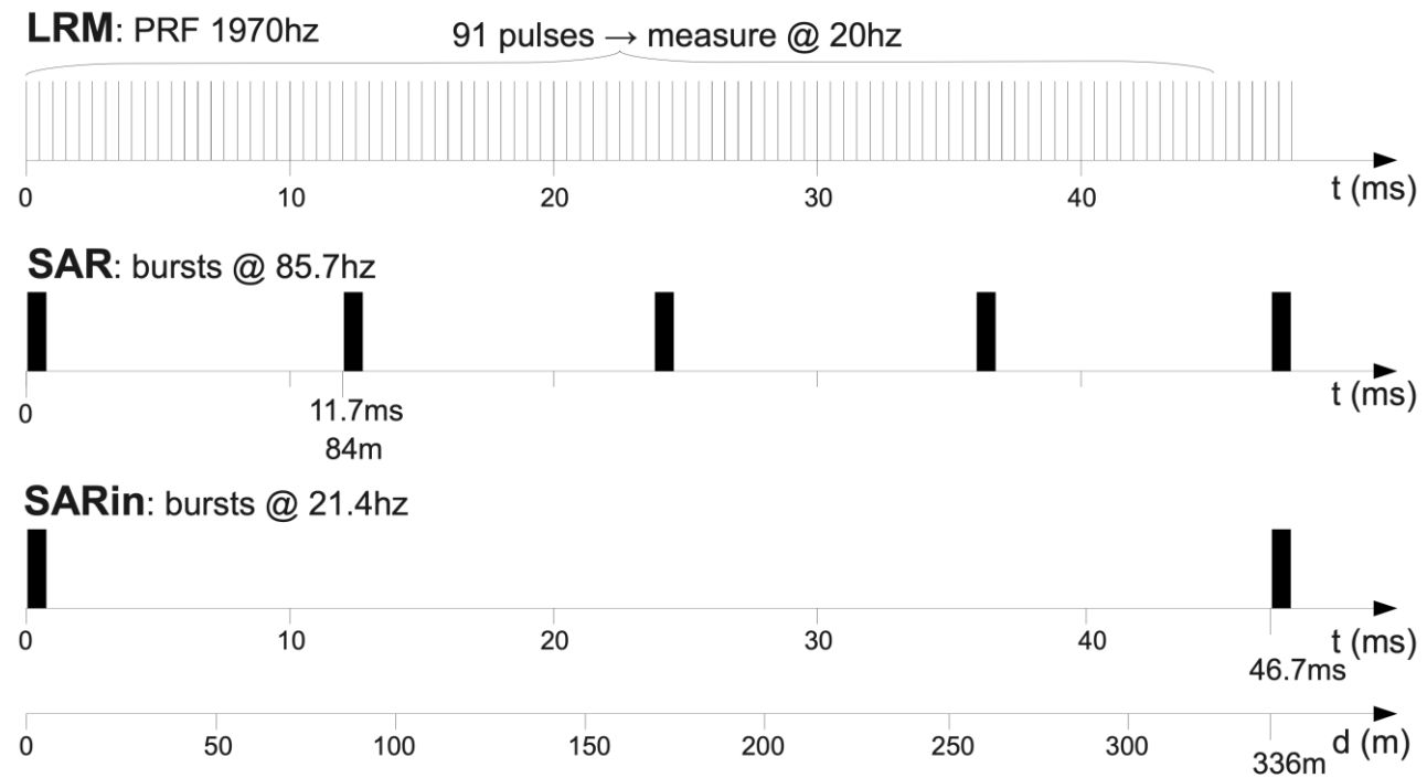
Figure 6: CryoSat Chronogram
