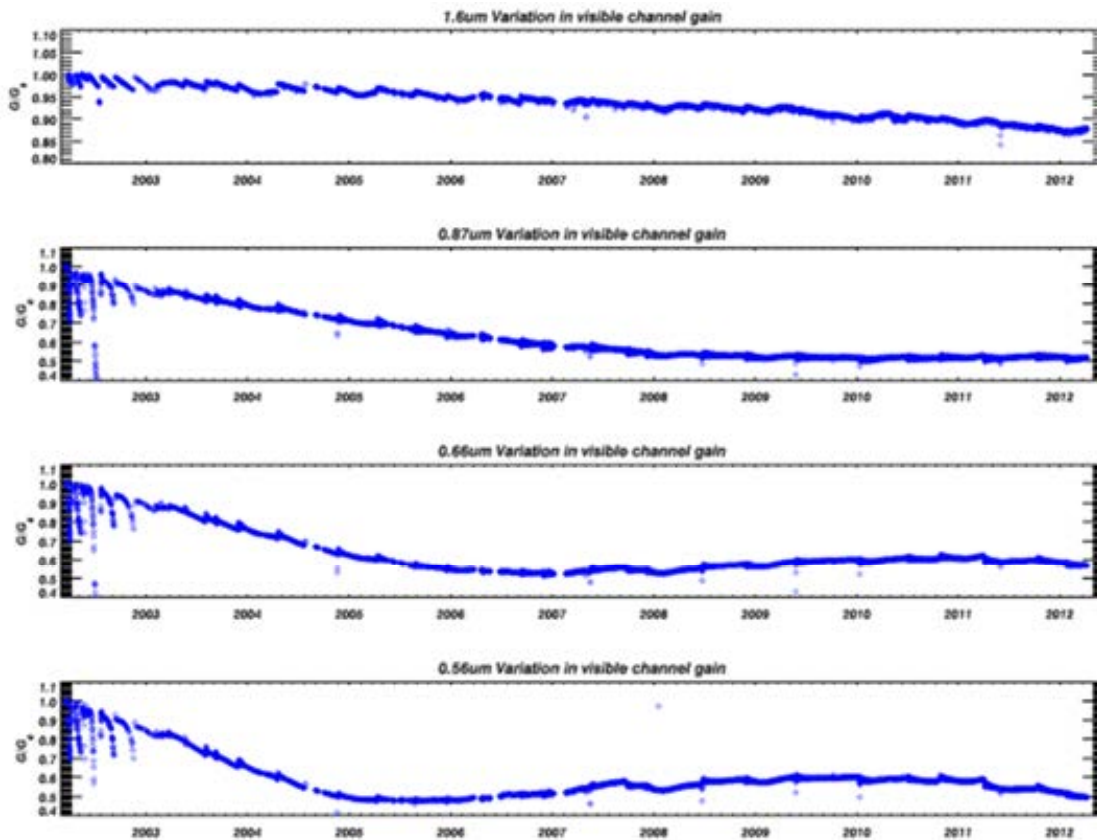
Figure 4. The 1.6 µm, 0.87 µm, 0.66 µm and 0.56 µm visible channel calibration levels, G , relative to the level at the start of the mission, G_0 (taken from RD.1).
