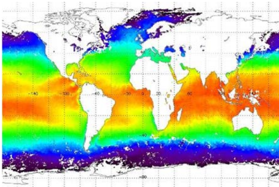
Figure 14. Monthly average dual-view SST, with a data range of 270 – 305 K for March 2012.
