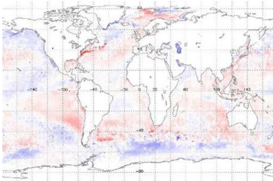
Figure 18. Anomaly map of dual-view SST for March 2012.
