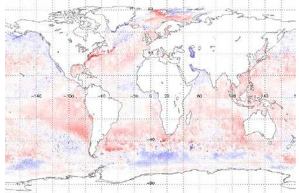
Figure 19. Anomaly map of nadir-view SST for March 2012
