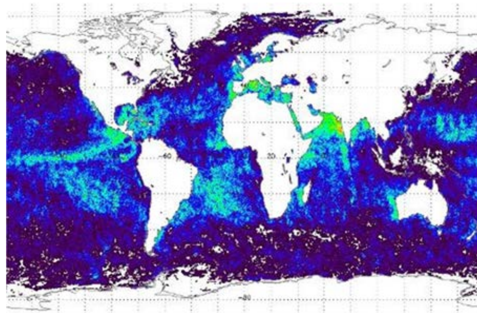
Figure 17. Number of contributory orbits to the calculation of the SST, with a colour key range of 0 to 16 (maximum value) for March 2012.
