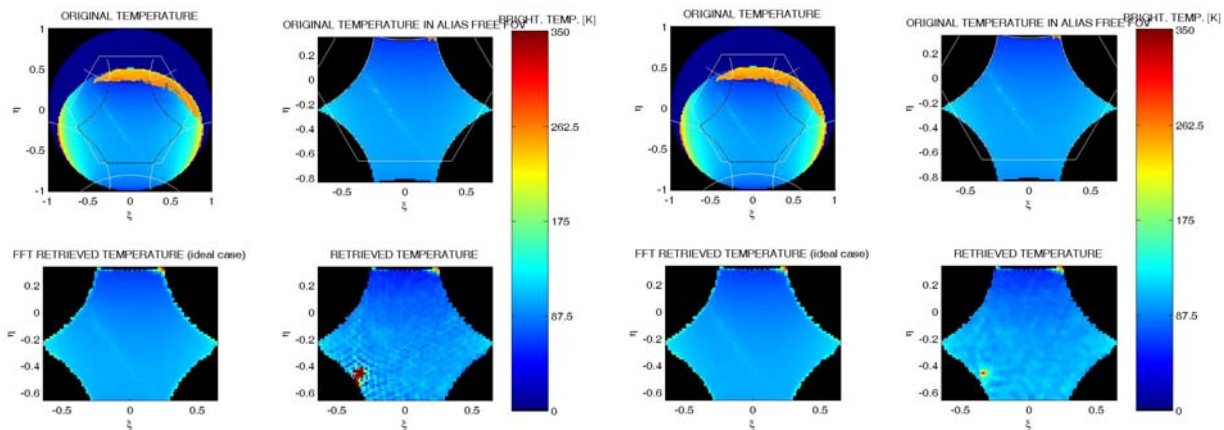
Figure 4: Uncorrected SUN effect (left) and Corrected SUN effect over sea (right)
