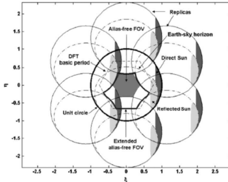
Figure 3: Areas in FOV for a 2-D aperture synthesis Y-shaped interferometric radiometer, with an antenna spacing of 0.875 wavelengths, 32° array tilt, 30° array steering and 755 km platform height [RA.01]
