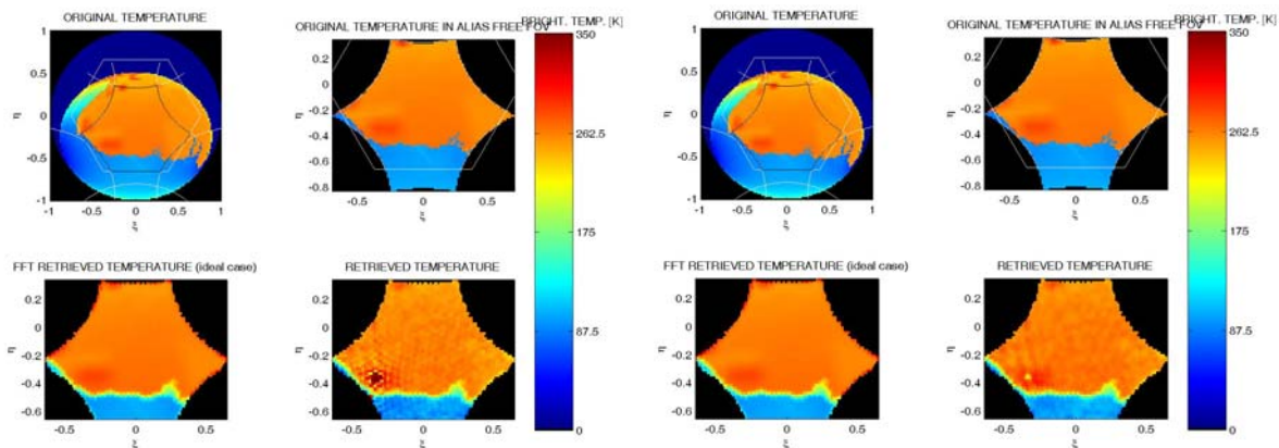
Figure 5: Uncorrected SUN effect (left) and Corrected SUN effect over land (right)
