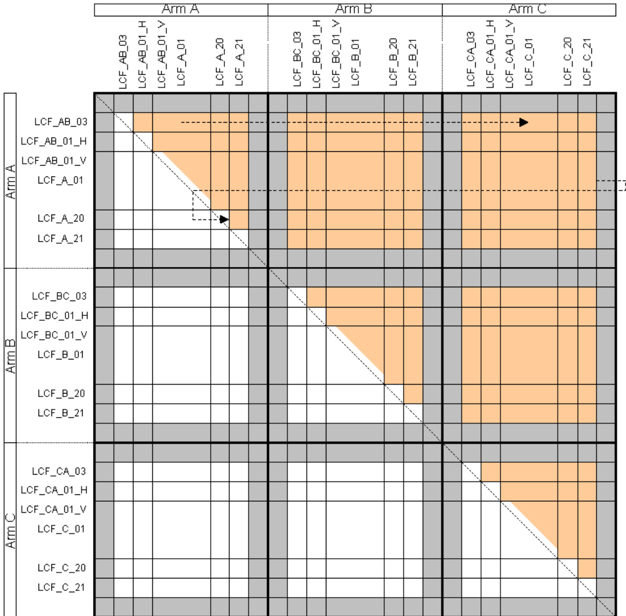
Figure 2: Ordering of calibrated visibilities structure (CALIB_VISIB)
