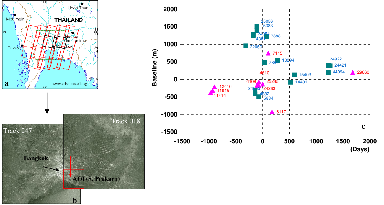
Fig.1 (a) Two scenes of ERS coverage (black squares) over Bangkok and its surroundings obtained for PSInSAR (b) Shows the Area of Interest (AOI) located southeast of Bangkok as the initial test site used for this study. (c) Shows temporal-spatial baseline distribution of the two interferometric stacks (magenta triangle: left stack, green square: right stack).
