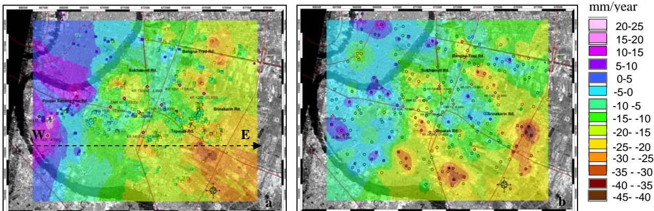
Fig.5. Derived spatial subsidence pattern from two interferometric stacks using PSInSAR technique. The left stack (a) contains 16 IFGMs, the W-E comparison profile is also indicated in black, the right stack (b) contains 10 IFGMs.
